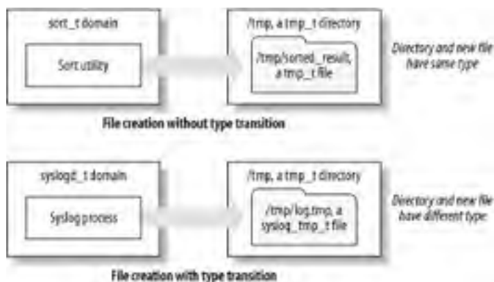
Figure 2-6. File creation and transition decisions
