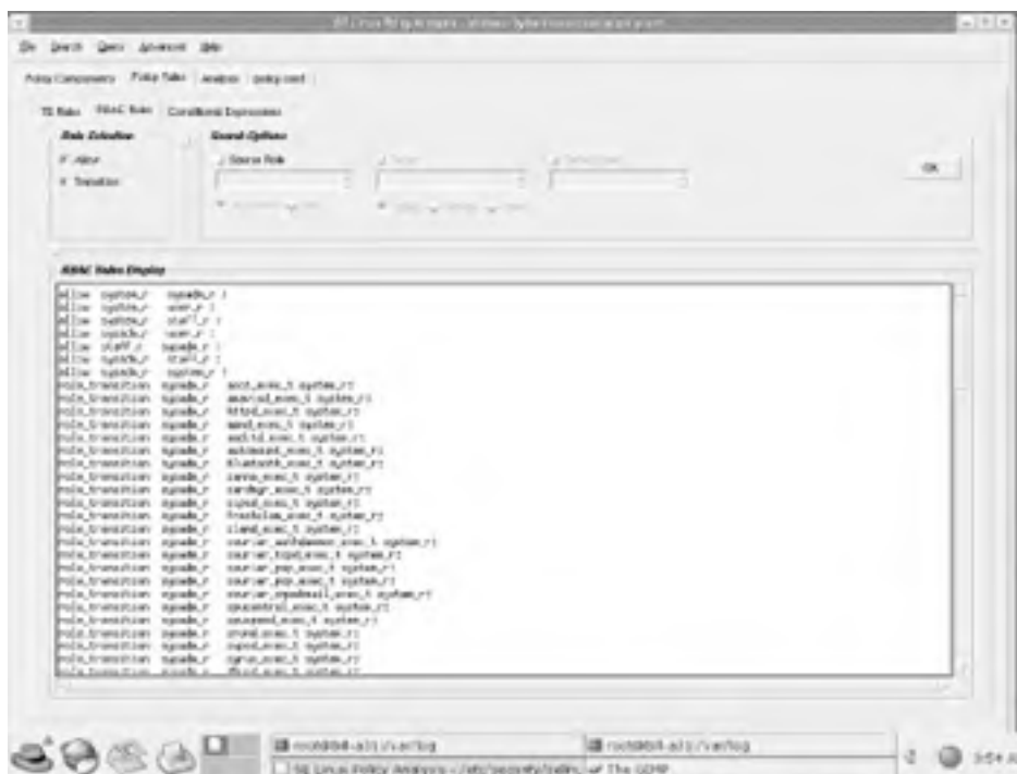
Figure 9-8. Apol's RBAC Rules tab
