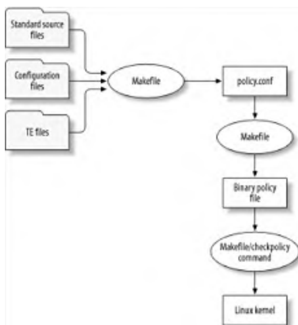
Figure 2-7. Creating and loading the SELinux binary policy file
