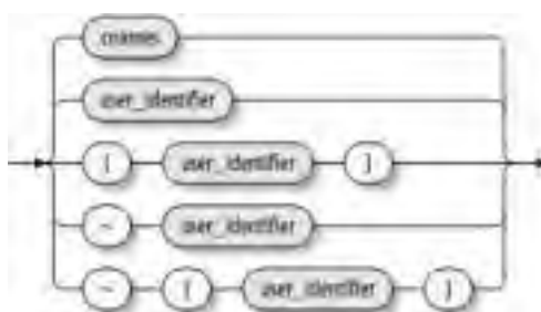
Figure 8-4. Syntax of user_names
