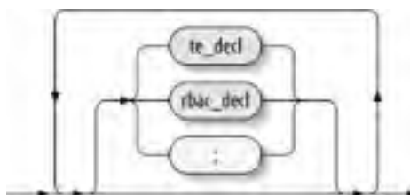
Figure 6-10. TE and RBAC declarations ( te_rbac )
