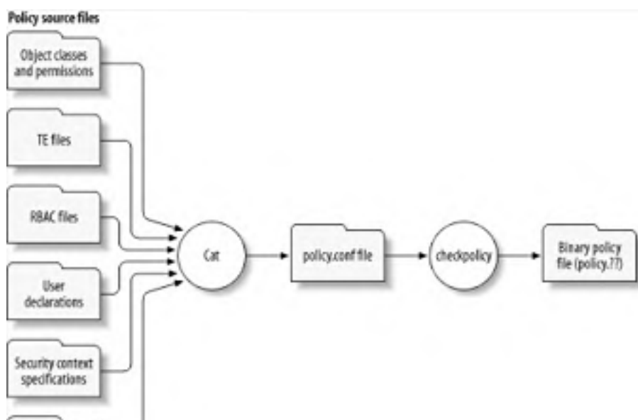
Figure 5-2. Transforming an SELinux policy from source to binary form
