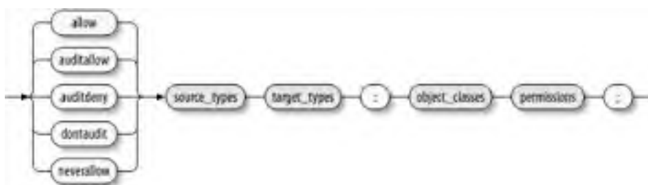
Figure 7-4. TE access vector rule declaration (te_avtab_def)
