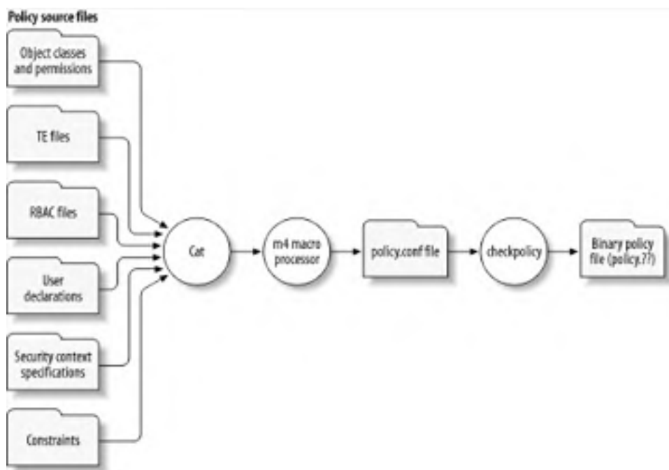
Figure 5-3. Transforming an SELinux policy, including M4 macro expansion
