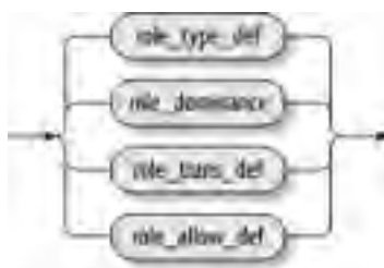
Figure 6-15. RBAC declarations ( rbac_decl )
