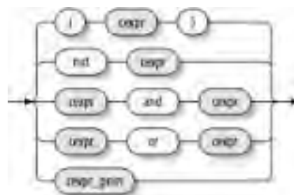
Figure 8-2. Syntax of cexpr
