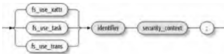
Figure 8-7. Filesystem labeling declaration
