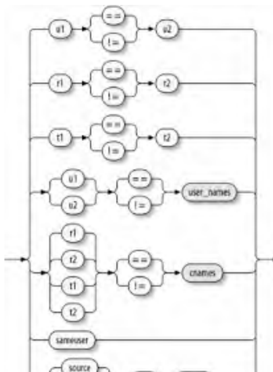
Figure 8-3. Syntax of cexpr_prim
