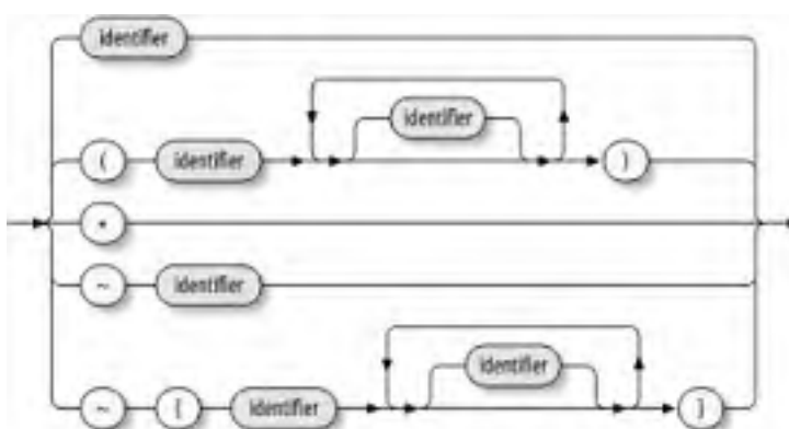
Figure 8-5. Syntax of cnames
