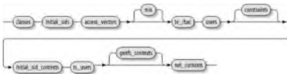
Figure 6-9. The SELinux Policy
