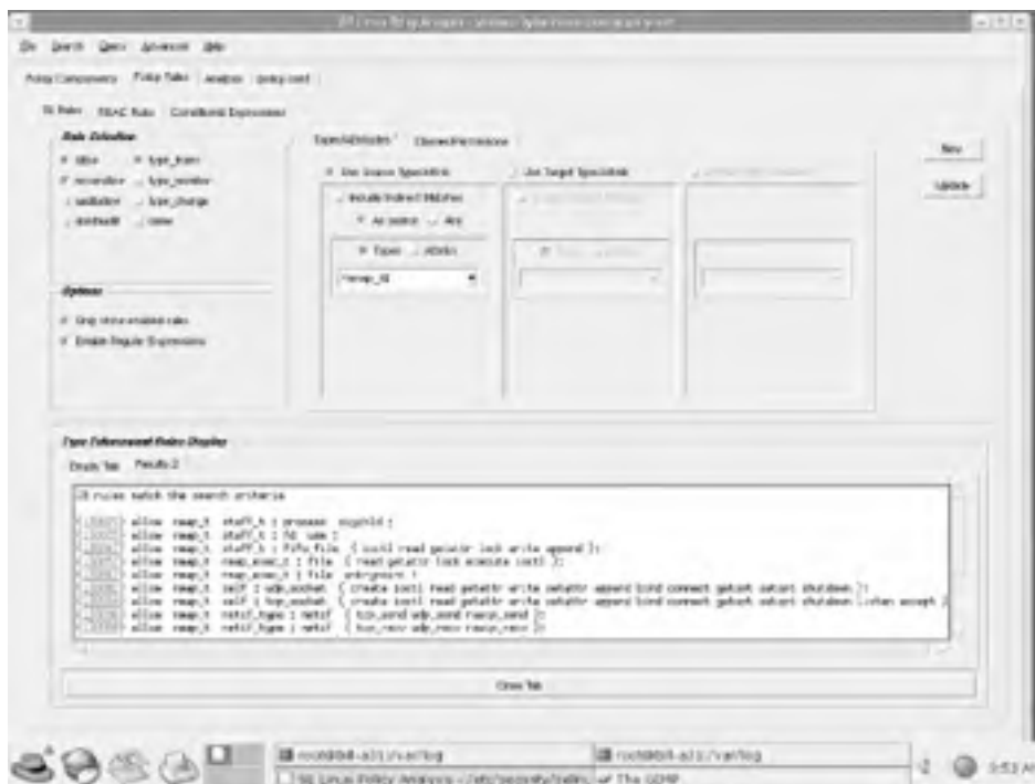
Figure 9-7. Apol's Policy Rules tab
