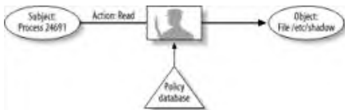
Figure 2-2. A typical SELinux decision
