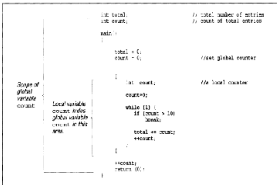
Figure 9-2 Hidden variables
