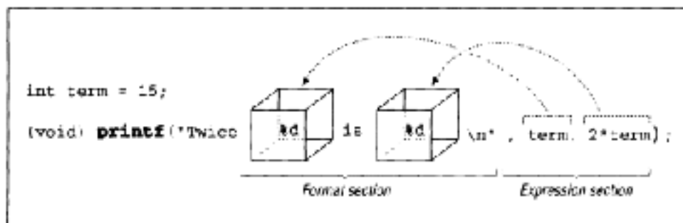
Figure 16-1. printf structure
