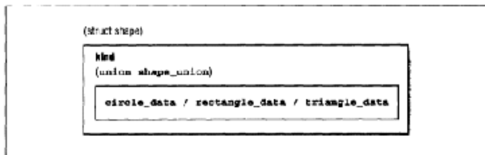
Figure 12-2 "shape" layout
