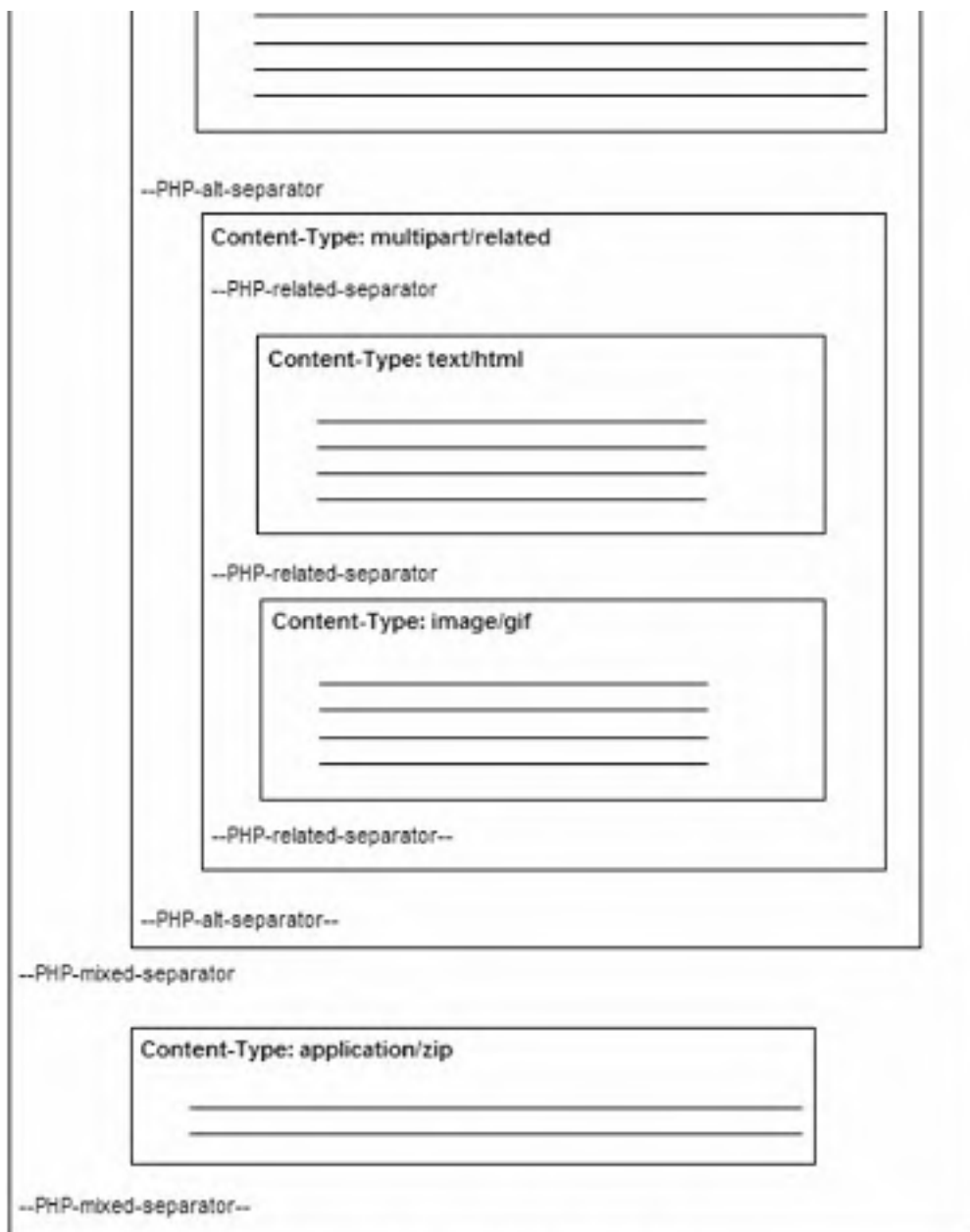
Figure 16.1c: HTML Mail Layout with attachment and embedded image.
