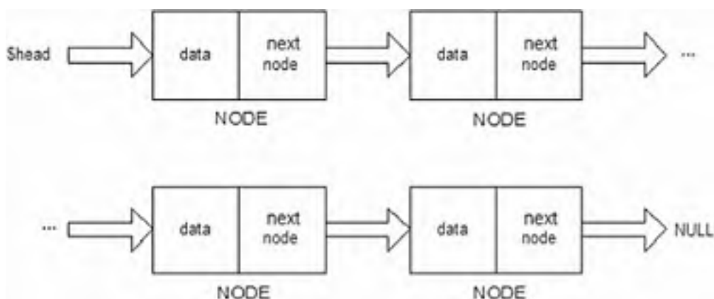
Listing 7.10.1. Structure of a linked list.
