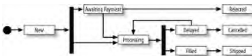
Figure 9-1. Order processing state transitions
