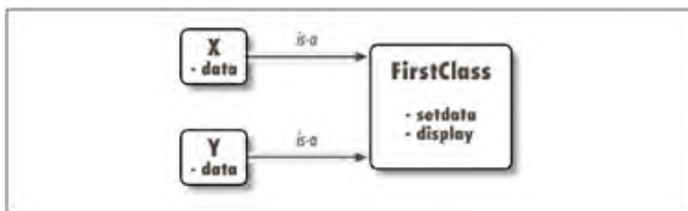
Figure 6.1. Classes and instances are linked namespace objects
