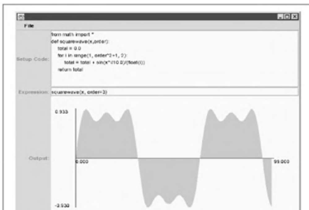
Figure 10.6. Output of grapher.py
