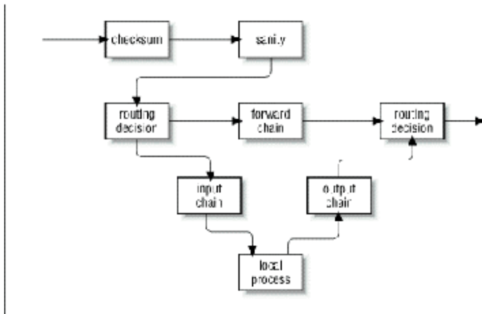
Figure 9.9: Datagram processing chain in netfilter
