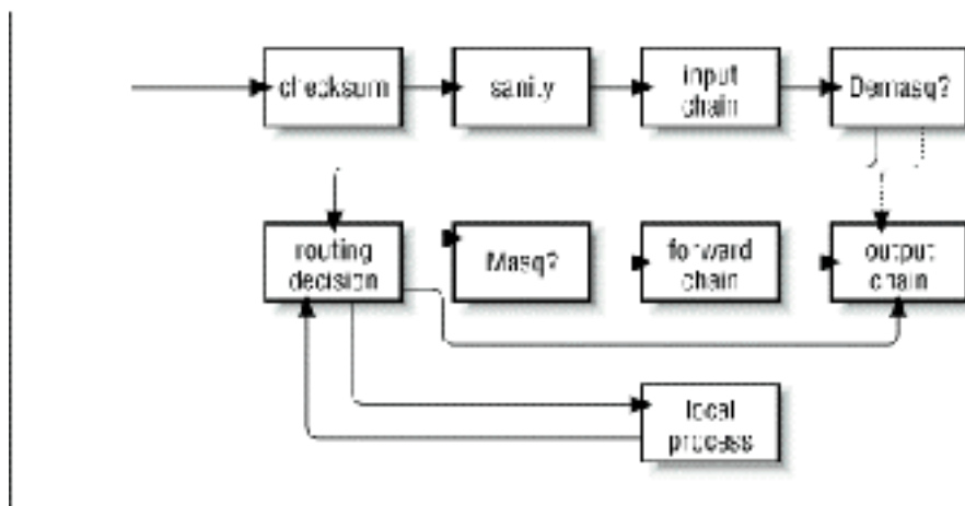
Figure 9.8: Datagram processing chain in IP chains
