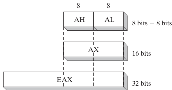
FIGURE 2-6 General-Purpose Registers.
