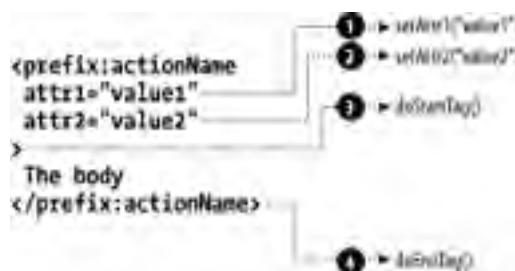
Figure 21-4. Tag interface methods and property setter methods
