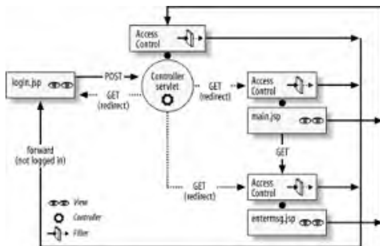
Figure 19-2. Project Billboard application combining servlet and JSP components
