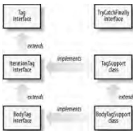
Figure 21-3. The primary classic tag handler interfaces and support classes
