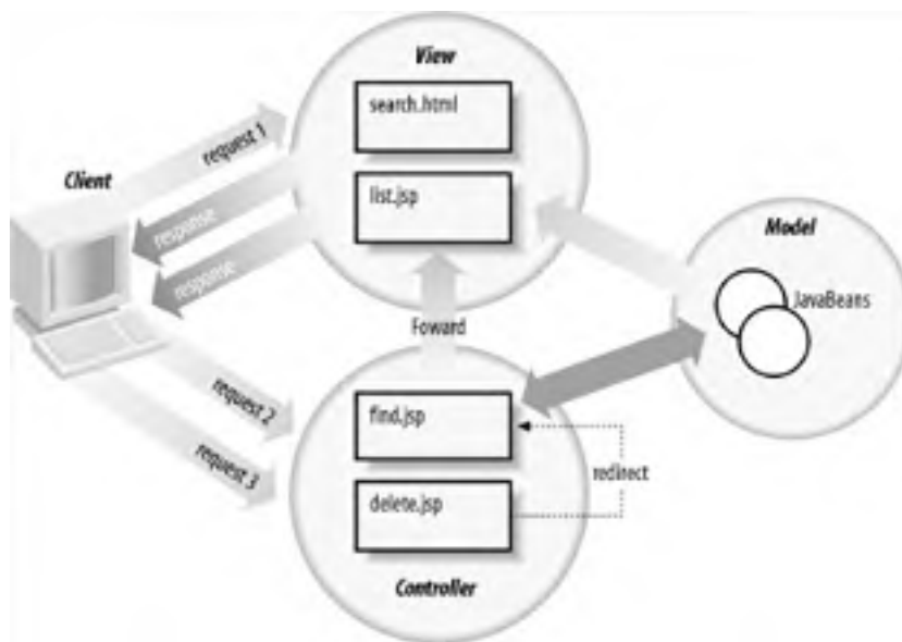
Figure 18-2. MVC roles in a pure JSP scenario
