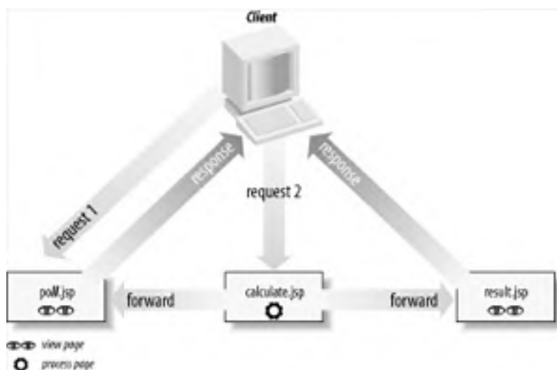
Figure 14-1. Localized poll application pages
