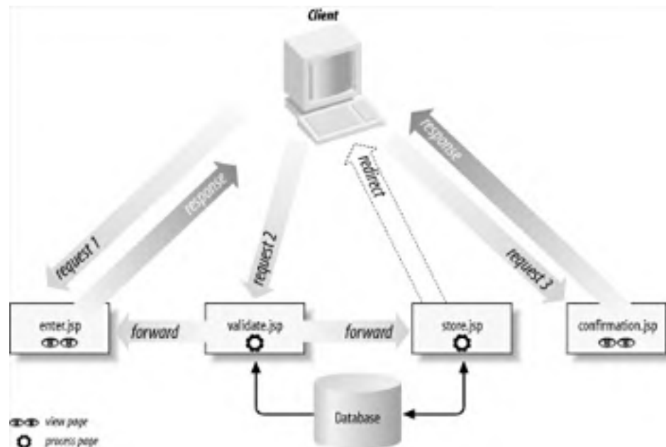
Figure 12-1. Employee registration pages
