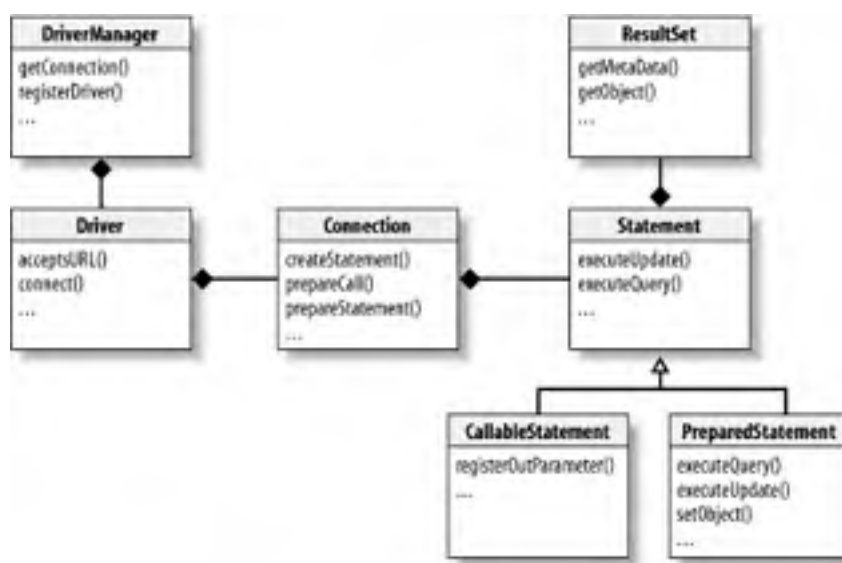
Figure 24-1. Main JDBC interfaces and classes
