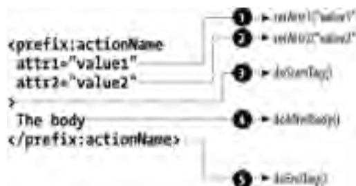
Figure 21-5. IterationTag interface methods
