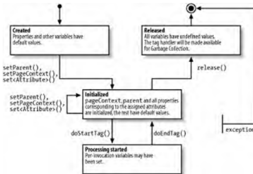
Figure 21-7. Lifecycle for a tag handler implementing the Tag interface
