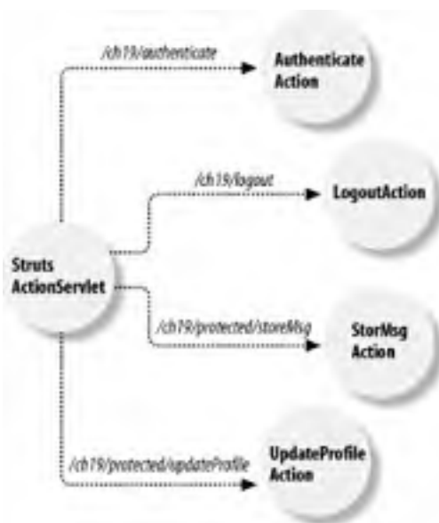
Figure 19-3. Controller split over dispatcher servlet and action classes
