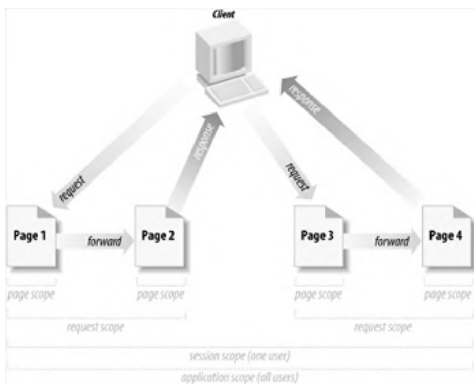
Figure 10-2. Lifetime of objects in different scopes
