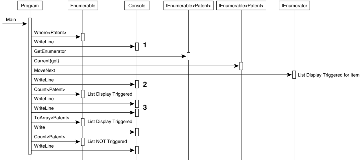
FIGURE 14.2: IEnumerator<T> and IEnumerable Interfaces
