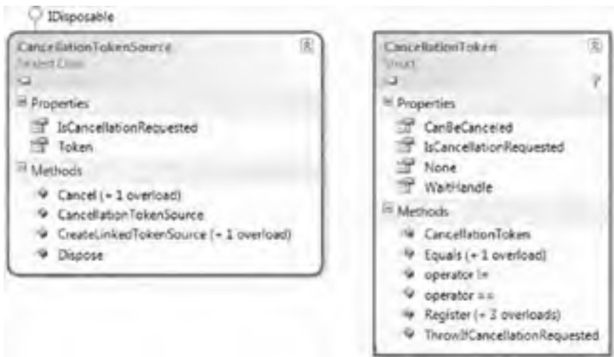
FIGURE 18.2: CancellationTokenSource and CancellationToken Class Diagrams
