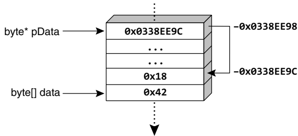
FIGURE 20.1: Pointers Contain the Address of the Data
