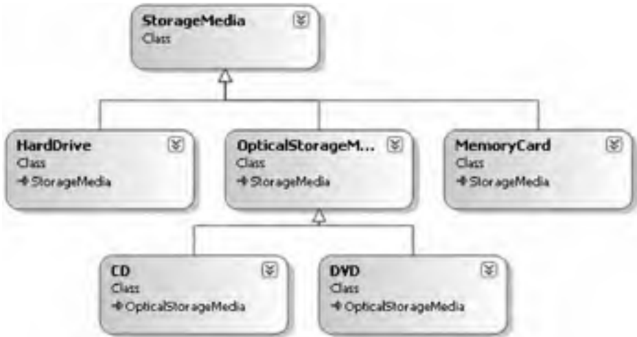
FIGURE 5.1: Class Hierarchy
