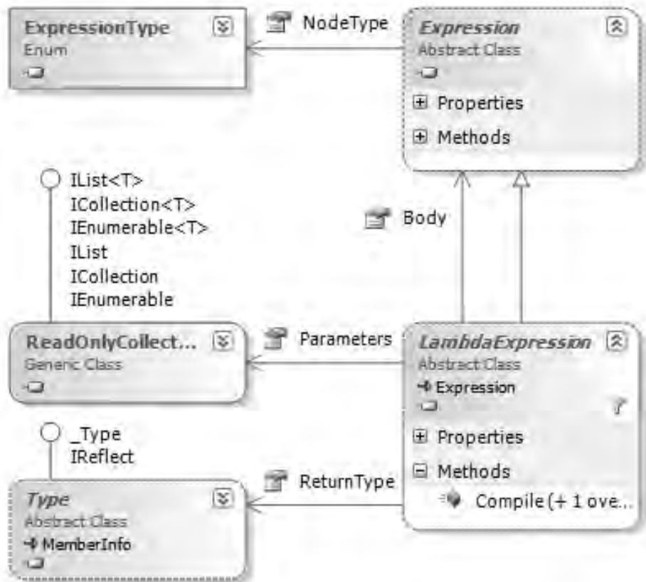
FIGURE 12.3: Object Graph of a Lambda Expression
