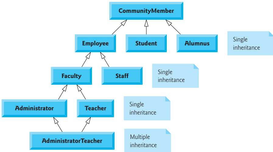
Fig. 20.2 | Inheritance hierarchy for university CommunityMembers .
