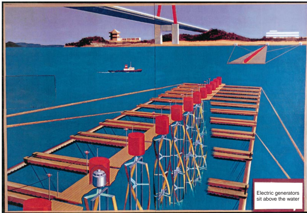
Figure 3 Artist rendition of the floating tidal power plant with vertical triple-helix turbines for Uldolmok Strait (Korean Peninsula).
