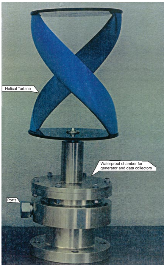
Figure 2 Double-helix turbine with electric generator for underwater installation.
