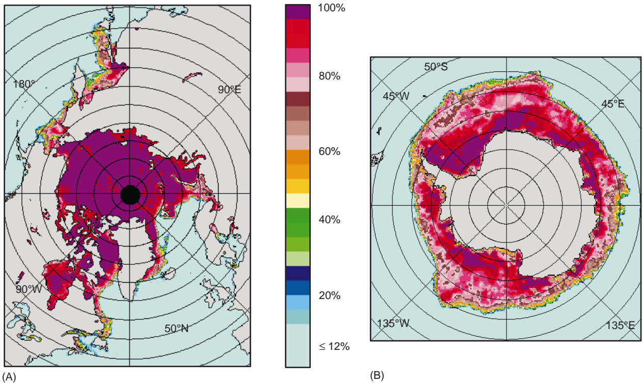
Figure 2 North and south polar sea ice concentration images for (A) 15 March 1998 and (B) 15 September 1998, respectively. The ice concentrations are derived from the data of the DMSP SSMI, including the 19.4 V data depicted in Figure 1 .
