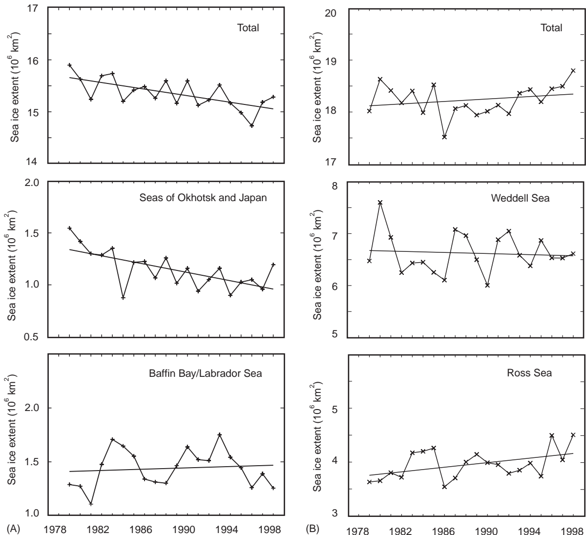
Figure 3 (A) Time series of monthly average 1979–1998 March sea ice extents for the Northern Hemisphere and two regions within the Northern Hemisphere. (B) Time series of monthly average 1979–1998 September sea ice extents for the Southern Hemisphere and two regions within the Southern Hemisphere. All ice extents are derived from the Nimbus 7 SMMR and DMSP SSM/I data. The trend lines have slopes of -31700\text{km}^2\text{y}^{-1} ( -2.0\% per decade) for the Northern Hemisphere total; -20000\text{km}^2\text{y}^{-1} ( -14.9\% per decade) for the Seas of Okhotsk and Japan; 3100\text{km}^2\text{y}^{-1} ( 2.2\% per decade) for Baffin Bay/Labrador Sea; 11900\text{km}^2\text{y}^{-1} ( 0.7\% per decade) for the Southern Hemisphere total; -5300\text{km}^2\text{y}^{-1} ( -0.8\% per decade) for the Weddell Sea; and 21300\text{km}^2\text{y}^{-1} ( 5.7\% per decade) for the Ross Sea.
