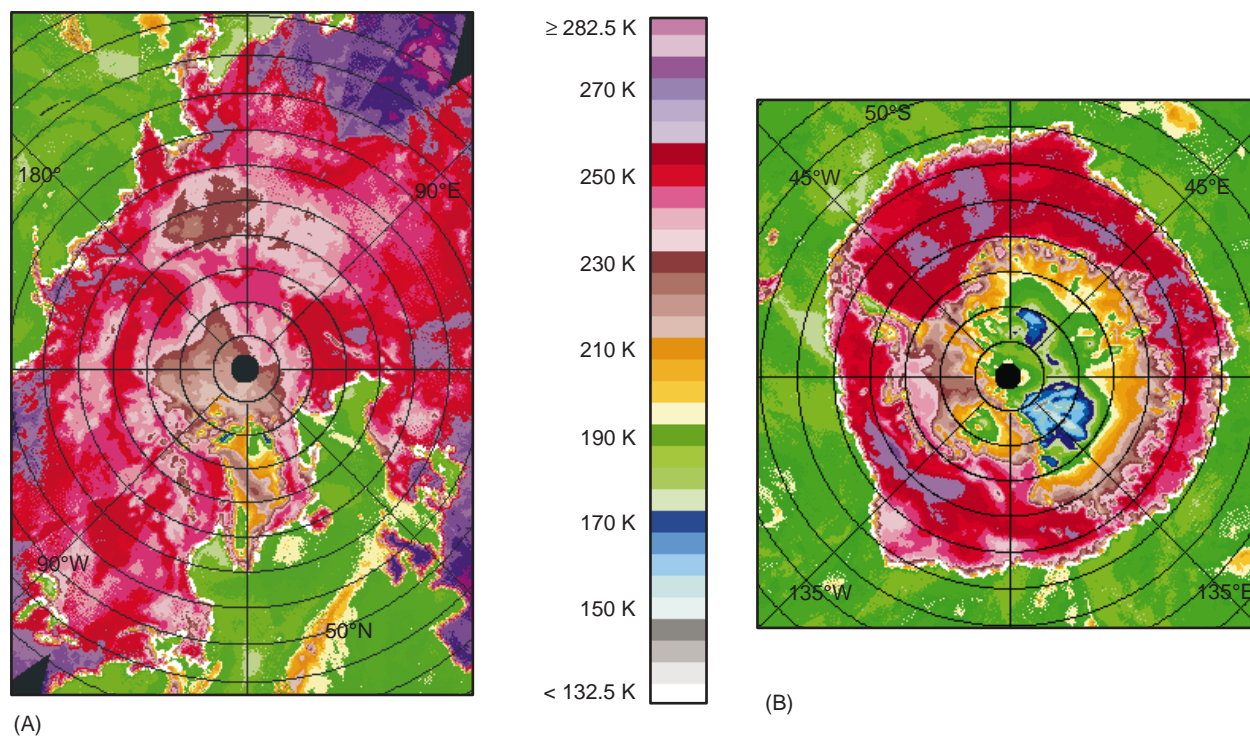
Figure 1 Late winter brightness temperature images of 19.4GHz vertically polarized (19.4V) data from the Defense Meteorological Satellite Program's Special Sensor Microwave Imager (SSMI) for (A) the north polar region on 15 March 1998, and (B) the south polar region on 15 September 1998, showing near-maximum sea ice coverage in each hemisphere. The dashed white curve has been added to indicate the location of the sea ice edge. Black signifies areas of no data; the absence of data poleward of 87.6° latitude results from the satellite's near-polar orbit and is consistent throughout the data set.
