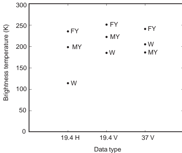
Figure 4 Brightness temperatures of first-year ice (FY), multi-year ice (MY), and liquid water (W) at three channels of SSMI data from the DMSP F13 satellite. These are the values used as tie points for the Arctic calculations in the NASA Team algorithm described in the text. (Data from Cavalieri et al. (1999).)
