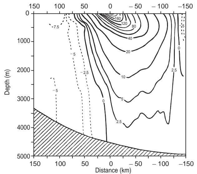
Figure 3 Downstream speed (positive) (cm s -1 ) of the Gulf Stream at 68°W measured with current meters. (Adapted from Johns et al. (1995).)
