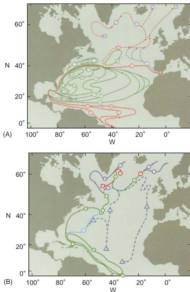
Figure 2 (A) Schematic showing the transport of the upper layer (temperatures greater than around 7^\circ\text{C} ) North Atlantic circulation (in Sverdrups, 1\text{ Sv} = 10^6\text{ m}^3\text{ s}^{-1} ). Transports in squares denote sinking and those in hexagons denote entrainment. Red lines show the upper layer flow of the meridional overturning circulation. The blue boxes attached to dashed lines indicate that significant cooling may occur. Solid green lines characterize the subtropical gyre and recirculations as well as the Newfoundland Basin Eddy. Dashed blue lines indicate the addition of Mediterranean Water to the North Atlantic. (B) Schematic circulation showing the transport in Sverdrups of North Atlantic Deep Water (NADW). Green lines indicate transports of NADW, dark blue lines and symbols denote bottom water, and red lines upper layer replacement flows. Light blue line indicates a separate mid-latitude path for lower NADW. The square represents sinking, hexagons entrainment of upper layer water, and triangles with dashed lines water mass modification of Antarctic Bottom Water. (Reproduced from Schmitz (1996).)
