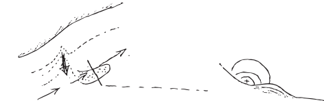
Figure 3 Contourite drift models. (Modified from Faugeres et al. , 1999.)
