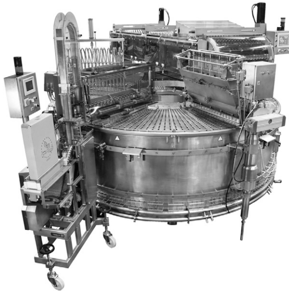
Figure 16.7 Novelty ice-cream stick product machine (Gram)
