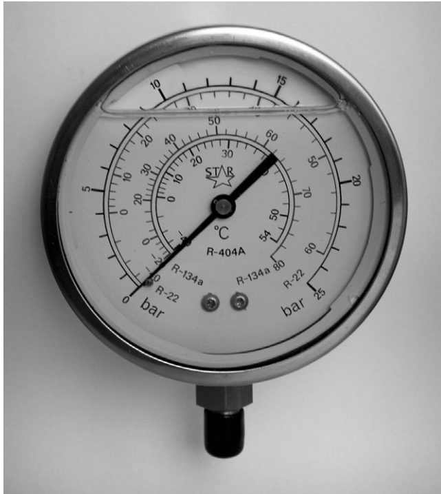
Figure 9.5 Refrigeration pressure gauge (Star Instruments)
