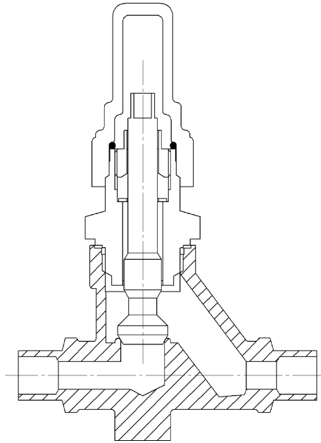
Figure 9.8 Seal cap shut-off valve (Henry)
