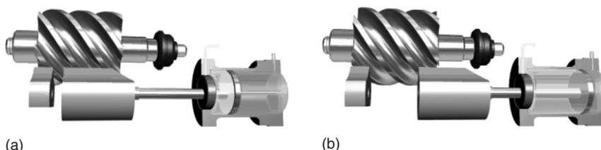
Figure 4.22 Capacity reduction slide for twin screw compressor (a) just starting to open, (b) at minimum load. The valve is moved by an oil pressure acting on a piston, shown on the right (Howden)
