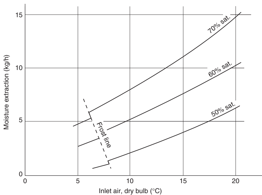
Figure 26.2 Performance of dehumidifier
