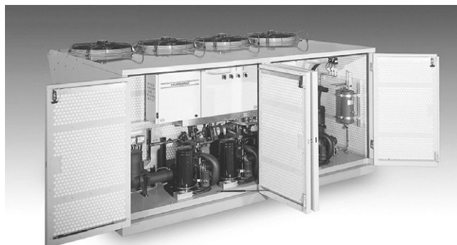
Figure 13.6 Scroll compressor pack within rooftop condenser (Hubbard)
