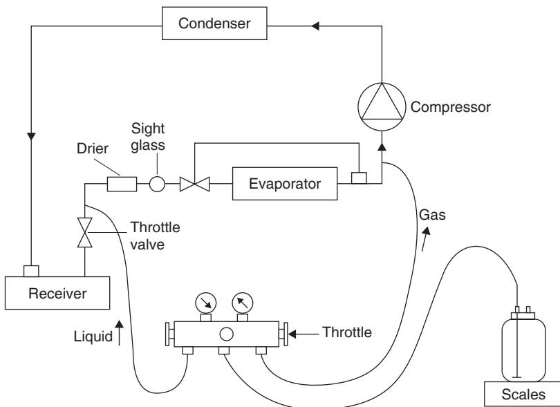
Figure 11.3 Charging connection
