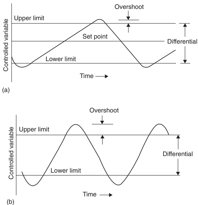
Figure 28.2 Limits of controlled variable with two-position control. (a) Capacity closely matched to load. (b) Capacity much greater than load
