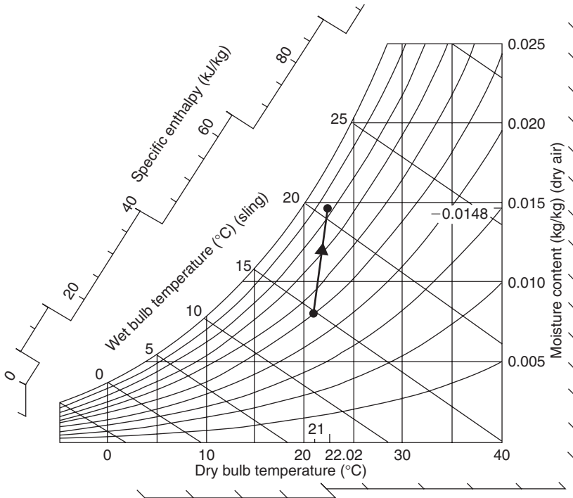
Figure 21.6 Addition of steam to air
