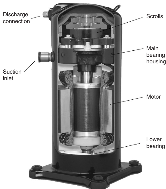
Figure 4.25 Cut away view of scroll compressor (Emerson Climate Technologies)
