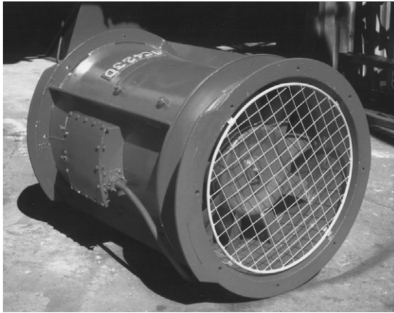
Figure 24.8 Vane-axial fan (CIBSE/FMA)
