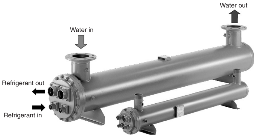
Figure 7.5 Onda shell and tube direct expansion evaporators (Titan)
