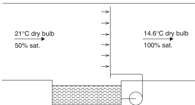
Figure 21.4 Adiabatic saturation to ultimate condition
