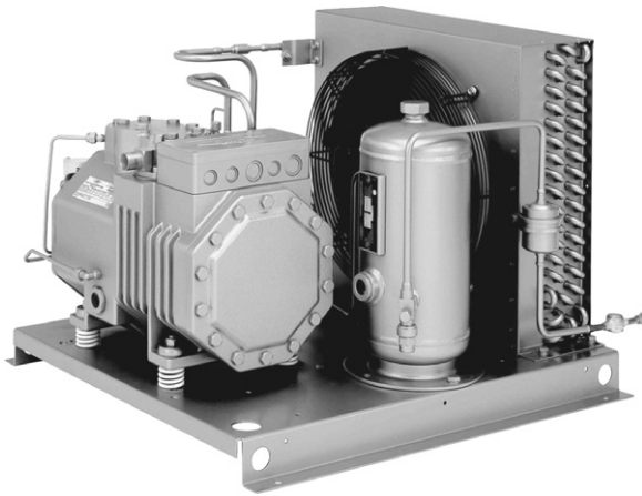
Figure 13.1 Air-cooled condensing unit, 2-cyl semi-hermetic compressor, suitable for several refrigerants (Bitzer)
