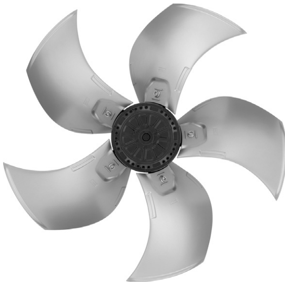
Figure 24.6 Low-pressure, high-volume ducted propeller fan (CIBSE/FMA)
