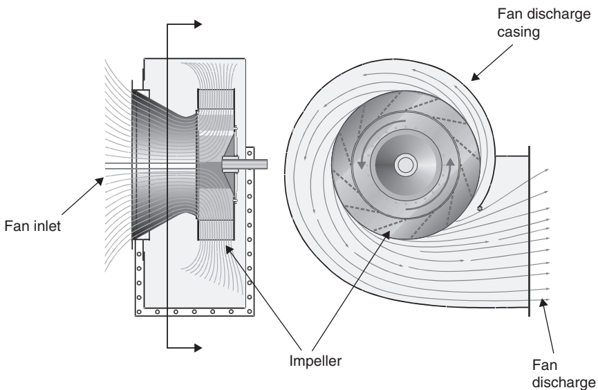
Figure 24.9 Cased centrifugal fan (CIBSE/FMA/Howden)
