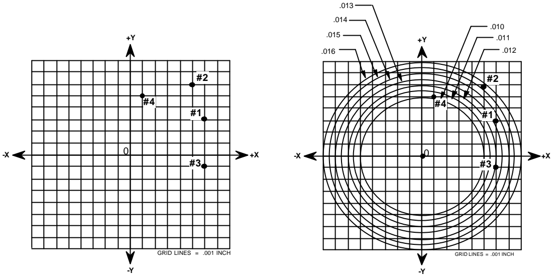
Figure 18-9 Paper gage verification of hole pattern location
