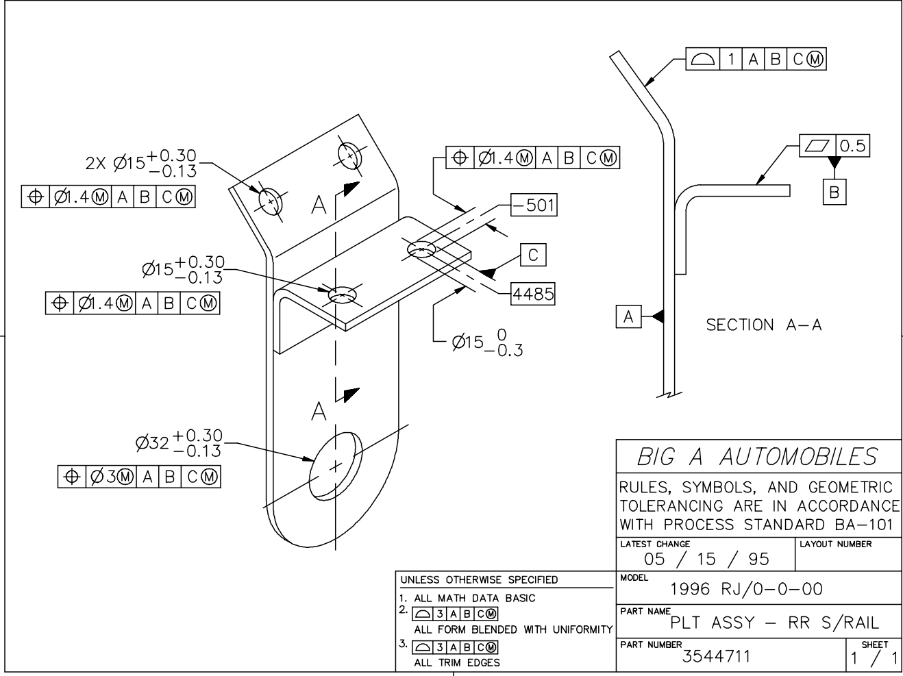
Figure 4-5 Stamped sheet metal part drawing
