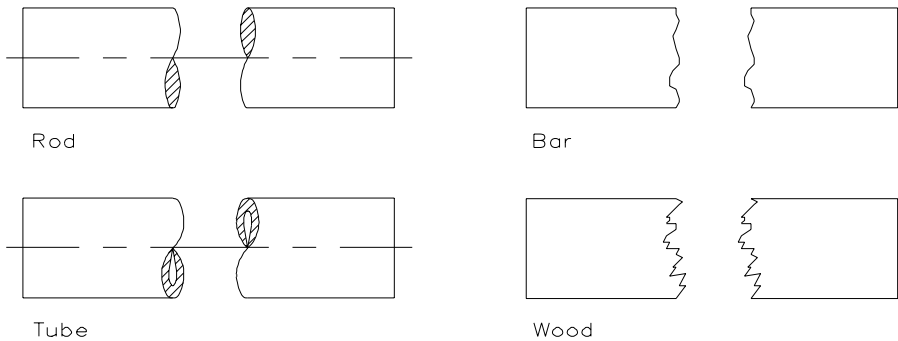
Figure 4-18 Conventional breaks
