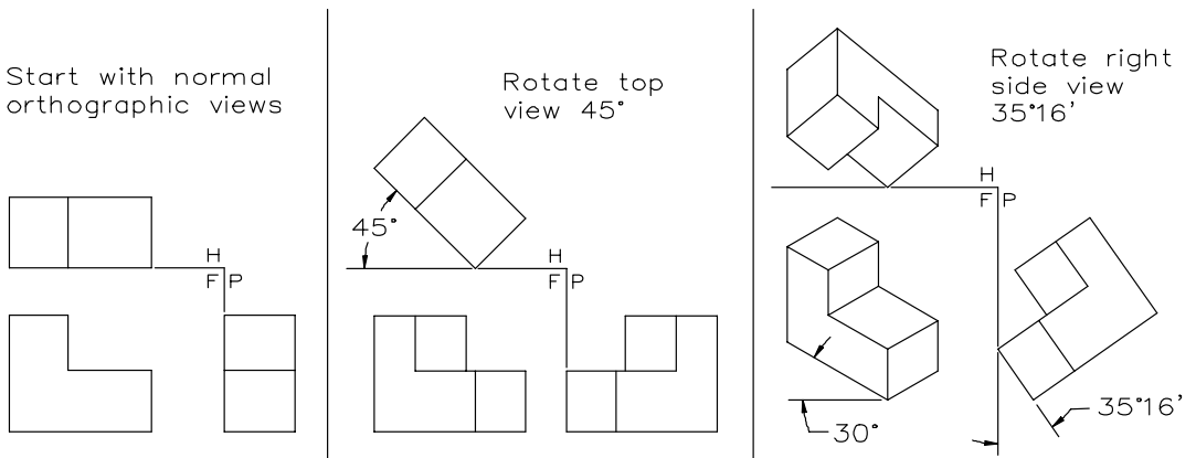
Figure 4-21 Isometric projection
