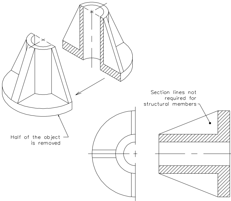
Figure 4-13 Full section
