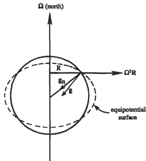
Figure 4.15 Effective gravity \mathbf{g} and equipotential surface.
