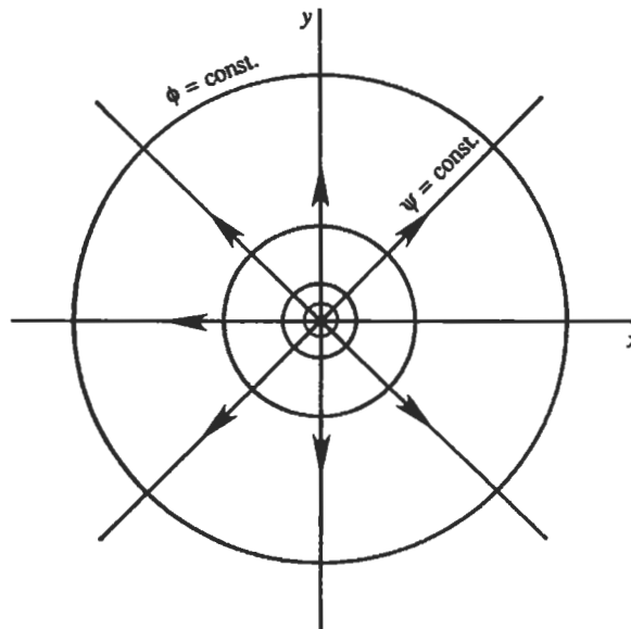
Figure 6.6 Plane source.
