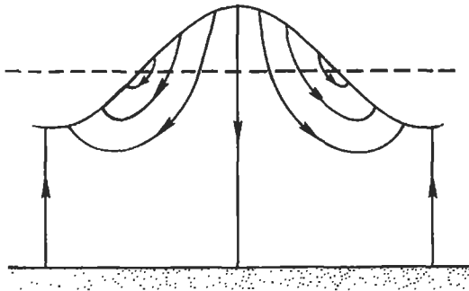
Figure 7.14 Instantaneous streamline pattern in a standing surface gravity wave. If this is mode n = 0 , then two successive vertical streamlines are a distance L apart. If this is mode n = 1 , then the first and third vertical streamlines are a distance L apart.
