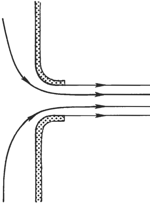
Figure 4.21 Flow through a rounded orifice.
