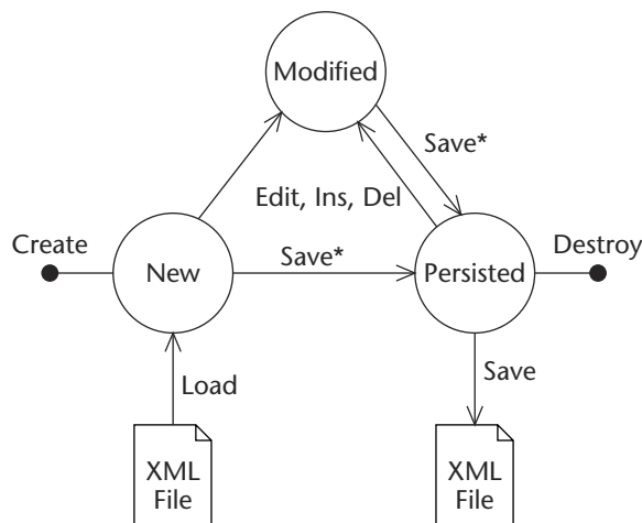
Figure 9.1 DOM lifecycle.
