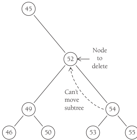
FIGURE 12.6. Deleting A Node With Two Children.
