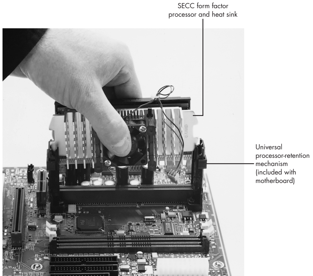
Figure 24.4 Installing a slot-based (Single Edge Contact Cartridge or SECC) processor. Motherboard and processor courtesy of Intel Corporation.
