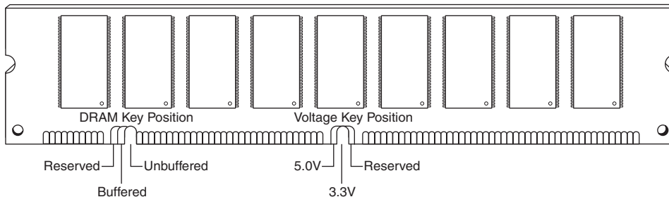
Figure 6.16 168-pin DRAM DIMM notch key definitions.
