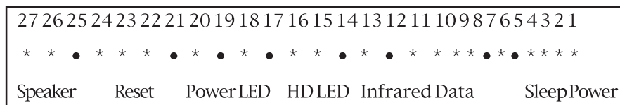
Figure 4.39 Typical ATX motherboard front panel connectors (Intel motherboard shown).
