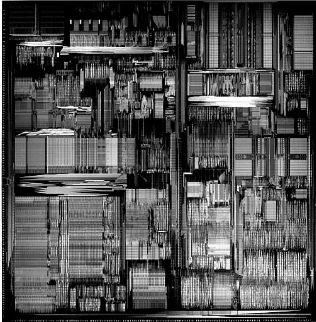
Figure 3.36 Pentium Pro processor die. Photograph used by permission of Intel Corporation.
