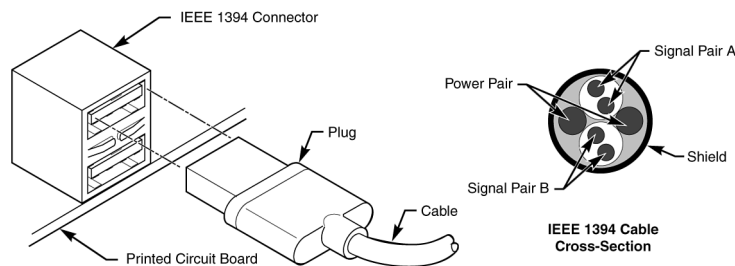
Figure 16.8 IEEE-1394 cable, socket, and connector plug.
