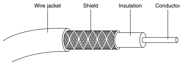
Figure 19.8 Coaxial cable.
