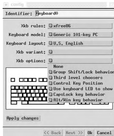
Figure 6-11: xf86cfg keyboard menu
