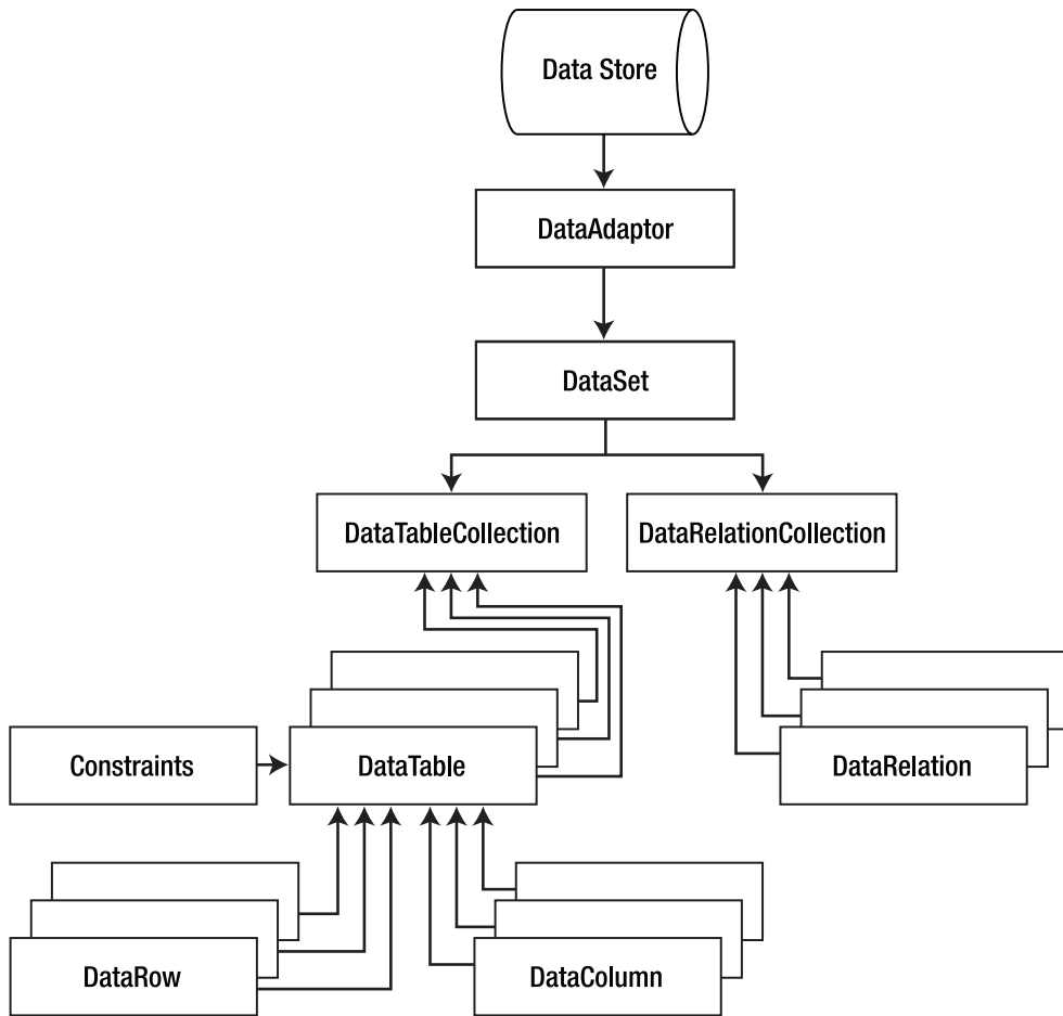
Figure 12-15. The disconnected ADO.NET class interaction
