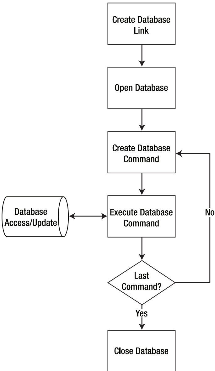
Figure 12-8. Nontransactional database access
