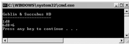
Figure 13-11. Output for the XPath expression //Monster[Name='Goblin' or Name='Succubus']/HitDice
