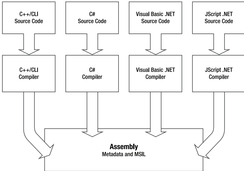
Figure 1-6. Many compilers, one output
