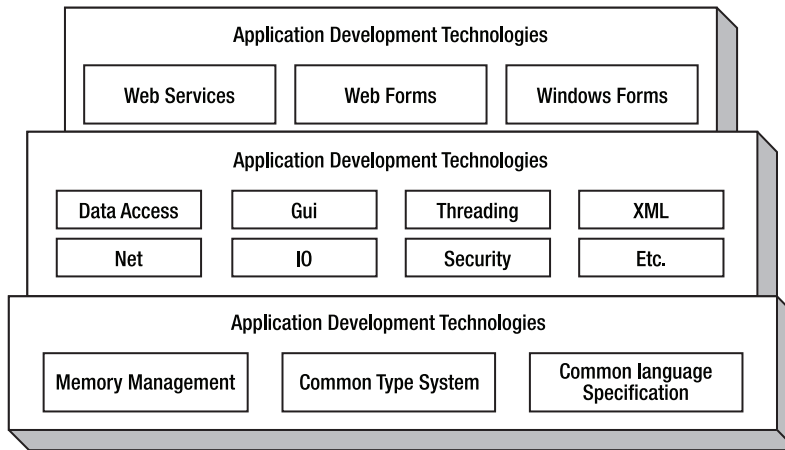
Figure 1-1. The .NET Framework hierarchy
