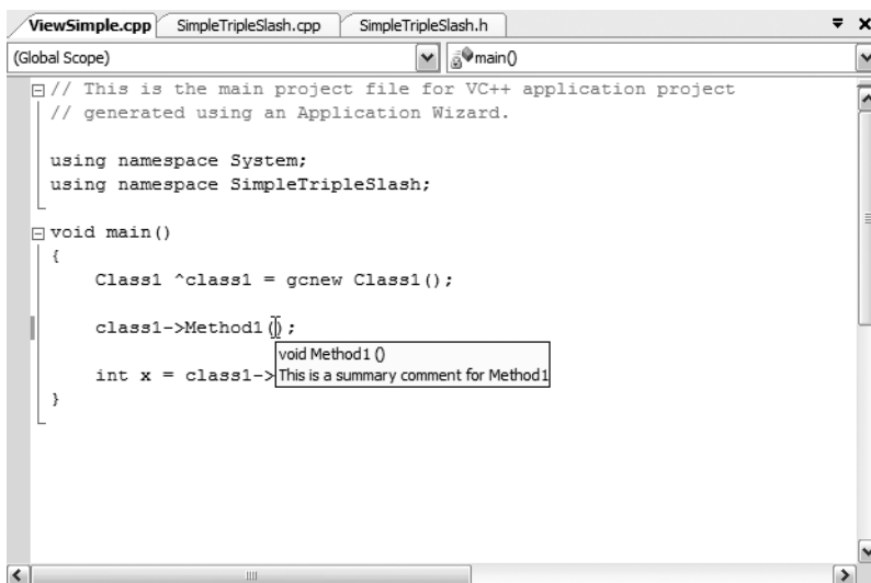
Figure 6-3. Automatically generated IntelliSense from triple slash comments
