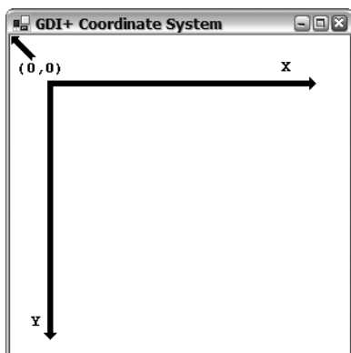
Figure 11-5. The default GDI coordinate system
