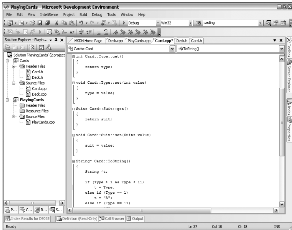
Figure 1-4. Visual Studio .NET's IntelliSense using metadata
