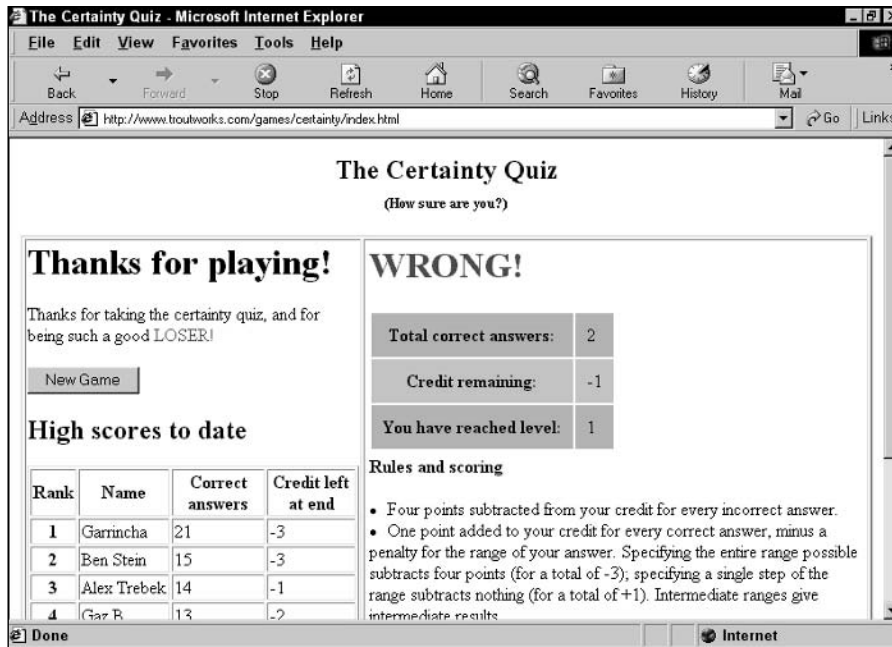
Figure 46-3: Game over
