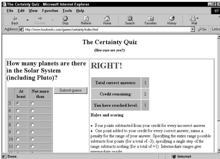
Figure 46-2: Continuing play
