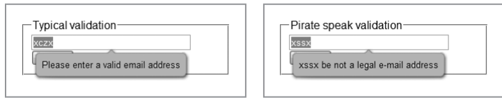
FIGURE 3.13 Opera rendering the default validation message for email (left) and our custom “speak like an angry pirate day” validation (right).
