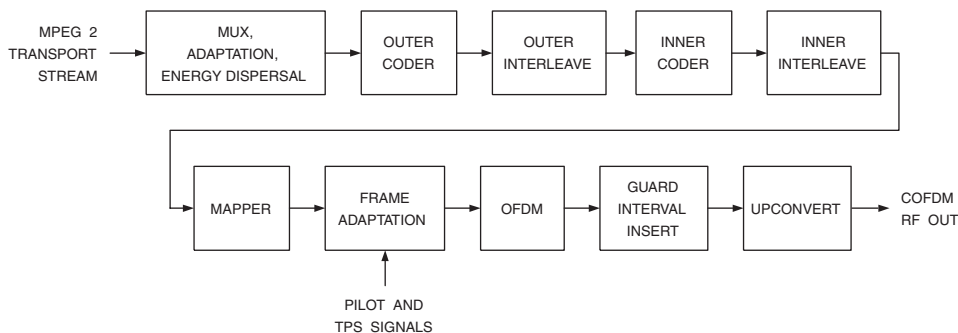
Figure 17.2. Simplified Block Diagram of a COFDM Modulator.
