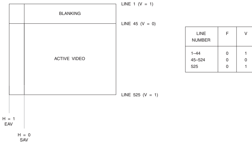
Figure 4.13. 480p Digital Vertical Timing (480 Active Lines). V changes state at the EAV sequence at the beginning of the digital line. Note that the digital line number changes state prior to start of horizontal sync, as shown in Figures 4.9 through 4.12.
