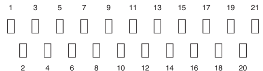
Figure 5.2. SCART Connector.
