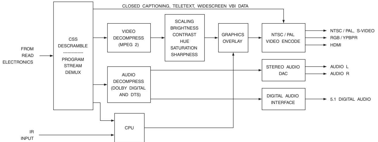
Figure 2.4. Simplified Block Diagram of a Basic DVD Player.
