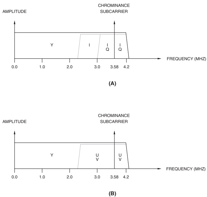
Figure 8.3. Video Bandwidths of Baseband (M) NTSC Video. (a) Using 1.3-MHz I and 0.6-MHz Q signals. (b) Using 1.3-MHz U and V signals.
