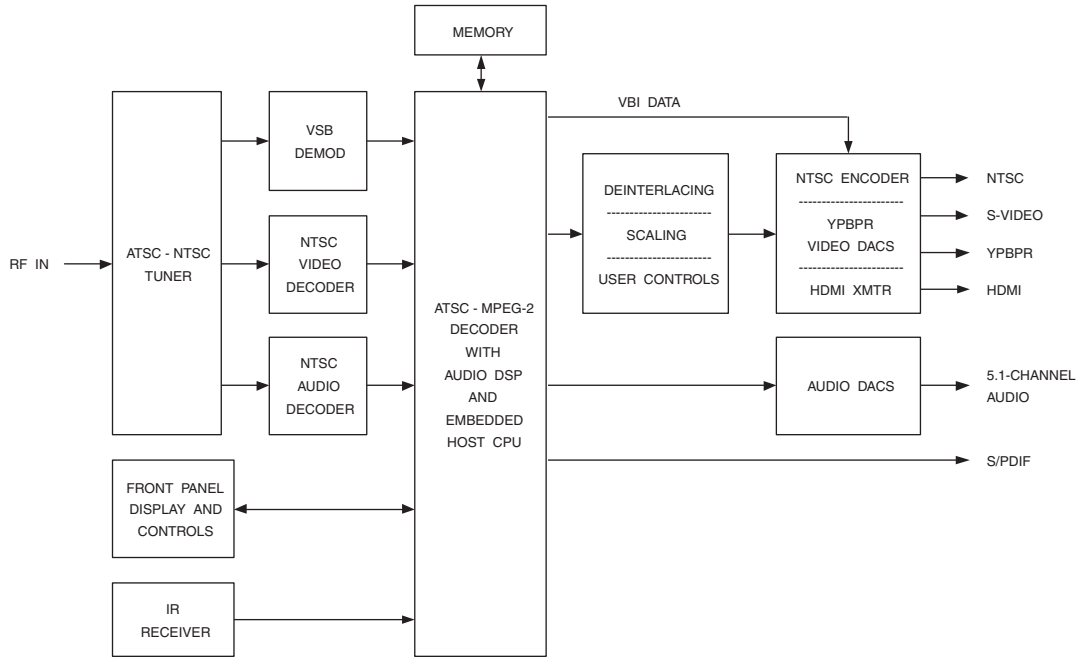
Figure 15.5. Typical ATSC Receiver Set-top Box Block Diagram.
