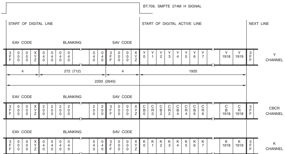
Figure 6.17. BT.1120 and SMPTE 274M Parallel Interface Data For One Scan Line. 1080i; 29.97-, 30-, 59.94-, and 60-Hz systems; 4:2:2:4 YCbCrK; 1920 active samples per line; 74.176, 74.25, 148.35, or 148.5 MHz clock; 10-bit system. The values for 25- and 50-Hz systems are shown in parentheses.
