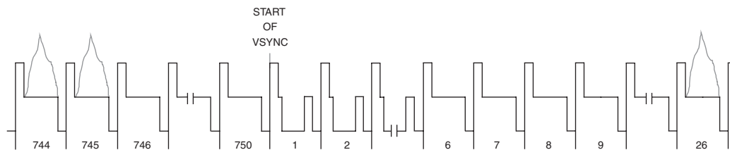
Figure 4.26. 720p Vertical Interval Timing.
