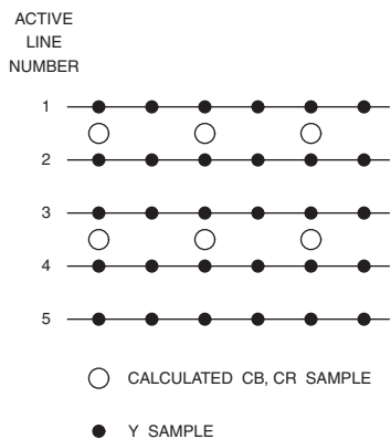
Figure 3.8. 4:2:0 Sampling for MPEG-2, MPEG-4 Part 2 and H.264. The sampling positions on the active scan lines of a progressive or noninterlaced picture.
