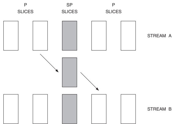
Figure 14.6. Using SP Slices to Switch to Another Stream.
