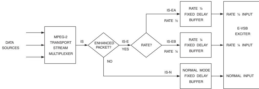
Figure 15.3. ATSC E-VSB Head-end Model.
