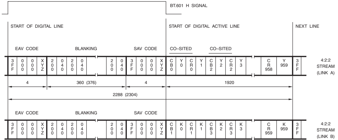
Figure 6.14. BT.1303 Parallel Interface Data For One Scan Line. 480i; 4:4:4:4 YCbCrK; 960 active samples per line; 36 MHz clock; 10-bit system. The values for 576i systems are shown in parentheses.
