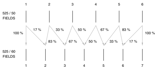
Figure 7.40. 50-Hz to 60-Hz Conversion Using Temporal Interpolation with No Motion Compensation.
