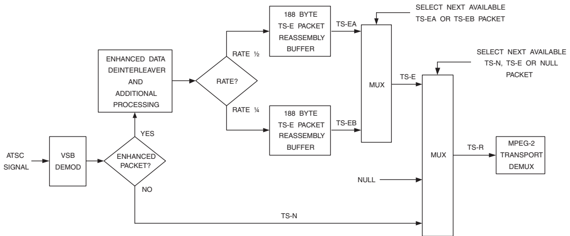
Figure 15.4. ATSC E-VSB Receiver Model.
