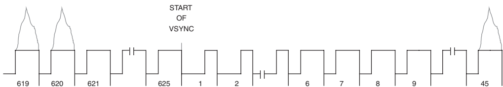
Figure 4.15. 576p Vertical Interval Timing.
