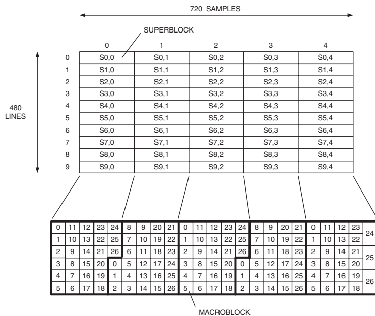
Figure 11.7. Relationship Between Super Blocks and Macroblocks (4:1:1 YCbCr, 720 × 480i).
