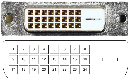
Figure 6.46. DVI-D Connector.
