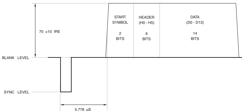
Figure 5.8. EIA-805, IEC 61880–2 and EIA-J CPR–1204–1 480p Line 41 CGMS Timing.
