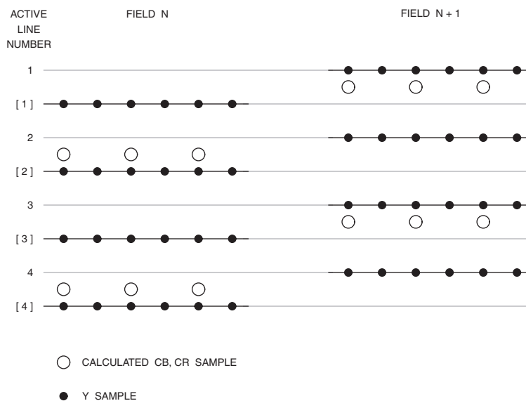
Figure 3.10. 4:2:0 Sampling for MPEG-2, MPEG-4 Part 2 and H.264. The sampling positions on the active scan lines of an interlaced picture (top_field_first = 0).
