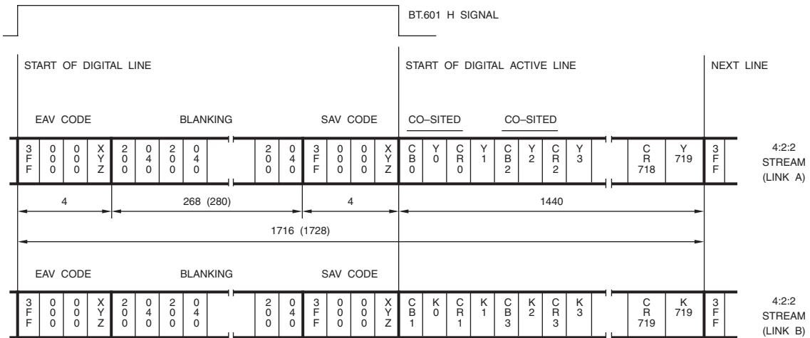
Figure 6.13. BT.799 and SMPTE RP-175 Parallel Interface Data For One Scan Line. 480i; 4:4:4:4 YCbCrK; 720 active samples per line; 27 MHz clock; 10-bit system. The values for 576i systems are shown in parentheses.
