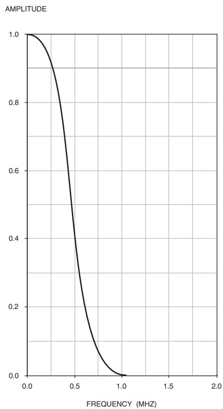
Figure 9.27. Typical 0.6-MHz Lowpass Digital Filter Characteristics.
