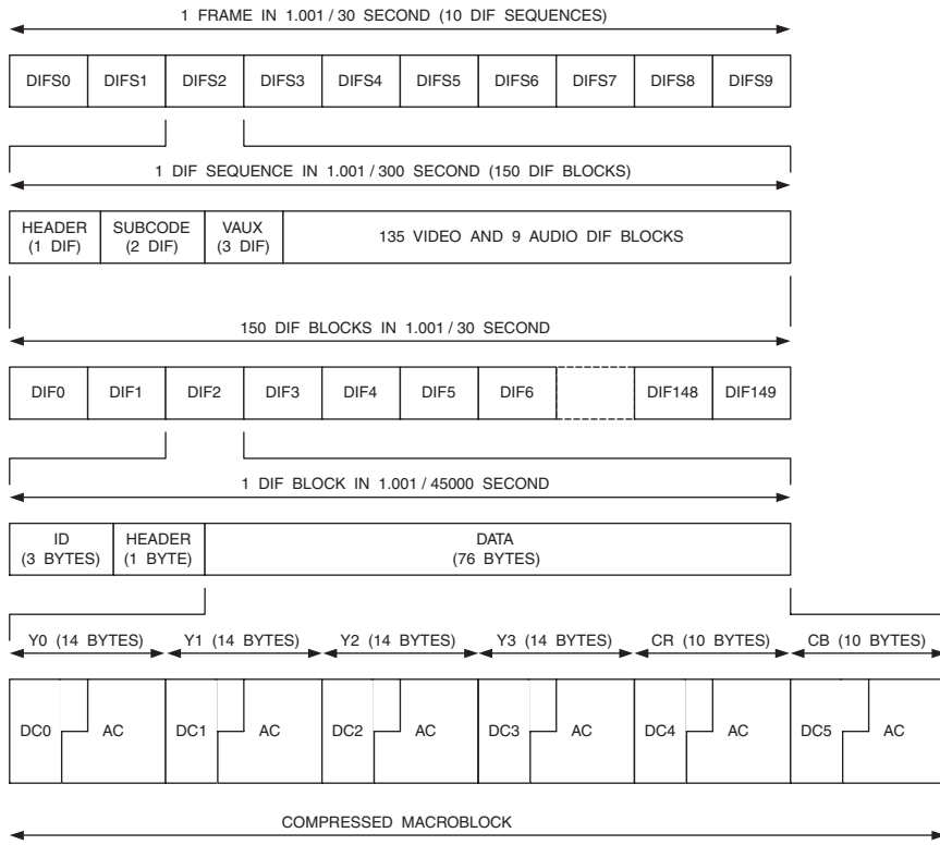
Figure 11.14. Packet Formatting for 25 Mbps 4:1:1 YCbCr 720 × 480i Systems.
