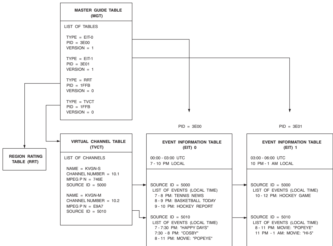
Figure 15.1. ATSC PSIP Table Relationships.
