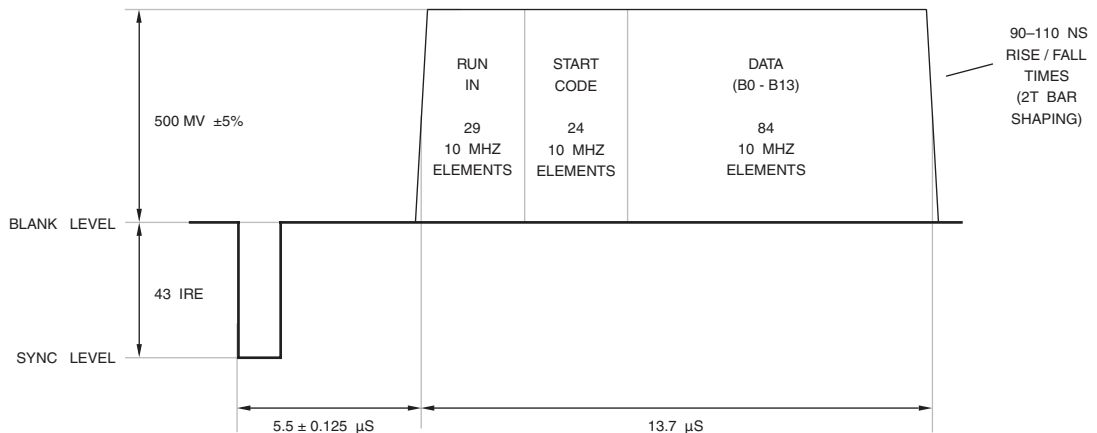
Figure 5.9. IEC 62375 576p Line 43 CGMS Timing.
