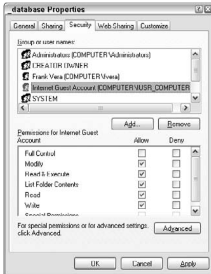
Figure 13-3: The _database Properties dialog box.
