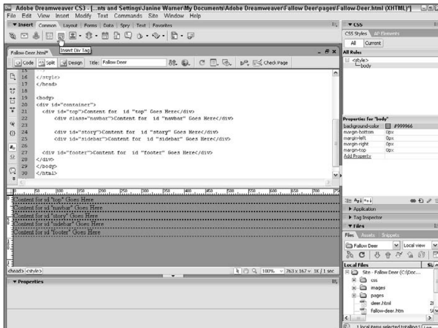
Figure 6-7: As you insert <div> tags, using split view can help you see the order in which the tags are being added to the page.
