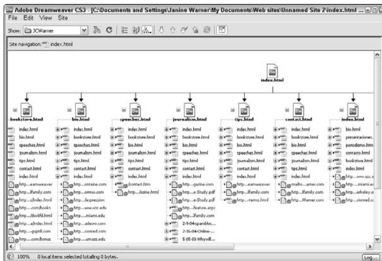
Figure 4-18: The site map provides a visual reference to the structure, hierarchy, and links in a Web site.
