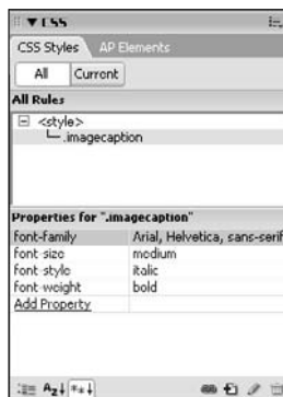
Figure 5-3: The CSS Styles panel showing a class style named .imagecaption .
