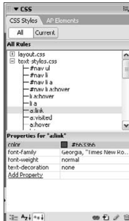
Figure 5-17: External style sheets linked to the current document appear in the CSS Styles panel.
