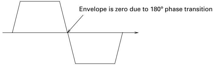
Figure 8.13 The envelope of a PSK signal passes through zero during a 180° phase transition, and gets distorted over a nonlinear channel.
