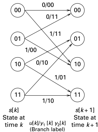
Figure 7.2 A section of the trellis representation of the code, showing state transitions between time k and k + 1 . Each trellis branch is labeled with the input and outputs associated with it, u[k]/y_1[k]y_2[k] .
