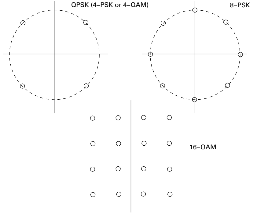
Figure 3.10 For linear modulation with no intersymbol interference, the complex symbols themselves provide a two-dimensional signal space representation. Three different constellations are shown here.
