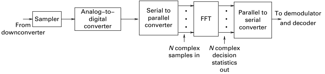
Figure 8.5 DSP-centric implementation of an OFDM receiver. Carrier and timing synchronization blocks are not shown.
