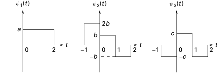
Figure 3.9 An orthonormal basis for the signal set in Figure 3.7, obtained by applying the Gram–Schmidt procedure. The unknowns a , b , and c are to be determined in Exercise 3.3.1.
