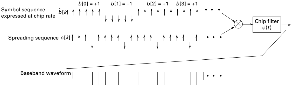
Figure 8.7 Example of DS modulation, with processing gain N = 5 and a short spreading sequence. In this chip rate implementation, the data sequence is converted to the chip rate and is multiplied chip-by-chip with the spreading sequence before modulating the chip waveform. These discrete-time chip rate sequences are indicated by delta functions in the figure. These are then passed through a chip filter (which may itself be implemented in DSP at a multiple of the chip rate, followed by digital-to-analog conversion) to obtain the baseband analog waveform to be upconverted.
