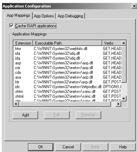
Figure 4-9: File extension mappings in IIS 5.0
