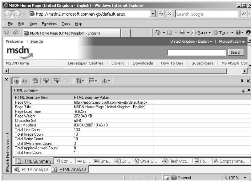
Figure 4-2: IEWatch performing HTTP and HTML analysis from within the browser
