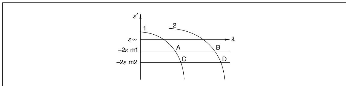
Fig. 9.13: Dispersion diagram showing the conditions of surface plasmon resonance absorption as a function of the wavelength of the incident light. Reproduced from Mulvaney, et al. (Ref. 8). Reproduced by permission of the Royal Society of Chemistry.
