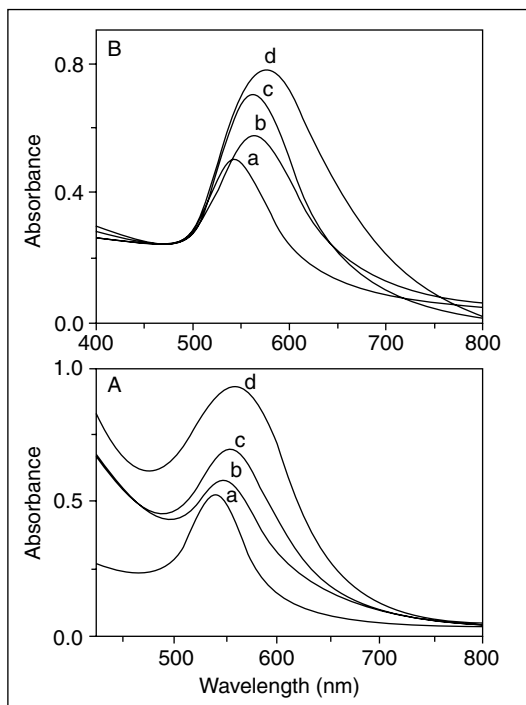
Fig. 9.14: The absorption spectra of Au@SiO 2 colloids as a function of solvent refractive index (top figures) and Ag@TiO 2 (bottom (A)) and Ag@ZrO 2 (bottom (B)) as a function of increasing core dimension, a–d (A) and increasing shell thickness, a–d (B). Reprinted with permission from Liz-Marzan, et al. (Ref. 2) (top) and Tom, et al. (Ref. 6) (bottom). Copyright (1996 and 2003, respectively) American Chemical Society.
