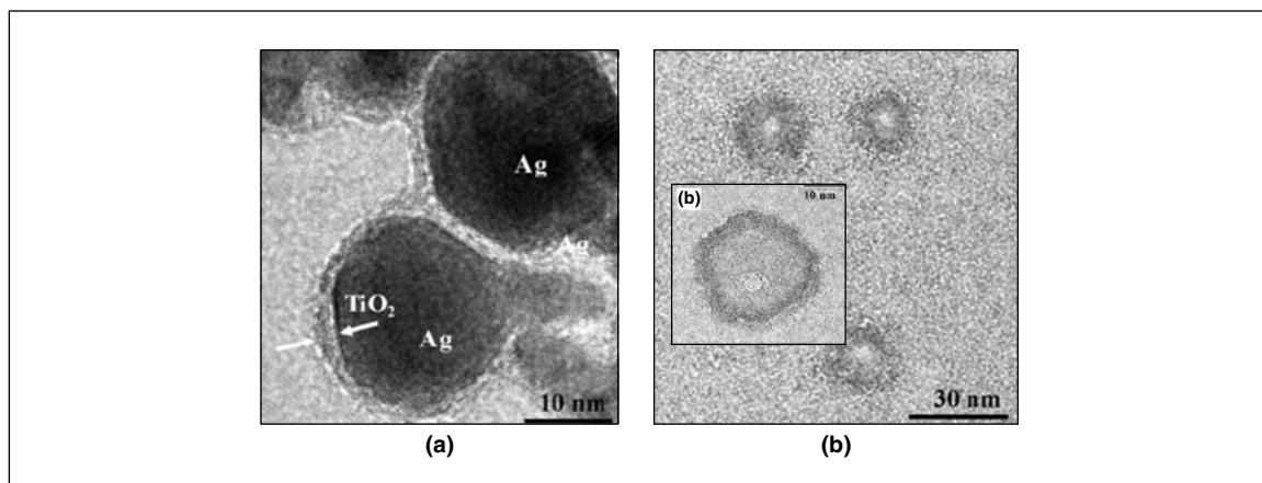
Fig. 9.17: TEM images of \text{Ag@TiO}_2 core-shell nanoparticles (a) and the \text{TiO}_2 nanoshells formed from the same after leaching the core with \text{NH}_3 . The inset of Fig. 9.17. (b) shows an expanded view of a \text{TiO}_2 shell. Reprinted from Ref. 46. Copyright (2002) Wiley-VCH.
