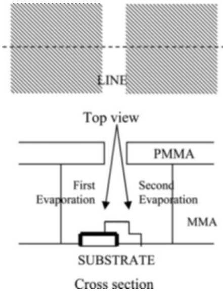
Figure 2. Schematic of the Double-Angle Evaporation Process
