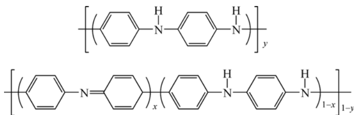
Figure 2.5 Modified molecular structure of the protonated PANI by adding protonation parameter ( x ) [15]
