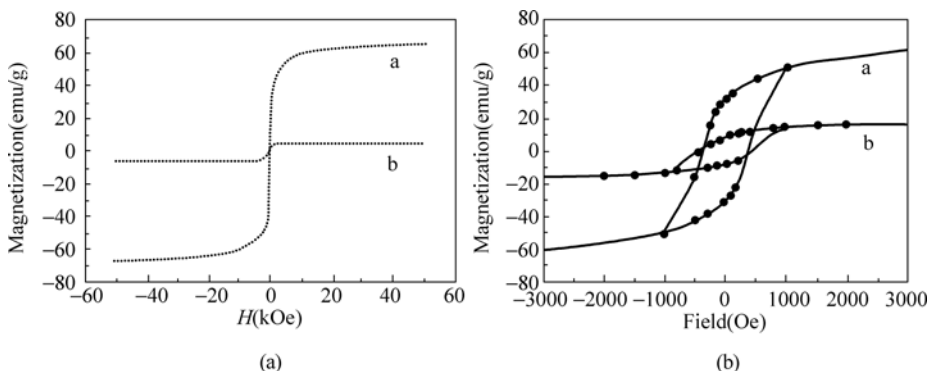
Figure 5.29 Dependence of magnetization on the applied magnetic field at room temperature: Fe 3 O 4 nano-particles and PANI-H 3 PO 4 /Fe 3 O 4 nanotubes (a) as well as γ-Fe 2 O 3 and PANI-H 3 PO 4 /γ-Fe 2 O 3 nanofibers (b) [134]
