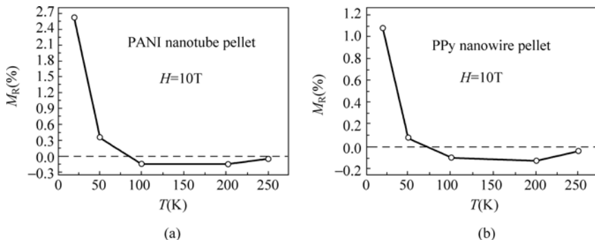
Figure 5.54 Temperature dependence of magneto-resistance of (a) polyaniline nanotube pellet and (b) polypyrrole nanowire pellet at H = 10\text{ T} [242]
