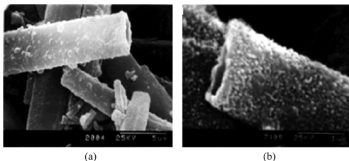
Figure 5.62 SEM images of the microtubes of PANI- \beta -NSA (a) and PANI- \beta -NSA/ D -glucose (b) prepared by template-free method [16]
