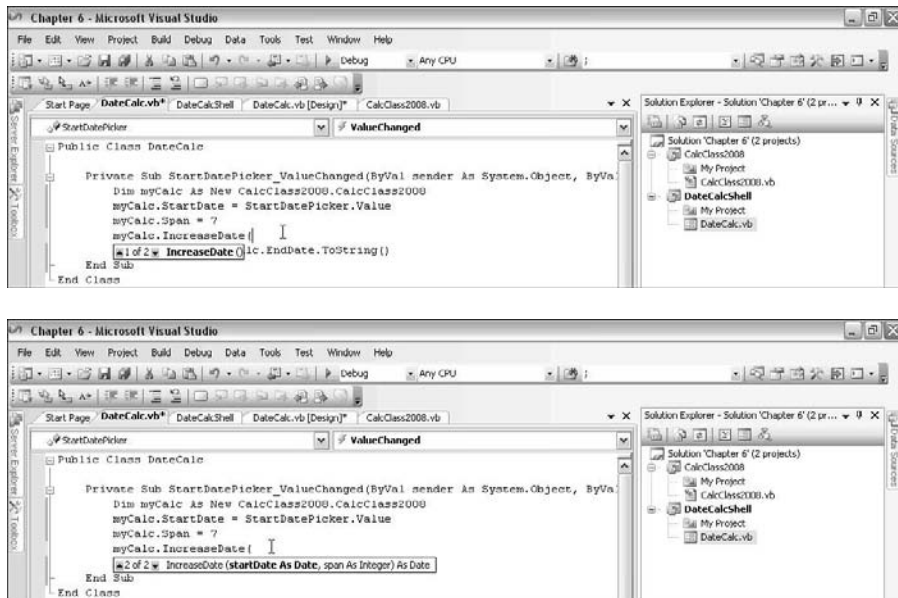
Figure 6-6: Overloading in the IDE—IntelliSense shows two overloads.
