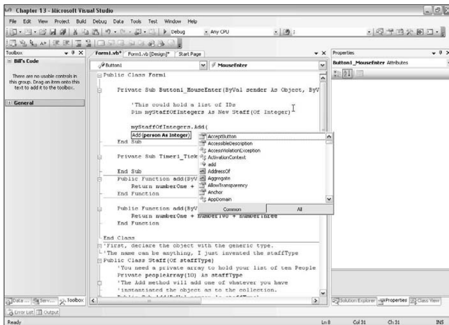
Figure 13-5: Using generics.
