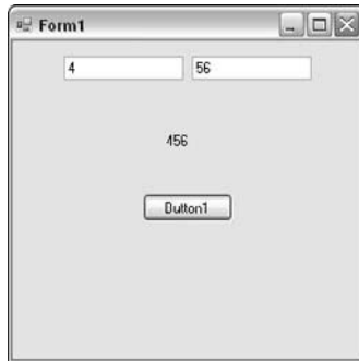
Figure 9-2: New math.
