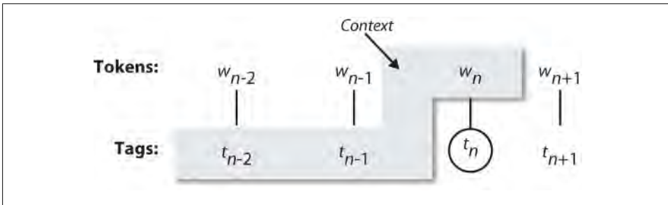
Figure 5-5. Tagger context.
