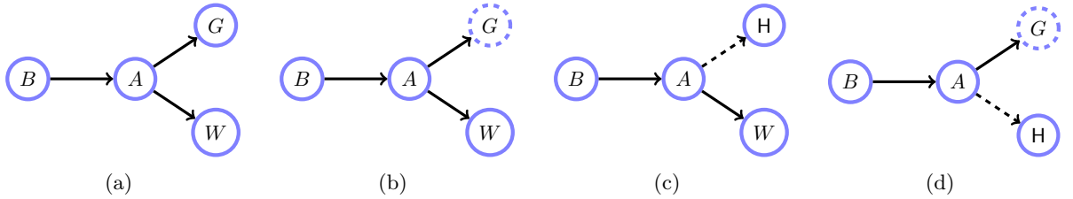
Figure 3.3: (a): Mr Holmes' burglary worries as given in [221]: (B)urglar, (A)larm, (W)atson, Mrs (G)ibbon. (b): Mrs Gibbon's uncertain evidence represented by a dashed circle. (c): Virtual evidence or the replacement of unreliable evidence can be represented by a dashed line. (d): Mrs Gibbon is uncertain in her evidence. Holmes also replaces the unreliable Watson with his own interpretation.
