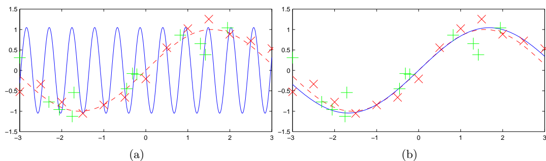
Figure 13.4: (a): The unregularised fit ( \lambda = 0 ) to training given by \times . Whilst the training data is well fitted, the error on the validation examples, denoted by + , is high. (b): The regularised fit ( \lambda = 0.5 ). Whilst the train error is high, the validation error is low. The true function which generated the noisy data is the dashed line; the function learned from the data is given by the solid line.
