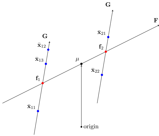
Figure 21.3: Latent Identity Model. The mean \boldsymbol{\mu} represents the mean of the faces. The subspace \mathbf{F} represents the directions of variation of different faces so that \mathbf{f}_1 = \boldsymbol{\mu} + \mathbf{F}\mathbf{h}_1 is a mean face for individual 1, and similarly for \mathbf{f}_2 = \boldsymbol{\mu} + \mathbf{F}\mathbf{h}_2 . The subspace \mathbf{G} denotes the directions of variability for any individual face, caused by pose, lighting etc. This variability is assumed the same for each person. A particular mean face is then given by the mean face of the person plus pose/illumination variation, for example \bar{\mathbf{x}}_{12} = \mathbf{f}_1 + \mathbf{G}\mathbf{w}_{12} . A sample face is then given by a mean face \bar{\mathbf{x}}_{ij} plus Gaussian noise from \mathcal{N}(\boldsymbol{\epsilon}_{ij}|\mathbf{0}, \boldsymbol{\Sigma}) .
