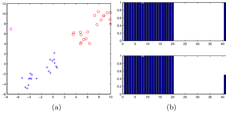
Figure 20.9: Class conditional GMM training and classification. (a): Data from two different classes. We fit a GMM with two components to the data from each class. The (magenta) diamond is a test point far from the training data we will classify. (b): Upper subpanel are the class probabilities p(c = 1|n) for the 40 training points, and the 41 st point, being the test point. The lower subpanel are the class probabilities but including the additional large variance Gaussian term. See demoGMMclass.m .
