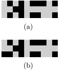
Figure 26.7: (a): The training sequence consists of a random set of vectors ( V = 3 ) over T = 10 time steps. (b): The reconstruction using H = 7 hidden units. The initial state \mathbf{v}(t = 1) for the recalled sequence was set to the correct initial training value albeit with one of the values flipped. Note that the method is capable of sequence disambiguation in the sense that the transitions of the form \mathbf{a}, \mathbf{b}, \dots, \mathbf{a}, \mathbf{c} can be recalled.
