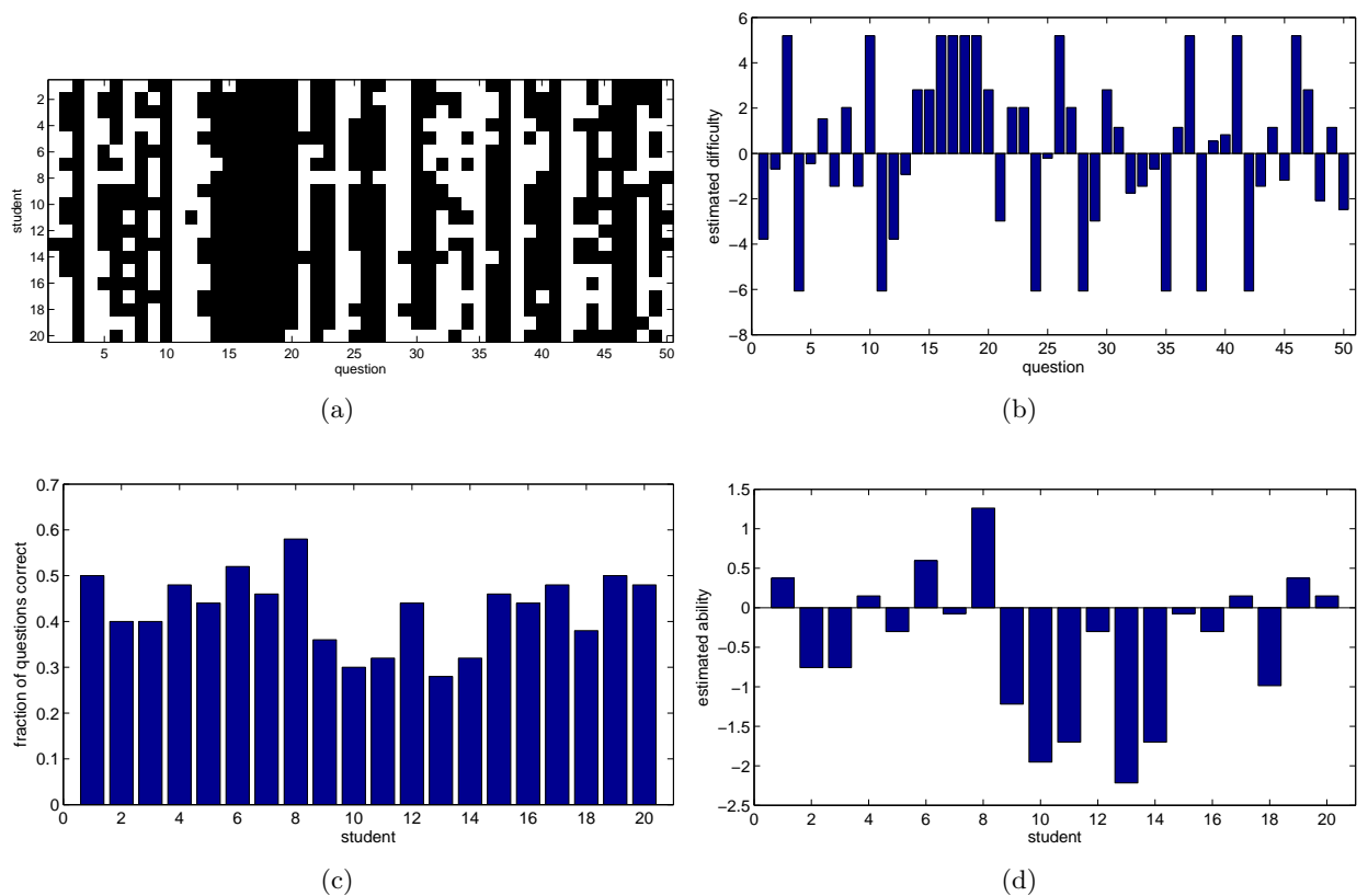
Figure 22.2: Rasch model. (a) : The data of correct answers (white) and incorrect answers (black). (b) : The estimated latent difficulty of each question. (c) : The fraction of questions each student answered correctly. (d) : The estimated latent ability.
