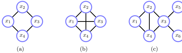
Figure 4.1: (a): \phi(x_1, x_2)\phi(x_2, x_3)\phi(x_3, x_4)\phi(x_4, x_1)/Z_a (b): \phi(x_1, x_2, x_3, x_4)/Z_b (c): \phi(x_1, x_2, x_4)\phi(x_2, x_3, x_4)\phi(x_3, x_5)\phi(x_3, x_6)/Z_c .
