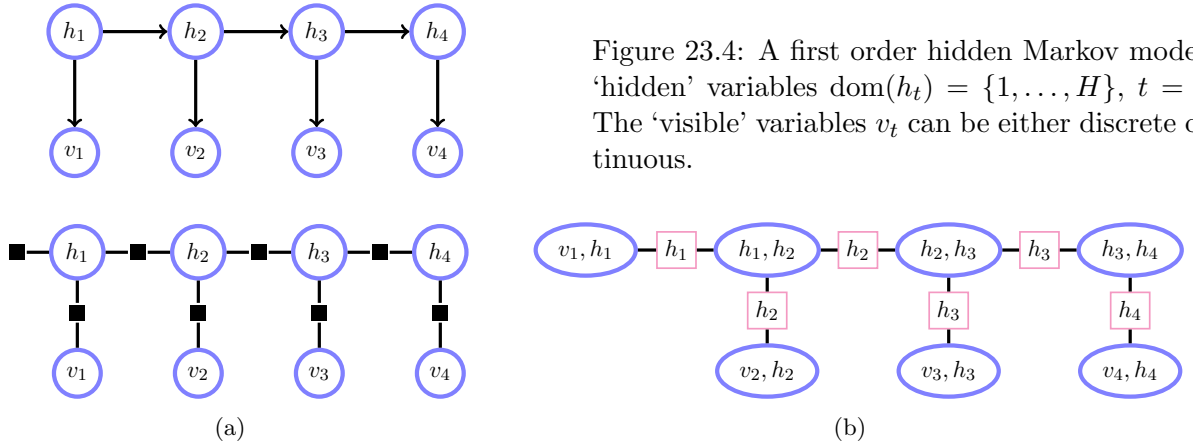
Figure 23.5: (a): Factor graph for the first order HMM of fig(23.4). (b): Junction tree for fig(23.4).
