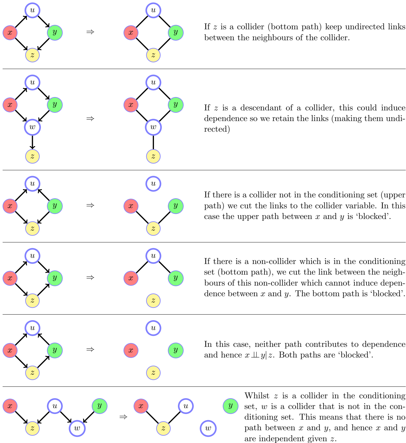
Figure 3.9: Graphical manipulations to determine independence x \perp\!\!\!\perp y \mid z . After these manipulations, if there is no undirected path between x and y , then x and y are independent, conditioned on z . Note that the graphical rules here differ from those in definition(3.3) which considered the effect on the graph having eliminated a variable (via conditioning or marginalisation). Here we consider rules for determining independence based on a graphical representation in which the variables remain in the graph.
