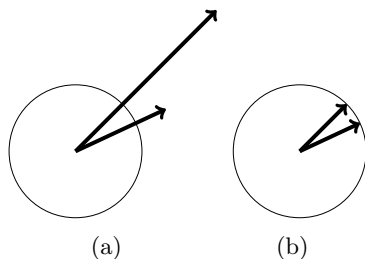
Figure 15.10: (a): Two bag-of-word vectors. The Euclidean distance between the two is large. (b): Normalised vectors. The Euclidean distance is now related directly to the angle between the vectors. In this case two documents which have the same relative frequency of words will both have the same dissimilarity, even though the number of occurrences of the words is different.
