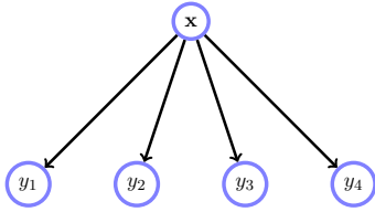
Figure 28.7: An information transfer problem. For a fixed distribution p(\mathbf{x}) and parameterised distributions p(y_j|\mathbf{x}) = \sigma(\mathbf{w}_i^\top \mathbf{x}) , find the optimal parameters \mathbf{w}_i that maximise the mutual information between the variables \mathbf{x} and \mathbf{y} . Such considerations are popular in theoretical neuroscience and aim to understand how the receptive fields \mathbf{w}_i of a neuron relate to the statistics of the environment p(x) .
