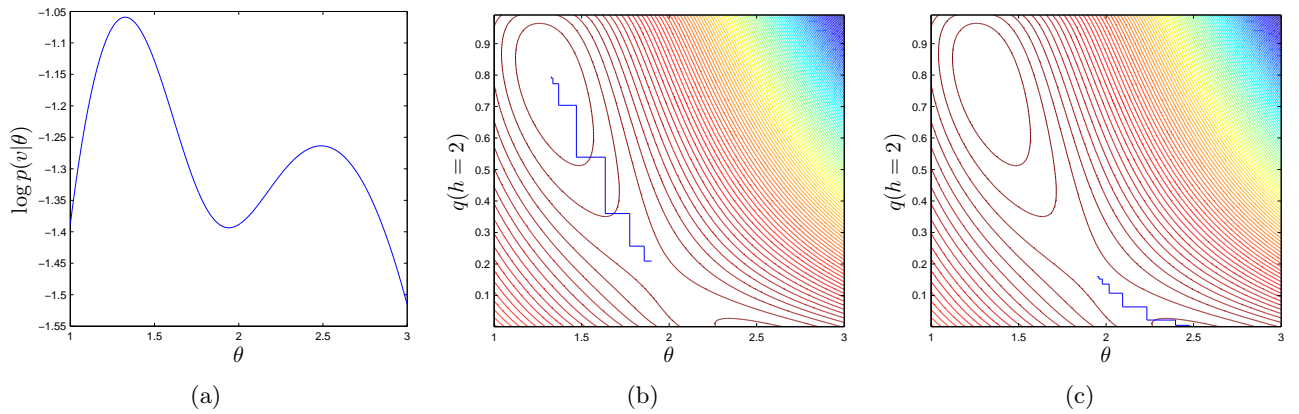
Figure 11.2: (a): The log likelihood for the model described in example(11.2). (b): Contours of the lower bound LB(q(h=2), \theta) . For an initial choice q(h=2) = 0.5 and \theta = 1.9 , successive updates of the E (vertical) and M (horizontal) steps are plotted. (c): Starting at \theta = 1.95 , the EM algorithm converges to a local optimum.
