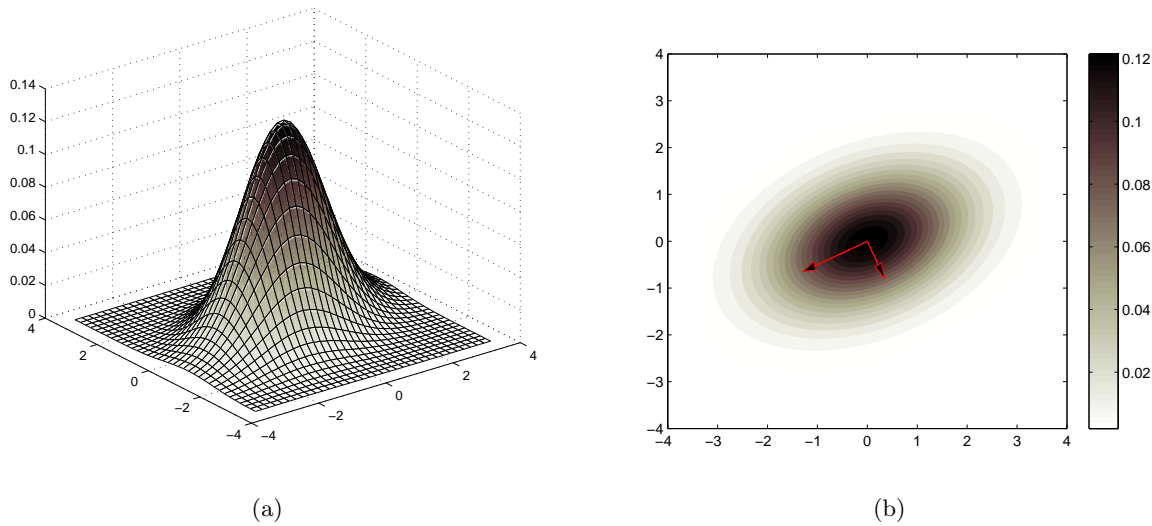
Figure 8.6: (a): Bivariate Gaussian with mean (0, 0) and covariance [1, 0.5; 0.5, 1.75] . Plotted on the vertical axis is the probability density value p(x) . (b): Probability density contours for the same bivariate Gaussian. Plotted are the unit eigenvectors scaled by the square root of their eigenvalues, \sqrt{\lambda_j} .
