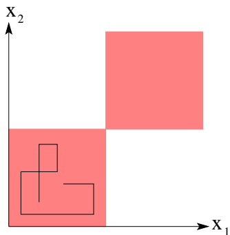
Figure 27.5: A two dimensional distribution for which Gibbs sampling fails. The distribution has mass only in the shaded quadrants. Gibbs sampling proceeds from the l^{\text{th}} sample state (x_1^l, x_2^l) and then sampling from p(x_2|x_1^l) , which we write (x_1^{l+1}, x_2^{l+1}) where x_1^{l+1} = x_1^l . One then continues with a sample from p(x_1|x_2 = x_2^{l+1}) , etc. If we start in the lower left quadrant and proceed this way, the upper right region is never explored.
