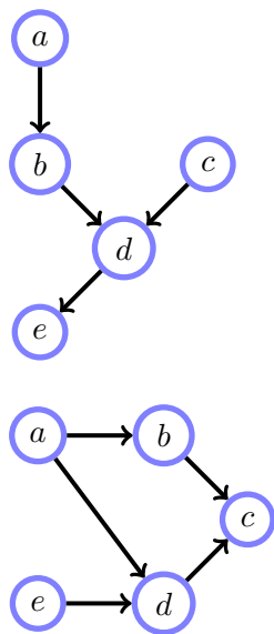
Figure 3.8: Collider examples for d -separation and d -connection.
