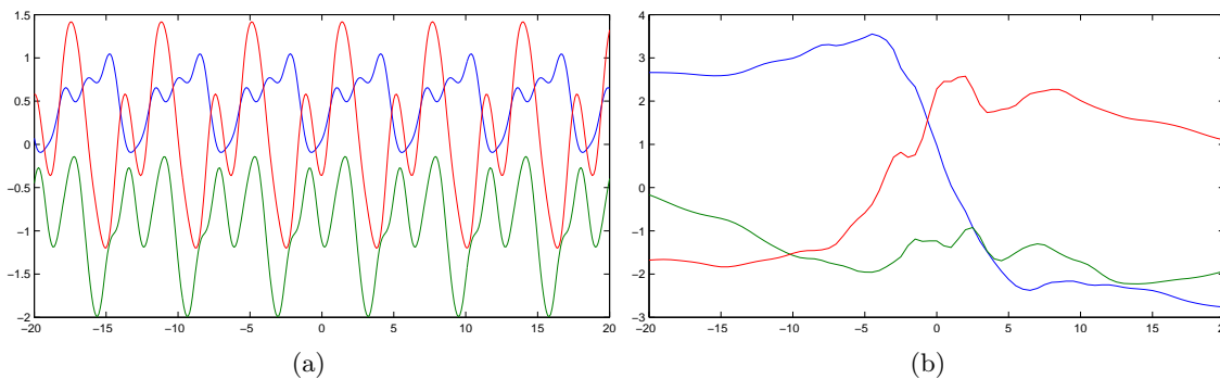
Figure 19.4: Samples from a GP prior for 500 x points uniformly placed from -20 to 20. (a): Sampled from the periodic covariance function \exp(-2\sin^2 0.5(x-x')) . (b): Neural Network covariance function with bias b = 5 and \lambda = 1 .
