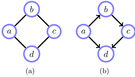
Figure 4.9: (a): An undirected model for which we wish to find a directed equivalent. (b): Every DAG with the same structure as the undirected model must have a situation where two arrows will point to a node, such as node d (otherwise one would have a cyclic graph). Summing over the states of variable d will leave a DAG on the variables a, b, c with no link between a and c . This cannot represent the undirected model since when one marginalises over d this adds a link between a and c .
