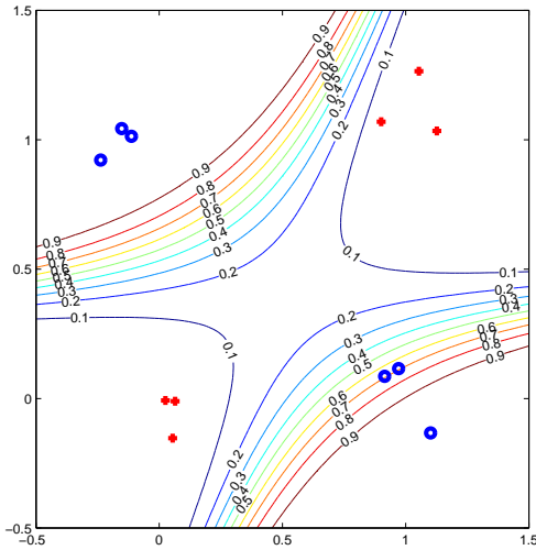
Figure 17.12: Logistic regression p(c = 1|\mathbf{x}) = \sigma(\mathbf{w}^\top \phi(\mathbf{x})) using a quadratic function \phi(\mathbf{x}) = (1, x_1, x_2, x_1^2, x_2^2, x_1x_2)^\top . 1000 iterations of gradient ascent training were performed with a learning rate \eta = 0.1 . Plotted are the datapoints for the two classes (cross) and (circle) and the equal probability contours. The decision boundary is the 0.5-probability contour. See demoLogRegNonLinear.m .
