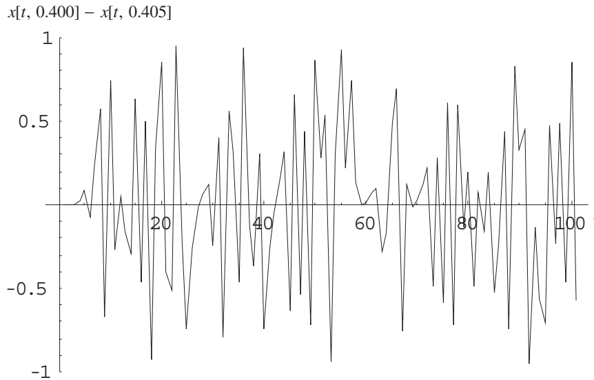
Figure 1.1.3: Small differences at the beginning signify much
