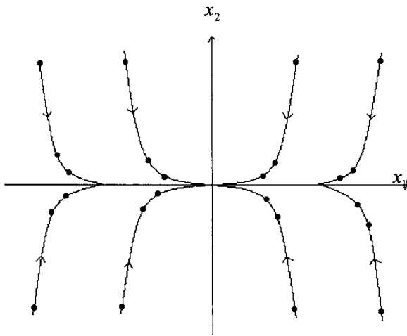
Figure 6.1.1: \rho_1 < \rho_2 < 1 , asymptotically stable node
