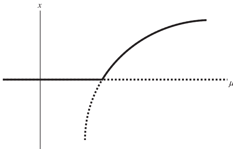
Figure 4.4.5: Transcritical bifurcation for f = \mu x(1 - x)
