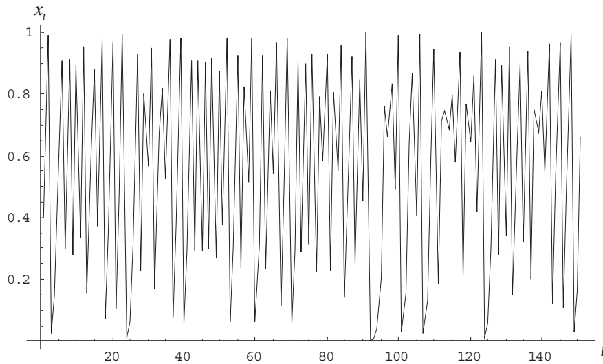
Figure 1.1.1: Chaos when a = 5.75 and x_0 = 0.4
