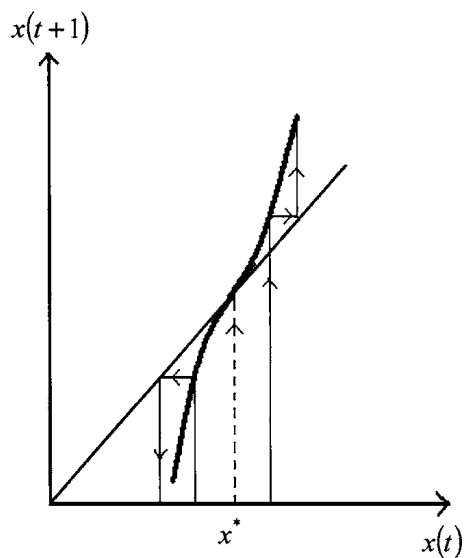
(c) unstable f''(x^*) = 0, f'''(x^*) > 0
