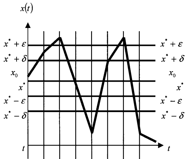
Figure 2.3.2: Unstable x_0
