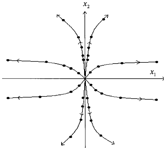
Figure 6.1.2: \rho_1 > \rho_2 > 1 , unstable node
