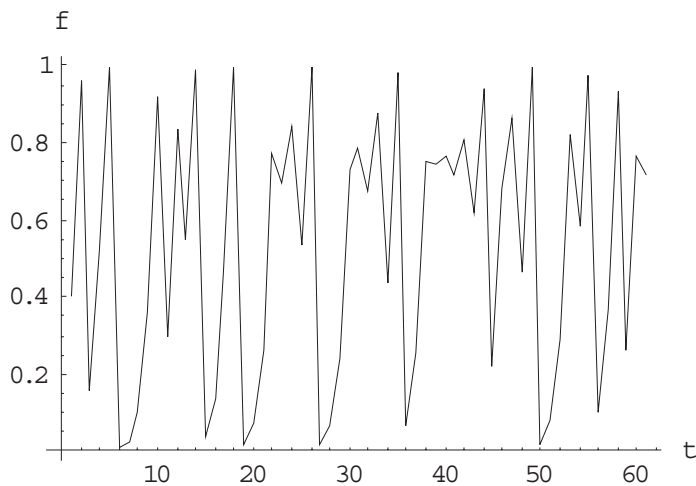
Figure 2.2.3: Time series plot of O(0.4) for f(x) = 4x(1-x)
