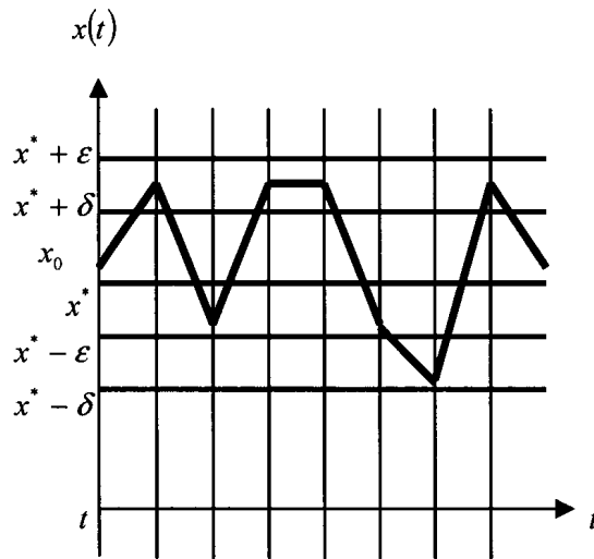
Figure 2.3.1: Stable x_0
