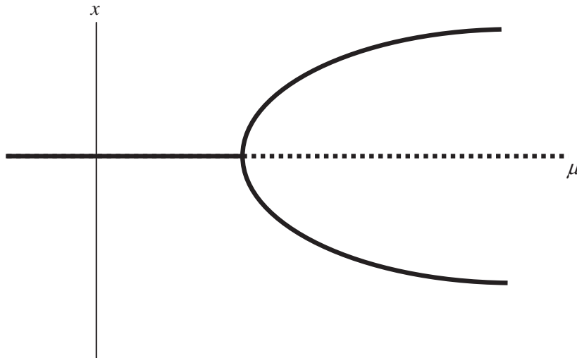
Figure 4.4.4: Supercritical pitchfork bifurcation for f = \mu x - x^3
