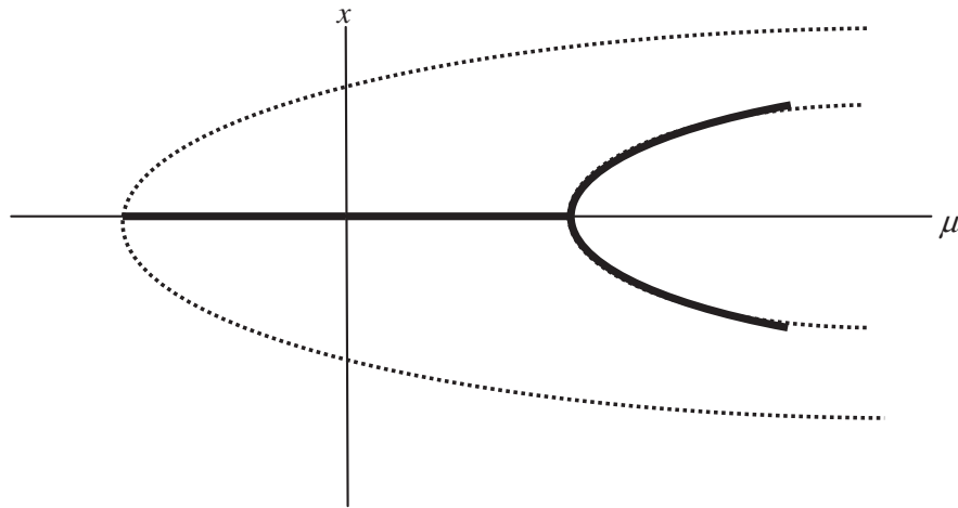
Figure 4.4.1: Part of the bifurcation diagram of f = \mu x - x^3
