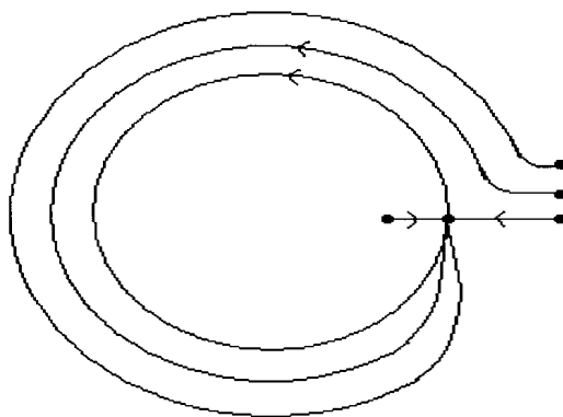
Figure 6.4.4: Attractive but not stable equilibrium
