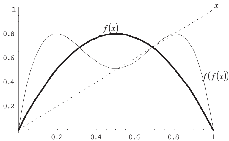
Figure 4.1.1: The solution of period 2 to f(x) = 3.2x(1 - x)
