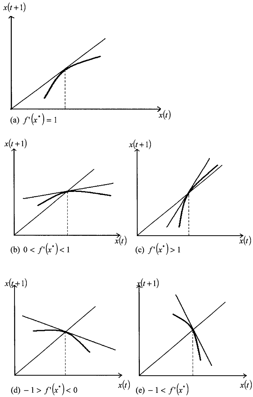
Figure 2.3.3: Stability types of scalar difference equations
