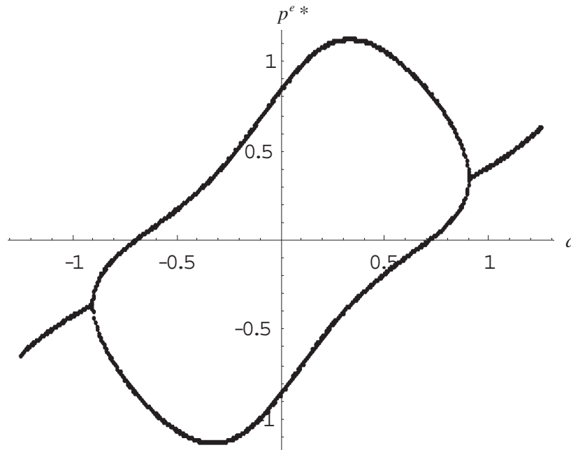
Figure 4.6.3: Bifurcation diagram for \mu = 3 , a \in [-1.25, 1.25]
