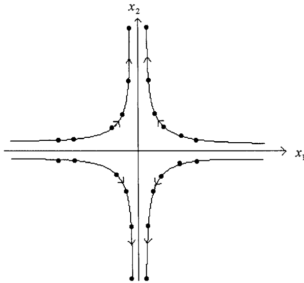
Figure 6.1.3: 0 < \rho_1 < 1, \rho_2 > 1 , saddle (unstable)
