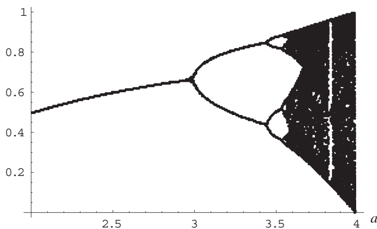
Figure 4.2.2: The bifurcation diagram of f = ax(1 - x)
