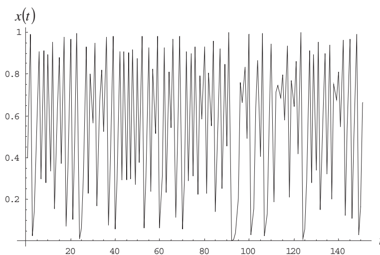
Figure 5.7.2: The existence of chaos for a = 5.75 with x_0 = 0.4
