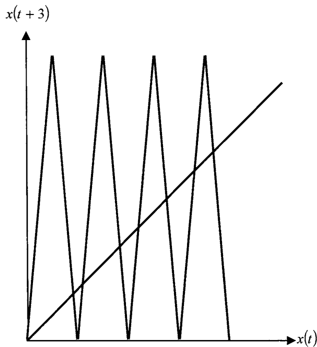
Figure 4.3.2: Fixed points of T^3
