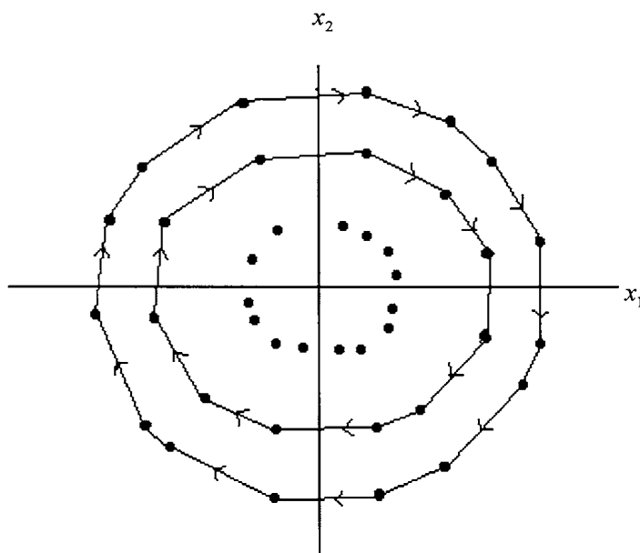
Figure 6.1.10: |\rho| = 1 , center (stable)
