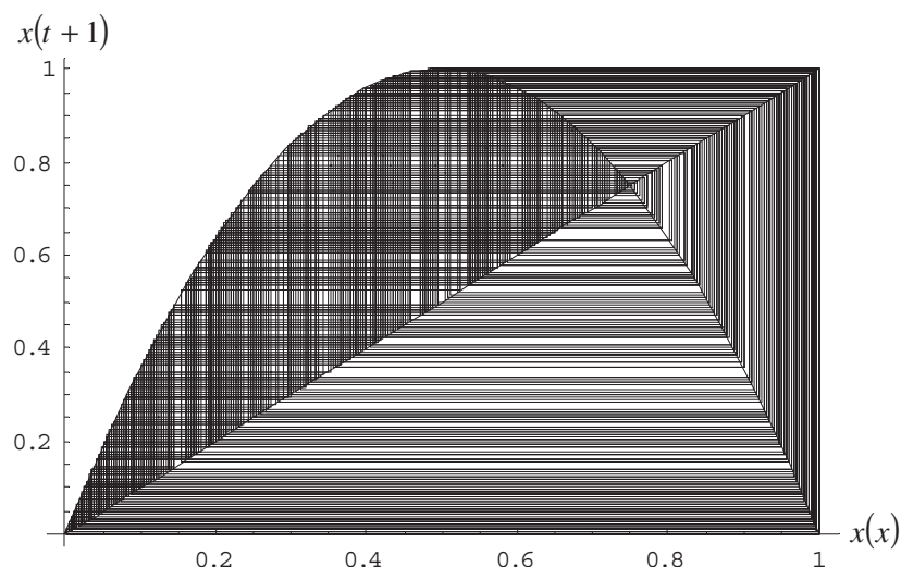
Figure 4.3.1: The orbit of f(x) = 4x(1 - x) with x_0 = 0.3
