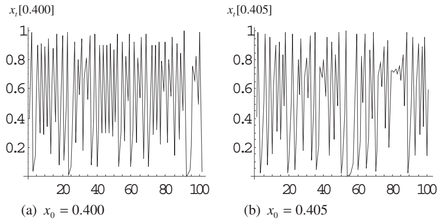
Figure 5.7.3: The dynamics with different initial conditions
