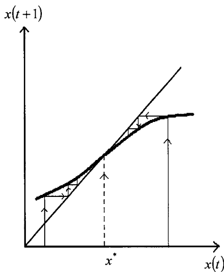
(d) asymptotically stable f''(x^*) = 0, f'''(x^*) < 0
