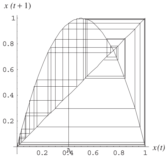
Figure 2.2.2: Staircase diagram of O(0.4) for f(x) = 4x(1-x)
