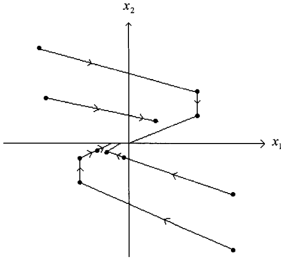
Figure 6.1.6: \rho_1 = \rho_2 < 1 , asymptotically stable node
