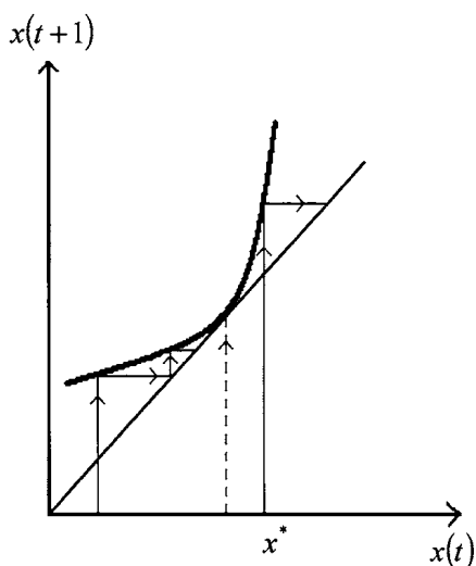
(a) unstable, f''(x^*) > 0 (semistable from the left)
