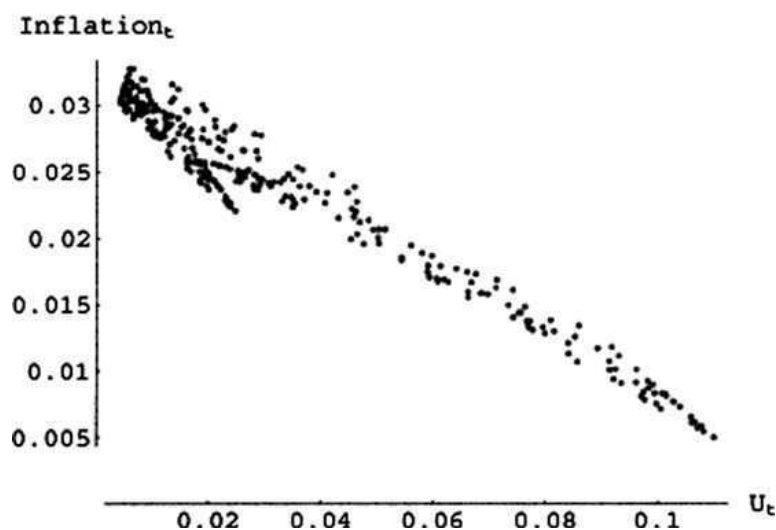
Figure 7.6.2: An attractor
