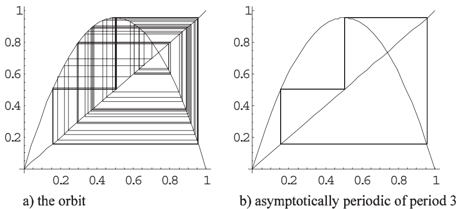
Figure 4.1.2: The orbit of f(x) = 3.82x(1 - x) with x_0 = 0.3
