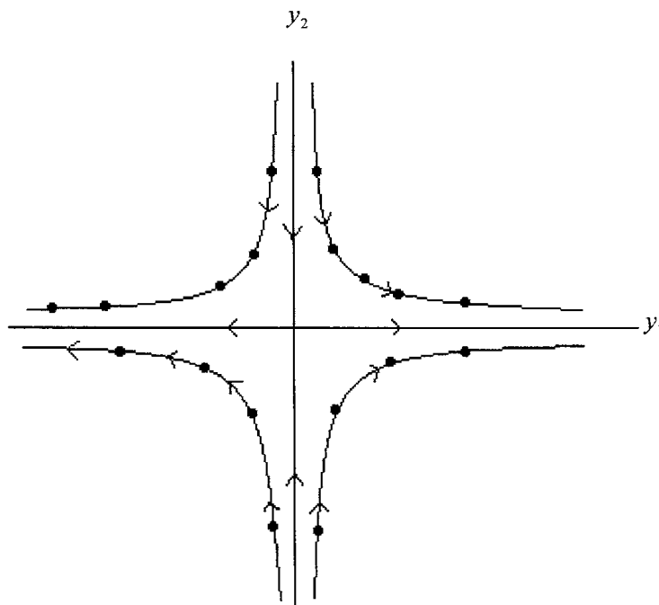
Figure 6.1.11: Saddle of the canonical form, y(t+1) = Jy(t)
