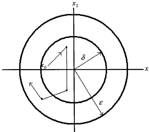
Figure 6.4.1: Stable equilibrium
