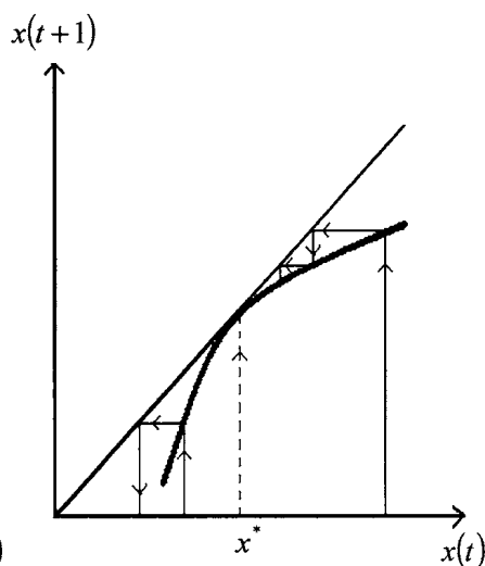
(b) unstable, f''(x^*) < 0 (semistable from the right)
