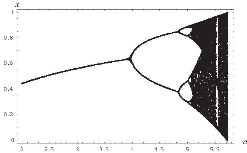
Figure 5.7.5: The map of bifurcations for a \in [2, 5.75]
