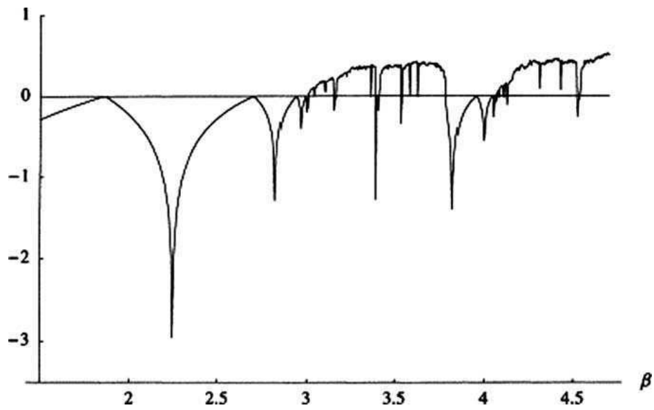
Figure 5.2.1: The Liapunov exponent for 1,5 \leq \beta \leq 4,7 with \alpha = 0,7
