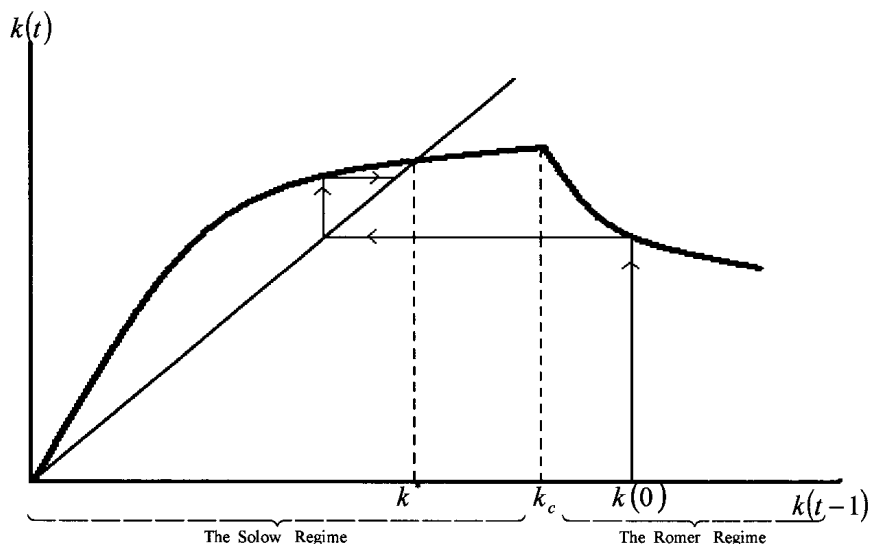
Figure 5.5.1: The growth by the Solow mechanism with sA < 1
