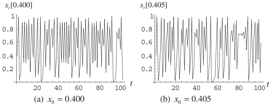
Figure 1.1.2: The dynamics with different initial conditions, a = 5.75
