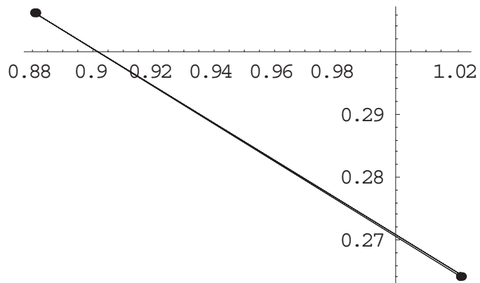
Figure 6.8.2: A 2-cycle for a = 0.3675 and b = 0.3
