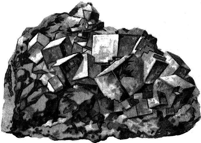
1, 2, Fluorite or Fluor-spar.
