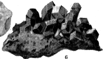
1, 2, Chalcopyrite. 3, Smaltite. 4, Tetrahedrite. 5, Pyrrargyrite. 6, Proustite.
