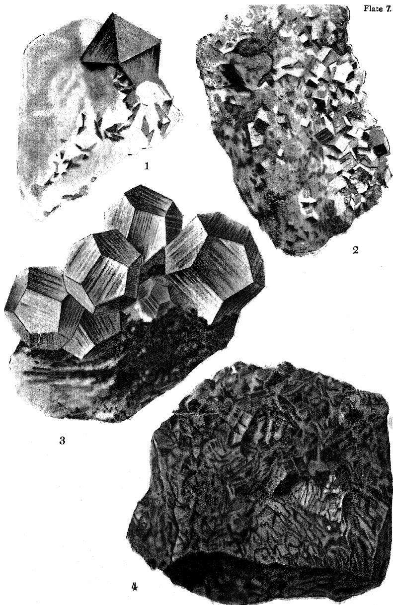
1, Marcasite. 2, 3, Iron-pyrites. 4, Pyrrhotite.
