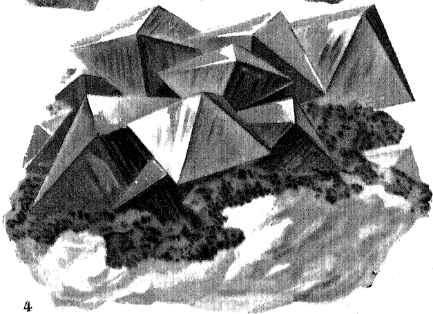
1, Niccolite. 2, 3, Cinnabar. 4, Mispickel or Arsenopyrite.
