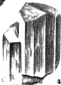
1, 2, Orthoclase. 3, Labradorite. 4, Microcline. 5, Anorthite.
