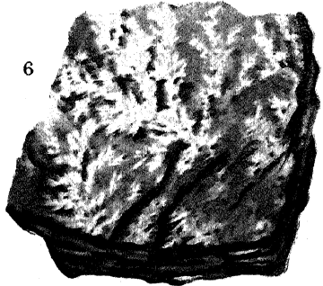
1, Augite. 2, 3, Diopside. 4, Enstatite. 5, Hypersthene. 6, Wollastonite.
