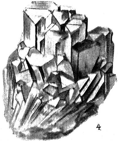
1, 2, Barytes. 3, Anglesite. 4, Celestite.
