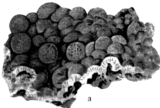
1, Epidote. 2, Axinite. 3, Phehnite.
