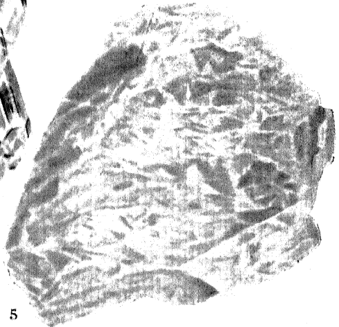
1, Amethyst. 2, Smoky-quartz. 3, Rock-crystal. 4, Cat's-eye. 5, Rose-quartz.
