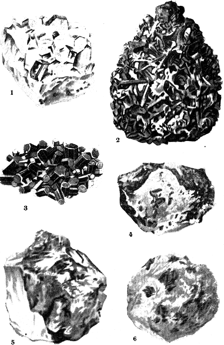
1, Apatite. 2, 3, Pyromorphite. 4, Vanadinite. 5, 6, Erythrite.
