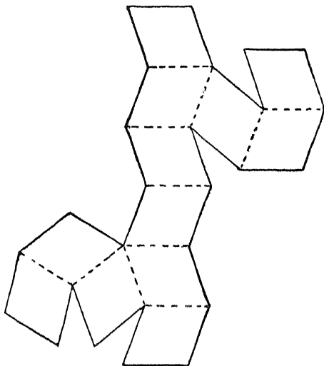
Fig. 6—Net for the construction of a Model of the Rhombic-Dodecahedron.*
