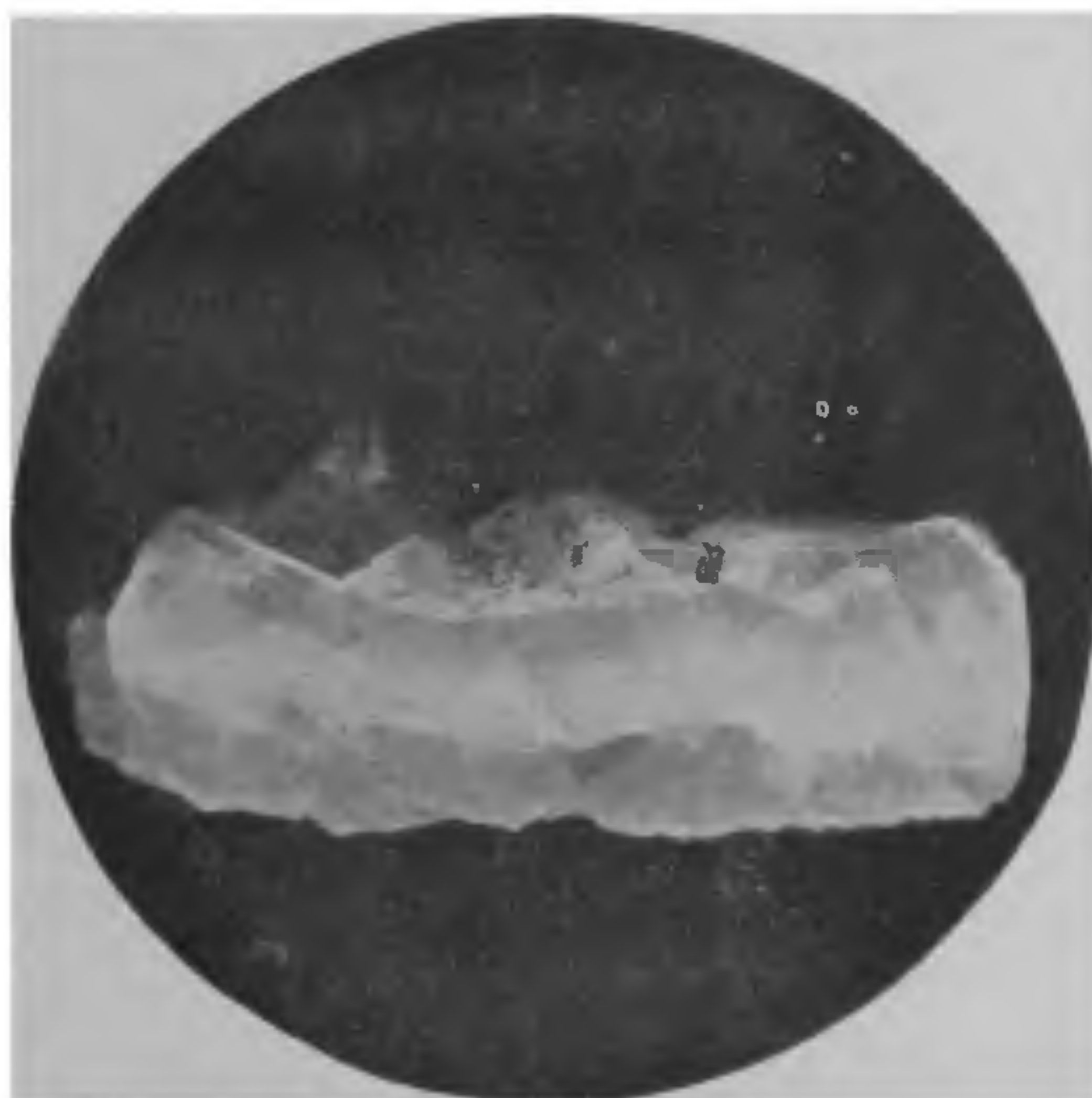
FIG. 3. Luminescent layer in Amba Dongar fluorite.
