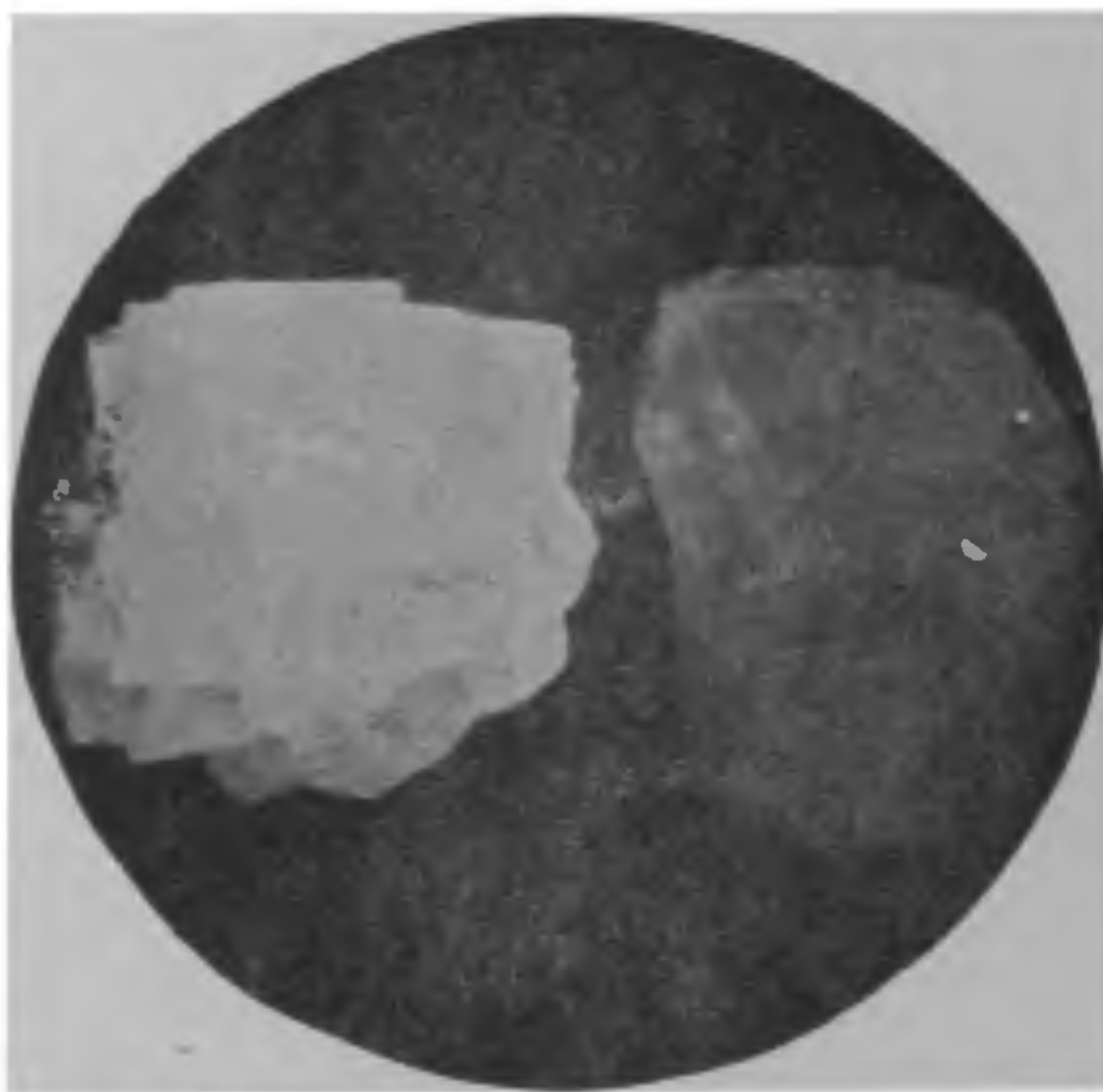
FIG. 2. Luminescent and non-luminescent fluorspar.
