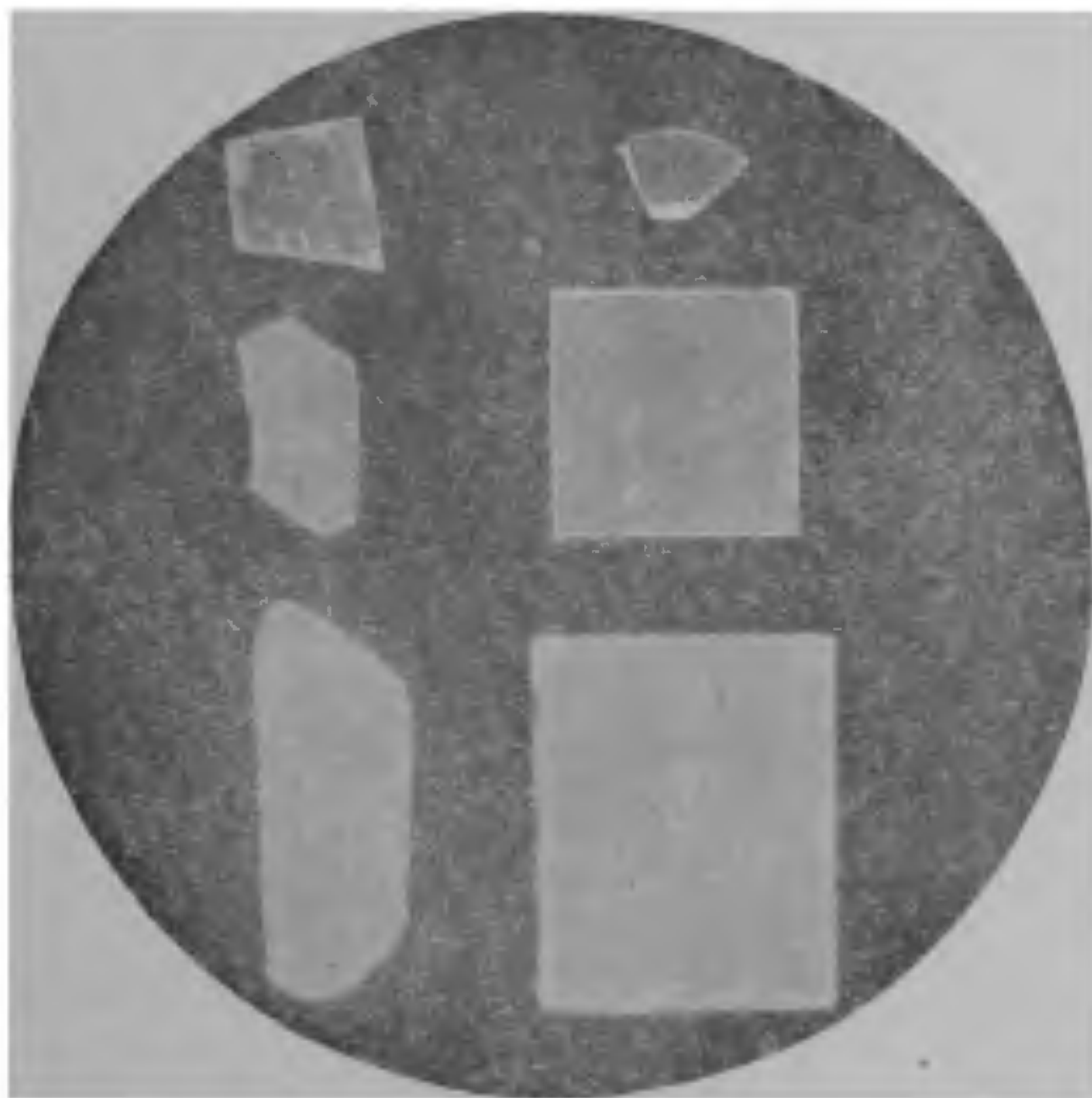
FIG. 1. Six specimens of fluorite under ultra-violet illumination.
