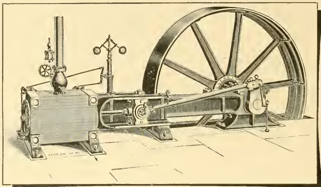
GIRDER FRAME ENGINE.
