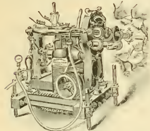
"R" Drill, Capacity 500 ft., Operated by Electricity.
