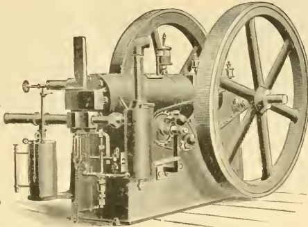
"LEWIS" IMPROVED GAS AND VAPOR ENGINE.
