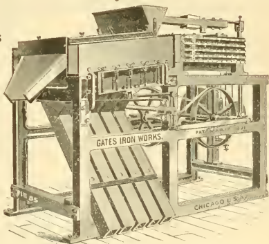
Above cut shows Gates Standard Breaker, with Main Shaft and Crushing Head removed.
