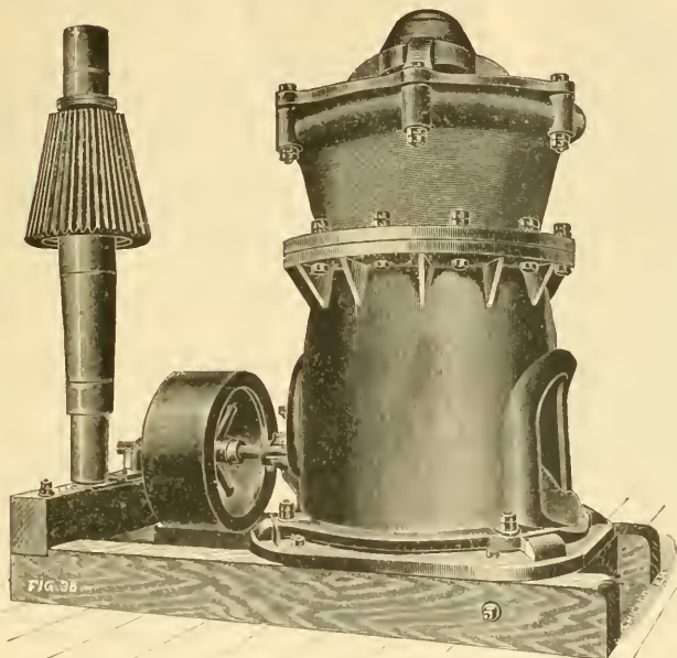
Above cut shows Gates Standard Breaker, with Main Shaft and Crushing Head removed.
