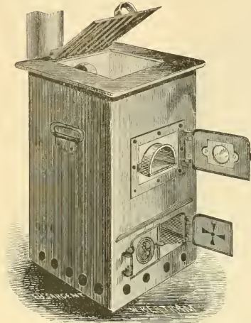
BROWN'S ASSAY FURNACE, "MODEL 1893."
