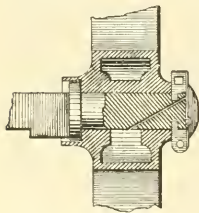
PATENT AXLE AND WHEEL.
