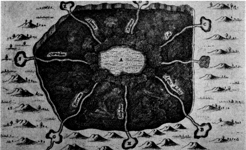
FIG. 69. The water issuing from the subterranean cavern A passes outwards to the surface by several different channels and issues as springs marked B , C , D , E , F , G , H . That coming by the passage A-B passes through rocks containing no soluble matter and issues as pure water. That reaching the surface by A-C passes through a country rock which is impregnated with saline material and issues as a salt spring. The others take up sulphurous, feruginous and other materials from the rocks which they traverse and come to the surface as mineral springs of various kinds. (Kircher, Mundus Subterraneus .)
