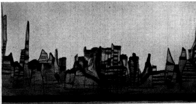
FIG. 53. A section of the "Ruin Marble" of Florence showing castellated forms due to a series of minute faults. (From Knorr, Recueil des Monumens des Catastrophes que le Globe terrestre a essuïées , Nuremberg, 1777.)
