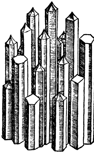
FIG. 25. Columns of Basalt. (From Gesner: De Rerum Fossilium . . . Figuris .)
