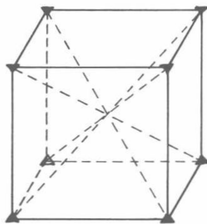
Fig. 8 Corner axes of 3-fold symmetry
