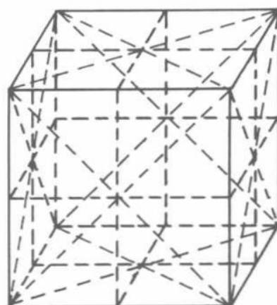
Fig. 11 Planes of symmetry
