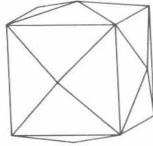
Fig. 15 Tetrahedron
