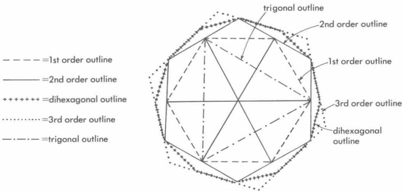
Fig. 19 Hexagon outlines
