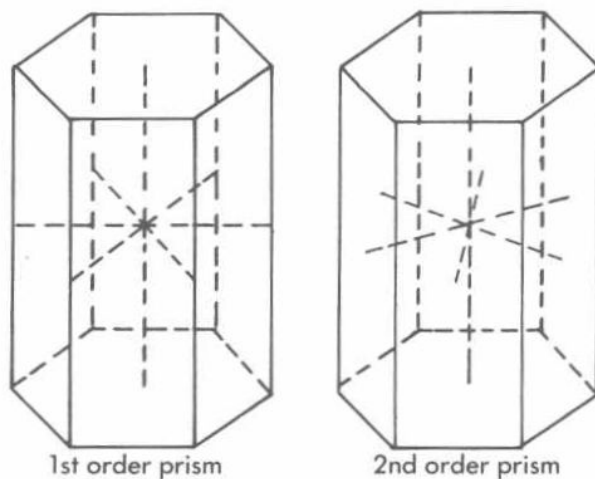
Fig. 18 Hexagonal system prisms
