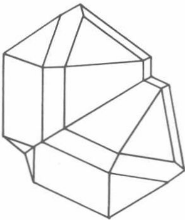
Fig. 27 Cassiterite twin
