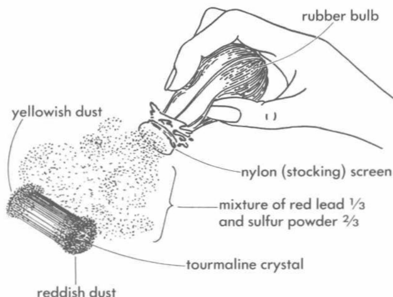
Fig. 6 Piezoelectricity testing device
