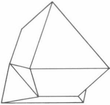
Fig. 24 Spinel twin
