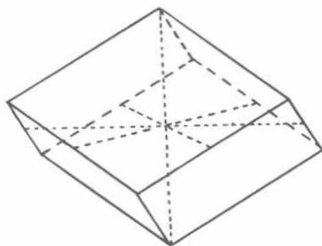
Fig. 20 Rhombohedron axes
