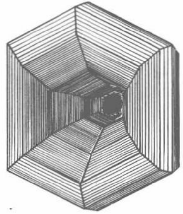
Fig. 26 Rutile "sixling"
