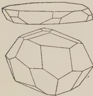
5. Hematite: kidney pp. 124, 38 ore (Cumberland, England)
