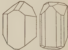
4. Diopside with essonite garnet p. 267 (Ala, Piedmont, Italy)
