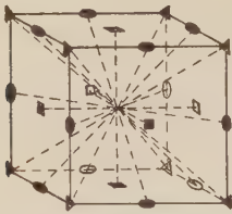
Fig. 10 Cubic axes of symmetry
