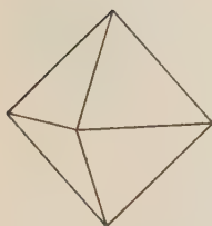
Fig. 29b Normal and elongated octahedron
