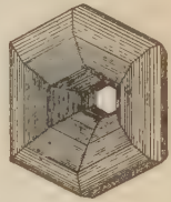
Fig. 26 Rutile "sixling"
