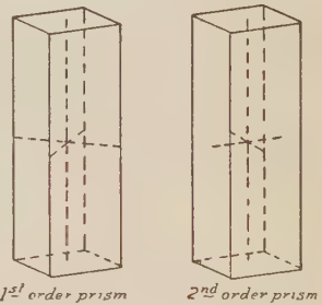
Fig. 17 Tetragonal system prisms
