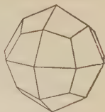
Fig. 16 Trisocta- hedron
