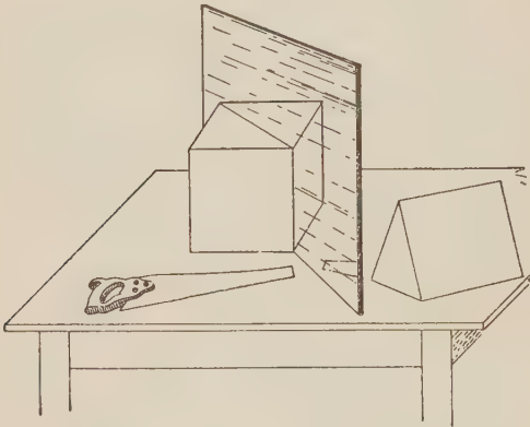
Fig. 11 Plane of symmetry
