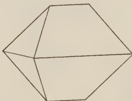
Fig. 29b Normal and elongated octahedron
