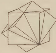
Fig. 25 Penetration twin of fluorite
