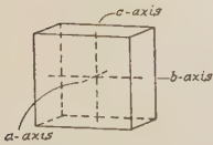
Fig. 21 Orthorhombic system axes and pinacoids
