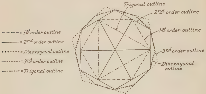
Fig. 19 Hexagon outlines
