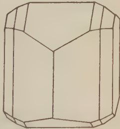
6. Wavellite p. 220 (Hot Springs, Arkansas)
