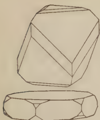
1. Eudialyte grains in rock p. 279 (Naujakasik, Greenland)
