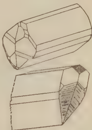
6. Epidote p. 298 (Untersulzbachtal, Austria)
