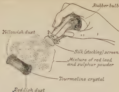
Fig. 6 Piezoelectricity testing device
