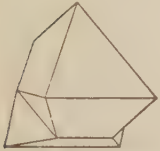
Fig. 24 Spinel twin
