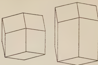
Fig. 29a Normal and elongated dodecahedron
