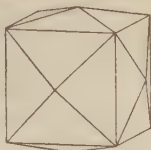
Fig. 15 Tetrahex- ahedron
