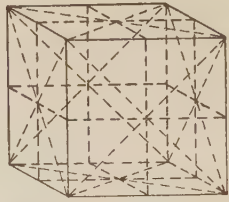
Fig. 12 Planes of symmetry
