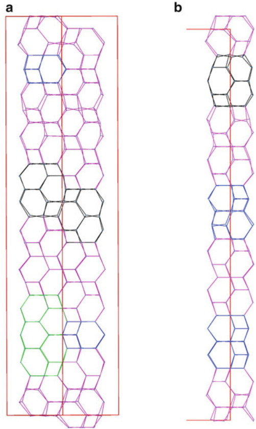
Fig. 1.10 A fragment of the tetrahedral framework (a) and cancrinite-type column (b) in the structure of biachellaite (After Chukanov et al. 2009). The unit cell is outlined
