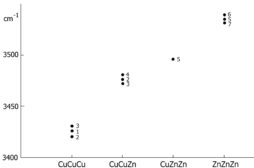
Fig. 1.14 Wavenumbers of the bands of O–H-stretching vibrations for differently coordinated OH groups in Zn-poor olivenite from Tsumeb, Namibia (1); Zn-enriched olivenite from Novoveská Huta, Slovakia (3); zincolivenite from Lavrion, Greece (4); Cu-enriched adamite from Dalnegorsk, Russia (5); Cu-poor adamite from Lavrion, Greece (6) and Cu-poor adamite from Ojuela mine, Mexico (7)
