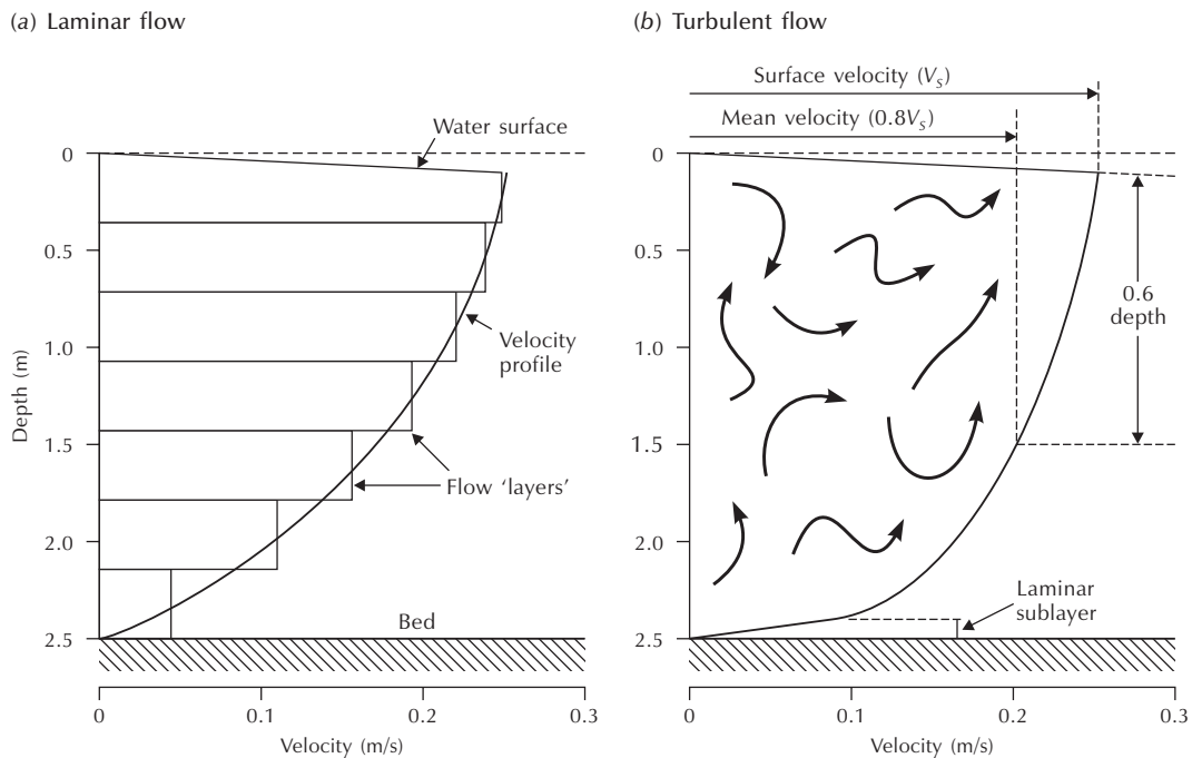
Figure 3.8 Velocity profiles of (a) laminar and (b) turbulent flow in a river.
