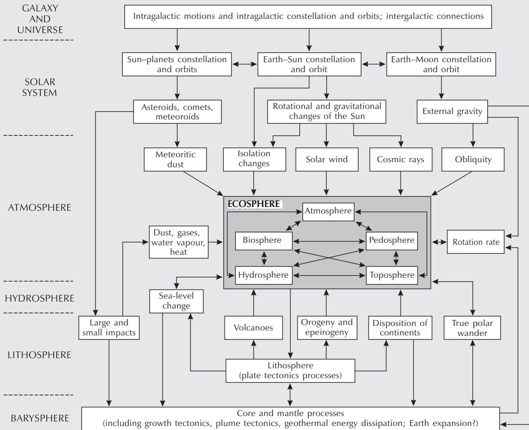
Figure 2.3 Interacting terrestrial spheres and their cosmic and geological settings. Source: Adapted from Huggett (1991, 1995, 1997)
