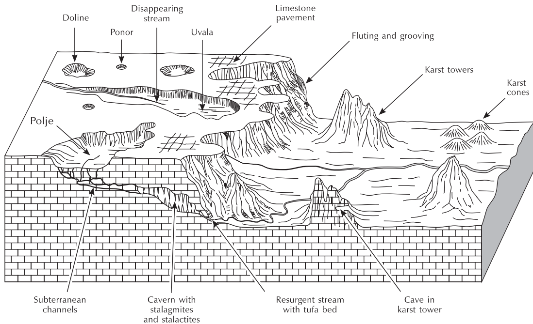
Figure 8.5 Schematic diagram of some karst features.
