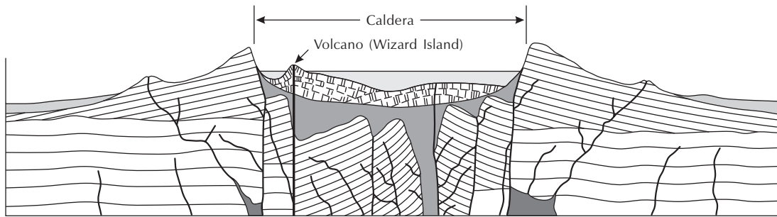
Figure 5.8 Crater Lake caldera, Oregon, USA. Source: Adapted from MacDonald (1972, 301)
