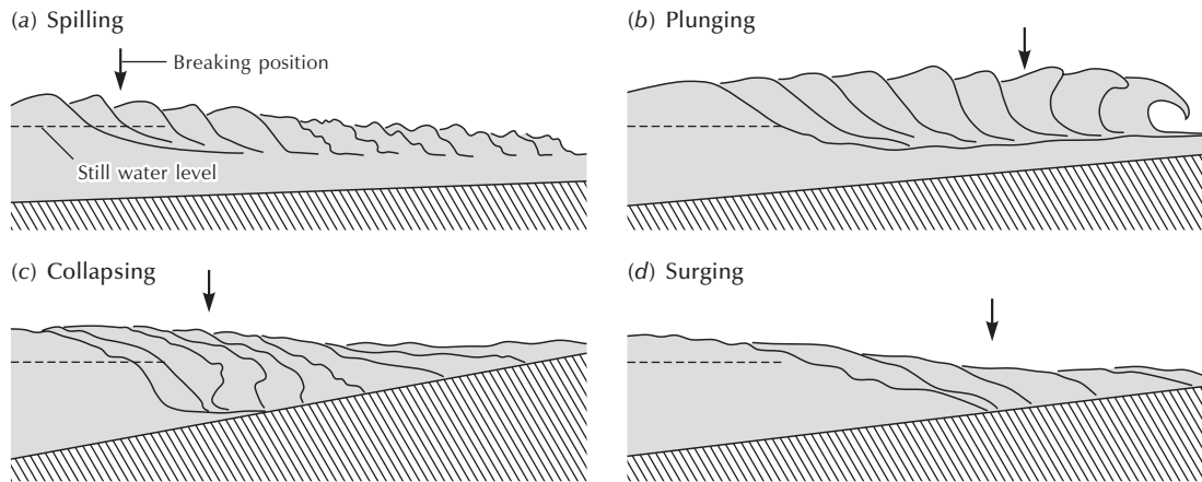
Figure 13.3 Kinds of breaking waves derived from high-speed moving pictures. Source: Adapted from Komar (1998, 210)
