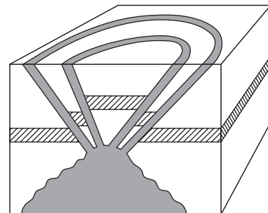
Figure 5.2 Minor intrusions. (a) Laccoliths and associated features (dykes, sills, and bysmaoliths). (b) Cone sheets. Source: Adapted from Sparks (1971, 90, 101)
