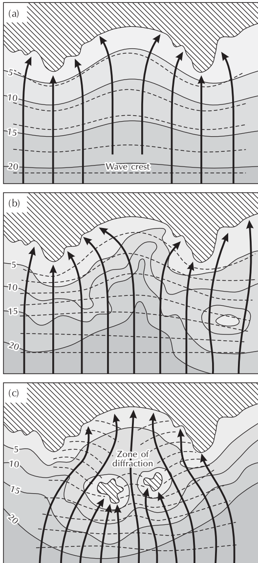
Figure 13.2 Wave refraction approaching headlands and bays above differing offshore topography. Source: Adapted from Bird (2000, 11)
