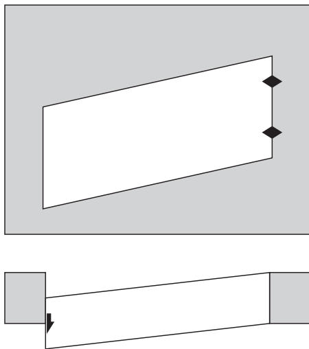
(c) Trapdoor
