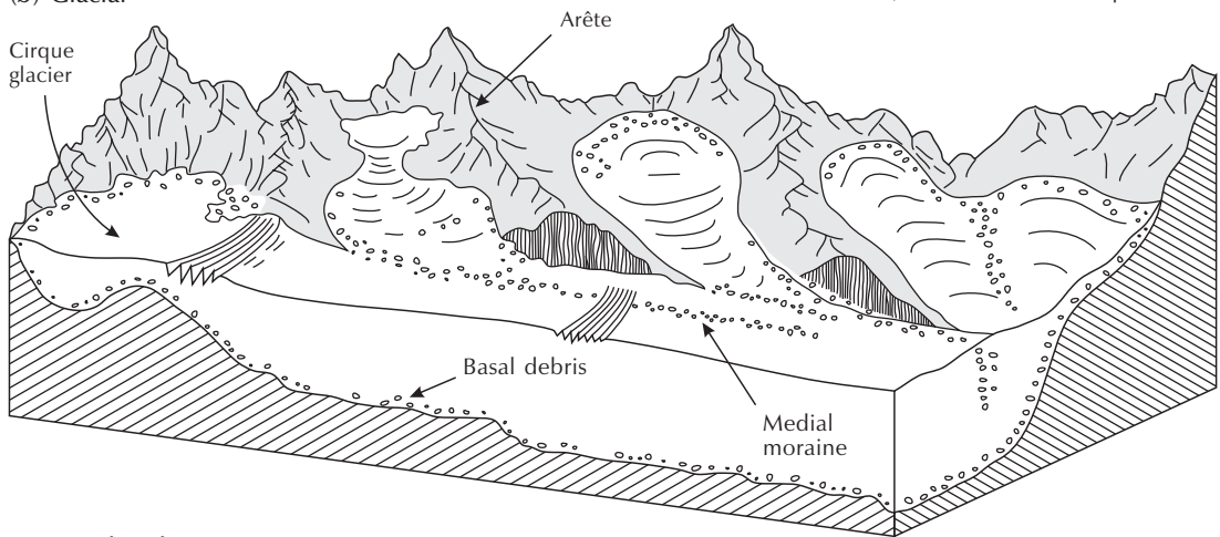
(c) Postglacial
