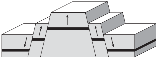
Figure 5.25 Up-faulted structures. (a) Horst. (b) Tilted block.
