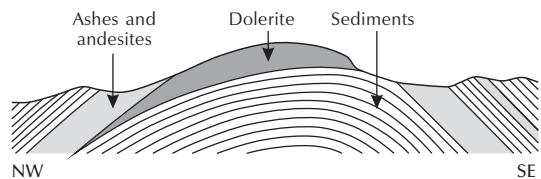
Figure 5.3 Phacoliths. (a) Occurrence in anticlinal crests and synclinal troughs. (b) Corndon Hill, near Montgomery in Wales, an eroded phacolith. Source: Adapted from Sparks (1971, 93, 94)
