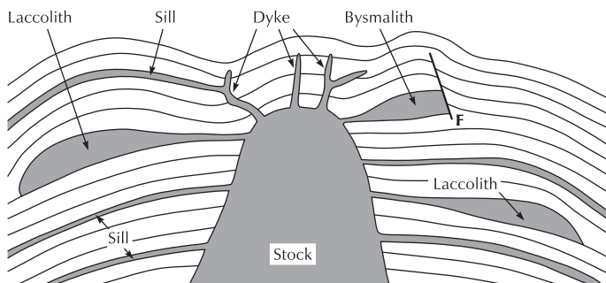
Figure 5.2 Minor intrusions. (a) Laccoliths and associated features (dykes, sills, and bysmaoliths). (b) Cone sheets. Source: Adapted from Sparks (1971, 90, 101)
