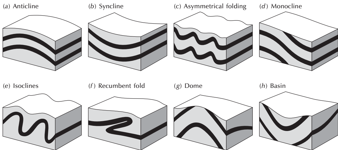
Figure 5.13 Structures formed in folded strata.
