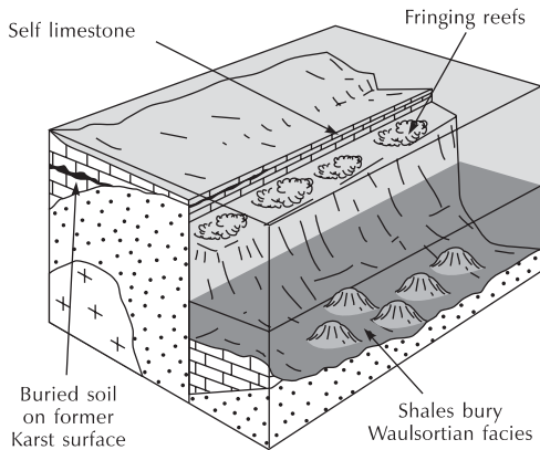
Figure 15.10 Schematic diagram showing the evolution of limestone landscapes in northern England. The Craven Fault, a major east–west fault across the northern Pennines, separates the Askrigg tilt-block from the Craven Deep.
