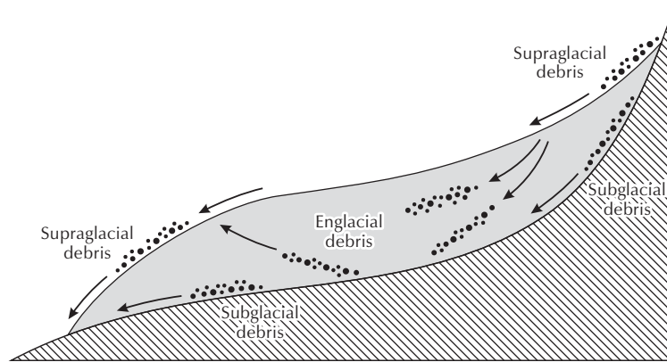
Figure 3.15 Transport by ice: supraglacial, englacial, and subglacial paths. Source: Adapted from Summerfield (1991, 271)
