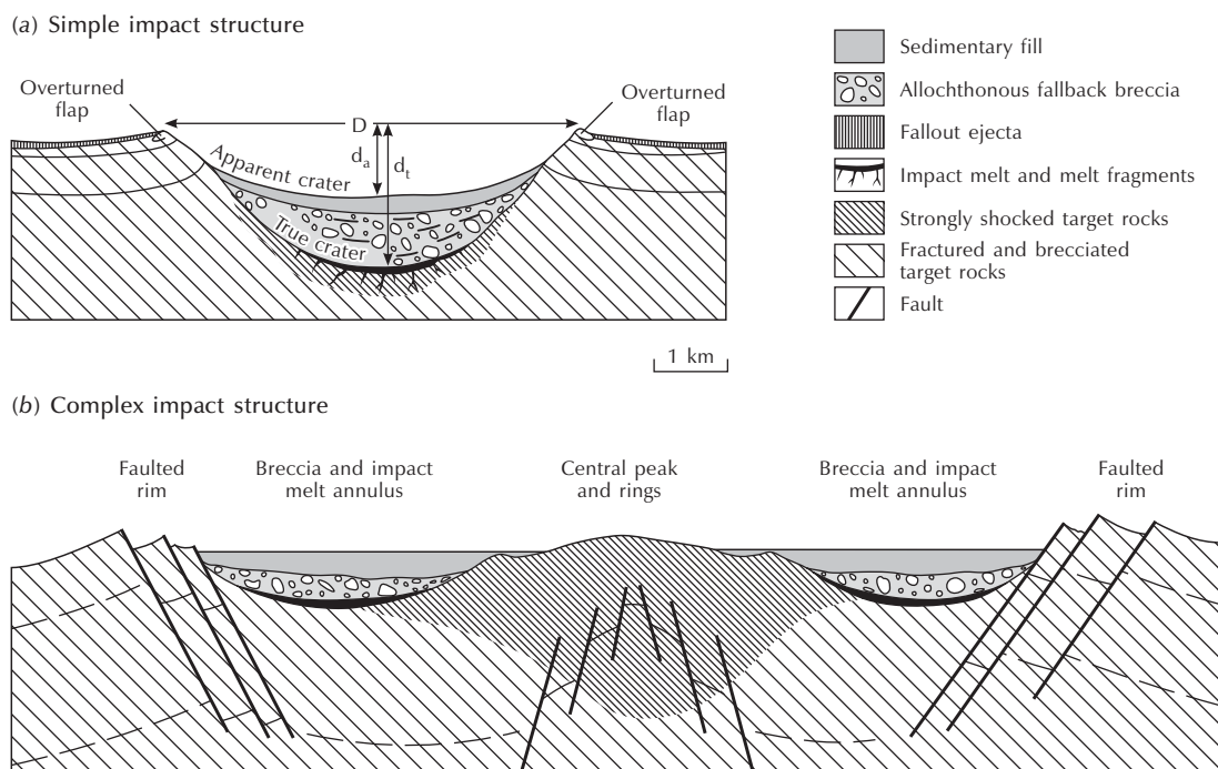
Figure 5.11 Simple and complex impact structures.
