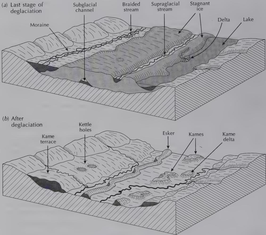
Figure 8.5 Subglacial and ice-margin landforms. (a) A landscape at the final stage of deglaciation. (b) A landscape after deglaciation.
