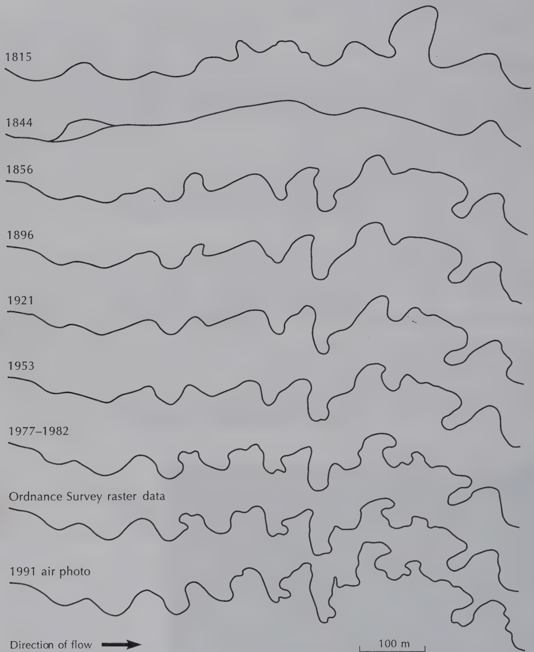
Figure 7.19 Channel change in Swinhope Burn, upper Weardale, northern Pennines, England. The diagram shows the channel centre-line determined from maps, plans, and an air photograph.
