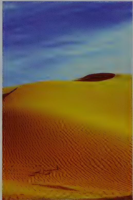
Colour Plate 15 Rippled linear dune flank in the northern Namib Sand Sea.
