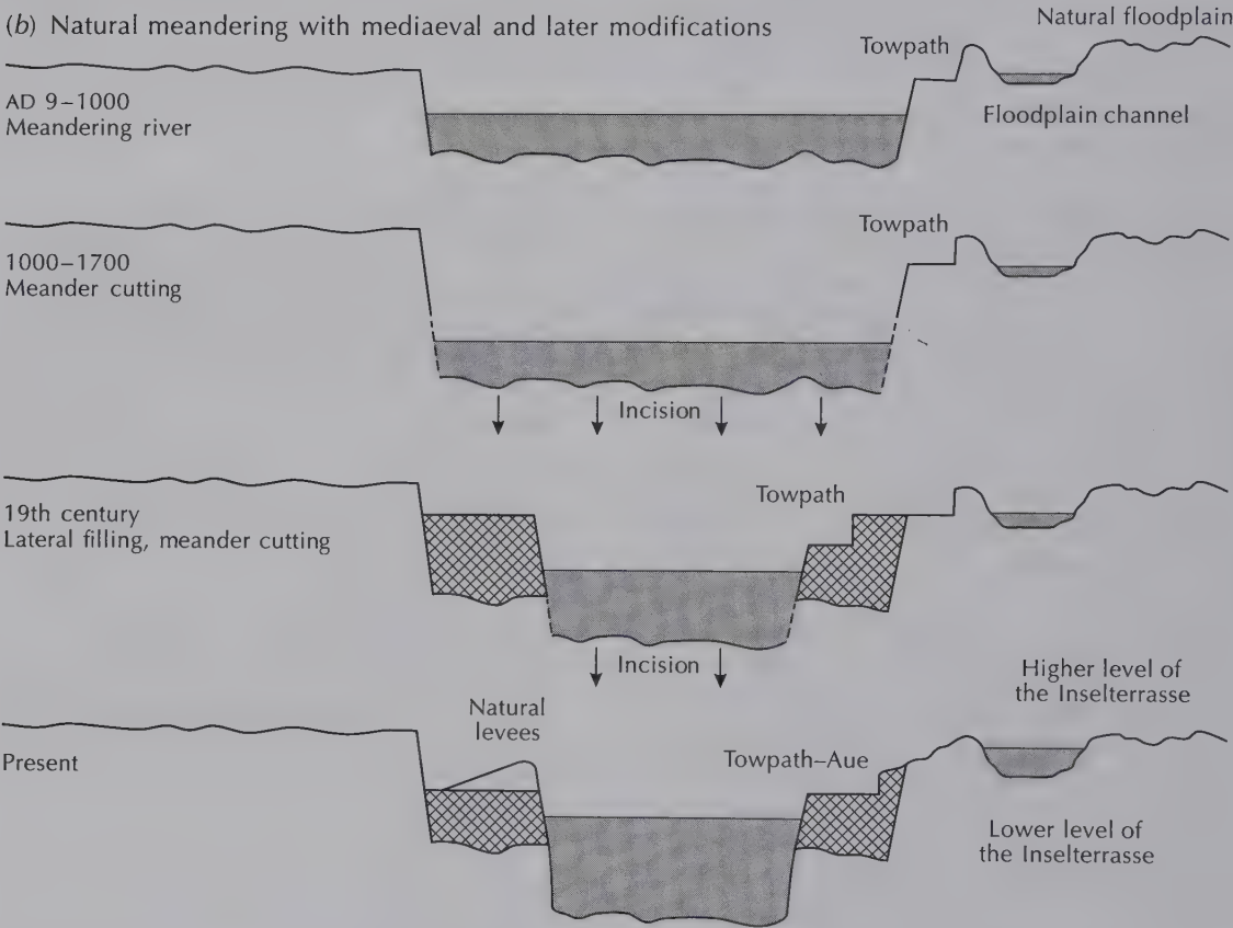
Figure 7.21 Evolution of Holocene terraces in the Lippe Valley. (a) Interpretation 1. (b) Interpretation 2. Source: Adapted from Herget (1998)
