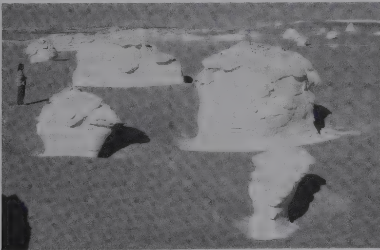
Plate 10.3 Zeugen , Farafra, Western Desert, Egypt. The limestone pillars are undercut by sandblasting. (Photograph by Tony Waltham Geophotos)
