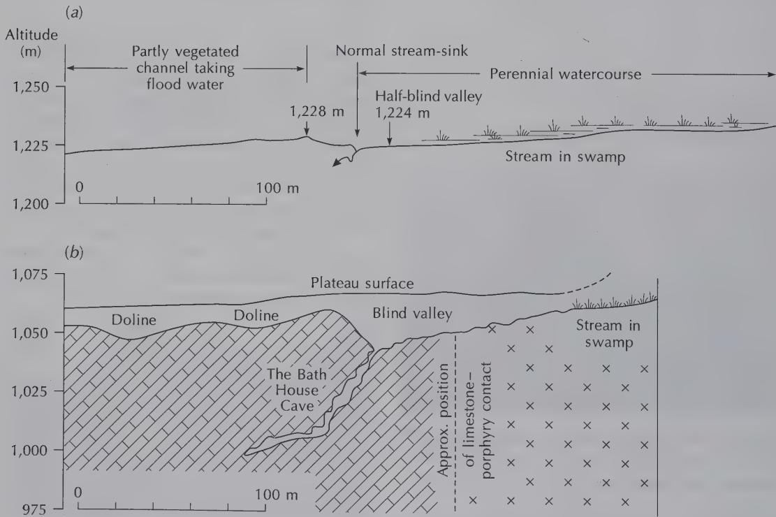
Figure 6.11 Blind and half-blind valleys in New South Wales, Australia. (a) A half-blind valley on Cooleman Plain. (b) A blind valley at Yarrangobilly.
