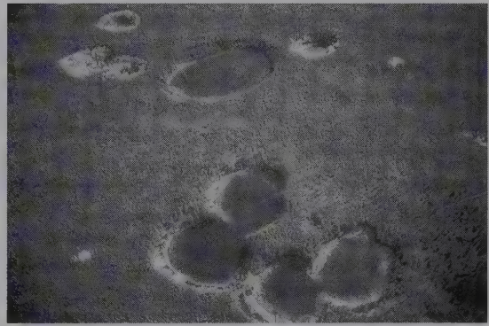
Plate 6.10 Collapse dolines at the water table, Wood Buffalo National Park, Alberta, Canada. The dolines are created by collapses through dolostone into underlying gypsum. The diameters are 40–100 m. (Photograph from Parks Canada archives)
