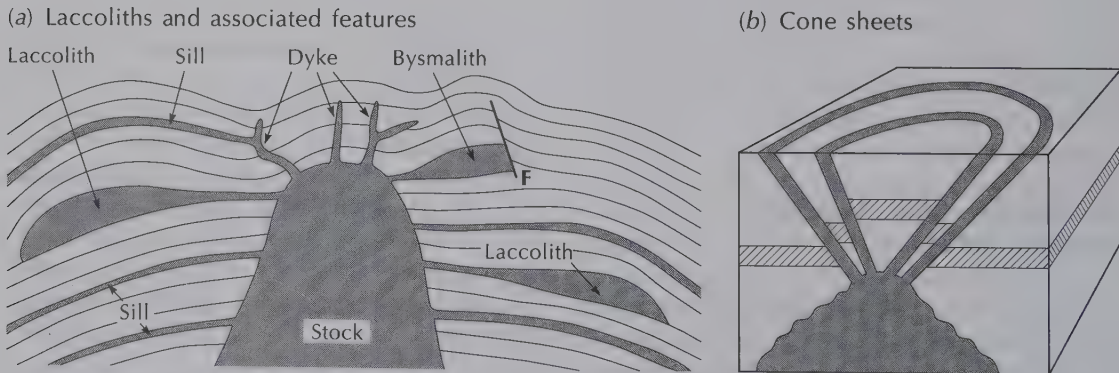
Figure 3.13 Minor intrusions. (a) Laccoliths and associated features (dykes, sills, and bysmaliths). (b) Cone sheets.
