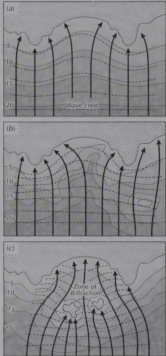
Figure 11.2 Wave refraction approaching headlands and bays above differing offshore topography.
