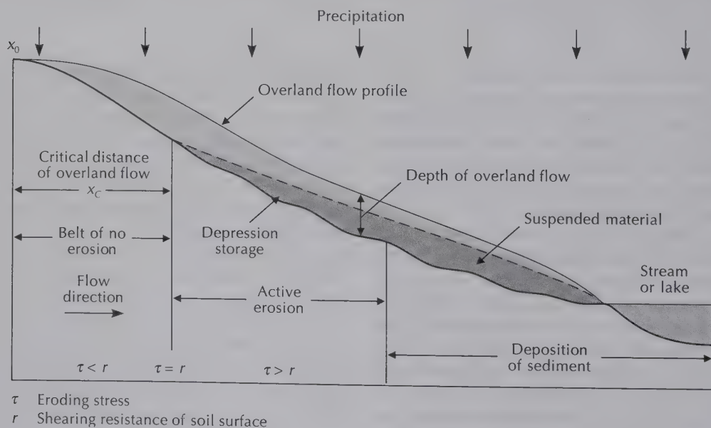
Figure 7.5 Horton's model of overland flow production.
