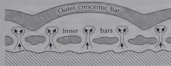
Figure 11.9 Cusps and crescentic bars.
