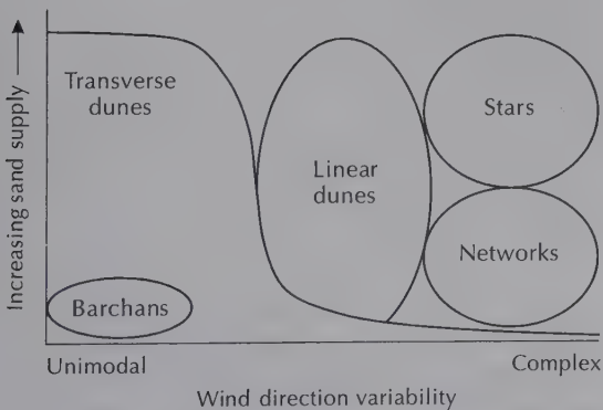
Figure 10.6 Dune types in relation to the variability of wind direction and sand supply.
