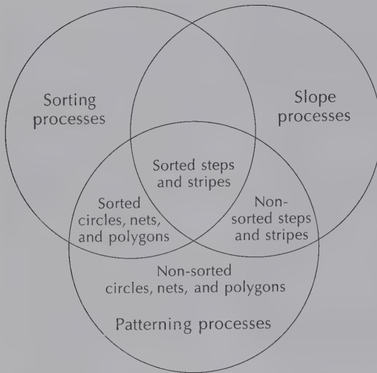
Figure 9.5 Relationships between patterned ground and sorting processes, slope processes, and patterning processes.
