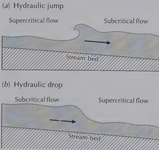
Figure 7.3 (a) Hydraulic jump. (b) Hydraulic drop.
