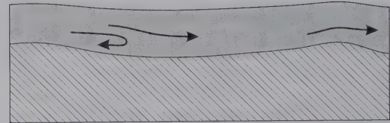
(f) Standing wave antidunes ( F \geq 1 )
