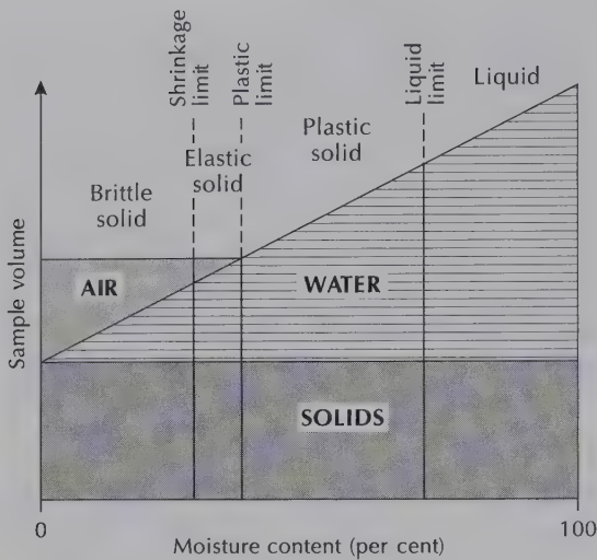
Figure 2.5 The composition of soil, ranging from air-filled pores, to water-filled pores, to a liquid. The Atterberg or soil limits are shown. Source: Adapted from Selby (1982, 76)
