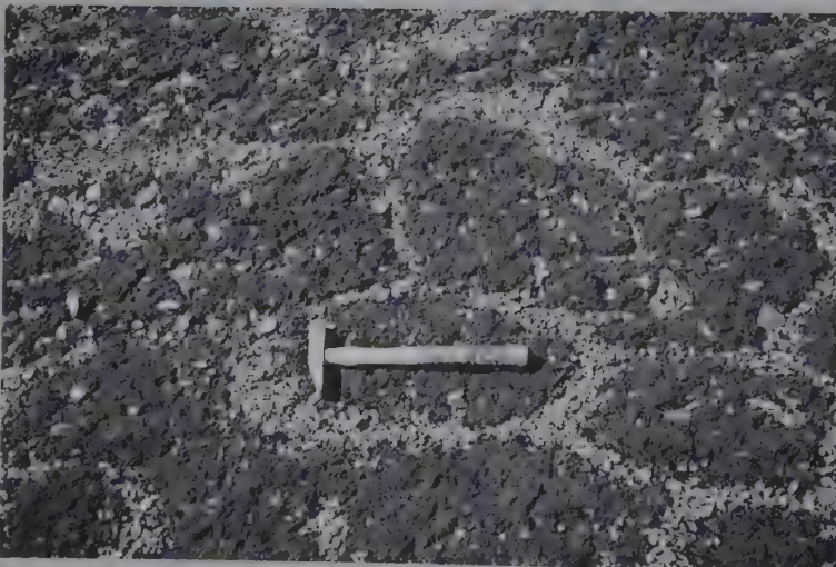
Plate 9.2 (a) Sorted polygons and (b) sorted stone stripes, Svartisen, northern Norway. The polygons and the stripes are found at the same site, the polygons on a very gently sloping area and the stripes on the steeper slope below. (Photographs by Wilfred H. Theakstone)
