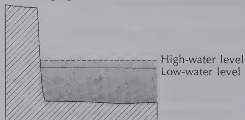
Figure 11.6 Three major forms on rocky coasts: shore platforms and plunging cliffs.
