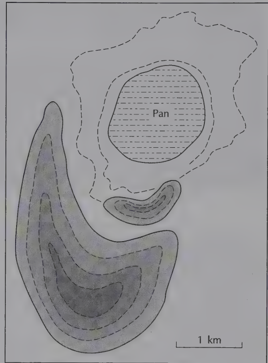
Figure 10.4 A pan and lunette in southern Africa.
