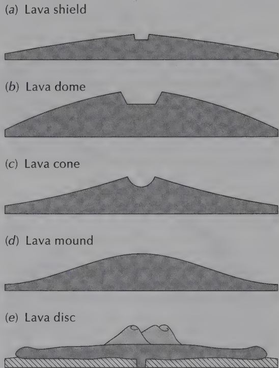
Figure 3.17 Types of basaltic volcano, not drawn to scale.
