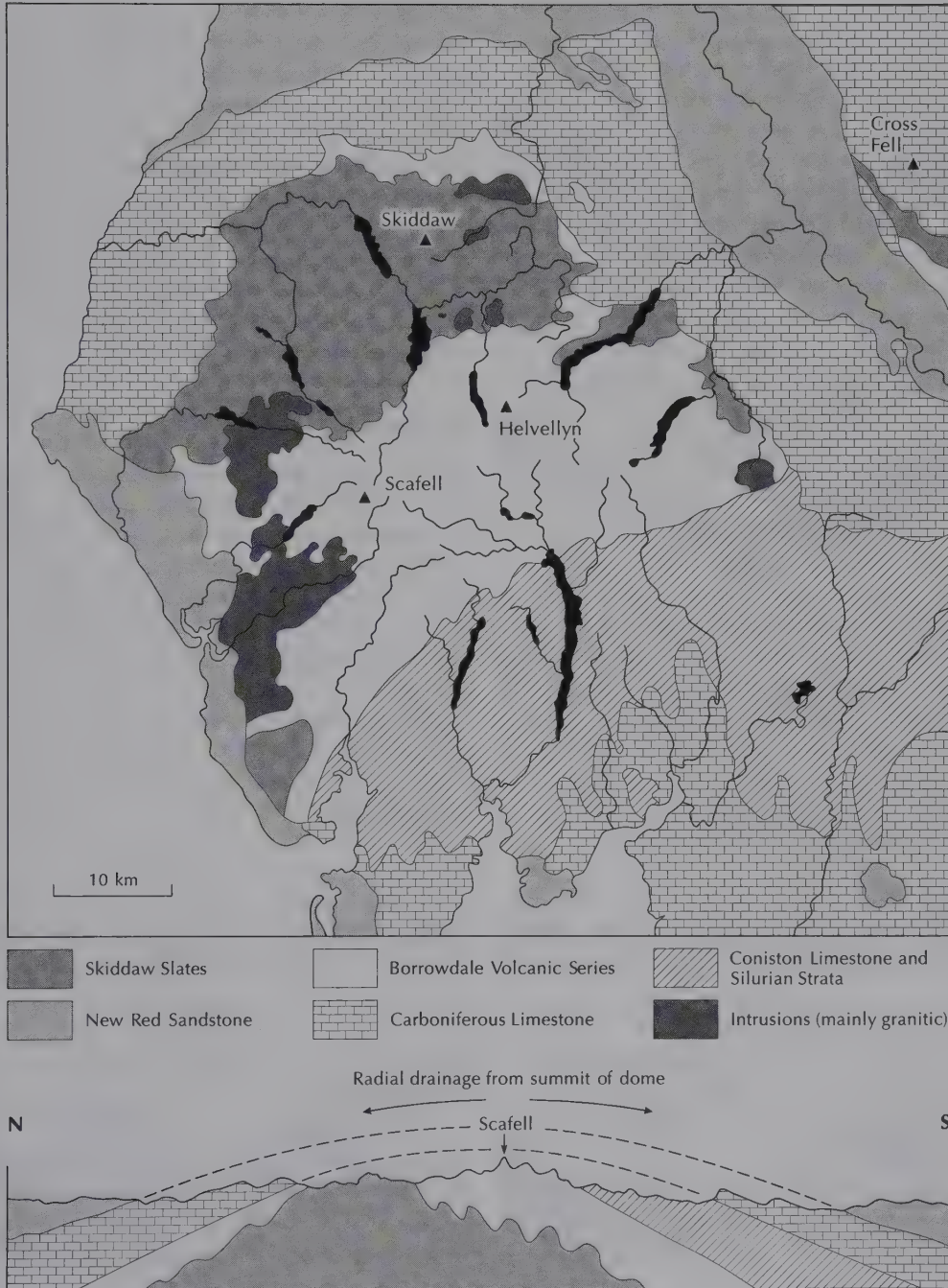
Figure 4.9 Superimposed drainage in the English Lake District. Source: Adapted from Holmes 1965, 564)
