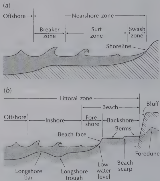
Figure 11.8 Terminology used to describe (a) wave and current processes in the nearshore, and (b) the beach profile. Source: Adapted from Komar (1998, 46)
