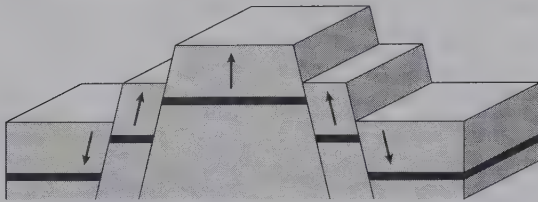
Figure 4.13 Up-faulted structures. (a) Horst. (b) Tilted block.
