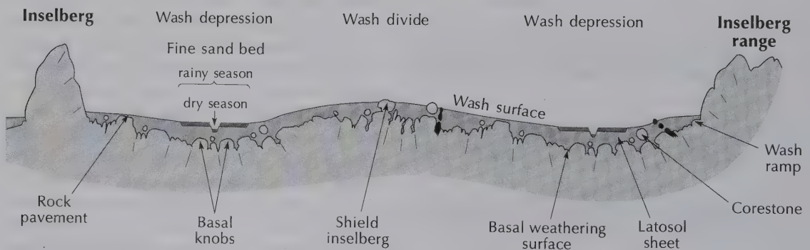
Figure 12.2 Double planation surfaces: the wash surface and the basal weathering surface. Source: Adapted from Büdel (1982, 126)
