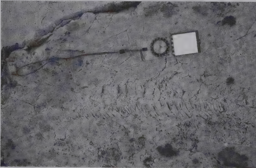
Plate 8.10 Chattermarks on Cambrian quartzite, An Teallach, north-west Highlands, Scotland. (Photograph by Mike Hambrey)
