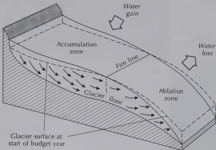
Figure 8.1 Glacier mass balance: schematic changes in the geometry of a glacier during an equilibrium budget year.
