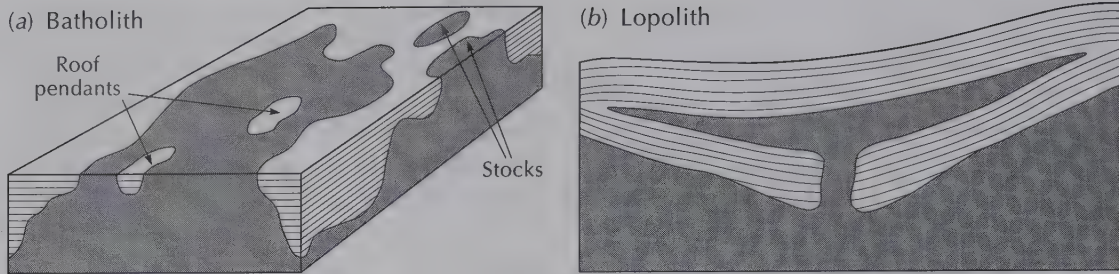
Figure 3.12 Major intrusions. (a) Batholith with stocks and roof pendants. (b) Lopolith.
