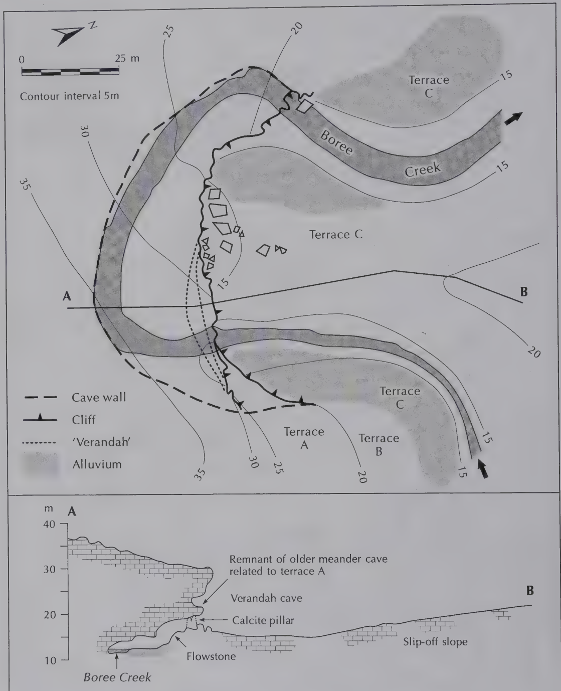
Figure 6.14 A meander cave on Boree Creek, Borenore, New South Wales, Australia.
