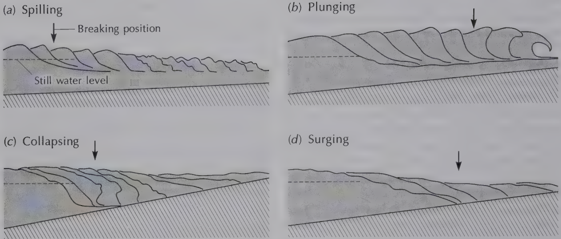
Figure 11.3 Kinds of breaking waves derived from high-speed moving pictures.
