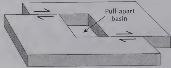
(a) Transtension
