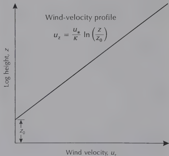
Figure 10.2 Wind-velocity profile
