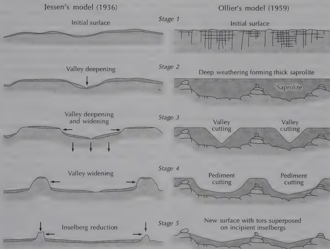
Figure 12.3 Theories of etchplanation. Source: Adapted from Jessen (1936) and Ollier (1959)
