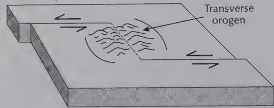
Figure 3.10 Landforms associated with oblique-slip faults. (a) Pull-apart basin formed by transtension. (b) Transverse orogen formed by transpression.
