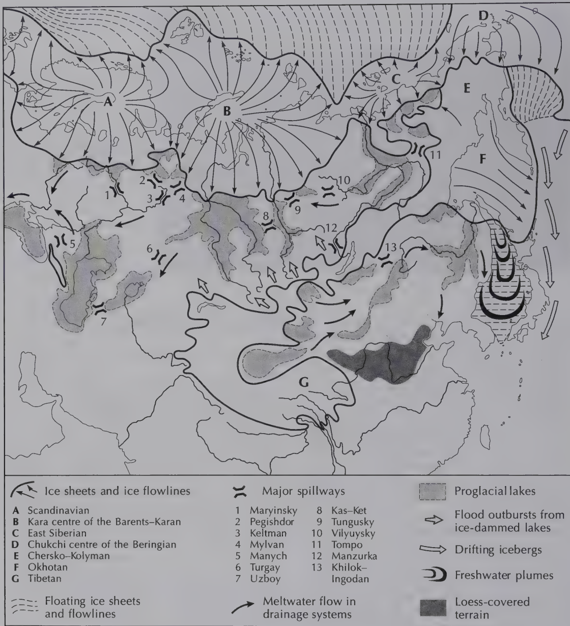
Figure 8.6 Glacial spillways in northern Eurasia. Source: Adapted from Grosswald (1998)
