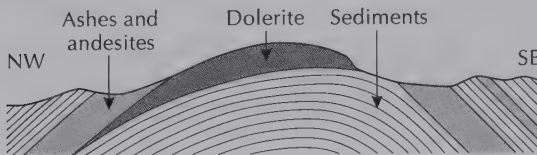
Figure 3.14 Phacoliths. (a) Occurrence in anticlinal crests and synclinal troughs. (b) Corndon Hill, near Montgomery in Wales, an eroded phacolith.
