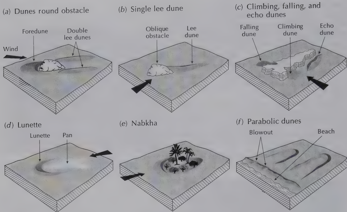
Figure 10.9 Types of anchored dune.
