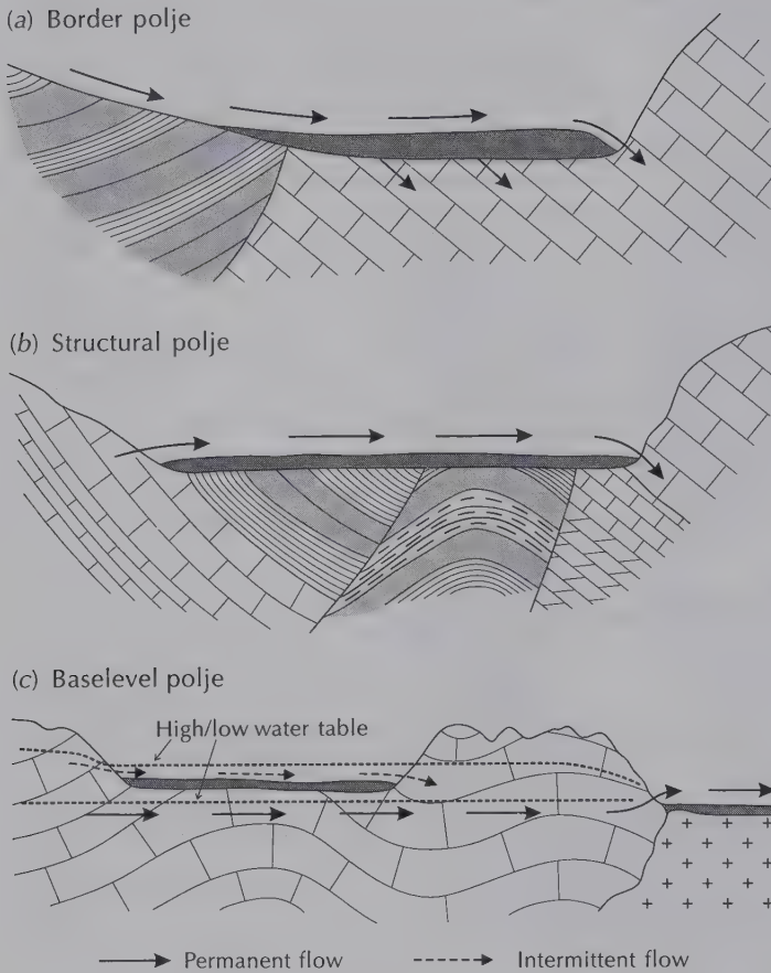
Figure 6.9 Types of polje. (a) Border polje. (b) Structural polje. (c) Baselevel polje. Source: After Ford and Williams (1989, 429)
