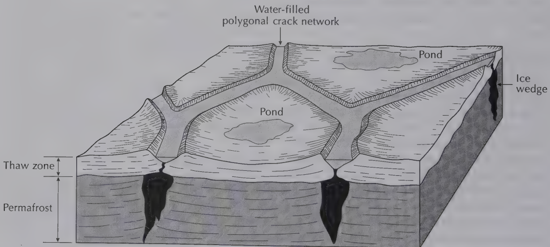
Figure 9.3 Ice wedges, ice-wedge polygons, and raised rims. Source: After Butzer (1976, 342)
