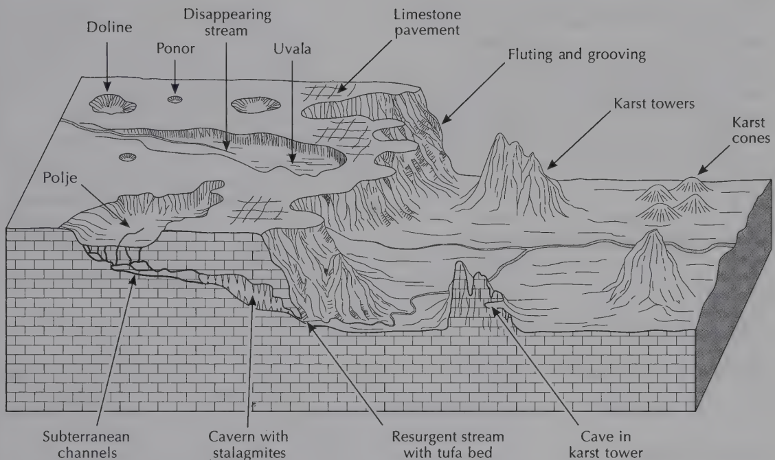
Figure 6.5 Schematic diagram of some karst features.
