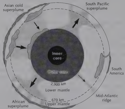
Figure 3.5 A possible grand circulation of Earth materials. Oceanic lithosphere, created at mid-ocean ridges, is subducted into the deeper mantle. It stagnates at around 670 km and accumulates for 100–400 million years. Eventually, gravitational collapse forms a cold downwelling onto the outer core, as in the Asian cold superplume, which leads to mantle upwelling occurring elsewhere, as in the South Pacific and African hot superplumes.
