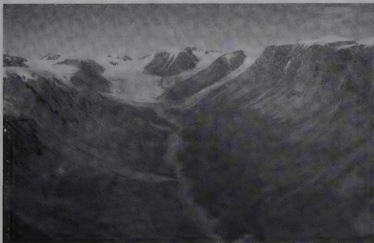
Plate 8.5 Glacial trough with valley glaciers at head, east Greenland. (Photograph by Mike Hambrey)
