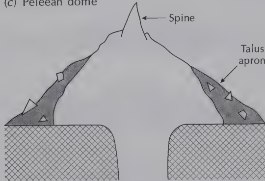
Figure 3.18 Lava domes. (a) Cumulo-dome. (b) Coulée. (c) Peléean dome. (d) Upheaved plug. Not drawn to scale. Source: Adapted from Blake (1989)
