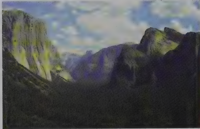
Colour Plate 12 Glacial trough with a hanging valley to the right, Yosemite, California, USA.
