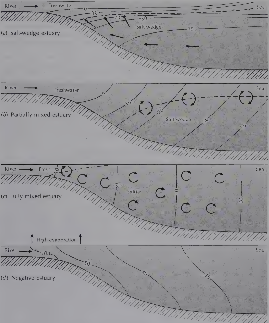
Figure 11.18 Types of estuary: a classification based on freshwater-seawater mixing.
