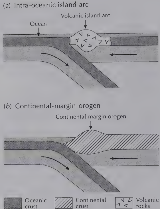
Figure 3.8 The two kinds of steady-state margin.
