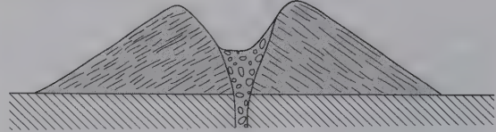
(a) Scoria cone
