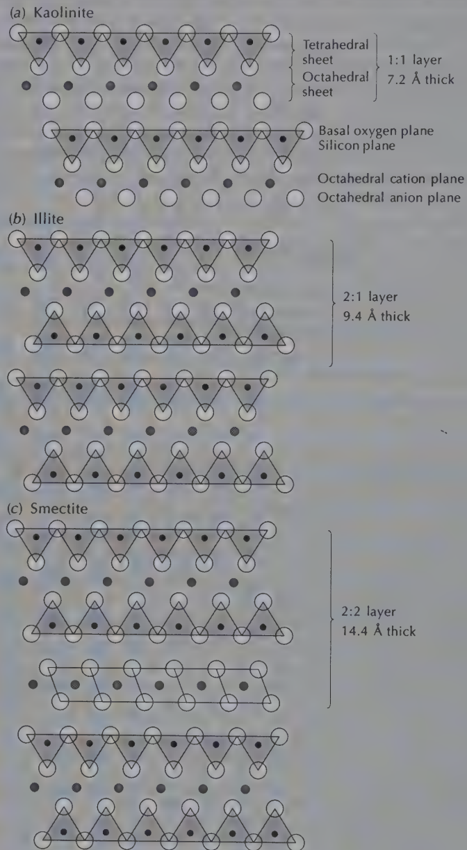
Figure 5.1 Clay mineral structure. (a) Kaolinite, a 1:1 dioctahedral layer silicate. (b) Illite, a 2:1 layer silicate, consisting of one octahedral sheet with two flanking tetrahedral sheets. (c) Smectite, a 2:2 layer silicate, consisting of 2:1 layers with octahedral sheets between. Å stands for an angstrom, a unit of length ( 1 \text{ \AA} = 10^{-8} \text{ cm} ).
