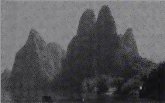
Plate 6.12 Tower karst on the south bank of the Li River near Guilin, Guangxi province, China. (Photograph by Derek C. Ford)
