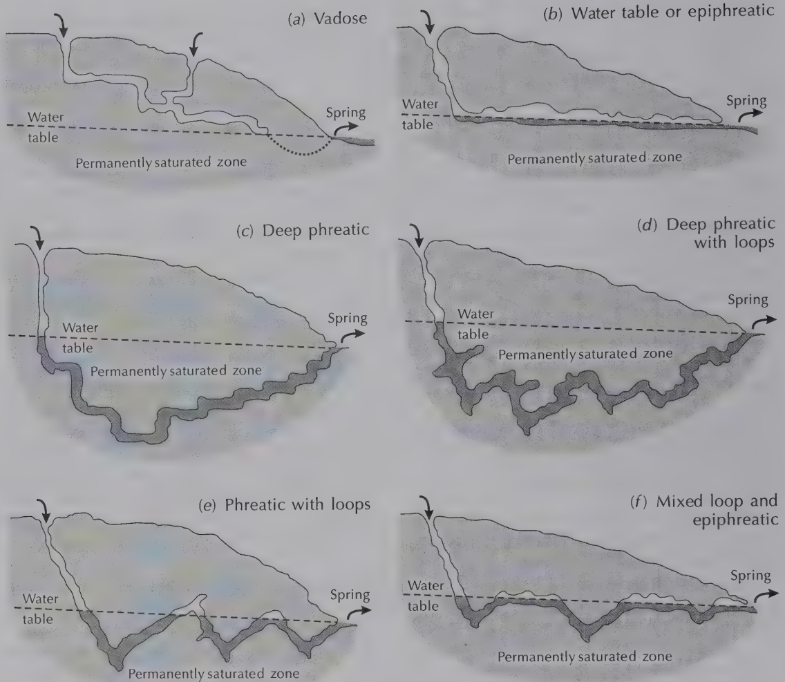
Figure 6.18 Types of caves.
