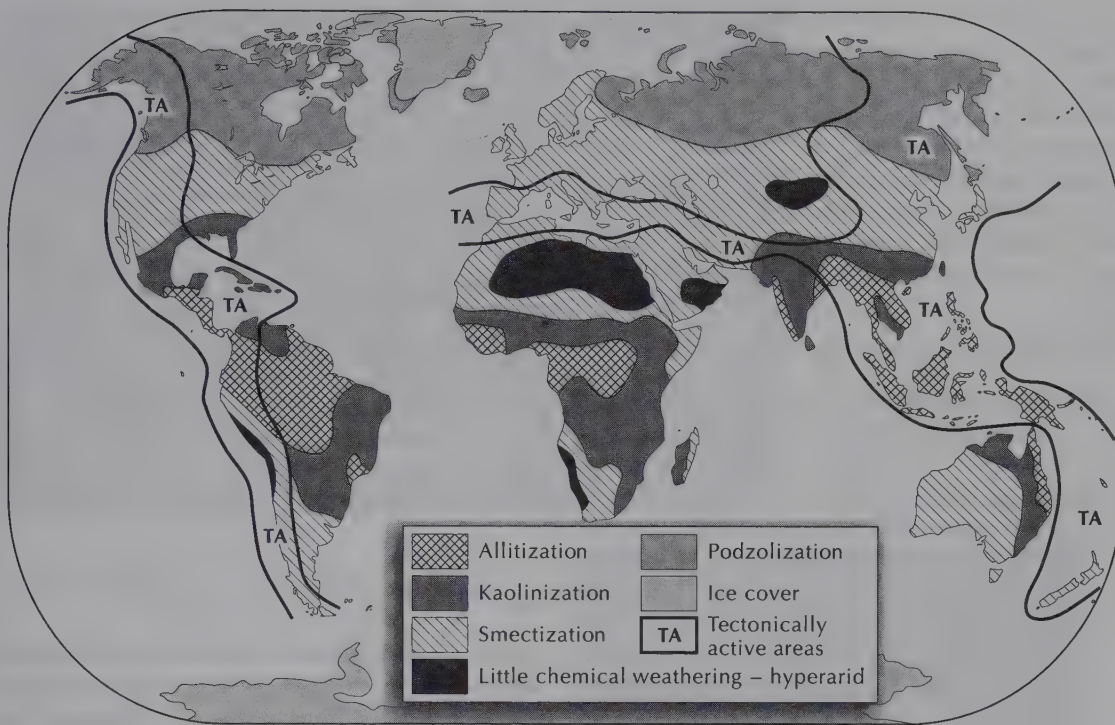
Figure 5.5 The main weathering zones of the Earth. Source: Adapted from Thomas (1994, 5)
