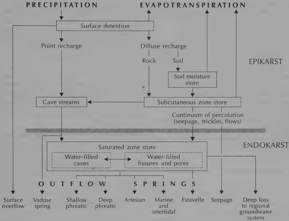
Figure 6.4 The karst drainage system: storages and flows. Source: Adapted from Ford and Williams (1989, 169)
