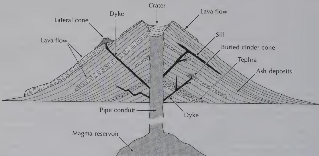
Figure 3.16 The structure of a typical strato-volcano. Source: Adapted from MacDonald (1972, 23)
