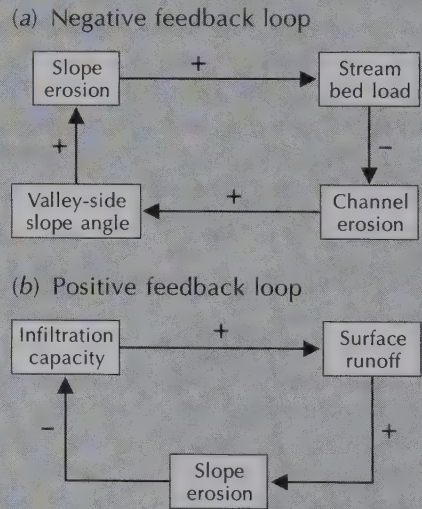
Figure 1.8 Feedback relationships in geomorphic systems. (a) Negative feedback in a valley-side slope-stream system. (b) Positive feedback in an eroding hillslope system. Details of the relationships are given in the text.
