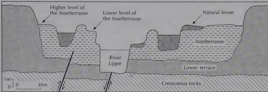
Figure 7.20 Schematic cross-section of the lower Lippe Valley in north-west Germany, showing terraces.
