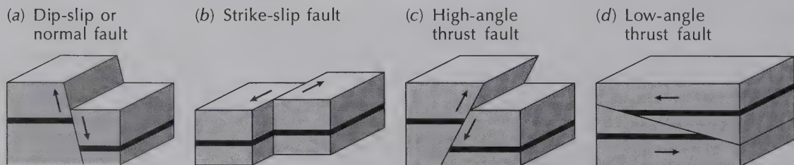
Figure 4.11 Faulted structures. (a) Normal fault. (b) Strike-slip fault. (c) High-angle reverse or thrust fault. (d) Low-angle thrust fault.
