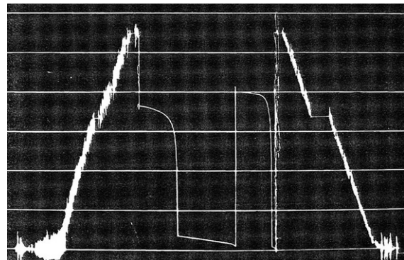
Fig. 4.18 Initial rapid built up pressure (Première remontée de pression surcharge)
