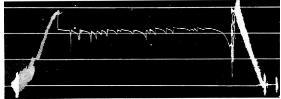
Fig. 4.35 Plugged formation through flow testing (Dèbit bouchè)
