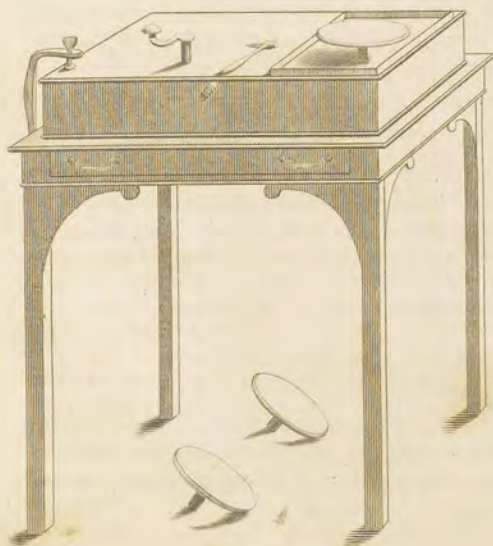
New invented Lapidaries apparatus for cutting & polishing Agates, &c.
