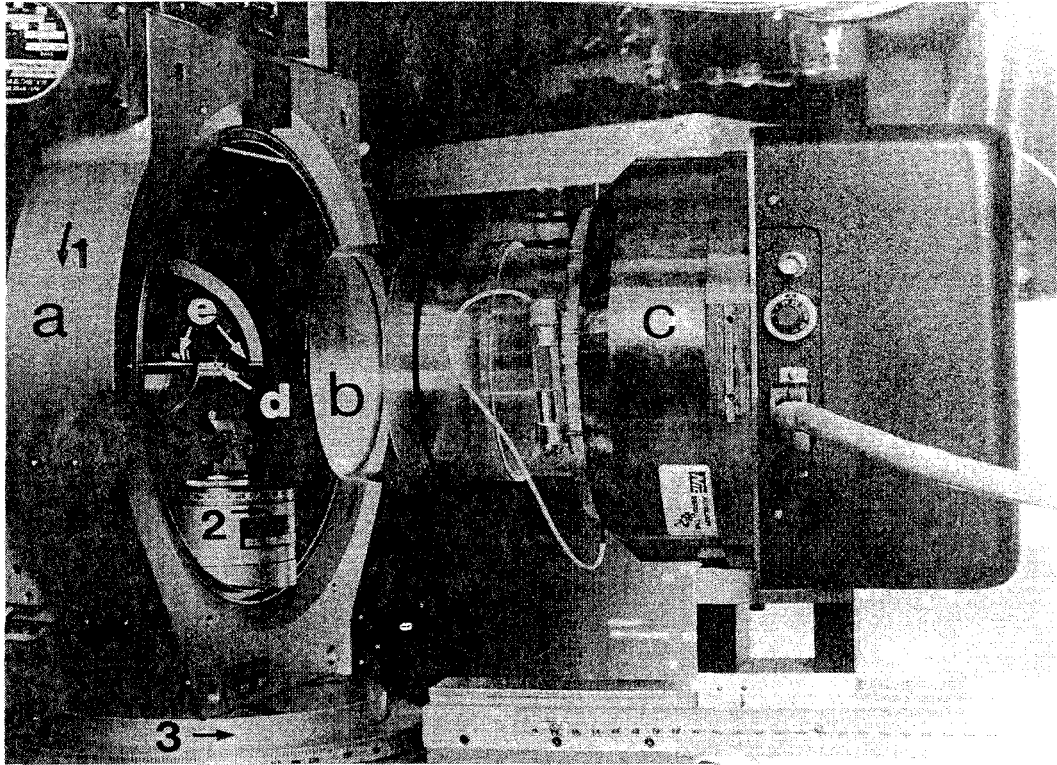
Figure 4.22 Diffractometer and area detector. Photo courtesy of Professor Leonard J. Banaszak.
