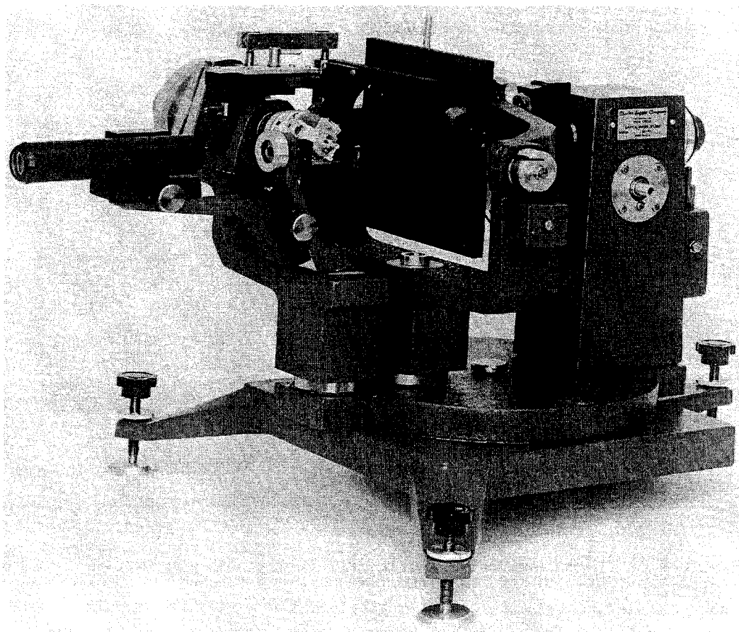
Figure 4.23 Precession camera with mounted goniometer head. To see a precession photograph, refer to Fig. 2.6. Photo courtesy of Charles Supper Company.
