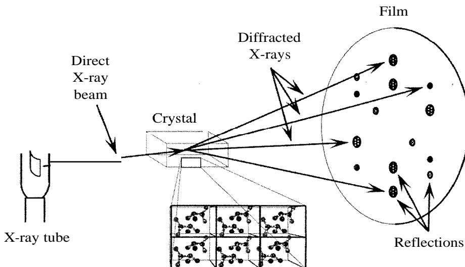
Figure 2.5 Crystallographic data collection. The crystal diffracts the source beam into many discrete beams, each of which produces a distinct spot (reflection) on the film. The positions and intensities of these reflections contain the information needed to determine molecular structures.
