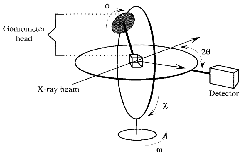
Figure 4.21 System of circles in diffractometry. The crystal in the center is mounted on a goniometer head.
