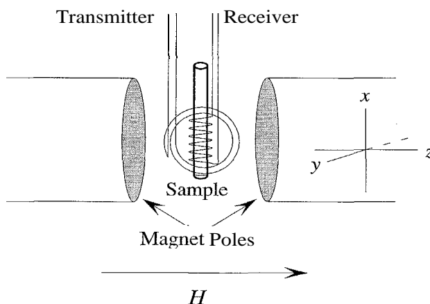
Figure 10.3 Diagram of an NMR experiment. The sample lies between the poles of a powerful magnet, and is spun rapidly around its long ( x ) axis in order to compensate for any unevenness (inhomogeneity) of the magnetic field. Radio frequency receiver coils form a helix around the x -axis, and transmitter coils spiral around the y -axis.
