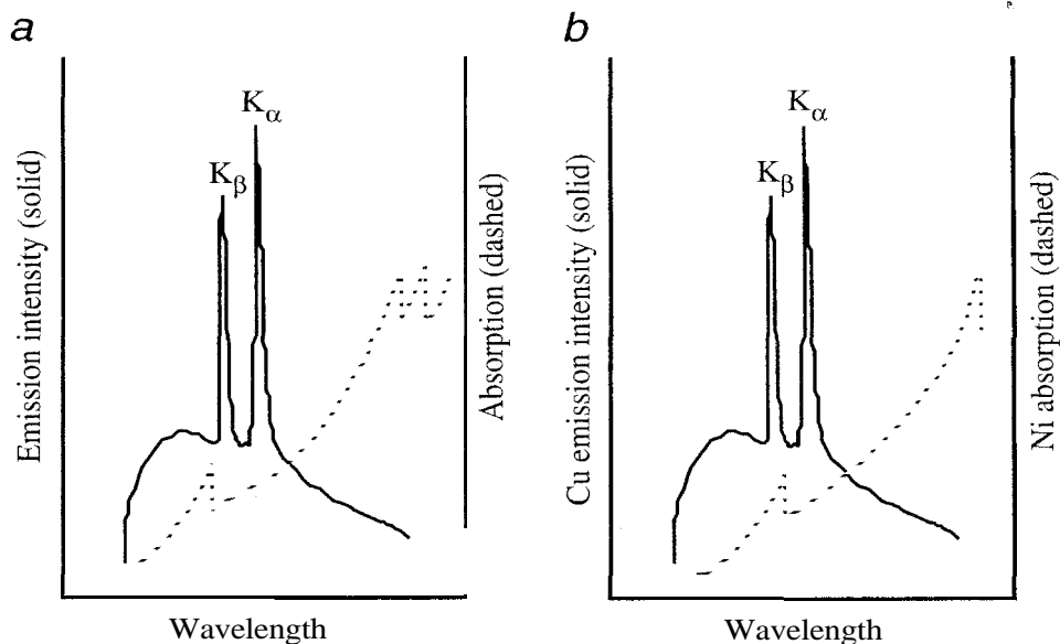
Figure 4.16 (a) Emission (solid) and absorption (dashed) spectra of copper. (b) Emission spectrum of copper (solid) and absorption spectrum of nickel (dashed). Notice that Ni absorbs K_\beta more strongly than K_\alpha .
