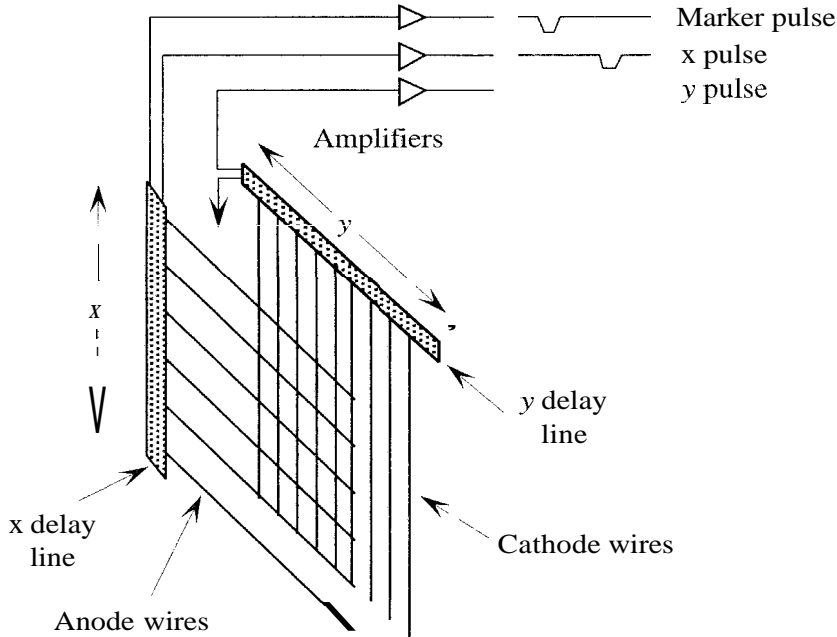
Figure 4.19 Exploded view of detector wires in multiwire area detector.
