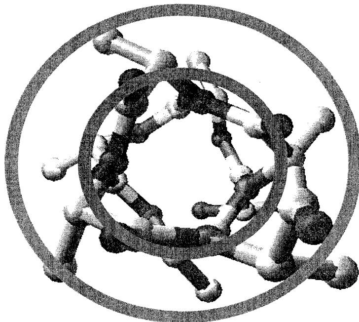
Figure 9.5 Polyaniline \alpha helix, viewed down the helix axis. An electron-density map averaged around this axis would merely show two circular peaks of electron density, one at the distance of the backbone atoms (inner circle) and another at the distance of the alpha carbons (outer circle).
