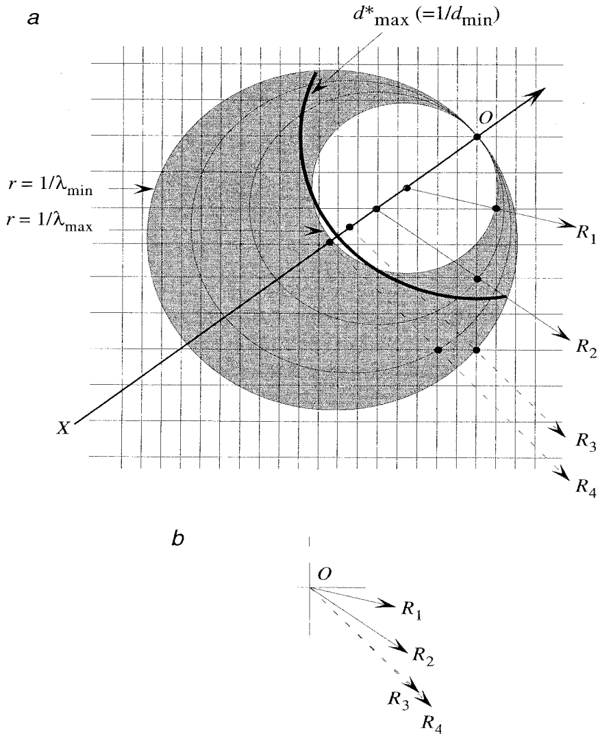
Figure 9.7 Geometric construction for Laue diffraction in reciprocal space.
