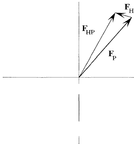
Figure 6.6 A structure factor \mathbf{F}_{\text{HP}} for the heavy-atom derivative is the sum of contributions from the native structure ( \mathbf{F}_{\text{P}} ) and the heavy atom ( \mathbf{F}_{\text{H}} ).
