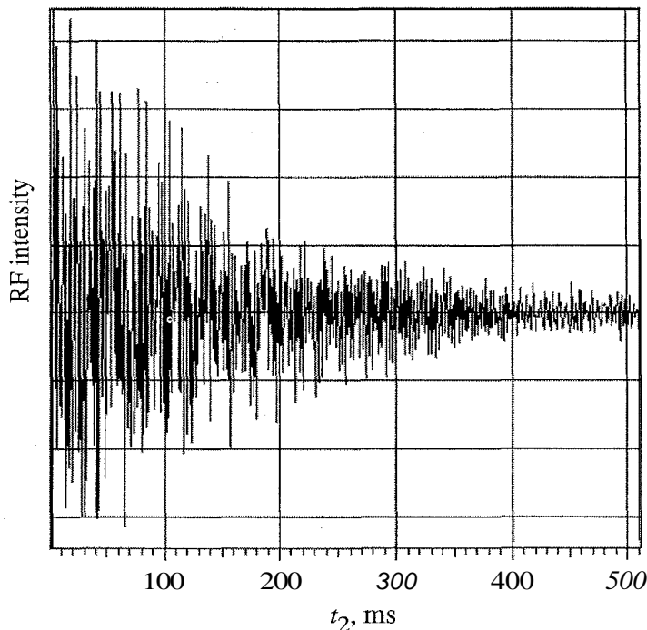
Figure 10.4 Free induction decay signal, which appears in the receiver coils after a 90^\circ pulse. The FID is a time-domain spectrum, showing RF intensity as a function of time t_2 . It is a composite of the RF absorption frequencies of all nuclei in the sample. The Fourier transform decomposes an FID into its component frequencies, giving a spectrum like that shown in Fig. 10.1. Figure generously provided by Professor John M. Louis.
