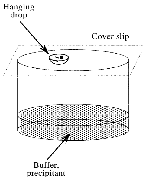
Figure 3.2 Growing crystals by the hanging-drop method. The droplet hanging under the cover slip contains buffer, precipitant, protein, and, if all goes well, growing protein crystals.
