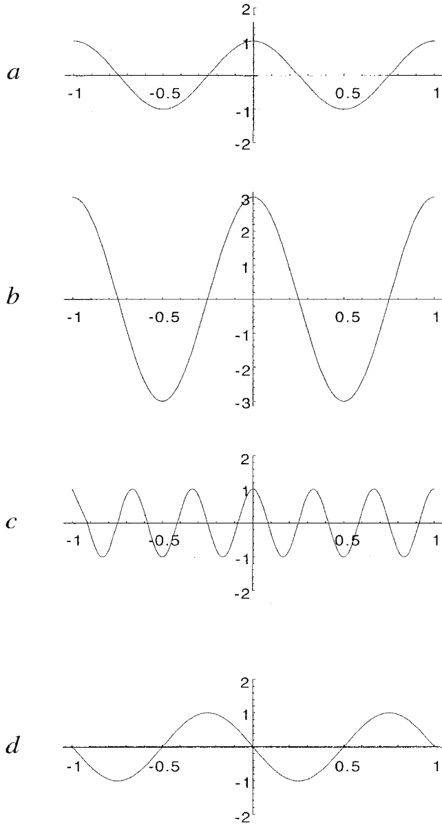
Figure 2.13 Graphs of four simple wave equations f(x) = F \cos 2\pi(hx + a) . (a) F = 1, h = 1, \alpha = 0 : f(x) = \cos 2\pi(x) . (b) F = 3, h = 1, \alpha = 0 : f(x) = 3 \cos 2\pi(x) . Increasing F increases the amplitude of the wave. (c) F = 1, h = 3, \alpha = 0 : f(x) = \cos 2\pi(3x) . Increasing h increases the frequency (or decreases the wavelength \lambda ) of the wave. (d) F = 1, h = 1, \alpha = 1/4 : f(x) = \cos 2\pi(x + 1/4) . Changing \alpha changes the phase (position) of the wave.
