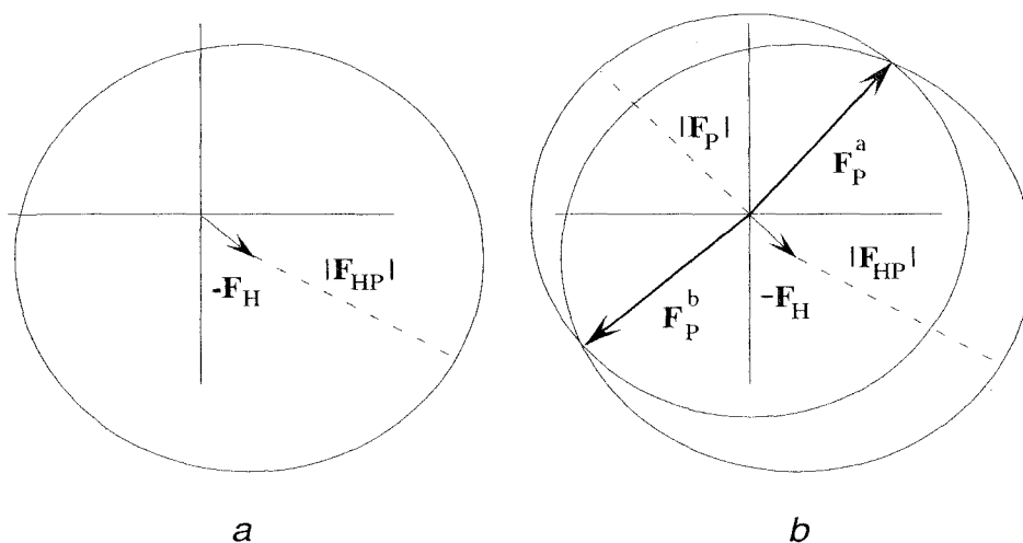
Figure 6.7 Vector solution of Equation (6.9). (a) All points on the circle equal the vector sum |\mathbf{F}_{HP}| - \mathbf{F}_H . (b) Vectors from the origin to intersections of the two circles are solutions to Eq. (6.9).
