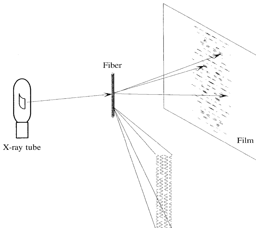
Figure 9.1 Fiber diffraction. Molecules in the fiber are oriented parallel to the beam axis but aligned at random. X-ray beams emerging from the fiber strike the detector in layer lines perpendicular to the fiber axis.
