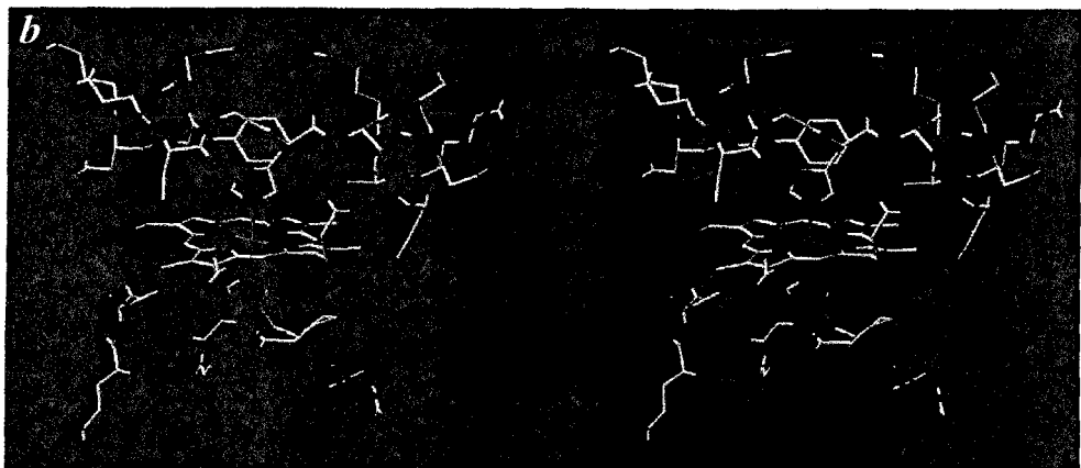
Plate 17 Heme region of cytochrome b5 (PDB 3b5c). (a) View without clipping; (b) same view after "slab" command to eliminate all except contents of a 12-Å slab in the z-direction. (For discussion, see Chapter 11.) Image: SPV/POV-Ray.
