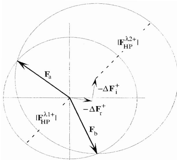
Figure 6.13 Vector solution of Eq. (5.13). \Delta \mathbf{F}_r and \Delta \mathbf{F}_i play the same role as \mathbf{F}_H in Figs. 6.7 and 6.8.
