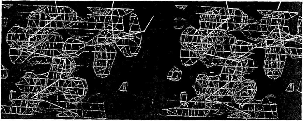
Plate 10 Alpha-carbon model of ALBP built into electron-density map. (For discussion, see Chapter 7.)
