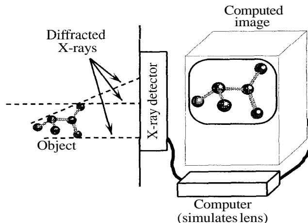
Figure 2.2 Crystallographic analogy of lens action. X-rays diffracted from the object are received and measured by a detector. The measurements are fed to a computer, which simulates the action of a lens to produce a graphics image of the object.
