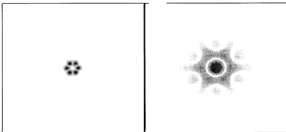
Figure 2.9 A planar hexagon of spheres (left) and its diffraction pattern (right).
