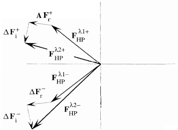
Figure 6.12 Under anomalous scattering, \mathbf{F}_{-h-k-l} is no longer the mirror image of \mathbf{F}_{hkl} .
