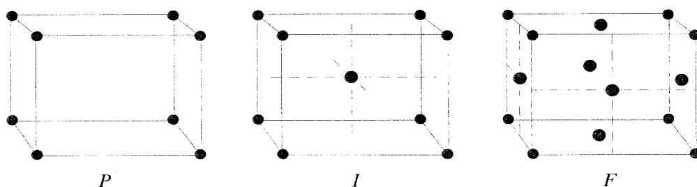
Figure 4.13 P , I , and F unit cells.
