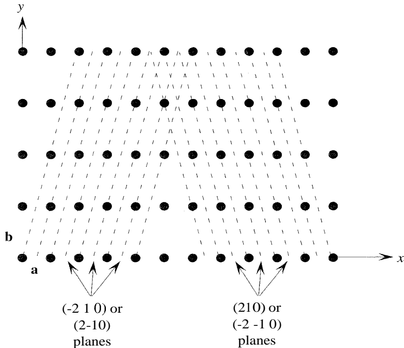
Figure 4.6 The (210) and (-2\ -1\ 0) planes are identical. The (210) planes tilt in the opposite direction from (2\ -1\ 0) and (-2\ 1\ 0) planes.
