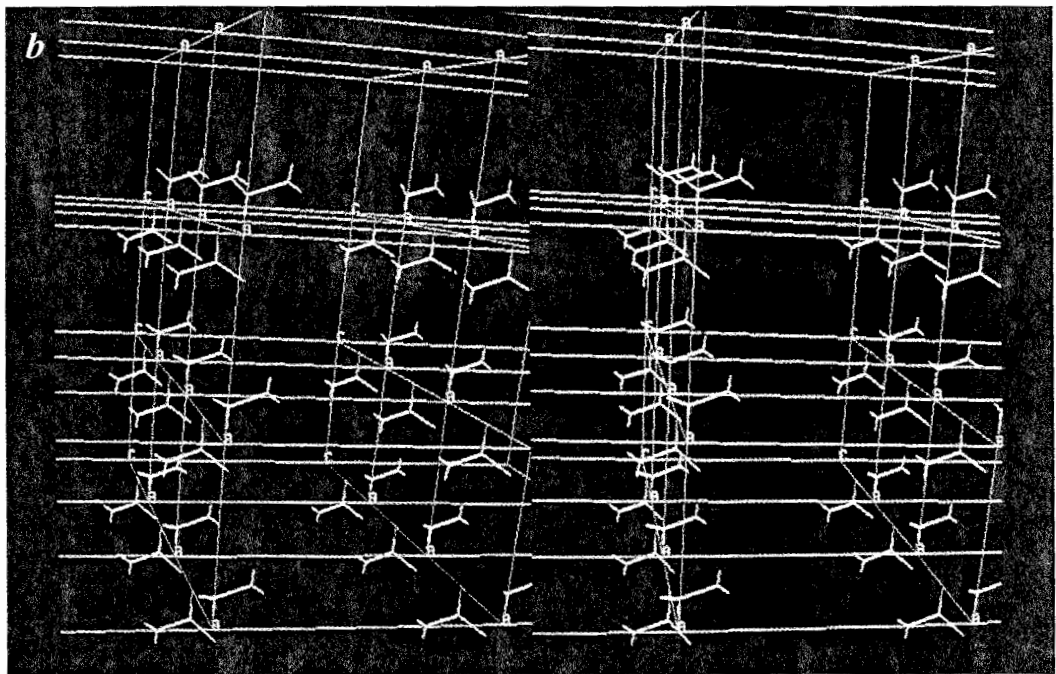
Plate 7 Alanine in hypothetical (a) P1 and (b) P2_1 unit cells. (For discussion, see Chapter 4.)
