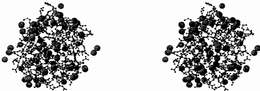
Plate 4 One molecule of crystalline adipocyte lipid-binding protein (ALBP, PDB 1alb), showing ordered water molecules on the surface and within a molecular cavity where lipids are usually bound. Protein is shown as a ball-and-stick model with carbon dark gray, oxygen red, and nitrogen blue. Ordered water molecules, displayed as space-filling oxygen atoms, are green. (For discussion, see Chapter 3.). Image: SPV/POV-Ray.
