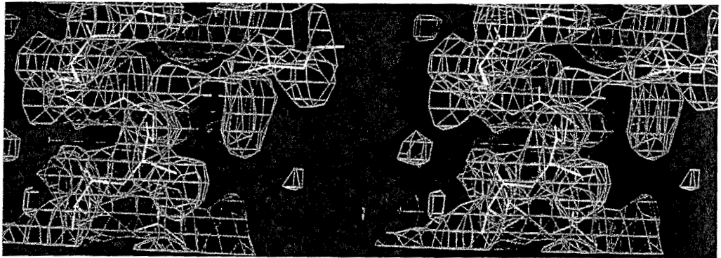
Plate 11 Polyalanine model of ALBP built into electron-density map. This section of the final ALBP model is shown in Plate 2. (For discussion, see Chapter 7.)
