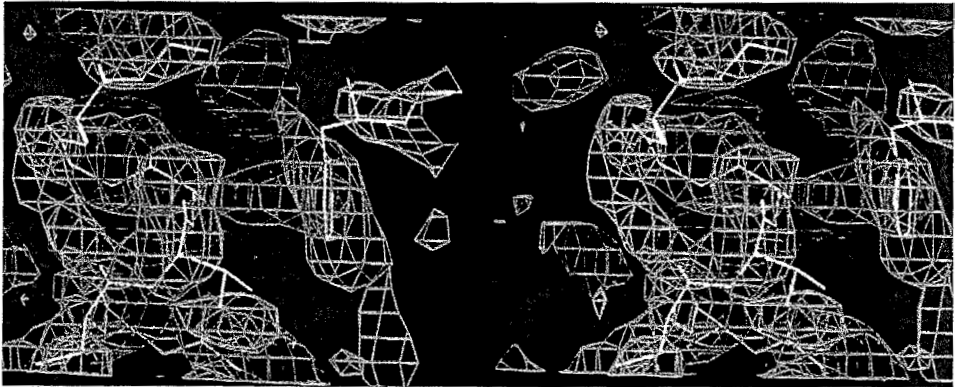
Plate 13 ALBP electron-density map calculated with molecular-replacement phases before any refinement, shown with the final model. Compare with Plate 2, which shows the final electron-density map in the same region. (For discussion, see Chapter 8.)
