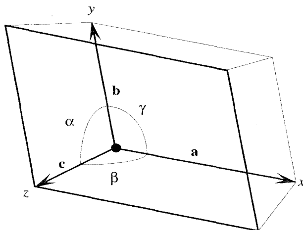
Figure 4.1 General (triclinic) unit cell, with edges a , b , c and angles \alpha , \beta , \gamma .
