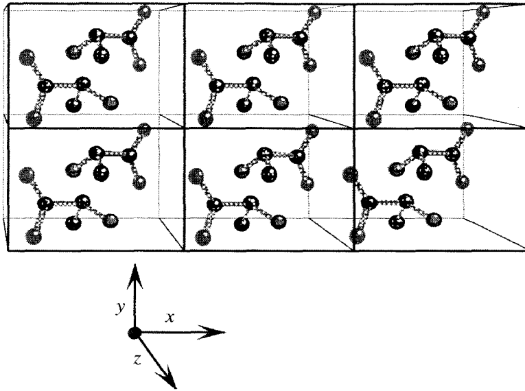
Figure 2.3 Six unit cells in a crystalline lattice. Each unit cell contains two molecules of alanine (hydrogen atoms not shown) in different orientations.
