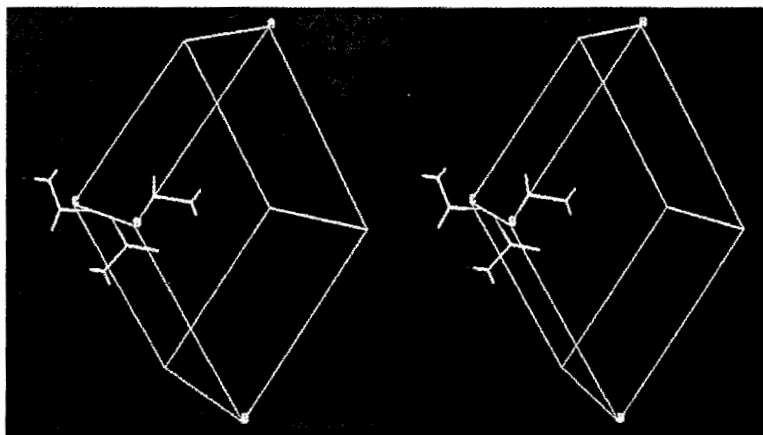
Plate 6 Threefold screw axis ( 3_1 ). (For discussion, see Chapter 4.)
