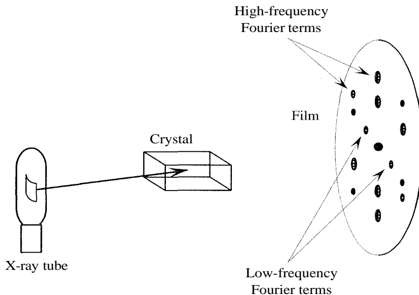
Figure 5.2 Structure factors of reflections near the center of the diffraction pattern are low-frequency terms in the Fourier series that approximates \rho(x,y,z) . Structure factors of reflections near the edge of the pattern are high-frequency terms.
