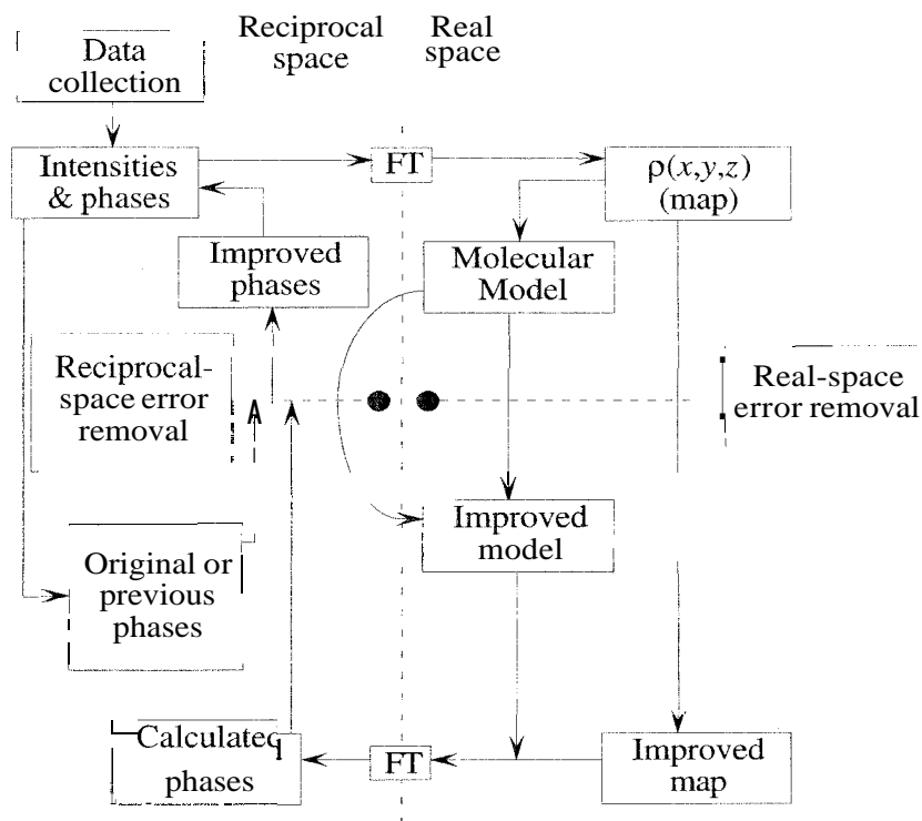
Figure 7.1 Block diagram of crystallographic structure determination.
