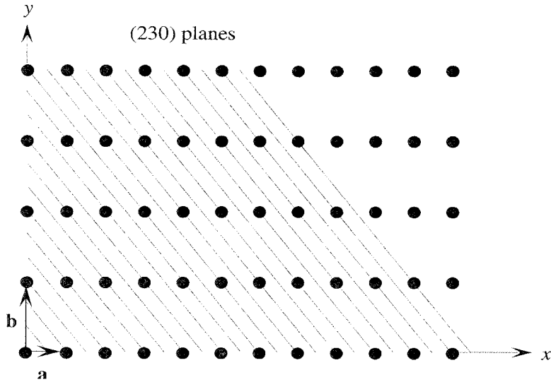
Figure 4.4 (230) planes in a two-dimensional section of lattice.
