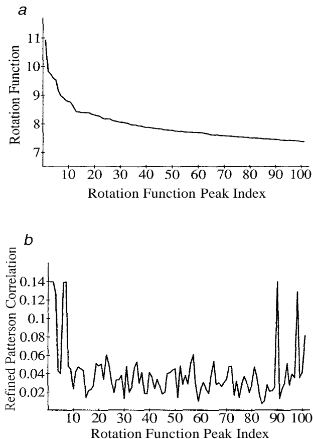
Figure 8.4 Rotation function results: P2 into crystalline ALBP. (a) Plot of the 101 best solutions to the rotation function, each peak numbered in the horizontal direction (abscissa). The correlation between the Patterson's of the probe molecule and the measured ALBP X-ray results are shown in the vertical direction (ordinate) and are given in arbitrary units. (b) Description of the rotation studies after Patterson correlation refinement. The peak numbers plotted in both panels (a) and (b) are the same. Reprinted with permission from Z. Xu et al. (1992) Biochemistry 31,3484–3492. Copyright 1992 American Chemical Society.
