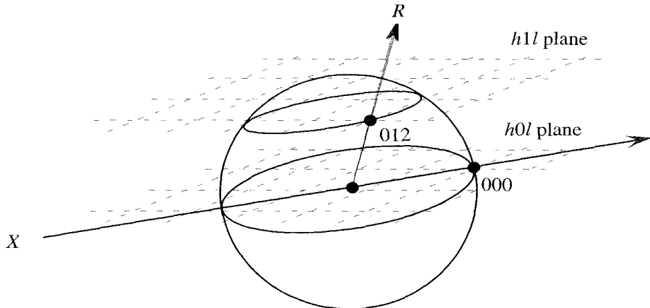
Figure 4.11 Sphere of reflection. When reciprocal lattice point 012 intersects the sphere, ray R emerges from the crystal as reflection 012.
