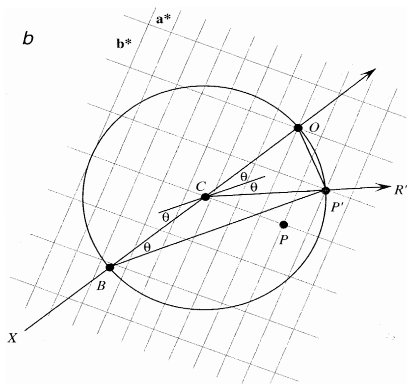
Figure 4.10 Diffraction in reciprocal space. (a) Ray R emerges from the crystal when reciprocal lattice point P intersects the circle. (b) As the crystal rotates, point P' intersects the circle, producing ray R' .
