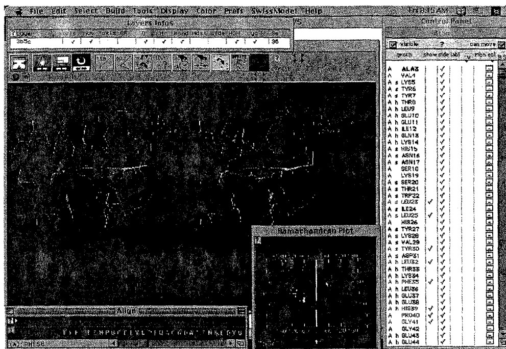
Plate 16 Screen shot of Swiss-PdbViewer in use on a Power Macintosh computer. Controls for manipulating the model are at the top of the main graphics window, which can be expanded to fill the screen. The Control Panel lists residues in the model and allows selection of residues for display, coloring, labeling, and surface displays. The Align window shows residue sequence also, including alignment of multiple models if present. The Ramachandran Plot window shows main-chain torsional angles for residues currently selected (purple in Align window and red in Control Panel). Dragging dots on the Rama plot changes torsion angles interactively. The Layers Infos window allows control of display features for multiple models in any combination. In the graphics window is a stereo display of the heme region of cytochrome b5 (PDB 3b5c). Selected hydrogen bonds are shown in green, and measured distances are shown in yellow. A torsion operation is in progress (dark button, top of graphic window). The side-chain conformation of phenylalanine-58 is being changed. Clashes between the side chain and other atoms are shown in pink. The user can read the PDB file of the currently active model by clicking the document icon at the upper right of the graphics window. Clicking a residue in the PDB file centers the graphics model on that residue. (For discussion, see Chapter 11.)
