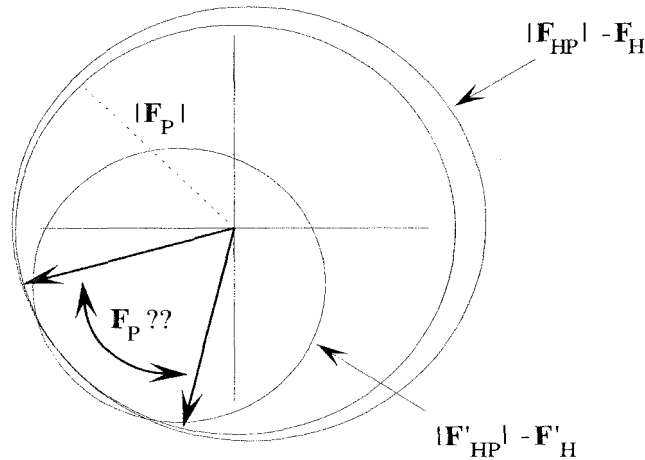
Figure 6.9 The MIR solution for this structure factor gives phase of high uncertainty.
