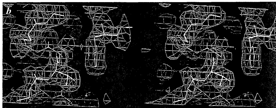
Plate 2 (a) Small section of molecular image displayed on computer graphics terminal. (b) Image (a) is interpreted by building a molecular model within the image. Computer graphics programs allow parts of the model to be added and their conformations adjusted to fit the image. The protein shown here is adipocyte lipid binding protein (ALBP, PDB 1alb). (For discussion, see Chapter 2.)
