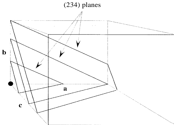
Figure 4.5 The intersection of three (234) planes with a unit cell. Note that the (234) planes cut the unit-cell edges a into two parts, b into three parts and c into four parts.
