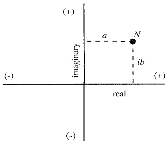
Figure 6.1 The complex number N = a + ib , represented as a point on the plane of complex numbers.
