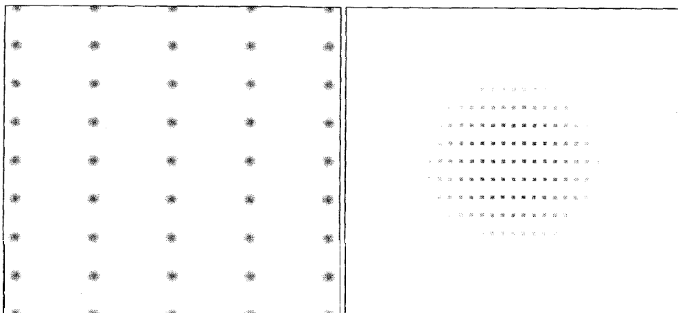
Figure 2.8 Lattice of spheres (left) and its diffraction pattern (right). If you look at the pattern and blur your eyes, you will see the diffraction pattern of a sphere. The pattern is that of the average sphere in the real lattice, but it is sampled at the reciprocal lattice points.
