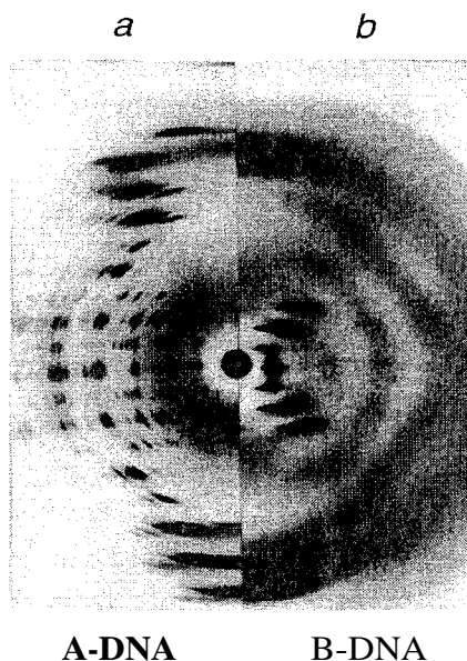
Figure 9.4 Fiber diffraction patterns from A-DNA (left half of figure) and B-DNA (right). A-DNA was microcrystalline and thus gave discrete, but overlapping, Bragg reflections. B-DNA was noncrystalline and thus gave continuous variation in intensity along each layer line. Image kindly provided by Professor Kenneth Holmes.
