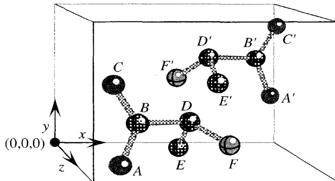
Figure 2.15 Every atom contributes to every reflection in the diffraction pattern, as described for this unit cell by Eq. (2.3).
