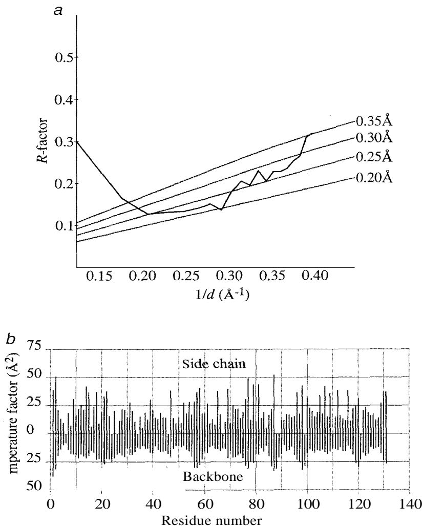
Figure 8.5 ALBP refinement results. (a) Theoretical estimates of the rms positional errors in atomic coordinates according to Luzzati (1952) are shown superimposed on the curve for the ALBP diffraction data. The coordinate error estimated from this plot is 0.25 \text{\AA} with an upper limit of about 0.35 \text{\AA} . (b) Mean values of the main-chain and side-chain temperature factors are plotted versus the residue number. The temperature factors are those obtained from the final refinement cycles. Reprinted with permission from Z. Xu et al. (1992) Biochemistry 31 , 3484–3492. Copyright 1992 American Chemical Society.
