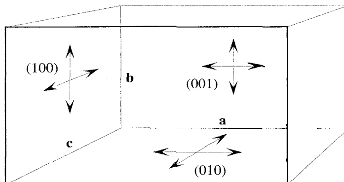
Figure 4.2 Indices of faces in an orthorhombic unit cell.
