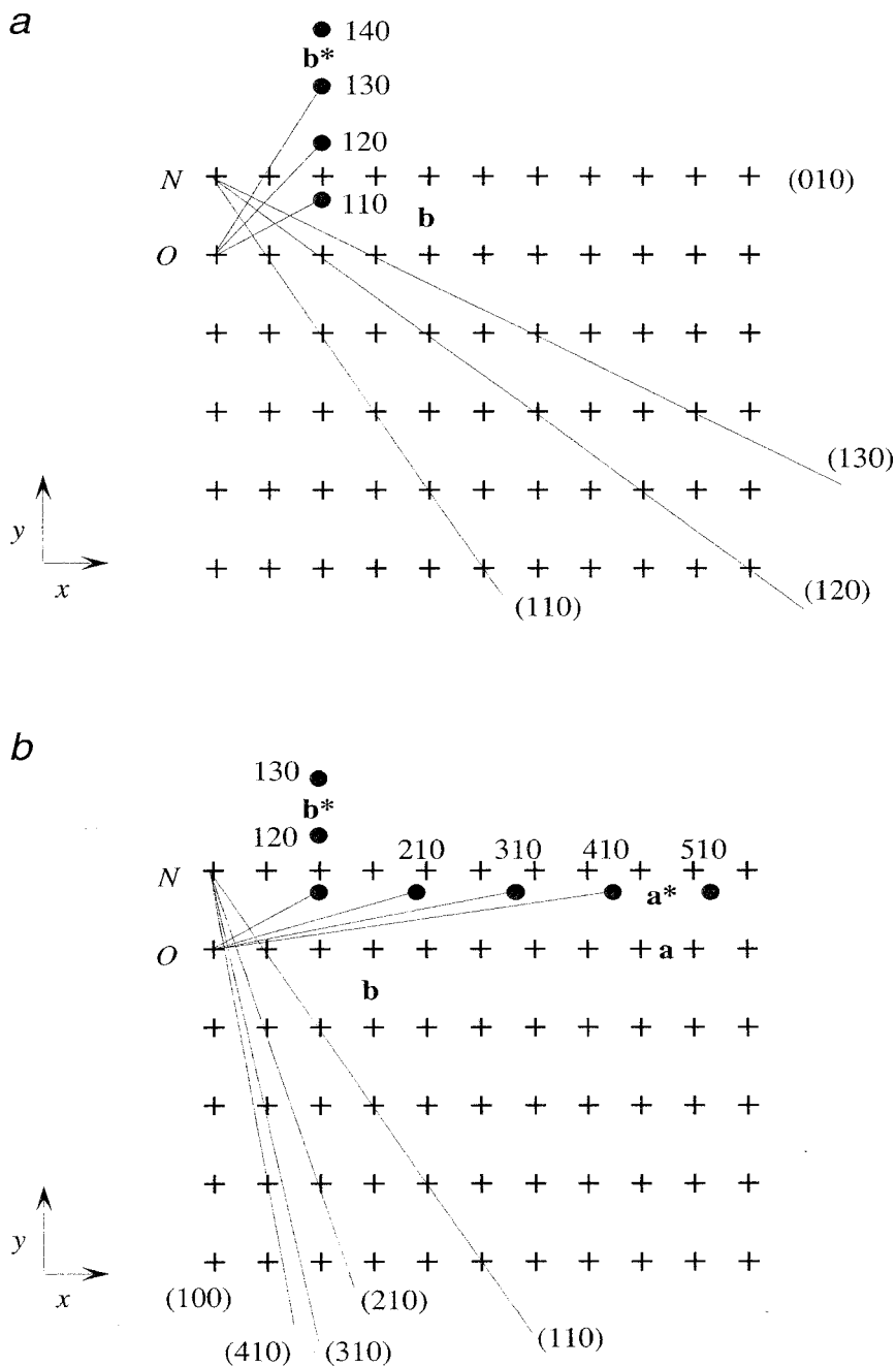
Figure 4.8 (a) Construction of reciprocal lattice. Real-lattice points are +s, and reciprocal lattice points are dots. Notice the real cell edges \mathbf{b} and a reciprocal cell edge \mathbf{b}^* . (b) Continuation of (a). Notice the real cell edges \mathbf{a} and a reciprocal cell edge \mathbf{a}^* .
