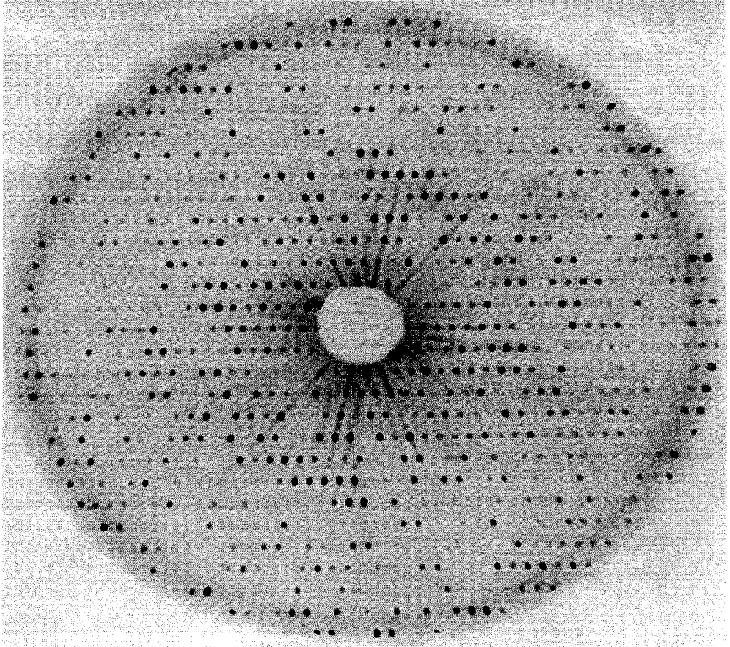
Figure 2.6 Diffraction pattern from a crystal of the MoFe (molybdenum–iron) protein of the enzyme nitrogenase from Clostridium pasteurianum . Notice that the reflections lie in a regular pattern, but their intensities (darkness of spots) are highly variable. [The hole in the middle of the pattern results from a small metal disk (beam stop) used to prevent the direct X-ray beam, most of which passes straight through the crystal, from destroying the center of the film.] Photo courtesy of Professor Jeffery Bolin.
