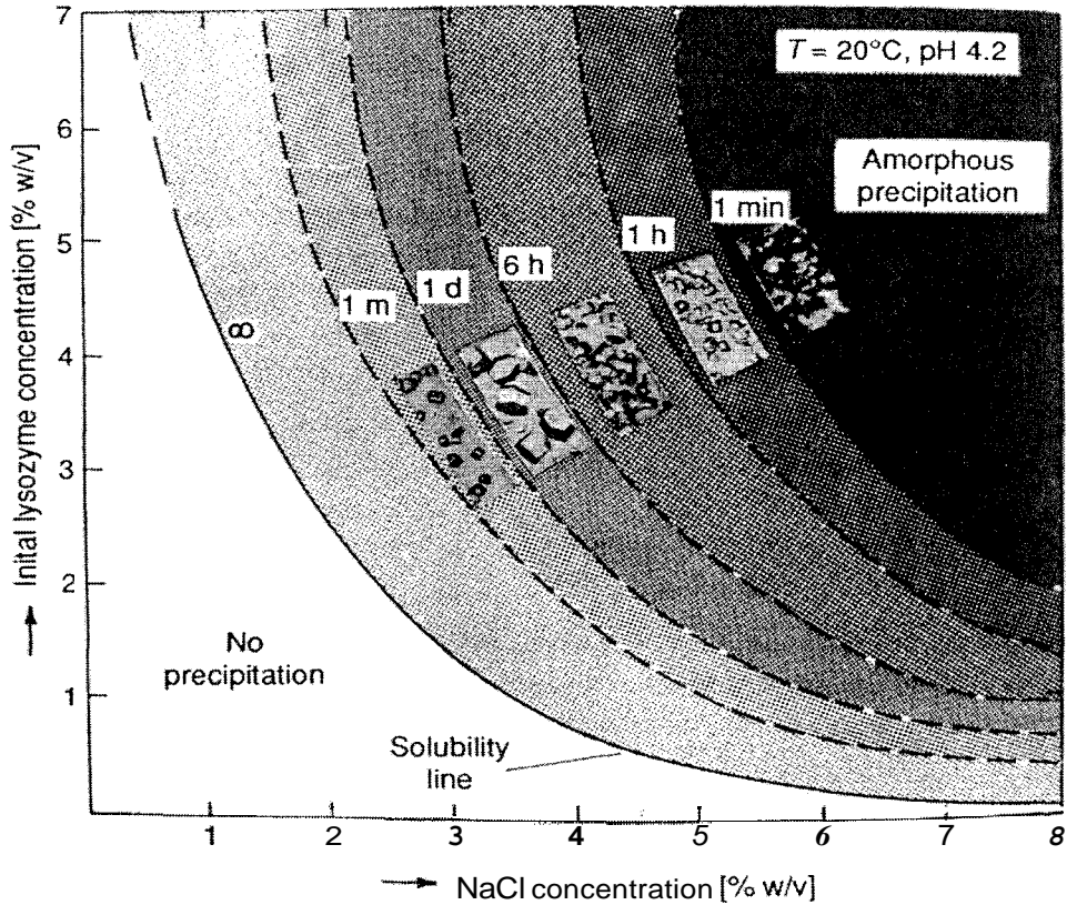
Figure 3.3 Schematic map of crystallization kinetics as a function of lysozyme and NaCl concentration obtained from a matrix of dishes. Inserts show photographs of dishes obtained 1 month after preparation of solutions. From G. Feher and X. Kam, in Methods in Enzymology 114 , H. W. Wyckoff, C. H. W. Hirs, and S. N. Timasheff, eds., Academic Press, Orlando, Florida, 1985, p. 90. Photo and caption reprinted with permission.
