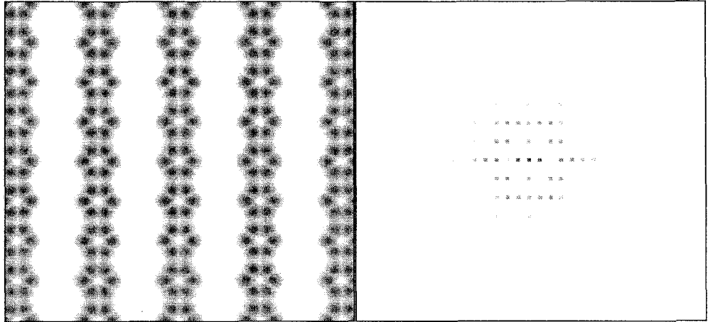
Figure 2.10 Lattices of hexagons (left) and its diffraction pattern (right). If you look at the pattern and blur your eyes, you will see the diffraction pattern of a hexagon. The pattern is that of the average hexagon in the real lattice, but it is sampled at the reciprocal lattice points.
