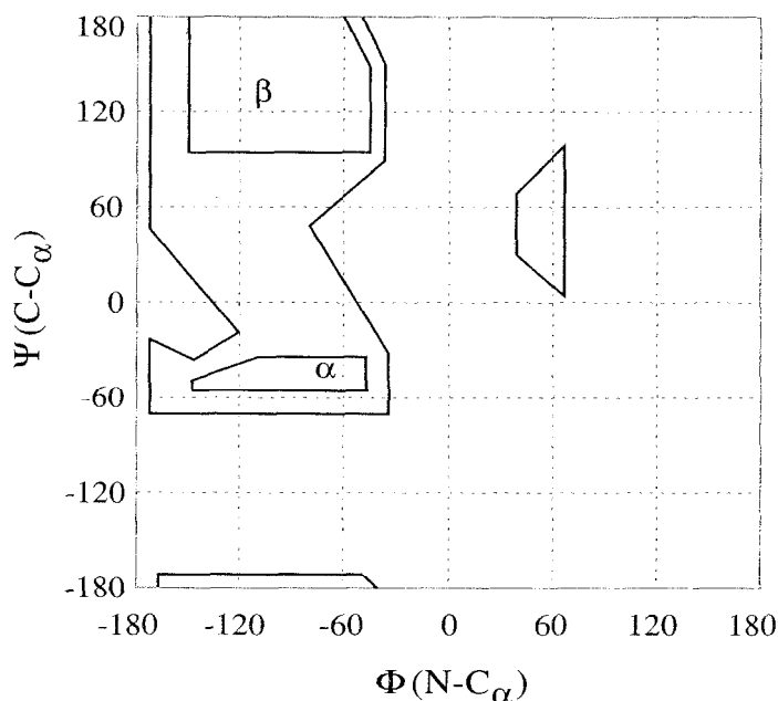
Figure 8.2 Ramachandran diagram for nonglycine amino-acid residues in proteins. Angles \Phi and \Psi are as defined in Fig. 8.1.
