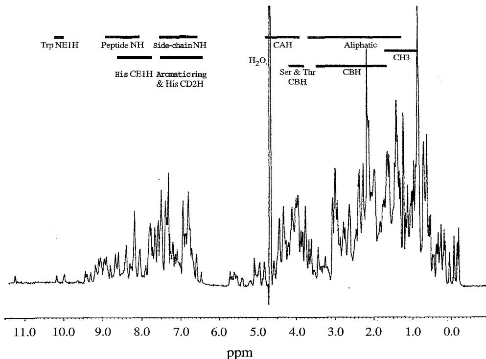
Figure 10.1 ^1\text{H} -NMR spectrum of thioredoxin, reduced form. Labels show chemical-shift values typical of various hydrogen types in protein chains having random coil conformation. Some signals lie outside these ranges because of specific interactions not present in random coils. Atom labels are as found in PDB coordinate files. Spectrum generously provided by Professor John M. Louis.
