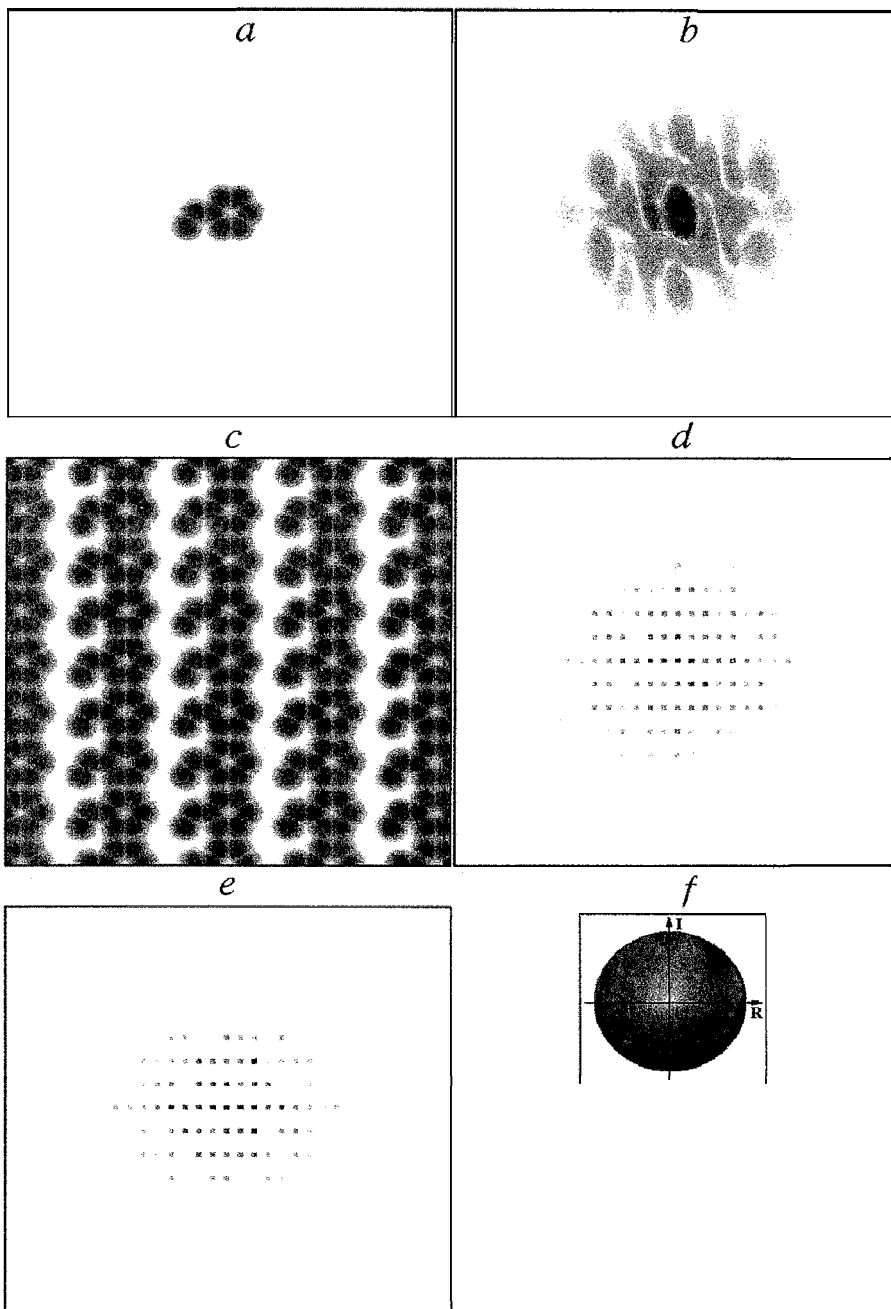
Plate 3 Simple asymmetric object, alone and in a lattice, and the computed diffraction pattern of each, with phases depicted by color. Darkness of color indicates the intensity of a reflection. The phase angle of a region in b or a reflection in d corresponds to the angle of its color on the color wheel. Experimental diffraction patterns do not contain phase information, as in e . (For discussion, see Chapter 2.) Images computed and generously provided by Dr. Kevin Cowtan. For more illustrations of Fourier transforms as they apply to macromolecular crystallography, direct your web browser to the CMCC Home Page ( www.usm.maine.edu/~rhodes/CMCC ) and select Kevin Cowtan's Book of Fourier.
