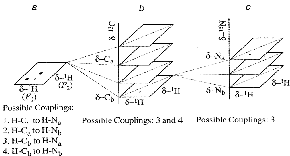
Figure 10.7 3-D and 4-D NMR. (a) 2-D NMR of H-C a /H-C b /H-N a /H-N b . Chemical shifts of H-C, and H-C b are identical, as are those of H-N, and H-N b . so only two peaks appear on the diagonal. One cross-peak could arise from four possible couplings, listed on the figure. (b) Spectrum of (a) spread onto planes, each at a different ^{13}\text{C} chemical shift \delta . The \delta - ^{13}\text{C} axis represents the third NMR dimension. Thin lines represent the position of the diagonal on each plane. The cross-peak occurs only on the plane at \delta - ^{13}\text{C}_b , revealing that coupling involves H-C b and eliminating two possible couplings. (c) Spectrum at in (b), spread onto planes, each at a different ^{15}\text{N} chemical shift \delta . The \delta - ^{15}\text{N} axis represents the fourth NMR dimension. The cross-peak occurs only on the plane at \delta - ^{15}\text{N}_a , revealing that coupling involves H-N a . Thus the coupling indicated by the cross peak in (a) is H-C b to H-N a .
