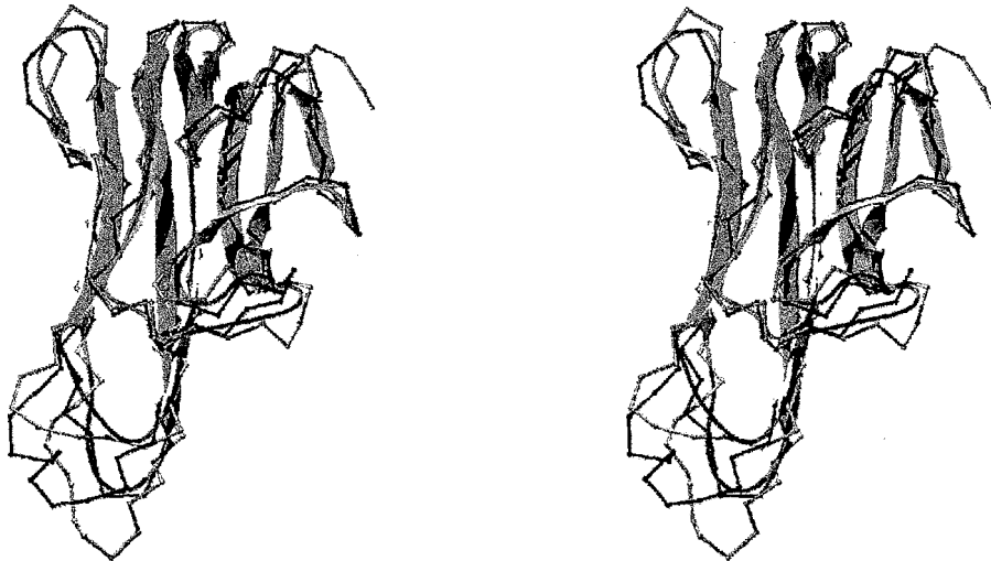
Plate 20 Homology modeling project returned from SWISS-MODEL. The target protein is a fragment of FasL, a ligand for the widely expressed mammalian protein Fas. Interaction of Fas with FasL leads to rapid cell death via apoptosis. The template proteins are (1) tumor necrosis factor receptor P55, extracellular domain (PDB 1tnr, black) and (2) tumor necrosis factor-alpha (PDB 2tun, gray). The modeled FasL fragment is shown as ribbon and colored by model \beta -factors. Only the alpha carbons of the templates are shown. (For discussion, see Chapter 11.) Image: SPV/POV-Ray.
