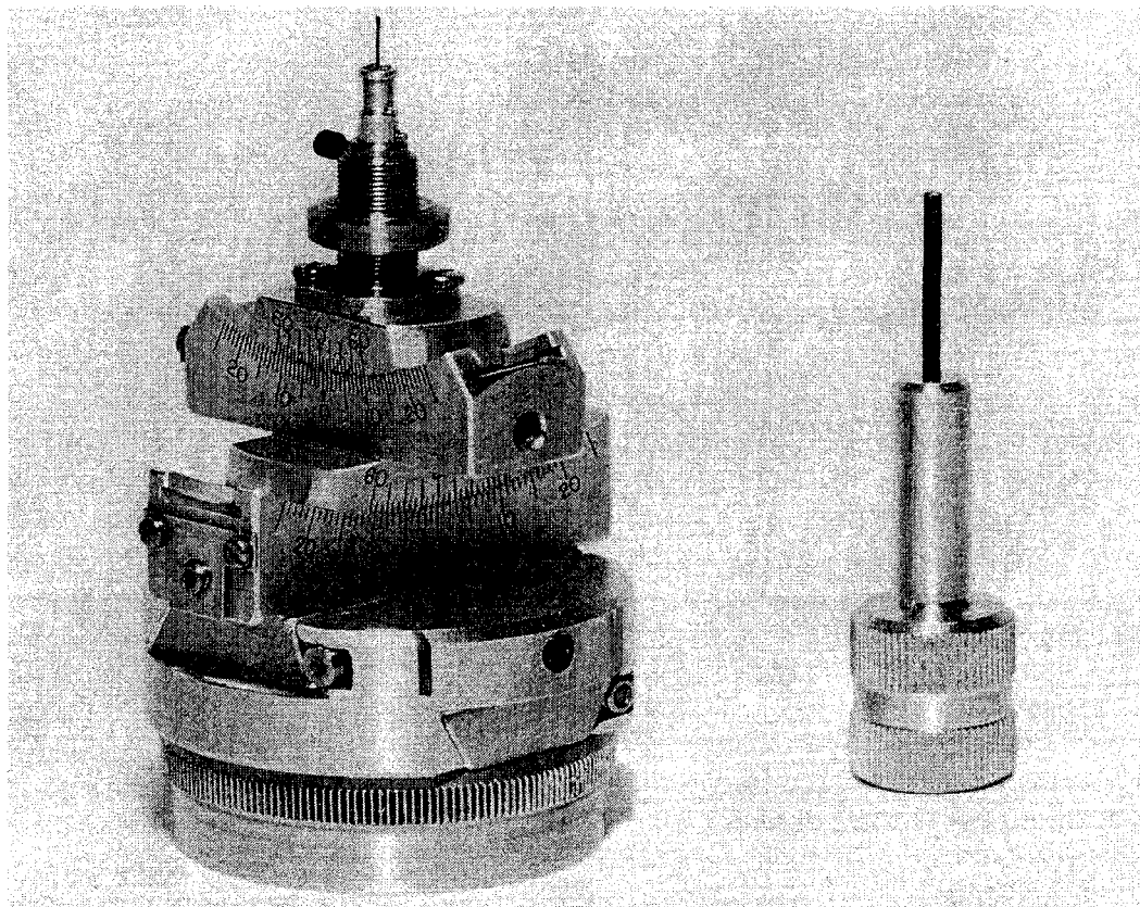
Figure 4.20 Goniometer head, with capillary tube holder at top. The tool (right) is an Allen wrench for adjusting arcs and sledges. Photo courtesy of Charles Supper Company.
