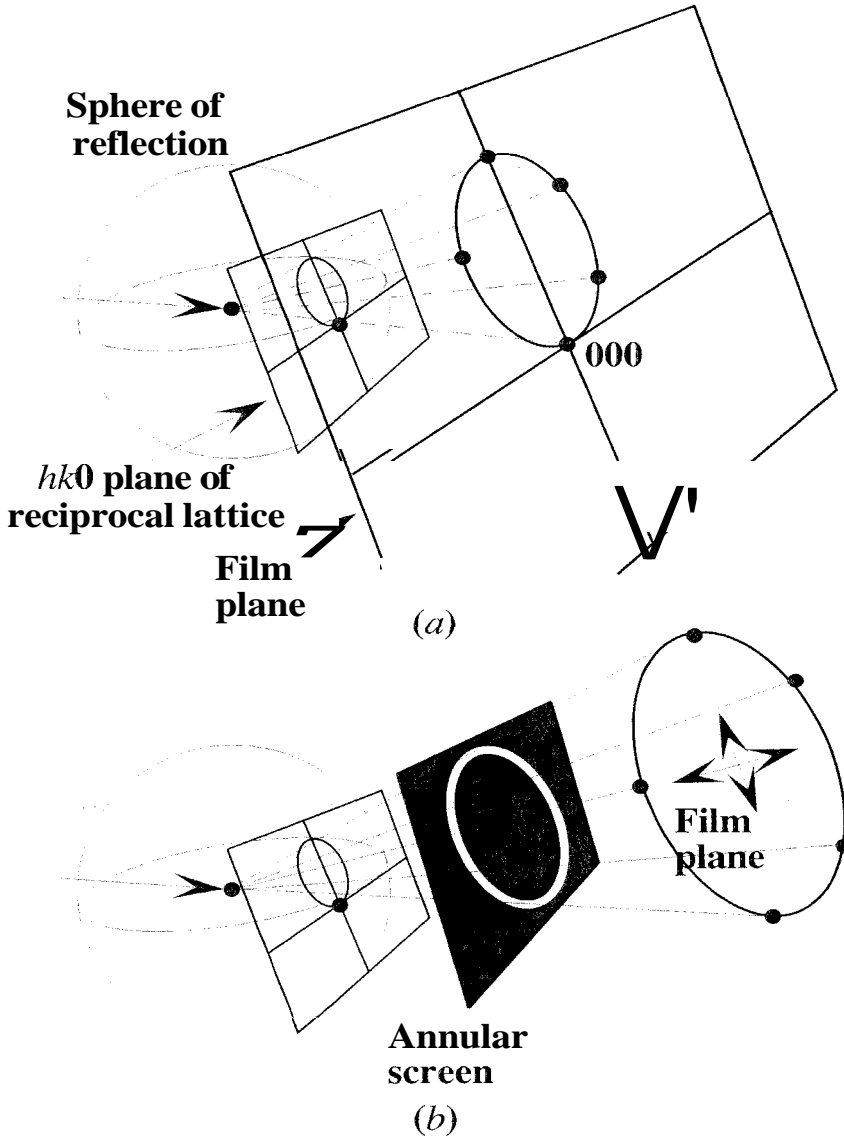
Figure 4.24 (a) Geometry of precession photography. Reflections from a single plane of the reciprocal lattice emerge from the crystal on the surface of a cone. (b) Annular screen selects one cone of reflections, and thus one plane of reciprocal-lattice points, for photography.
