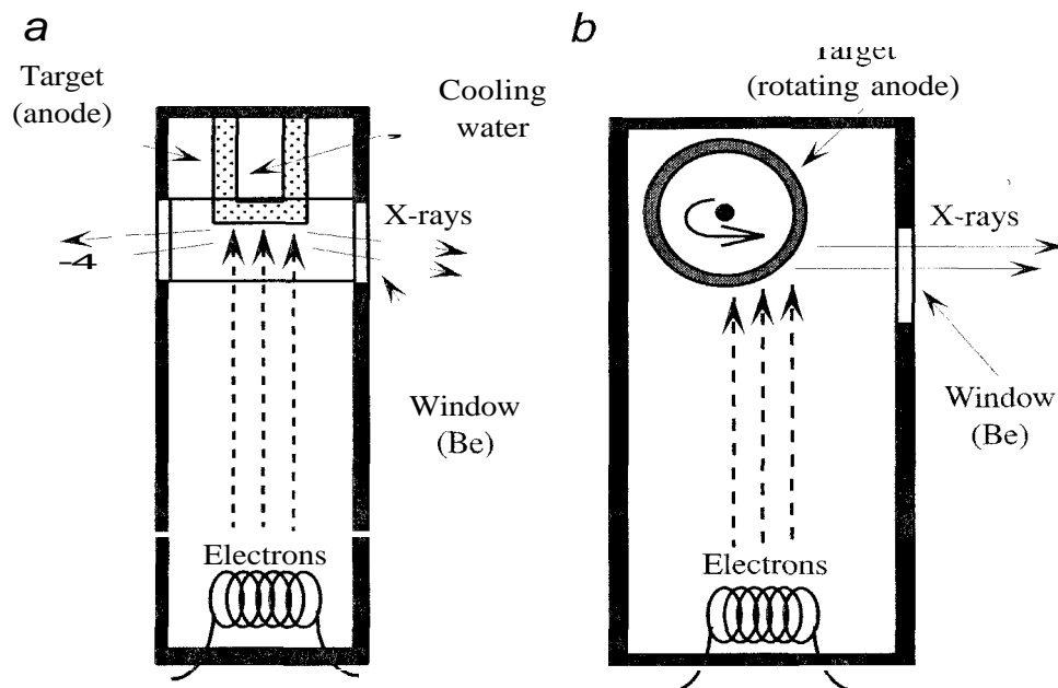
Figure 4.17 (a) X-ray tube. (b) Rotating anode tube.
