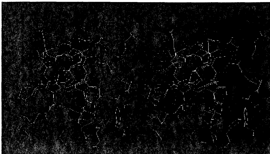
Plate 18 Dotted surface displays of heme in cytochrome b5 (PDB 3b5c). Smaller van der Waals surface encloses heme completely. Small outer dotted surface is the solvent-accessible surface of the heme. Most of the heme surface is buried within the protein. (For discussion, see Chapter 11.) Image: SPV/POV-Ray.
