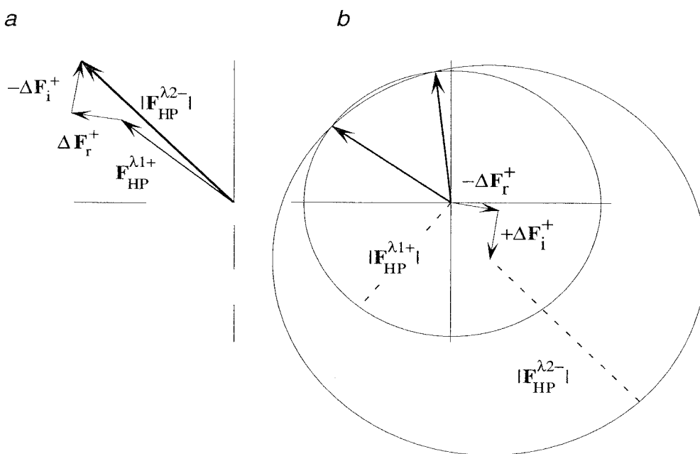
Figure 6.14 Reflection of \mathbf{F}^- components across the real axis gives a second vector equation involving the desired structure factor. (a) All reflected components are labeled with their equivalent contributions from \mathbf{F}^+ . (b) Vector solution of Eq. (6.14). These solutions are compatible only with \mathbf{F}_a in Fig. 6.13.
