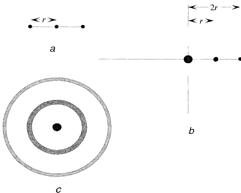
Figure 9.6 Radial Patterson function. (a) Linear triatomic molecule. (b) Patterson function constructed from (a). For construction procedure, see Chapter 6, Section III.C and Figure 6.10. (c) Patterson function (b) averaged by rotation, the expected result of calculating a Patterson function from diffraction intensities measured from an amorphous sample.
