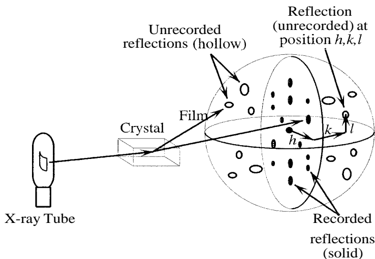
Figure 2.11 Crystallographic data collection, showing reflections measured at one particular crystal orientation (solid, on film) and those that could be measured at other orientations (hollow, within the sphere but not on the film). The relationship between measured and unmeasured reflections is more complex than shown here (see Chapter 4).
