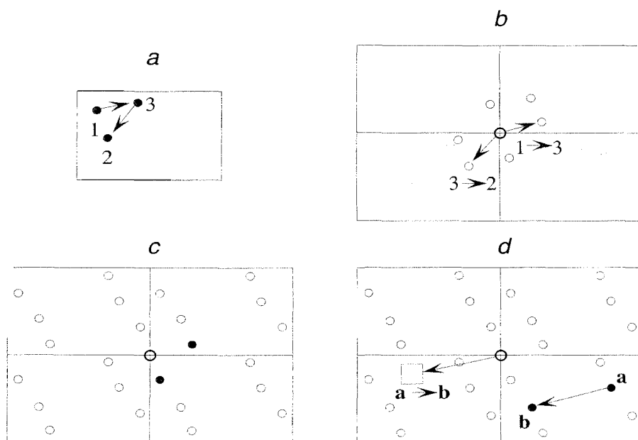
Figure 6.10 Construction and interpretation of a Patterson map. (a) Structure of unit cell containing three atoms. Two of the six interatomic vectors are shown. (b) Patterson map is constructed by moving all interatomic vectors to the origin. Patterson "atoms" (peaks in the contour map) occur at the head of each vector. (c) Complete Patterson map, containing all peaks from (b) in all unit cells. Peak at origin results from self-vectors. Image of original structure is present (origin and two darkened peaks) amid other peaks. (d) Trial solution of map (c). If origin and Patterson atoms a and b were the image of the real unit cell, the interatomic vector a \rightarrow b would produce a peak in the small box. Absence of the peak disproves this trial solution.
