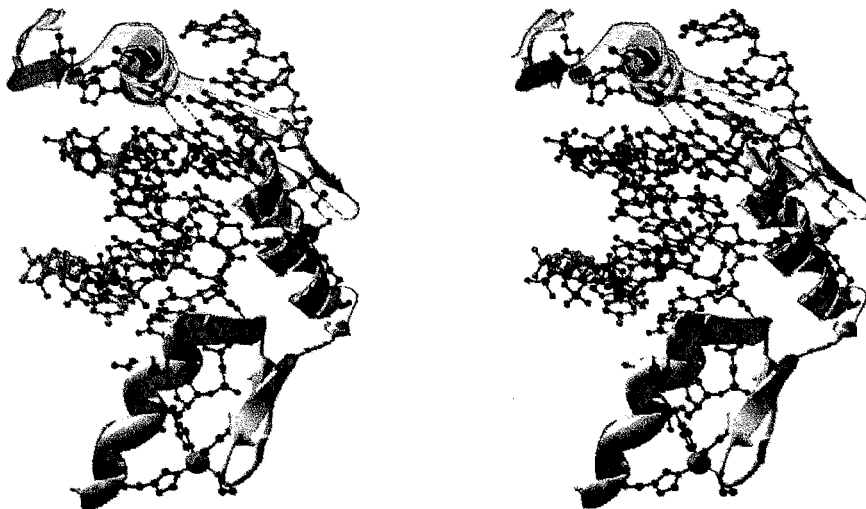
Plate 1 Stereo photograph of Zif268/DNA complex (see N. P. Pavletich and C. O. Pabo, Science 252, 809, 1991). (For discussion, see Chapter 1.) NOTE: Atomic coordinates for preparing this display were obtained from the Protein Data Bank (PDB), which is described in Chapter 7. The PDB file code is 1zaa. To expedite your access to all models shown in this book, I provide file codes in this format: PDB 1zaa. Image created by Swiss-PdbViewer, rendered by POV-Ray. To obtain these programs, see the CMCC Reader's Page.
