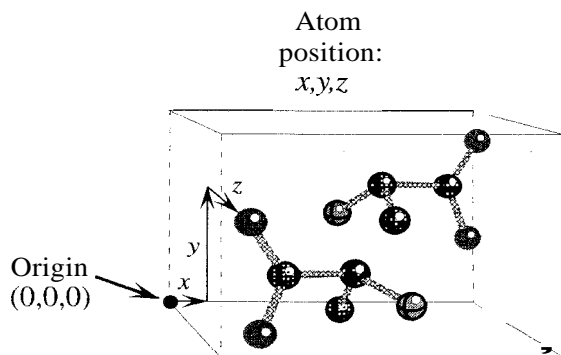
Figure 2.4 One unit cell from Fig. 2.3. The position of an atom in the unit cell can be specified by a set of spatial coordinates x , y , z .
