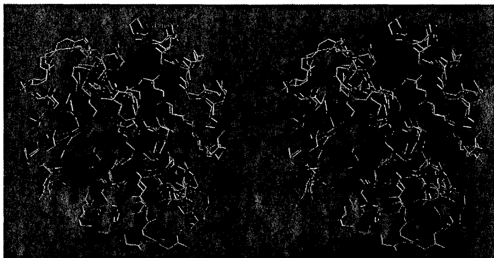
Plate 19 X-ray and NMR models of thioredoxin (PDB 1ert and 3trx) superimposed by least-squares fitting of corresponding alpha carbons in the two models. The x-ray model is gray. Residues of the NMR model are colored according to rms differences in atom positions between the two models. Residues with smallest deviations are blue, those with largest deviations are red, and those of intermediate deviations are in spectral colors between blue and red. (For discussion, see Chapter 11.) Image: SPV/POV-Ray.
