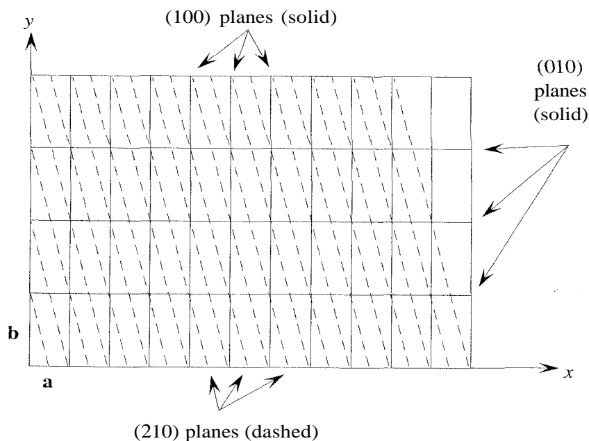
Figure 4.3 (210) planes in a two-dimensional section of lattice.
