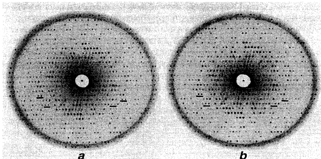
Figure 6.5 Precession photographs of the hk0 plane in native ( a ) and heavy-atom ( b ) crystals of the MoFe protein from nitrogenase. Corresponding underlined pairs in the native and heavy-atom patterns show reversed relative intensities. Photos courtesy of Professor Jeffrey Bolin.
