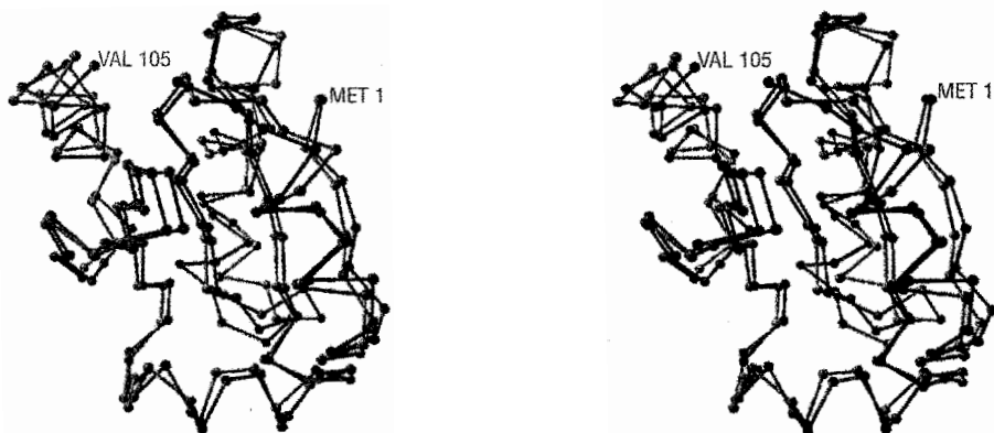
Plate 5 Models of the protein thioredoxin (human, reduced form) as obtained from x-ray crystallography (blue, PDB 1ert) and NMR (red, PDB 3trx). Only backbone alpha carbons are shown. The models were superimposed by least-squares minimization of the distances between corresponding atoms, using Swiss-PdbViewer. (For discussion, see Chapter 3.) Image: SPV/POV-Ray.
