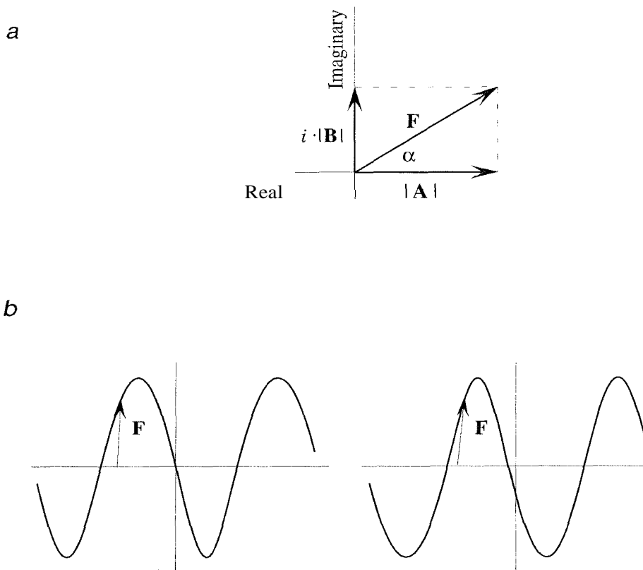
Figure 6.2 (a) The structure factor \mathbf{F} , represented as a vector on the plane of complex numbers. The length of \mathbf{F} is proportional to I^{1/2} , the square root of the measured intensity I , and the angle between \mathbf{F} and the positive real axis is the phase \alpha . (b) (Stereo pair) \mathbf{F} can be pictured as a complex vector spinning around its line of travel. The projection of the path taken by the head of the vector is the familiar sine wave.
