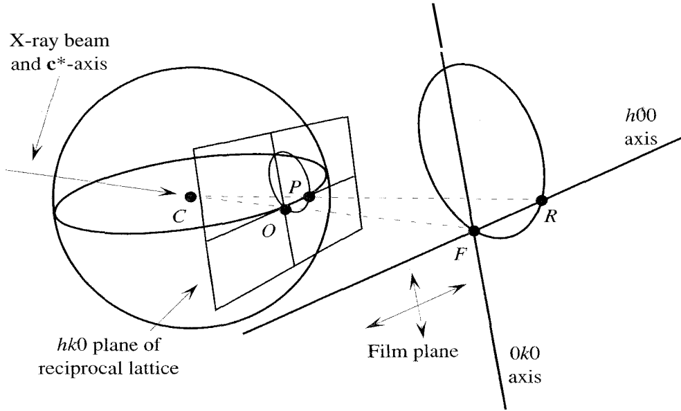
Figure 4.26 Reflection spacings on the film are directly proportional to reciprocal-lattice spacings, and so they are inversely proportional to unit-cell dimensions.
