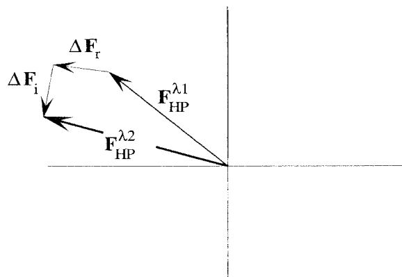
Figure 6.11 Real and imaginary anomalous-scattering contributions alter the magnitude and phase of the structure factor.
