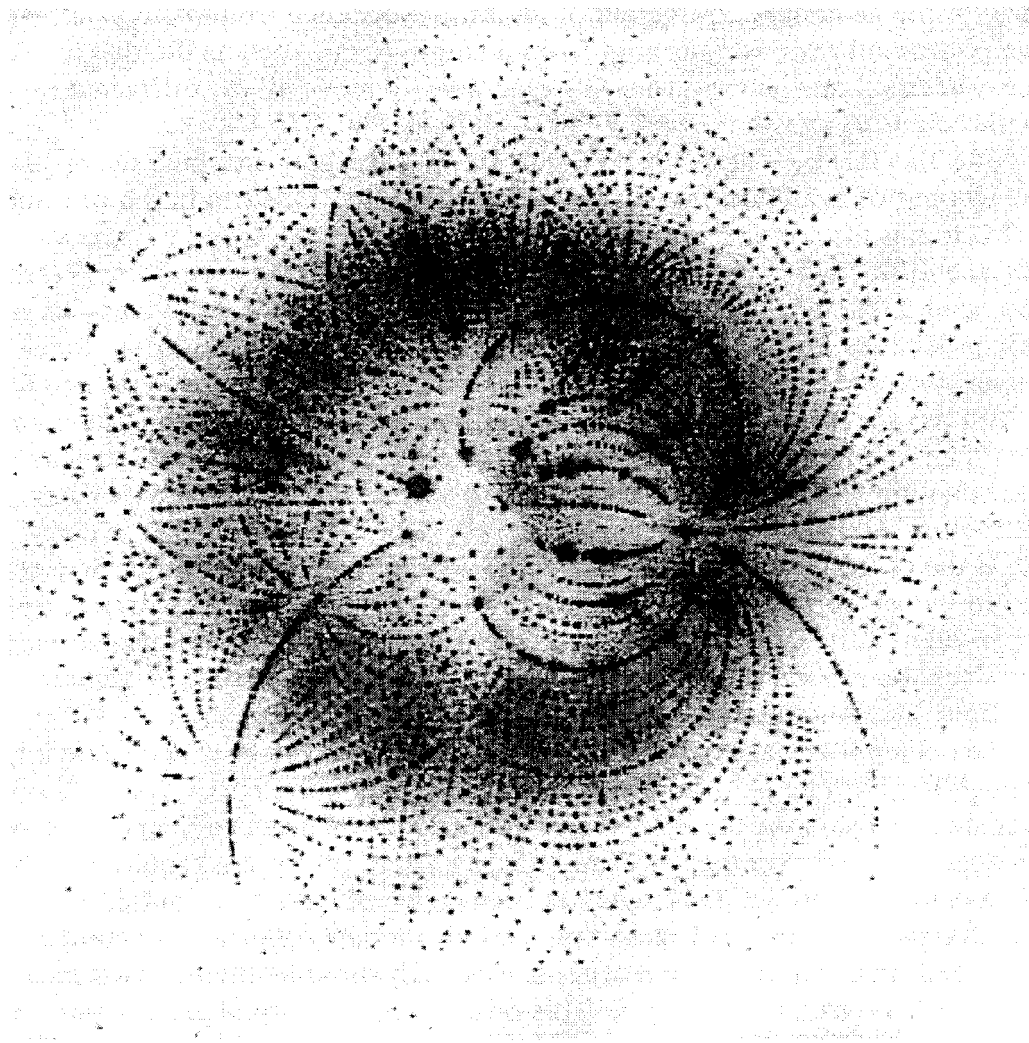
Figure 9.8 A typical Laue image.
