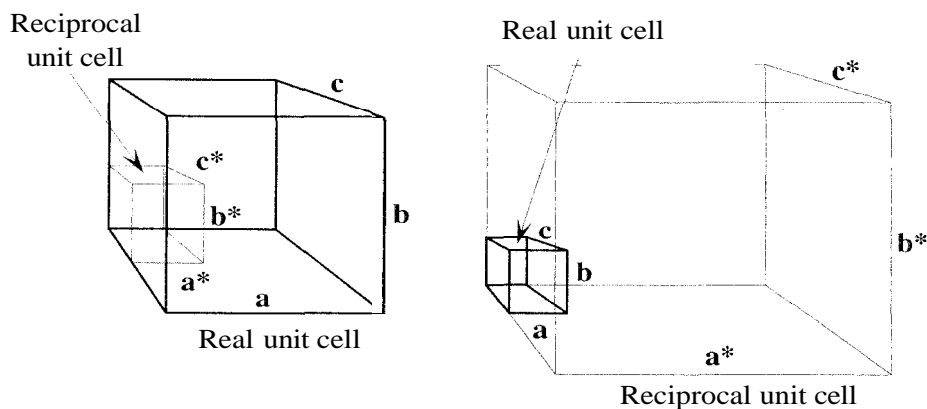
Figure 4.9 Reciprocal unit cells of large and small real cells.
