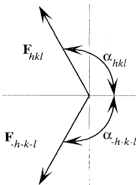
Figure 6.3 Structure factors of a Friedel pair. \mathbf{F}_{-h-k-l} is the reflection of \mathbf{F}_{hkl} in the real axis.
