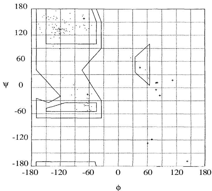
Figure 8.6 Ramachandran plot of the crystallographic model of ALBP. The main-chain torsional angle \psi (N-C, bond) is plotted versus \phi (C-C, bond). The following symbols are used: (.) nonglycine residues; (+) glycine residues. The enclosed areas of the plot show sterically allowed angles. Reprinted with permission from Z. Xu et al. (1992) Biochemistry 31 , 3484–3492. Copyright 1992 American Chemical Society.
