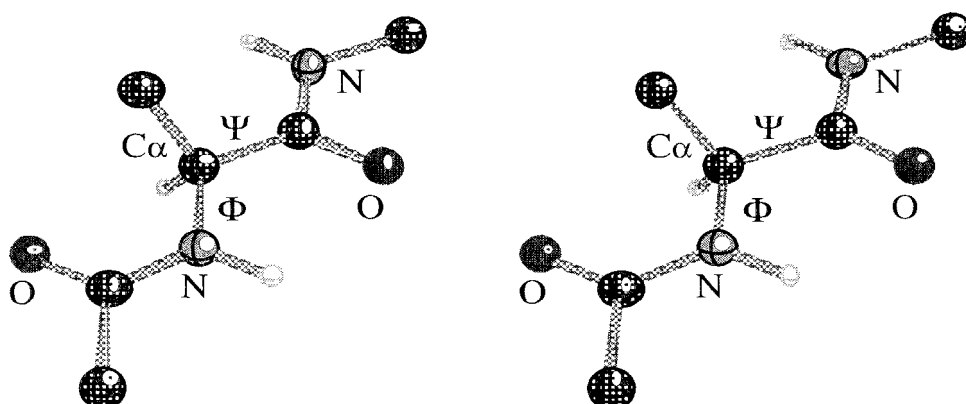
Figure 8.1 Backbone conformational angles in proteins (stereo).
