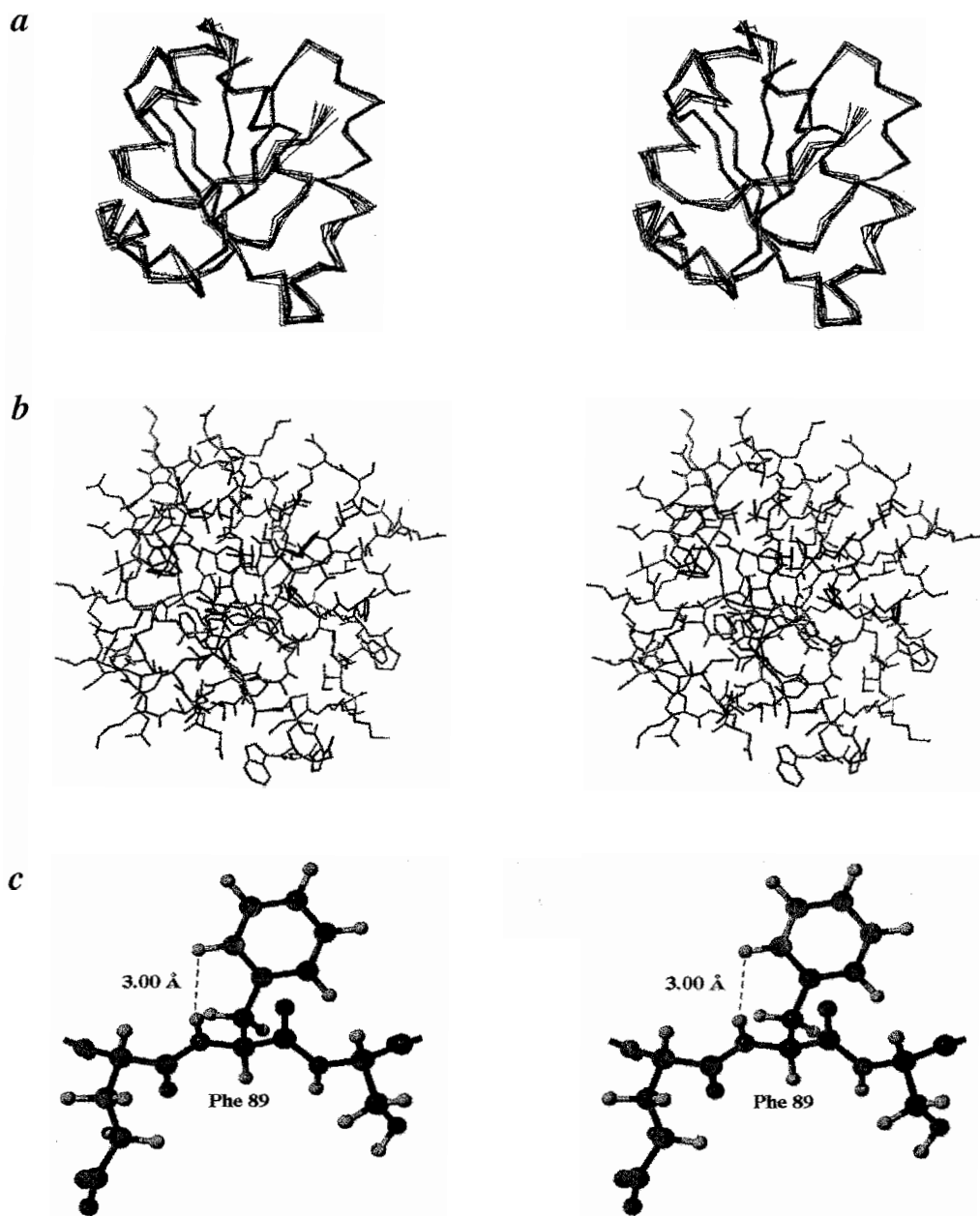
Plate 14 ( a ) Ten of the 33 NMR models of thioredoxin (PDB 4trx). ( b ) Averaged model (PDB 3trx), colored by rms deviation of atom positions in the ensemble from the average position. For each residue, main-chain colors reflect the average rms deviation for C, O, N, and CA, and all side-chain atoms are colored to show the average rms deviation for atoms in the whole side chain. ( c ) Detail of the averaged model at phenylalanine-89, showing the averaged distance between the two hydrogens involved in the distance restraint indicated as “F89N, \delta ” in the NOESY spectrum, Figure 10.6. (For discussion, see Chapter 10.) Image: SPV/POV-Ray.
