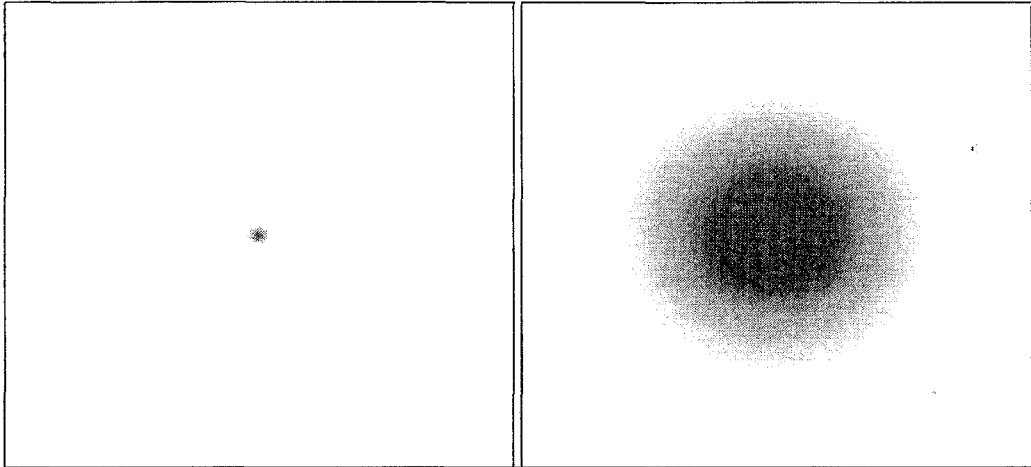
Figure 2.7 Sphere (cross-section, on left) and its diffraction pattern (right). Images for Figures 2.7–2.10 were generously provided by Dr. Kevin Cowtan.
