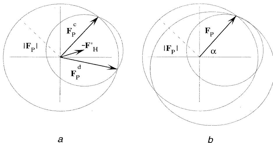
Figure 6.8 (a) A second heavy-atom derivative indicates two possible phases, one of which corresponds to \mathbf{F}_a in Fig. 6.7b. (b) \mathbf{F}_P , which points from the origin to the common intersection of the three circles, is the solution to Equation (6.9) for both heavy-atom derivatives. Thus \alpha is the correct phase for this reflection.
