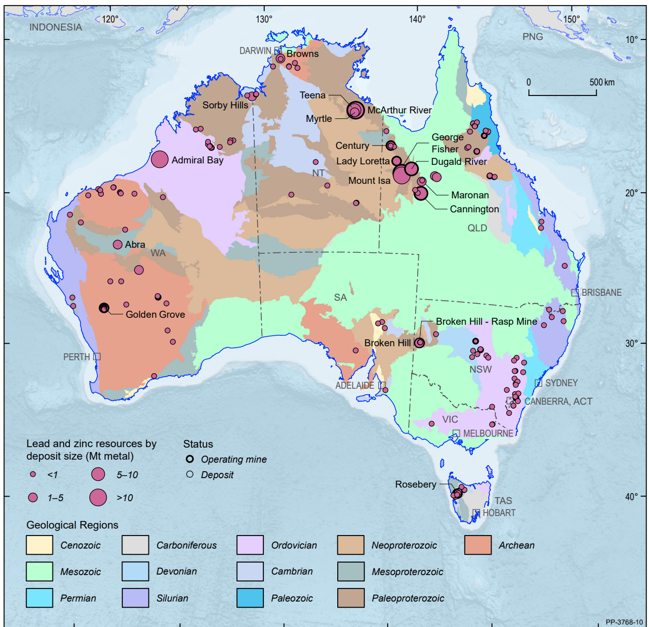
Figure 22 Australian lead and zinc deposits and operating mines, 2019.
