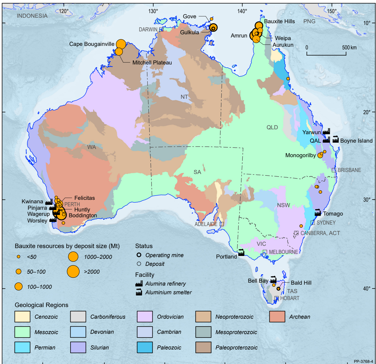
Figure 8 Australian bauxite deposits, operating mines, alumina refineries and aluminium smelters, 2019.
