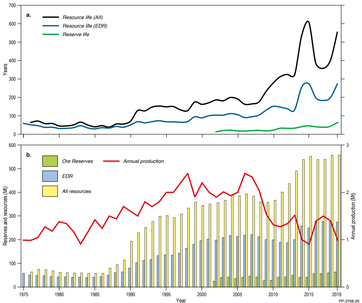
Figure 31 (a) Trends in ilmenite reserve and resource life. These ratios are derived from (b) ilmenite Ore Reserves, Economic Demonstrated Resources (EDR), all resources (EDR + Subeconomic Demonstrated Resources + Inferred) and annual production, 1975–2019.
