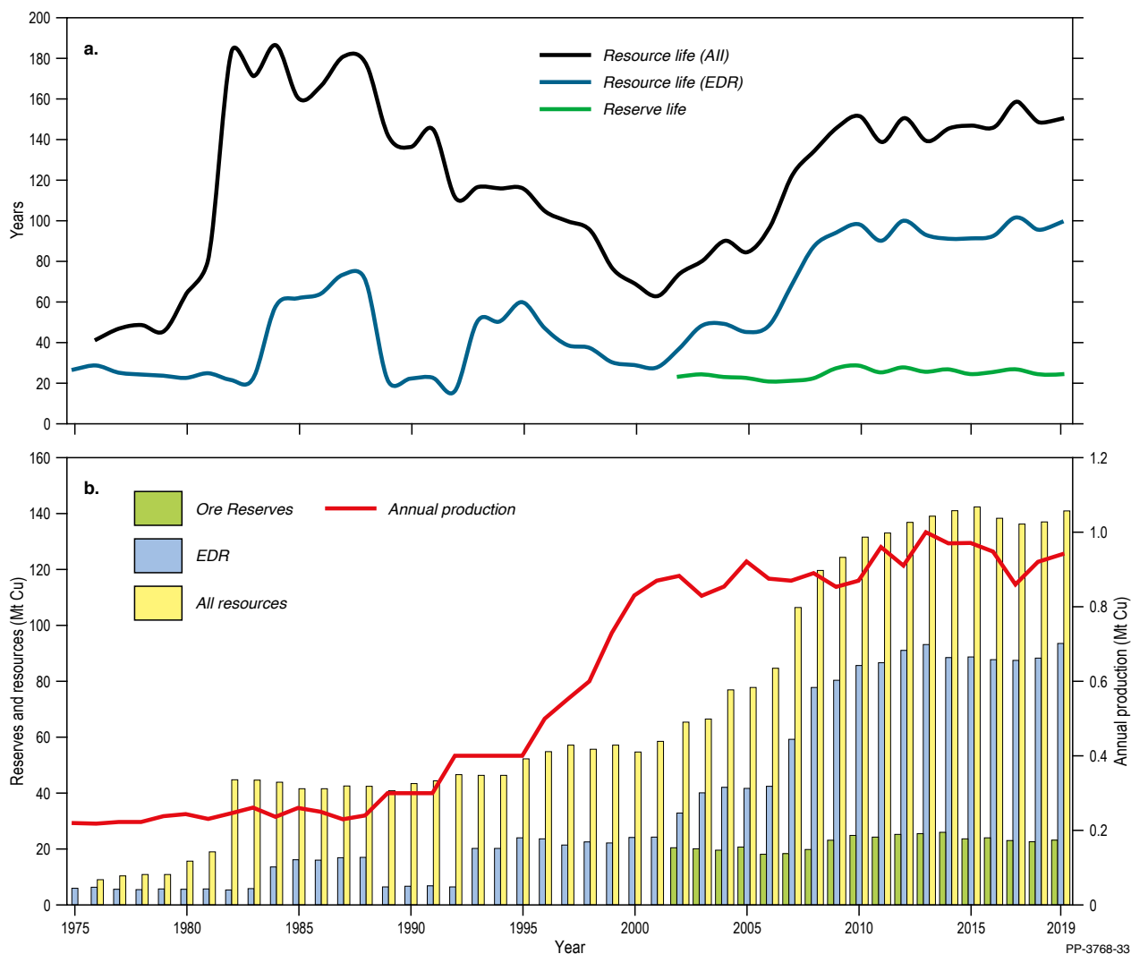
Figure 15 (a) Trends in copper reserve and resource life. These ratios are derived from (b) copper Ore Reserves, Economic Demonstrated Resources (EDR), all resources (EDR + Subeconomic Demonstrated Resources + Inferred) and annual production, 1975–2019.
