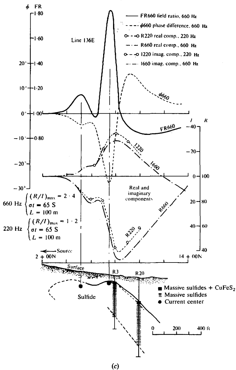
Figure 7.100. (Continued) (c) Sulfide response and interpreted section.
