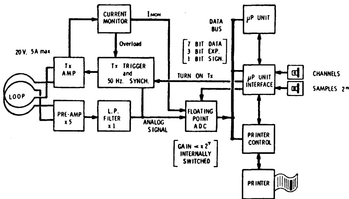
Figure 7.21. Simplified block diagram of SIROTEM. (After Buselli and O'Neill, 1977.)
