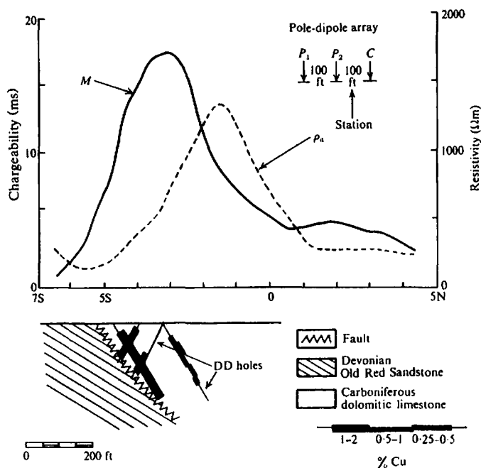
Figure 9.17. Time-domain IP over Gortdram copper-silver body. (From Seigel, 1967.)
