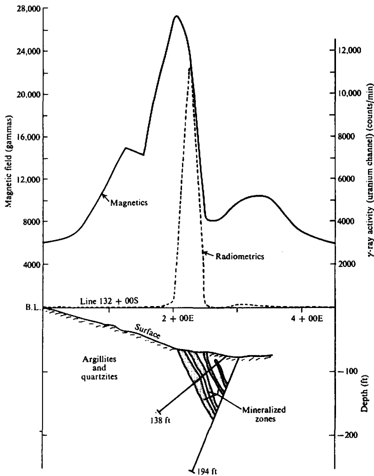
Figure 10.14. Radioactivity and magnetic profiles plus geologic section, line 132 + 00S, uranium survey.
