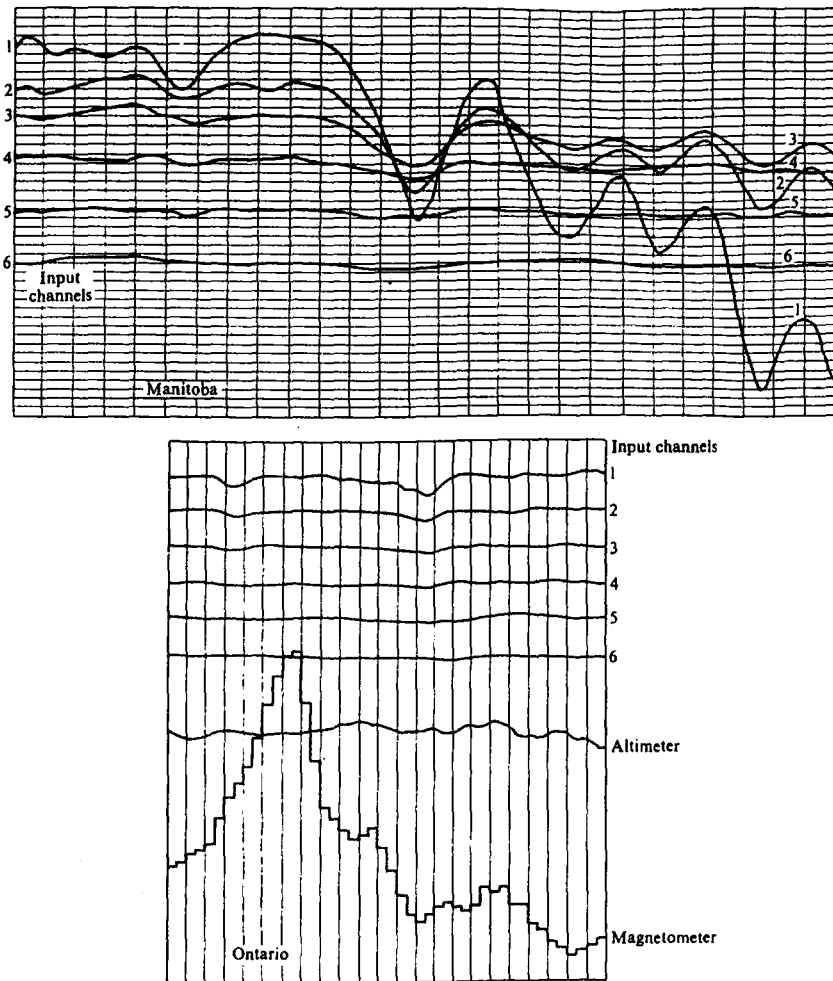
Figure 7.122. Airborne Input EM records.
