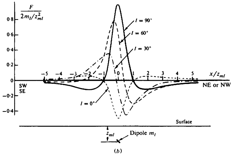
Figure 3.17. Profiles normal to a horizontal line of dipoles. (a) Vertical-field profiles, I = 45^\circ . (b) F profiles for \beta = \pm 45^\circ .
