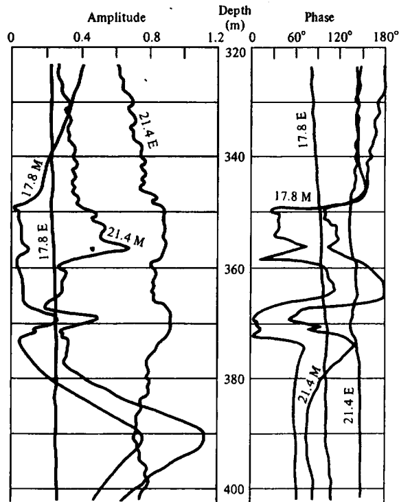
Figure 11.20. Amplitude and phase plots of VLF log past a conductor. E is the electric and M is the magnetic reading, each at 17.8 and 21.4 kHz.
