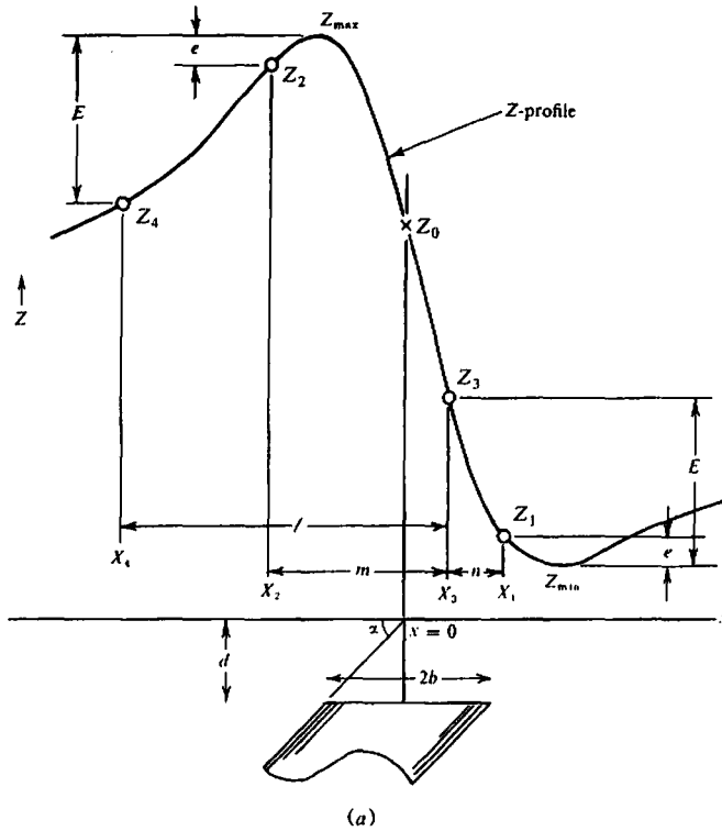
Figure 3.26. Two-dimensional dike of infinite depth extent. (a) Location of conjugate points and X = 0 .
