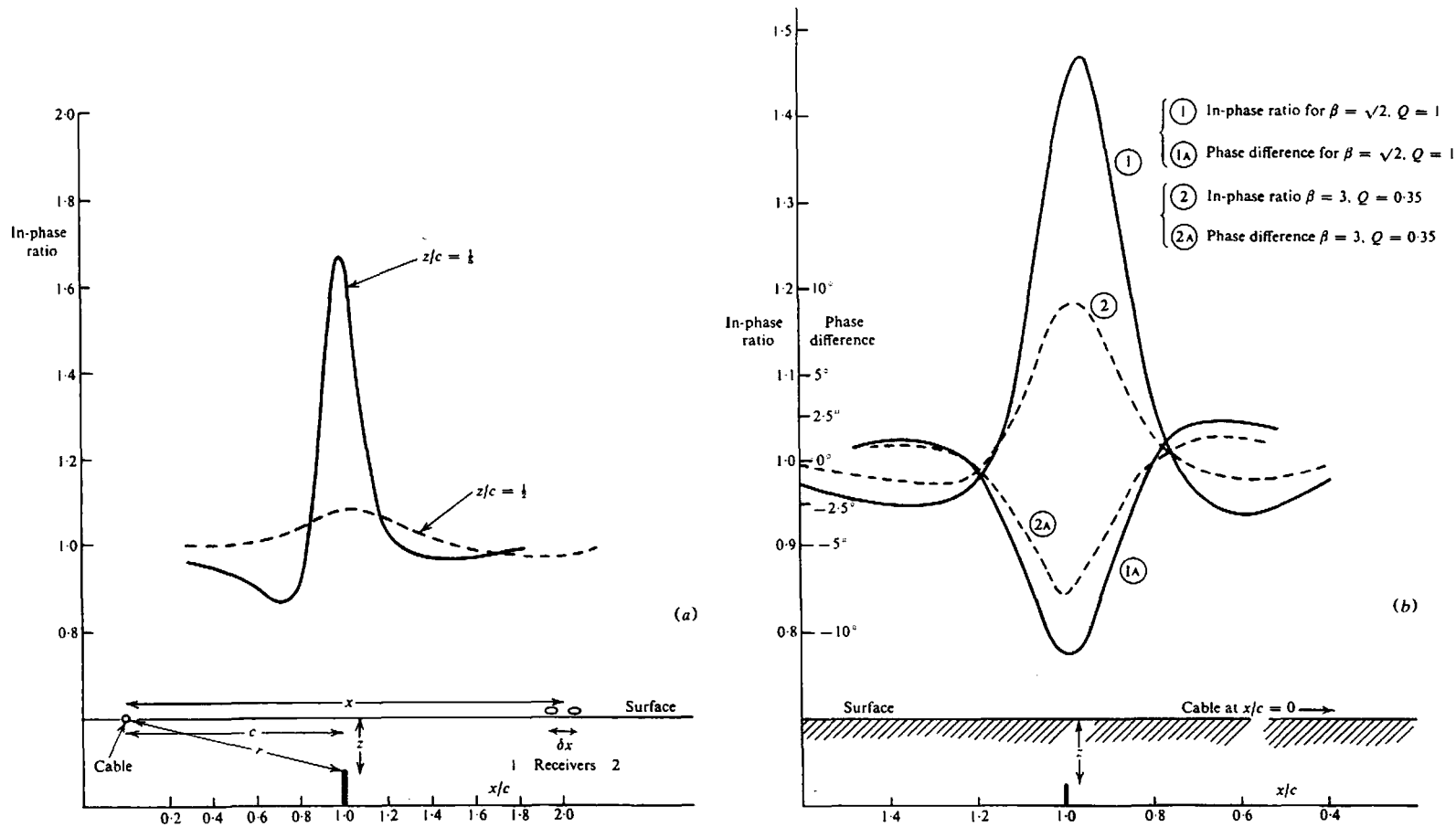
Figure 7.37. Effect of depth and conductivity on Turam profiles over a semiinfinite vertical sheet. Q = \omega L/R , (Eq. (7.16a)). \beta = (1 + 1/Q^2)^{1/2} (Eq. (7.44b)). \delta x/c = 0.1 . (a) Effect of depth variations for \sigma_1 = \infty . (b) Effect of varying conductivity: \sigma_1/\sigma_2 = 2.1 , z/c = 0.2 .
