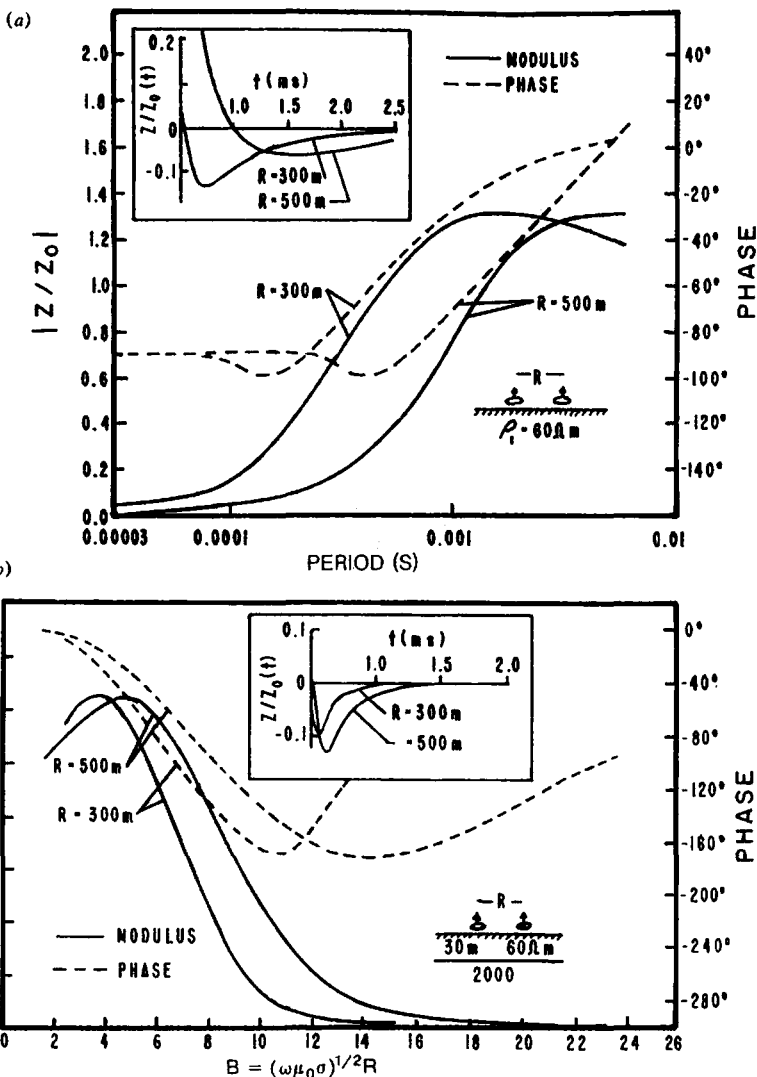
Figure 7.75. Modulus and phase of the mutual coupling ratio in the frequency domain and time domain (small insert) for the horizontal coplanar loop system [Eq. (7.41a)]. (After Patra and Mallick, 1980.) (a) Homogeneous earth. (b) Two-layer earth.
