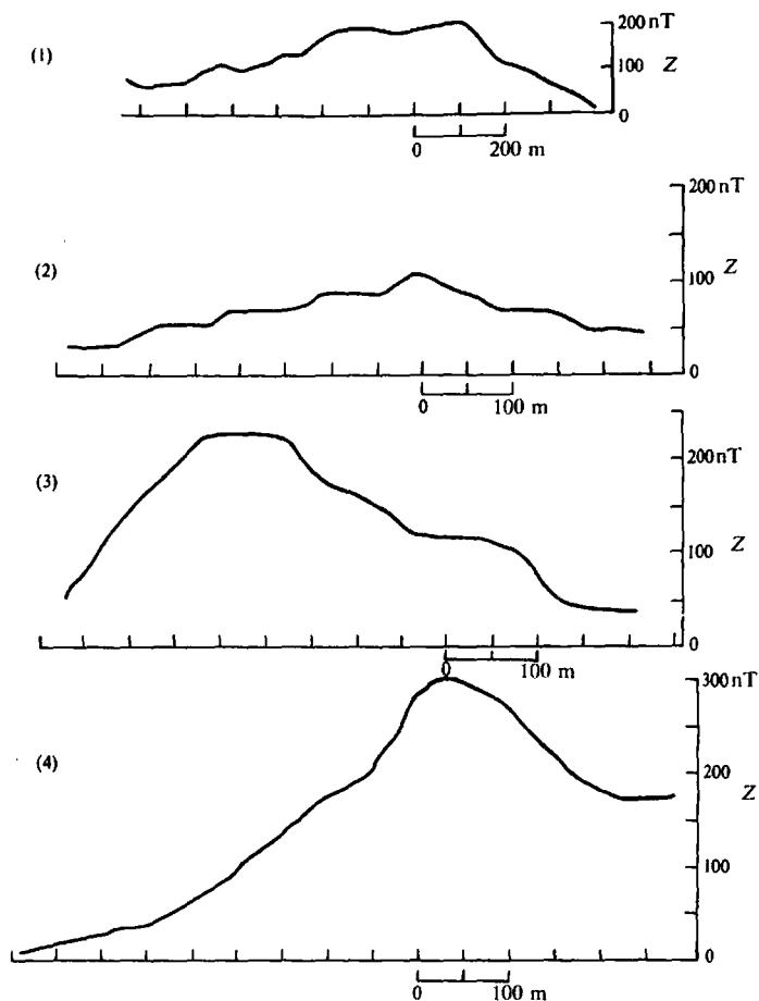
Figure 3.39. Vertical-component magnetic profiles, Manitoba Nickel Belt.
