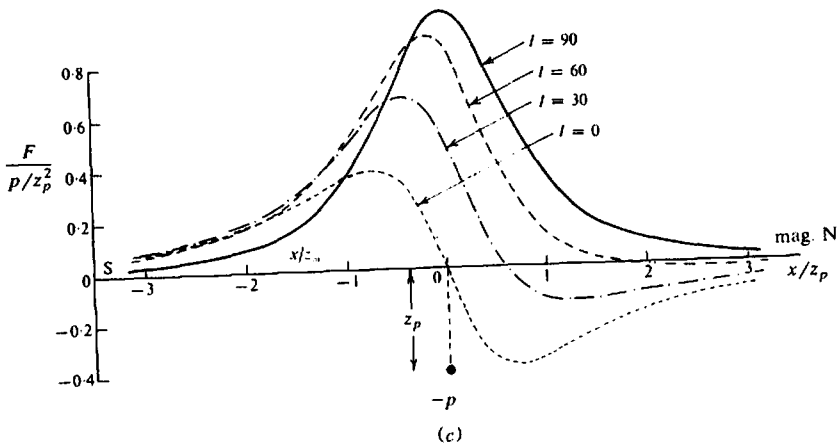
Figure 3.14. (Continued) (b) Contours of |\mathbf{H}_R| = |\mathbf{H} + \mathbf{H}_e| for H_{max} = H_e = 0.38 . (c) F profiles for various inclinations. (After Smellie, 1967.)
