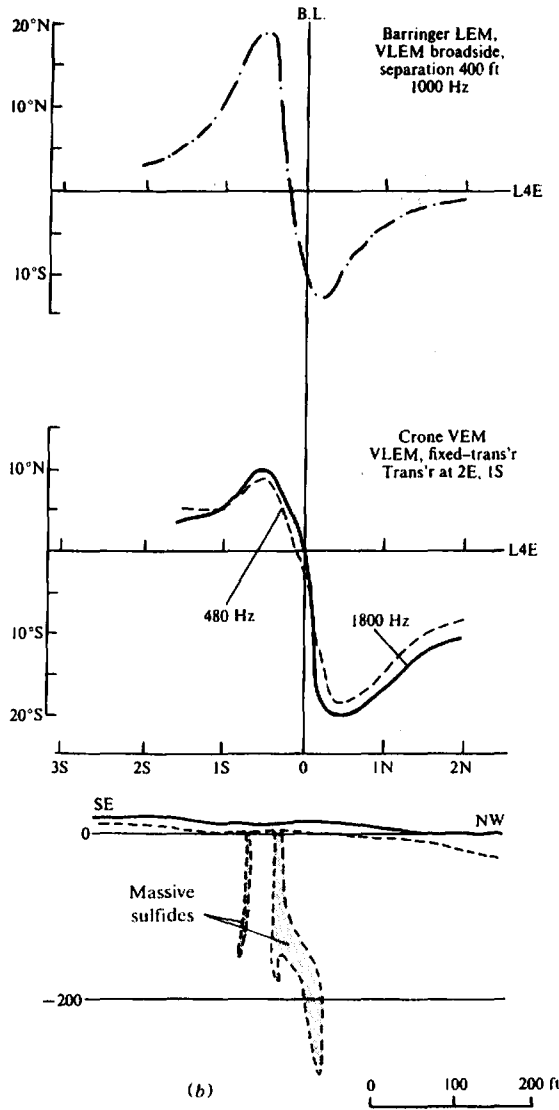
Figure 7.95. (Continued) (b) VLEM profiles and ore section.
