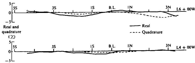
Figure 12.15. HLEM profiles, Abitibi West, Quebec. Frequency 1,000 Hz, T-R separation 300 ft.
