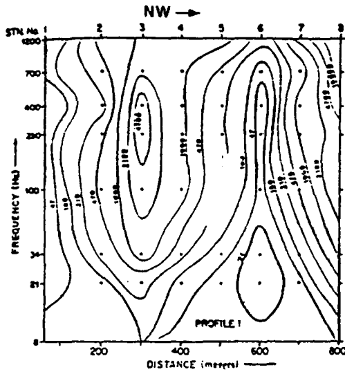
Profile 1 pseudo-section.
