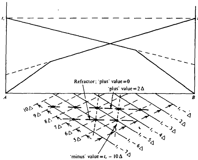
Figure 4.94. The plus-minus method. (After Hagedoorn, 1959.)
