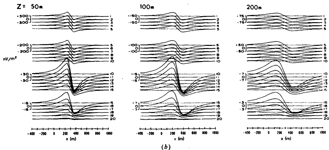
Figure 7.53. (Continued) (b) Variation in \partial H_z/\partial t with depth z ; dip = 90^\circ .
