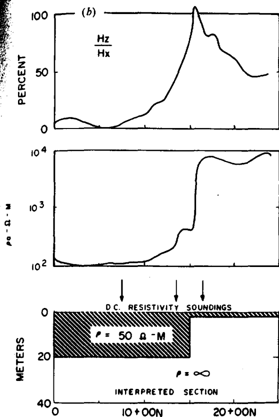
Figure 7.80. (Continued) (b) Curves of (H_z/H_x) and \rho_a on the EM16 profile, plus interpreted section.
