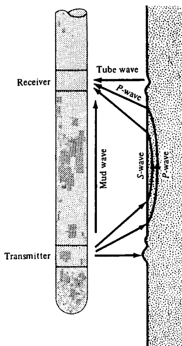
Figure 11.22. Propagation paths for P, S, mud, and tube waves. (From Labo, 1987.)
