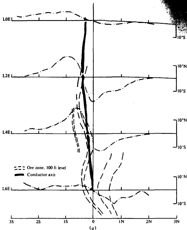
Figure 7.95. EM survey, Uchi Lake, northwest Ontario. (a) Dip-angle broadside profiles. Frequency 1,000 Hz, l = 400 ft, station interval 25 ft.
