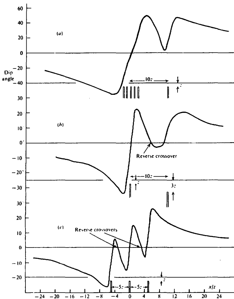
Figure 7.40. VLF profiles over multiple vertical-sheet conductors. (a) Five sheets spaced z apart plus one sheet distant 10z from the midpoint of the five sheets, all at depth z . (b) Two sheets at depths of z and 3z , spaced 10z apart. (c) Three sheets at depth z and spaced 5z apart.
