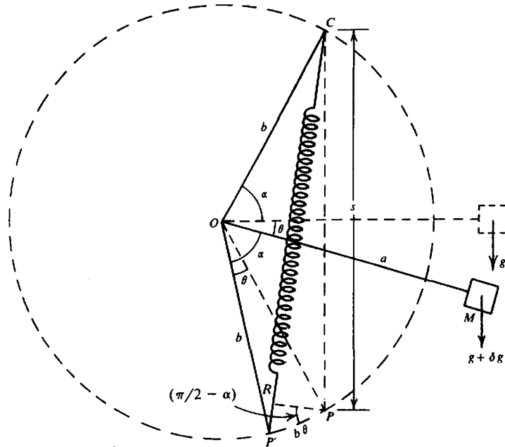
Figure 2.14. Basic principle of the Worden gravimeter.
