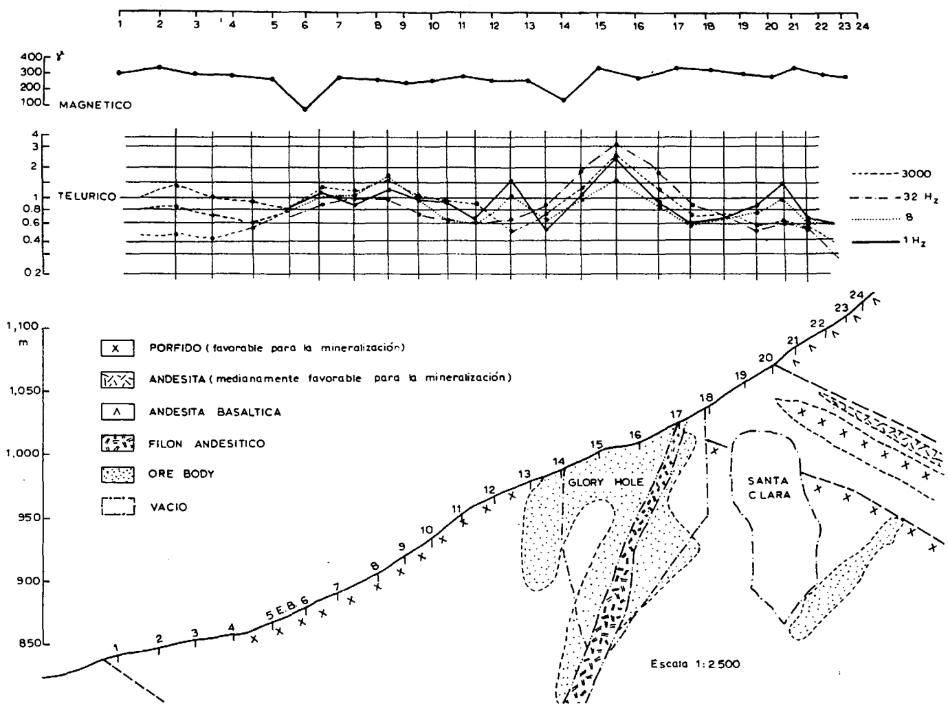
Figure 6.39. Geologic section with magnetic and telluric surface profiles over mine area. Chile.
