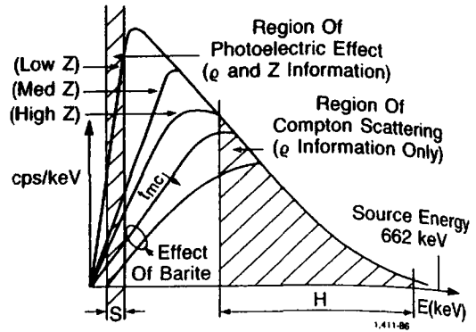
Figure 11.37. Gamma-ray energy spectrum showing the two windows in which measurements are made. The counts in the high-energy window H depend on density only, whereas those in the low-energy windows depend on both density and atomic number Z of the capturing atom. (From Snyder and Fleming, 1985.)
