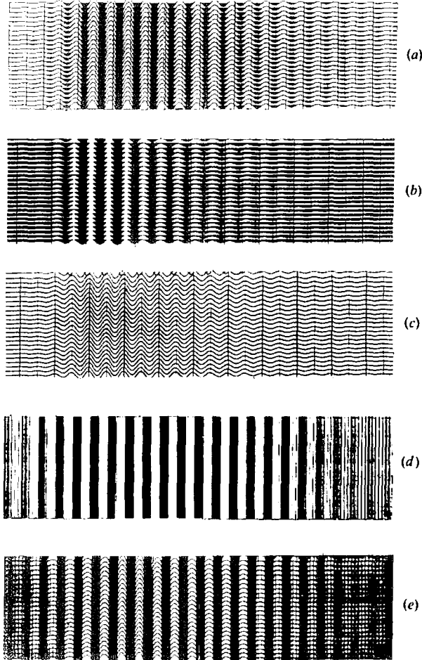
Figure 4.57. Modes of displaying seismic data. (Courtesy Geo Space Corp.) (a) Wiggle superimposed on variable area. (b) Variable area. (c) Wiggle. (d) Variable density. (e) Wiggle superimposed on variable density.
