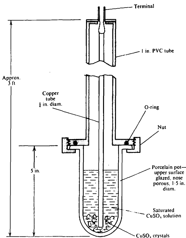
Figure 6.3. Walking-stick SP electrode.
