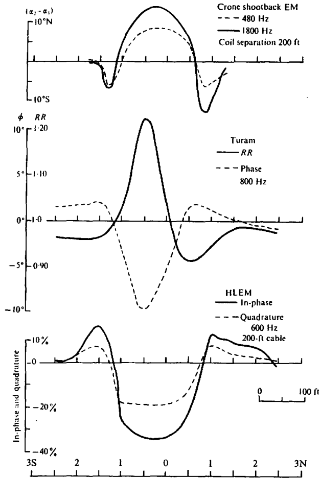
Figure 7.116. Shootback, Turam, and HLEM profiles, western Ontario.
