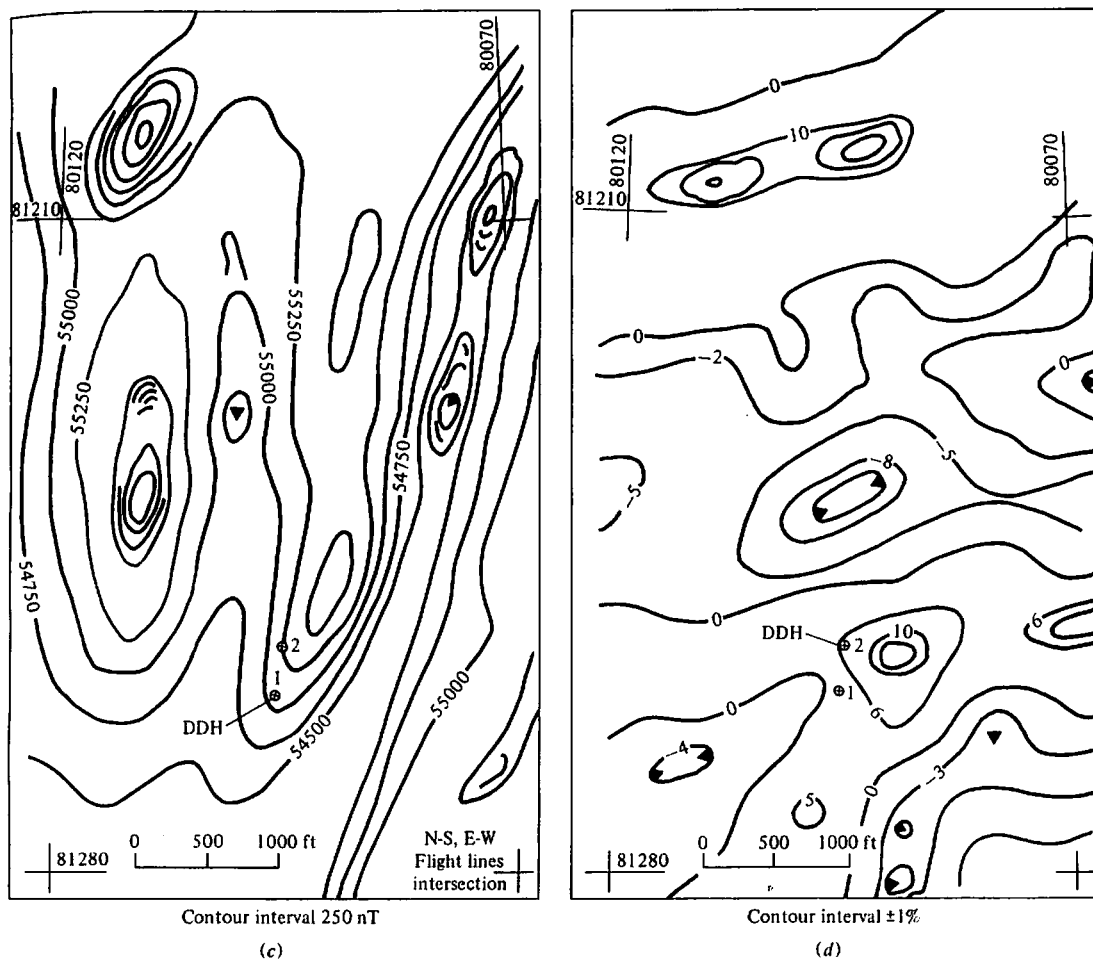
Figure 12.11. (Continued) (c) Total-field magnetic contours. (d) Total-field VLF contours.
