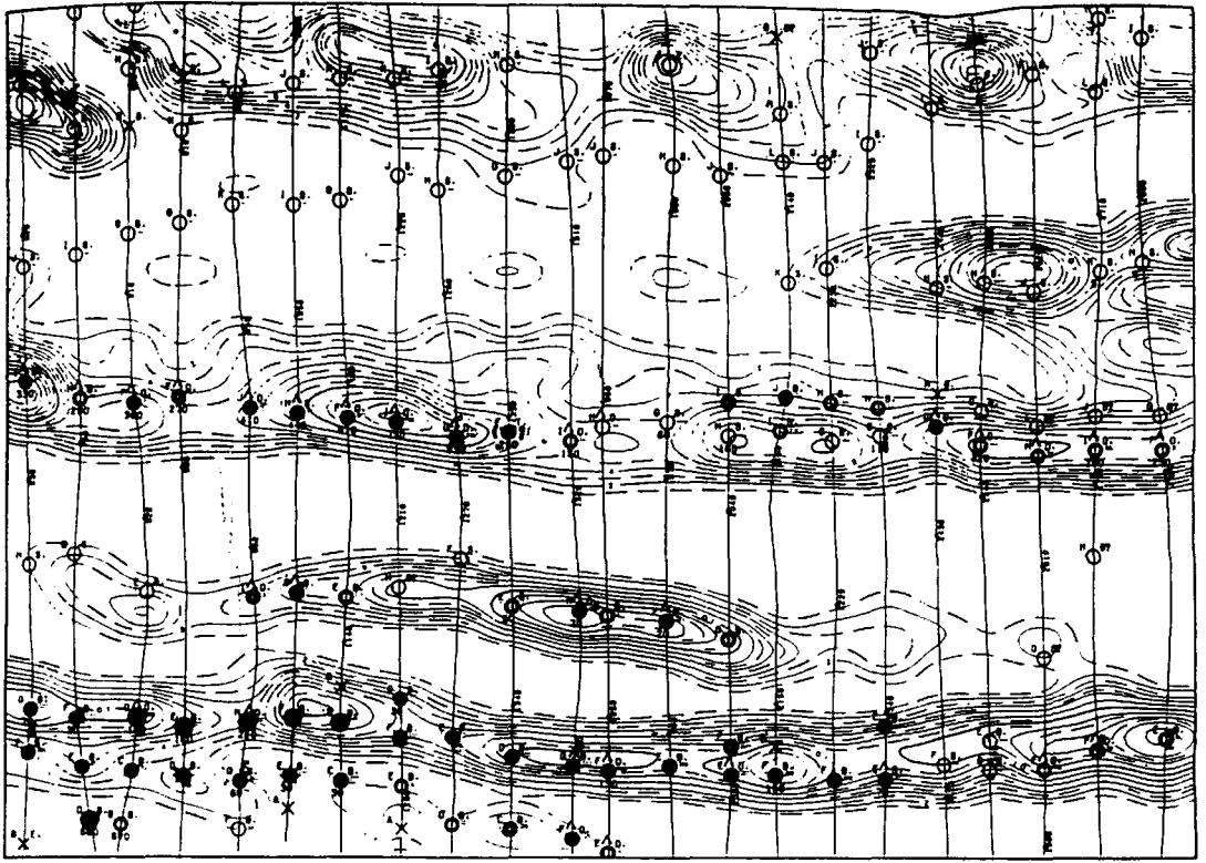
Figure 7.79. Total-field VLF contours from a Totem-2A survey near Utik Lake, Manitoba. Circles indicate conductors located by a helicopter phase-component survey. (After Herz, 1986.)
