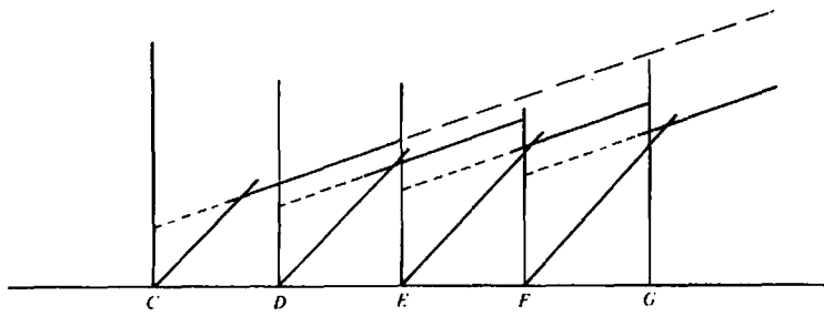
Figure 4.70. Unreversed refraction profiles for a single refractor, showing projections back to the intercept time (short dashes) and compositing for shot C by upward translation of segments of the curves.
