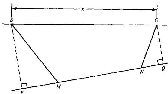
Figure 4.87. Illustrating delay time.
