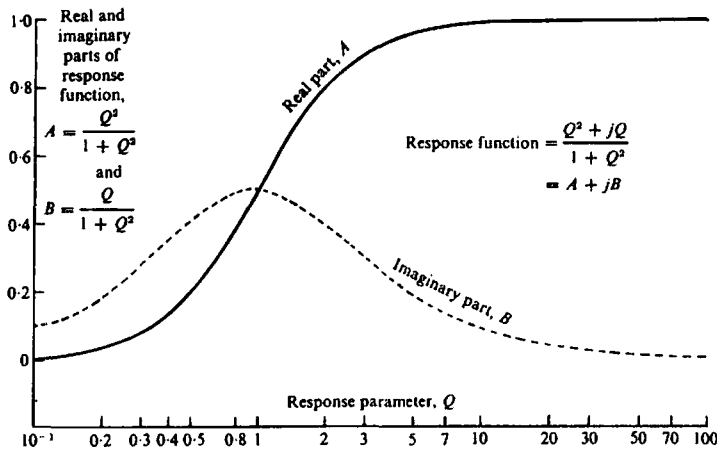
Figure 7.10. Response function of a conductor in an ac field. (After Grant and West, 1965).
