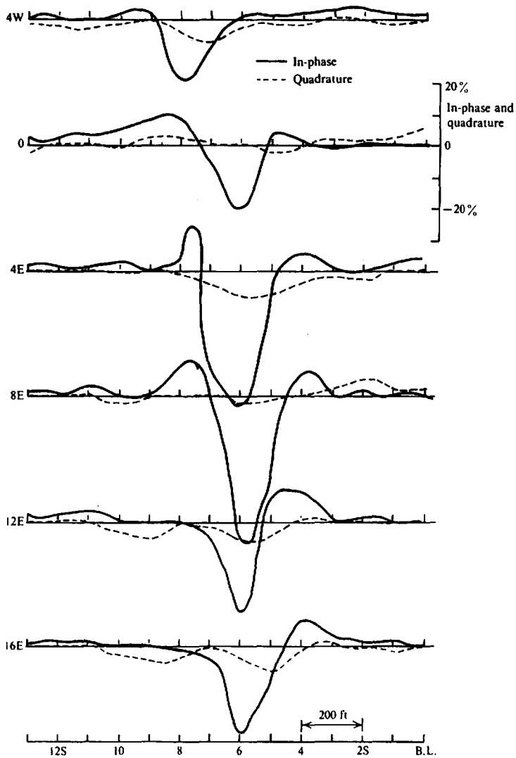
Figure 7.113. HLEM profiles, Chibougamau Area, Quebec.
