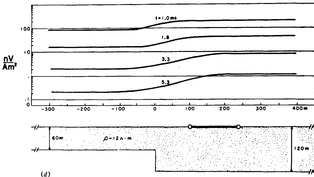
Figure 7.57. (Continued) (d) Coincident-loop traverse over step.
