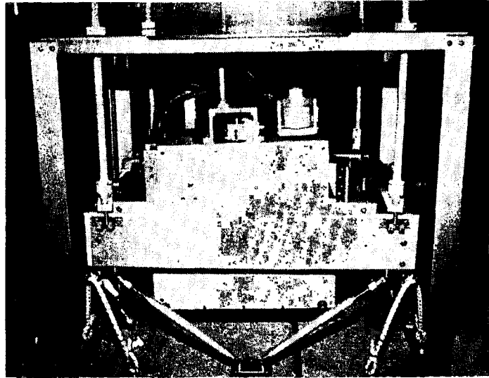
Figure 2.16. Photograph of a shipboard gravimeter.
