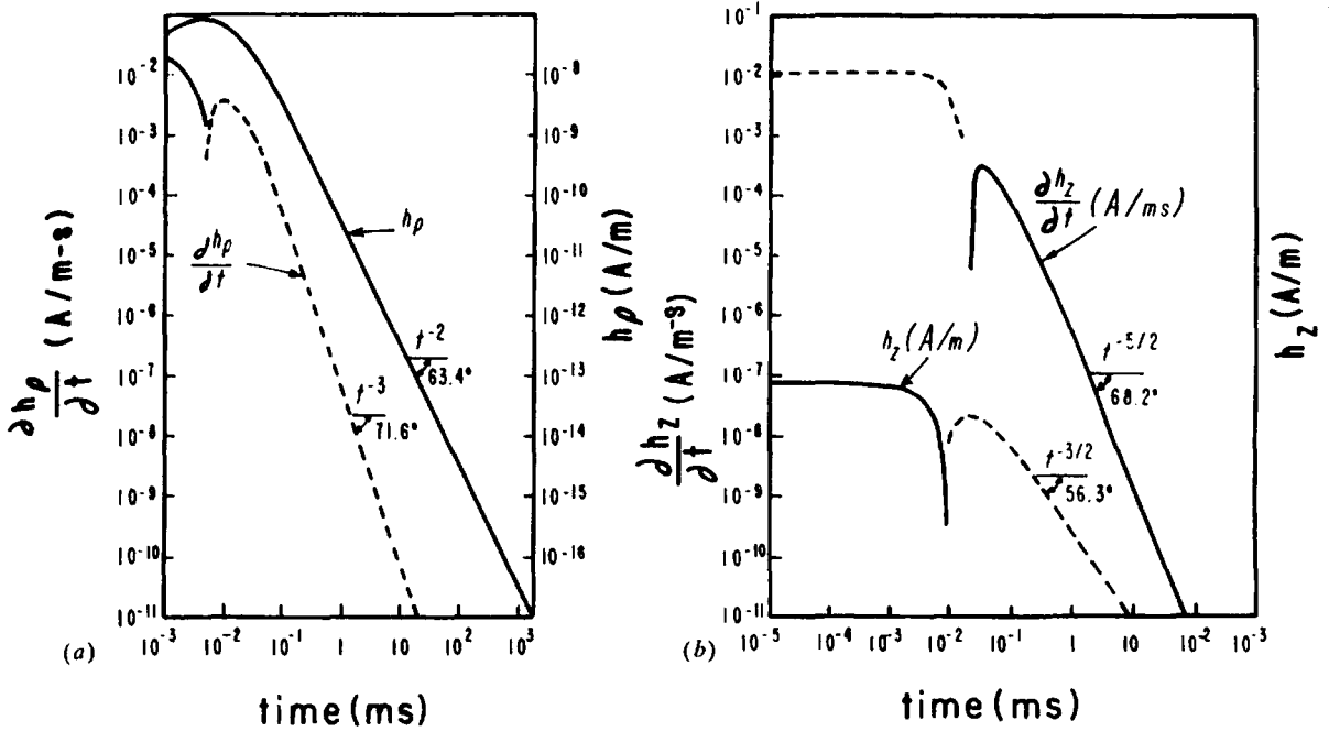
Figure 7.12. TD transient decay curves at a point 100 m from a vertical magnetic dipole on 100 \Omega m homogeneous earth. (From Ward and Hohmann, 1988.) (a) h_p and \partial h_p/\partial t . (b) h_z and \partial h_z/\partial t .
