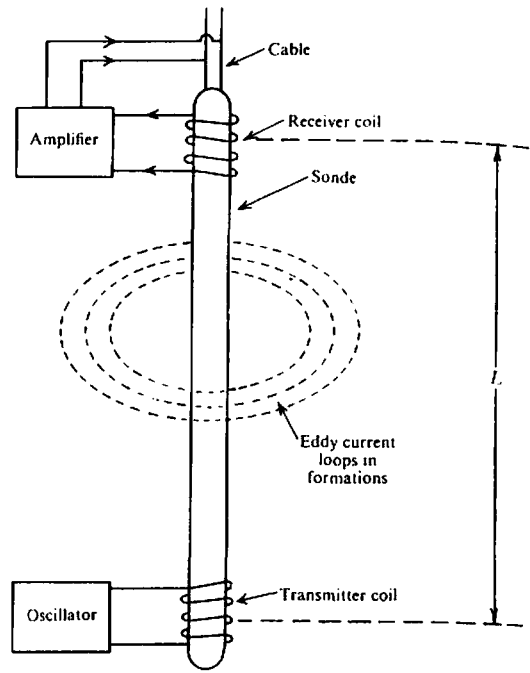
Figure 11.7. Induction log schematic. The tool itself is made of nonconducting material.
