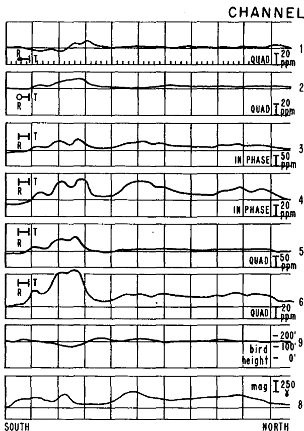
Figure 7.27. Dighem multicoil record over widespread conductors. (After Fraser, 1978.)
