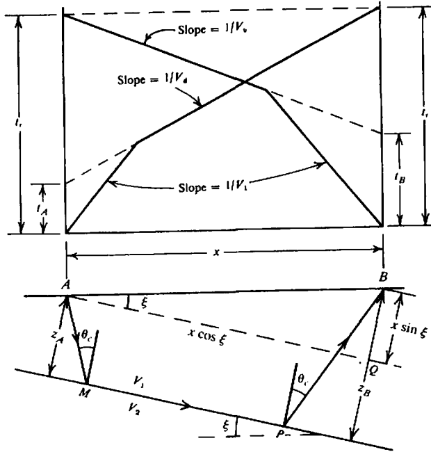
Figure 4.33. Raypaths and traveltimes for a dipping refractor.
