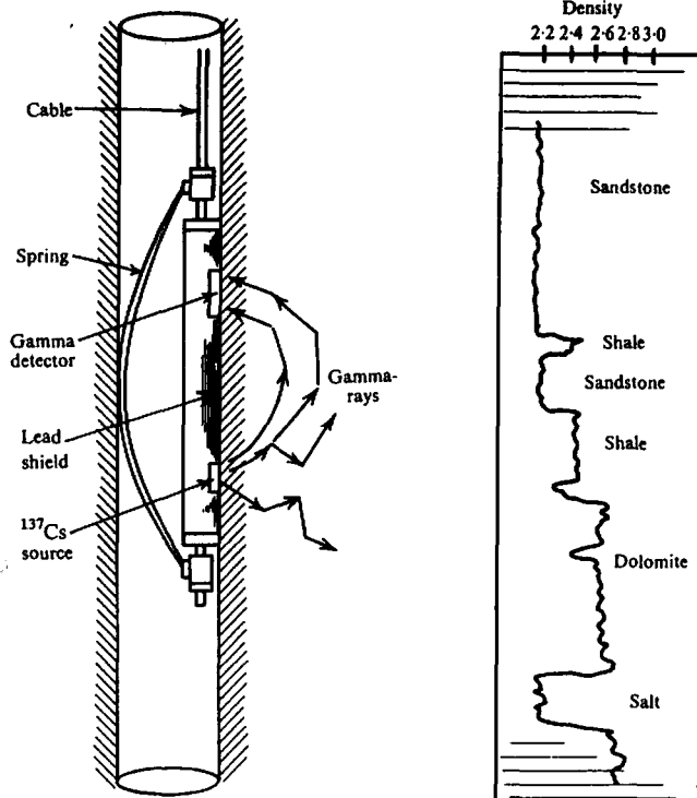
Figure 11.35. Density log schematic and typical log.
