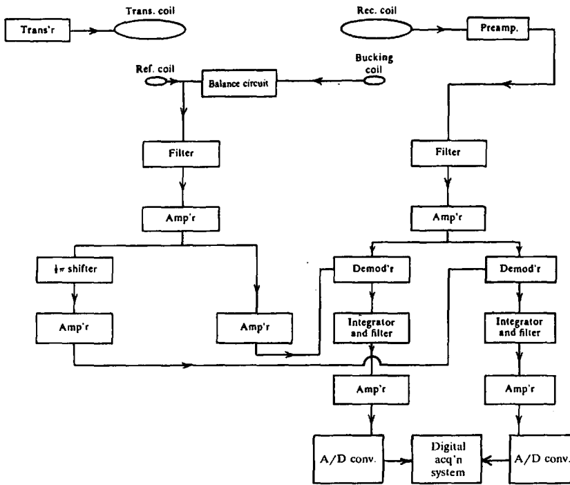
Figure 7.25. Block diagram of the airborne phase-component system. (From Keller and Frischknecht, 1966.)
