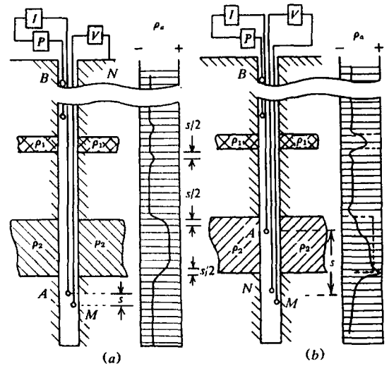
Figure 11.4. Electrode configurations and log curves; \rho_1 , \rho_2 indicate resistive beds. P is the power source, I is the ammeter, V is the voltmeter, s is the spacing. (a) Two-electrode (normal) arrangement. (b) Three-electrode (lateral) arrangement; the upper B electrode is on the cable sheath well above the sonde.
