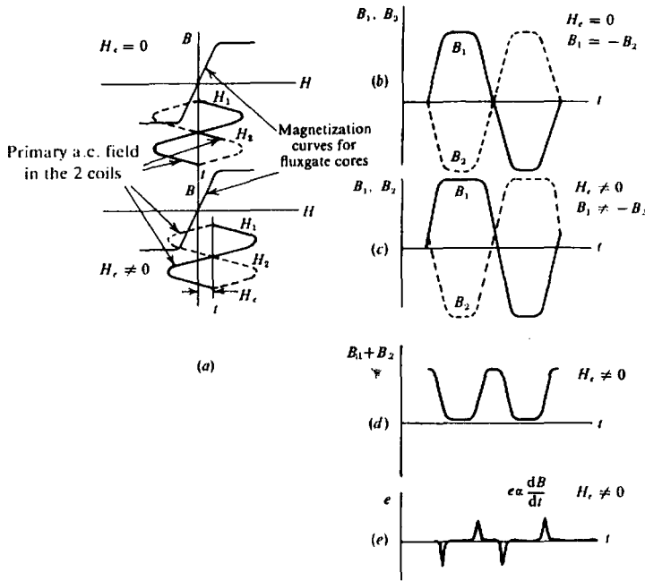
Figure 3.7. Principle of the fluxgate magnetometer. Note that H_e = F_e , etc. (From Whitham, 1960.) (a) Magnetization of the cores. (b) Flux in the two cores for F_e = 0 . (c) Flux in the two cores for F_e \neq 0 . (d) F_1 + F_2 for F_e \neq 0 . (e) Output voltage for F_e \neq 0 .
