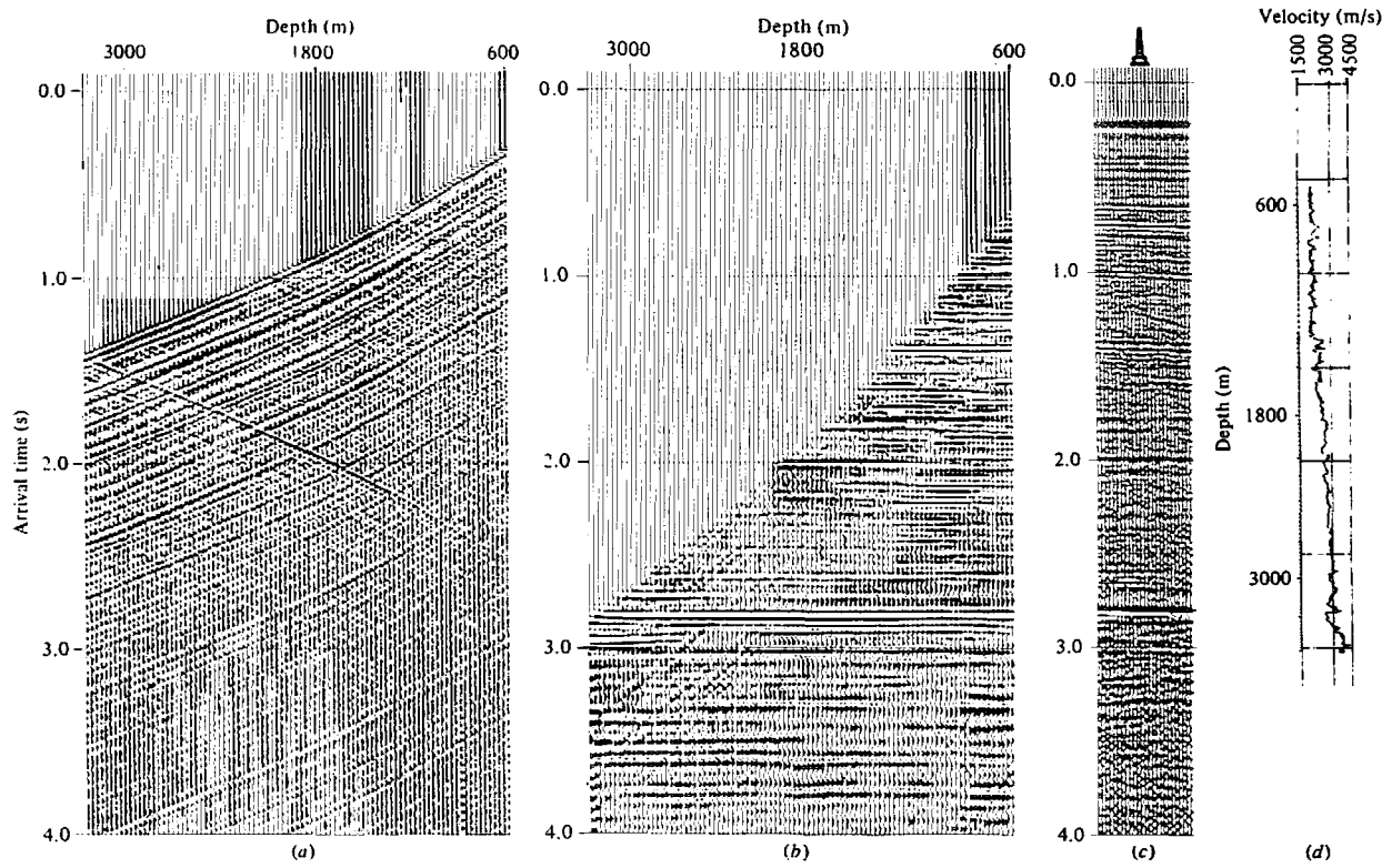
Figure 4.114. Vertical seismic profile. (Courtesy SSC.) (a) Each trace is recorded at a station in a borehole using an air gun source at the surface. (b) Same except each trace has been shifted by the one-way travelttime to the surface, thus aligning reflections (upcoming events) horizontally. (c) Portion of reflection record shot across the wellhead. (d) Sonic log in the well.
