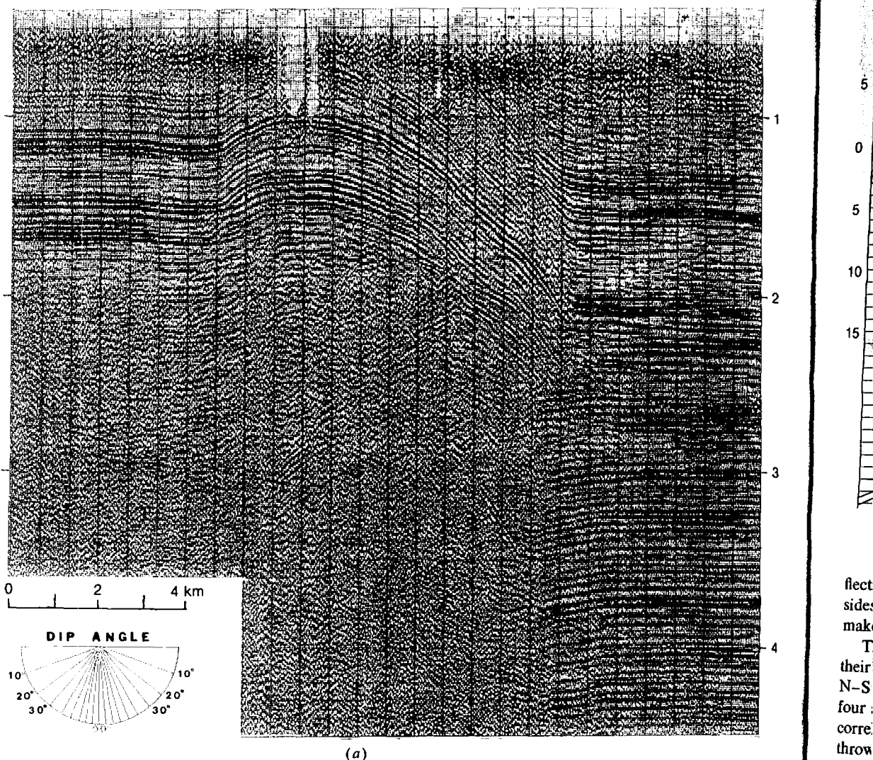
Figure 4.98. Section across a thrust fault in the Oregon Basin, part of the Big Horn Basin of Wyoming. (After Stone, 1985.) (a) Seismic section.
