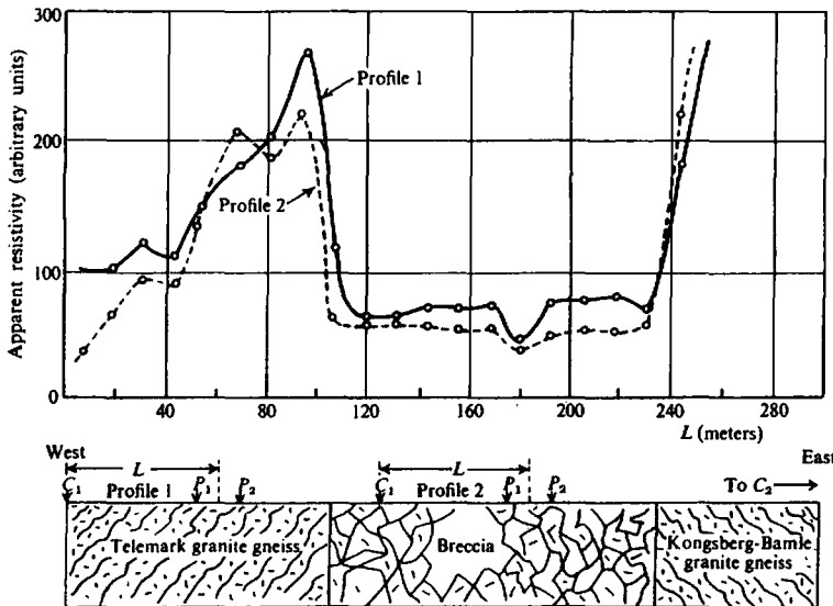
Figure 8.40. Mapping vertical contacts with the half-Schlumberger array, Kongsberg, Norway. (After Van Nostrand and Cook, 1966.)
