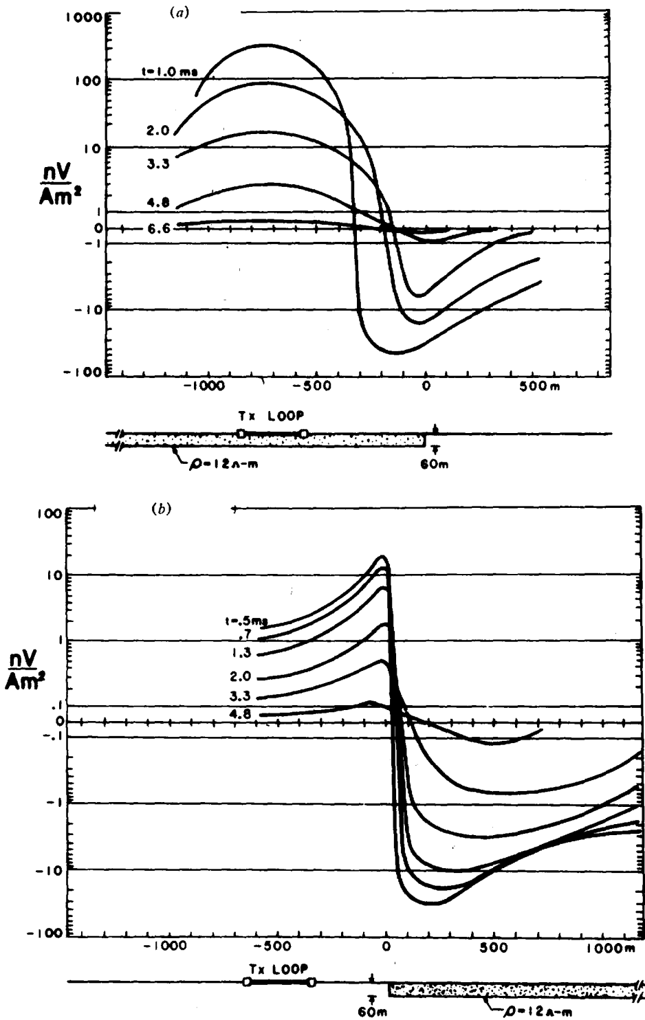
Figure 7.54. Comparison of responses of Turam-type (TDEM) and SIROTEM(1) over conductive overburden. Turam: Tx loop 600 \times 300 \text{ m} in (a), (b), and (c). (After Spies and Parker, 1984.) (a) Tx on overburden \sim 550 \text{ m} from edge. (b) Tx offset \sim 350 \text{ m} from edge.
