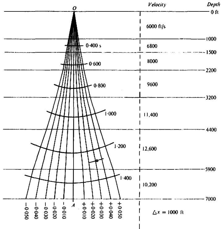
Figure 4.117. Simplified wavefront chart formerly used to plot cross sections on a transparent overlay. Chart shows rays traced through a series of constant-velocity layers for \Delta t_d values of 0, \pm 0.010, \dots, \pm 0.050 s, \Delta x = 1000 ft. Wavefronts are shown for t_0 = 0.4 to 1.4 s assuming that the rays are reflected upward along the downward paths. Plotted reflector is for t_0 = 1.28 s, \Delta t_d = 0.033 s.
