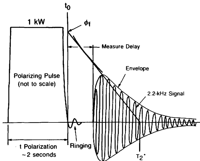
Figure 11.41. Nuclear-magnetic-resonance signal decay. Signals from resonances other than those of the free fluid decay before measurement begins. The signal decay is exponential so that the free-fluid index ( \phi_f ) can be found by extrapolating the log of the decay back to zero time. (After Pinnington, 1981.)
