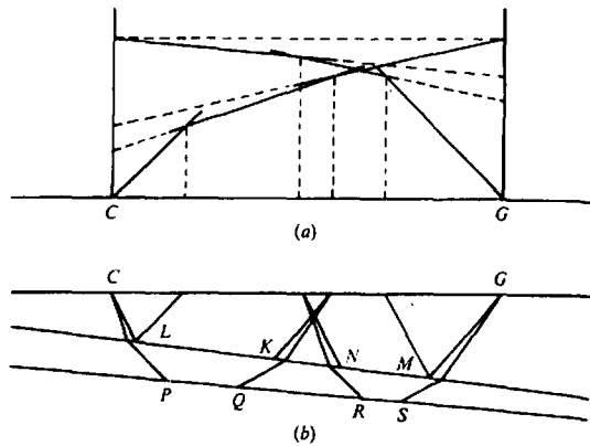
Figure 4.69. Reversed refraction profiles for two-refractor case. (a) Time-distance plot. (b) Section showing raypaths for two refractors.
