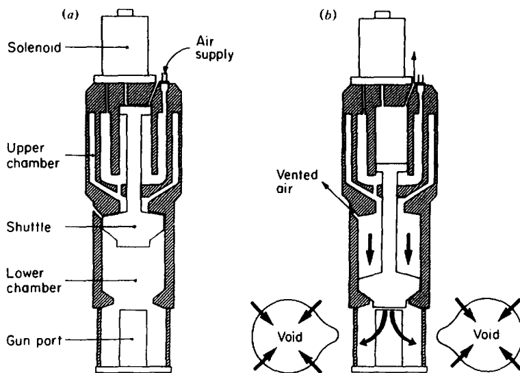
Figure 4.62. Water-gun schematic. (From Safar, 1985.) (a) At beginning of firing cycle. (b) At end of firing cycle.
