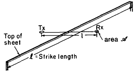
Figure 7.9. Coupling factor of horizontal-loop system over a long vertical sheet conductor.
