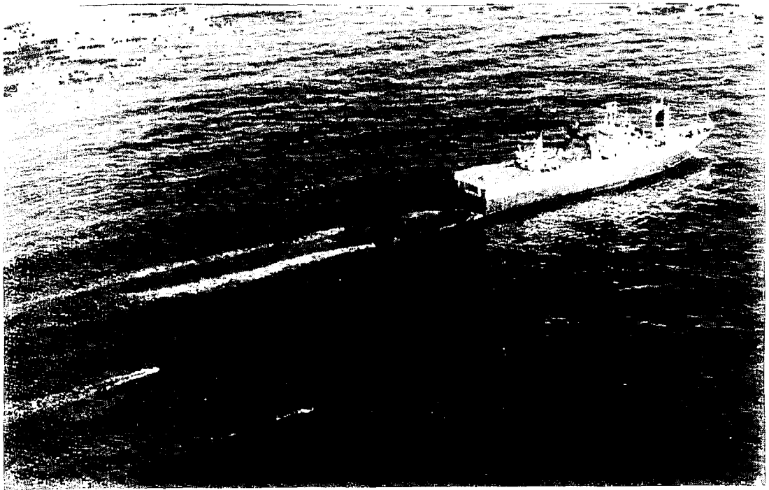
Figure 4.60. Seismic ship towing two streamers and two air-gun arrays. The outer wakes are produced by paravanes that pull streamers off to each side and the inner two wakes are produced by the two air-gun arrays. (Courtesy Western Geophysical Co.)
