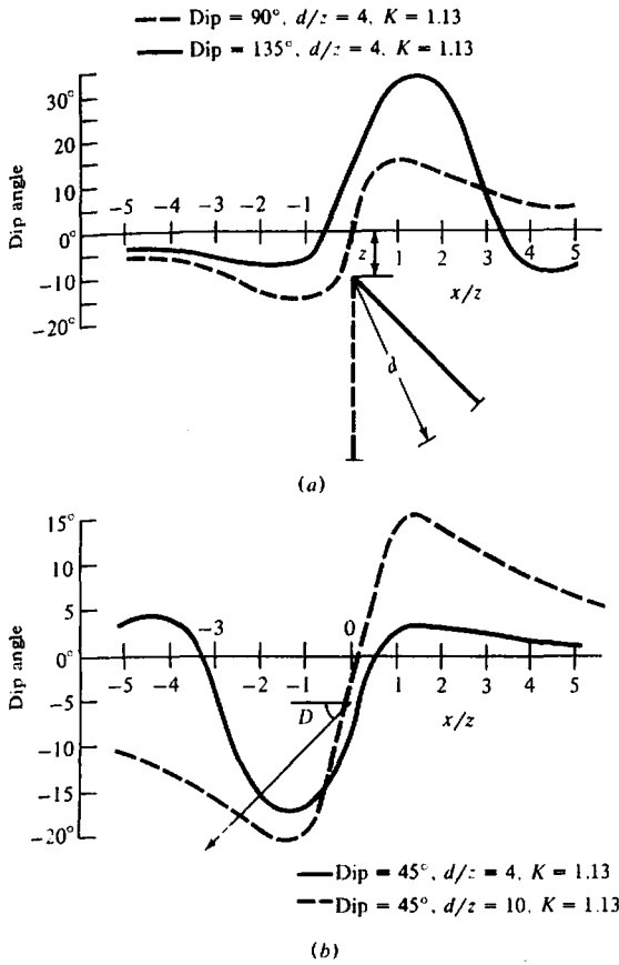
Figure 7.47. VLF profiles over dipping sheet obtained from ac circuit analysis. (a) Dip 90 and 135°, d/z = 4 . (b) Dip 45°, d/z = 4 and 10.
