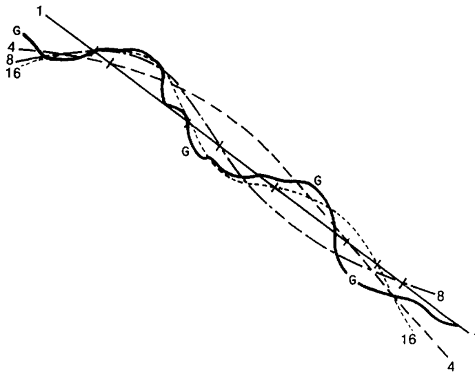
Figure 2.18. Illustrating least-squares surface-fitting. Curve G represents a gravity profile and curves 1, 4, 8, 16 represent fits of the respective orders. The surface fit, and hence the residual, depends on the dimensions that are fitted (from Nettleton, 1976).
