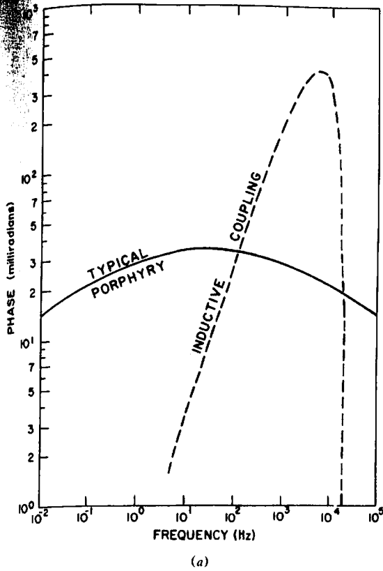
Figure 9.10. Phase-angle spectra and their use in removing EM coupling effects. Double-dipole array: n = 1 , x = 30 m. (After Pelton et al., 1978.) (a) Typical porphyry spectrum and EM coupling spectrum over homogeneous earth. (b) Observed data and curve (solid line) obtained using two Cole-Cole dispersion terms; dashed line is EM coupling spectrum calculated using the Cole-Cole parameters; the dash-dot line is the difference between the two previous curves.
