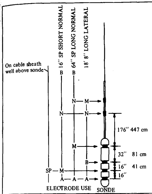
Figure 11.3. Showing how electrodes on a sonde can be used to record different electrical logs. A and B are current electrodes, M and N are potential electrodes. (After Labo, 1987.)
