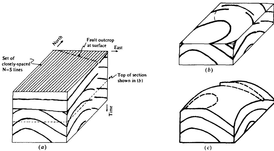
Figure 4.112. Three-dimensional data obtained from a set of closely spaced N-S lines. (a) Isometric diagram of the volume these data occupy. The easternmost N-S section is shown along with an E-W section made from the southernmost traces on each N-S line. (b) The data set with the top portion removed. The top now constitutes a time-slice. (c) The data sliced along one reflection constitutes a horizon-slice. Such maps show reflectivity variations along the same horizon such as may indicate stratigraphic or fluid-content changes.
