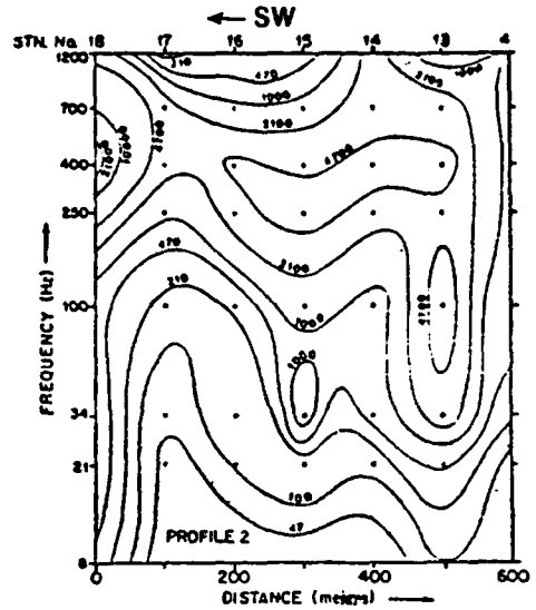
Profile 2 pseudo-section.
