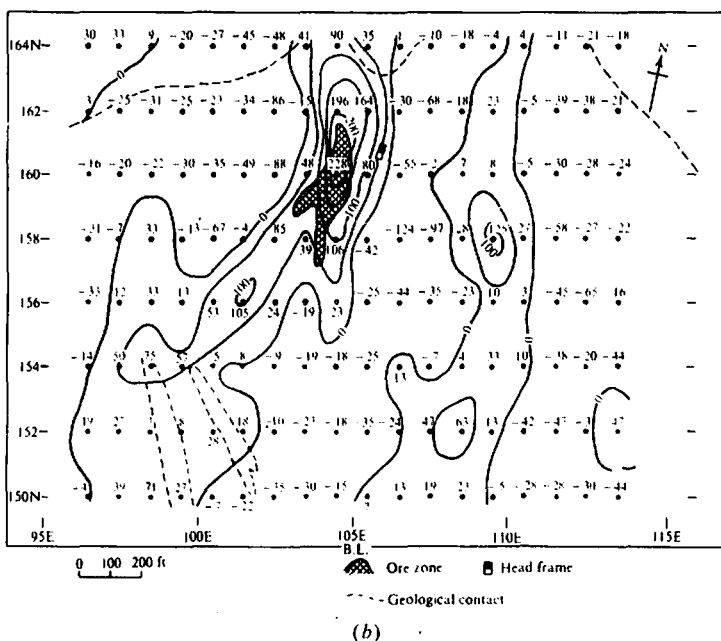
Figure 7.96. Results of VLF survey, Atlantic Nickel property, southern New Brunswick. Transmitter station: Cutler, Maine (24.0 kHz). (a) VLF profiles. (b) VLF contours.
