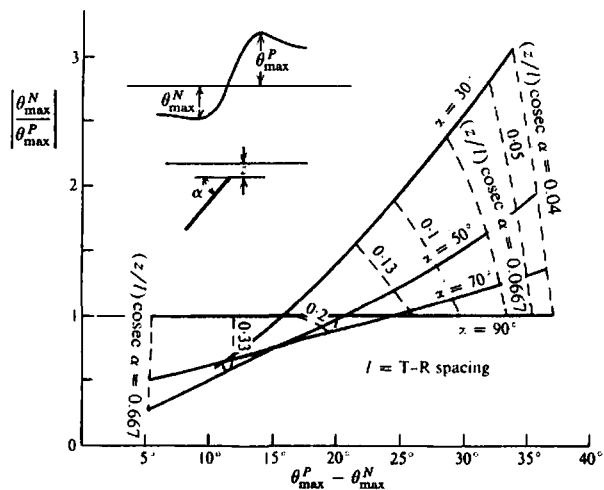
Figure 7.42. Characteristic curves for semiinfinite dipping-sheet conductor. (a) Depth to the top of a steeply dipping sheet from the crossover slope and peak tilt. Broadside array. (From Ward, 1967.) (b) Depth and dip using fixed-transmitter, dip-angle system. (From Grant and West, 1965.)
