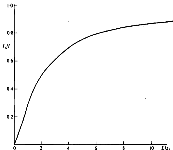
Figure 8.7. Fraction of current flowing below depth z_1 for an electrode spacing L .
