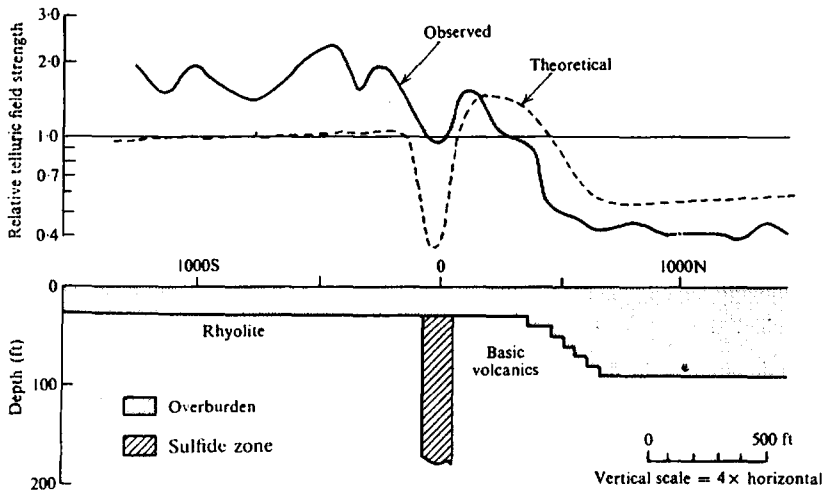
Figure 12.4. Telluric profile and geologic section, Mobern Sulfide Deposit, northwestern Quebec. For theoretical model, \rho_{sul} = 1 \Omega m , \rho_{over} = 70 \Omega m , and \rho_{host} = 7,000 \Omega m .
