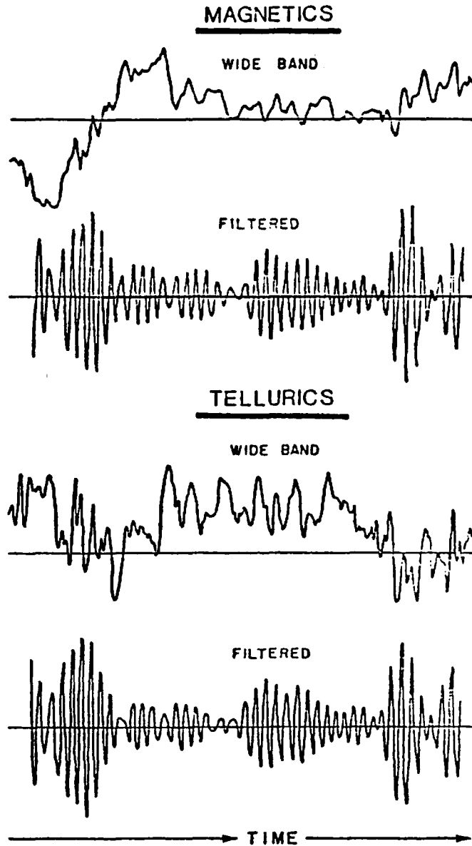
Figure 6.10. Magnetic and telluric field data before and after filtering.
