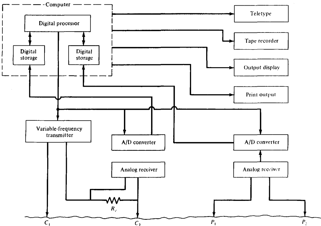
Figure 9.7. Block diagram of complex-resistivity system with double-dipole array. (After Sumner, 1979.)
