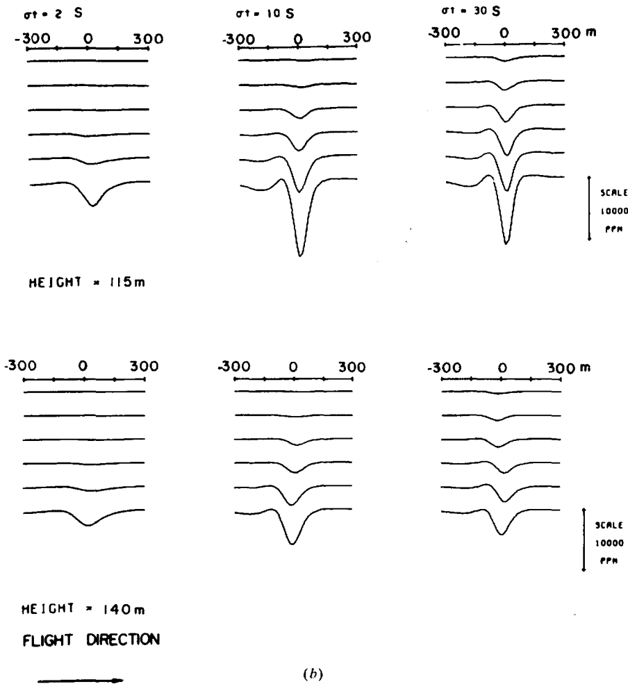
Figure 7.87. (Continued) (b) Six-channel response for two flight heights and several values of \sigma t ; the top of the sheet is at zero height. (After Palacky and West, 1973.)
