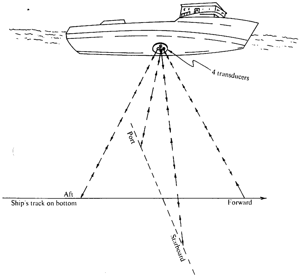
Figure B.3. Doppler-sonar navigation. (From Sheriff, 1984.)
