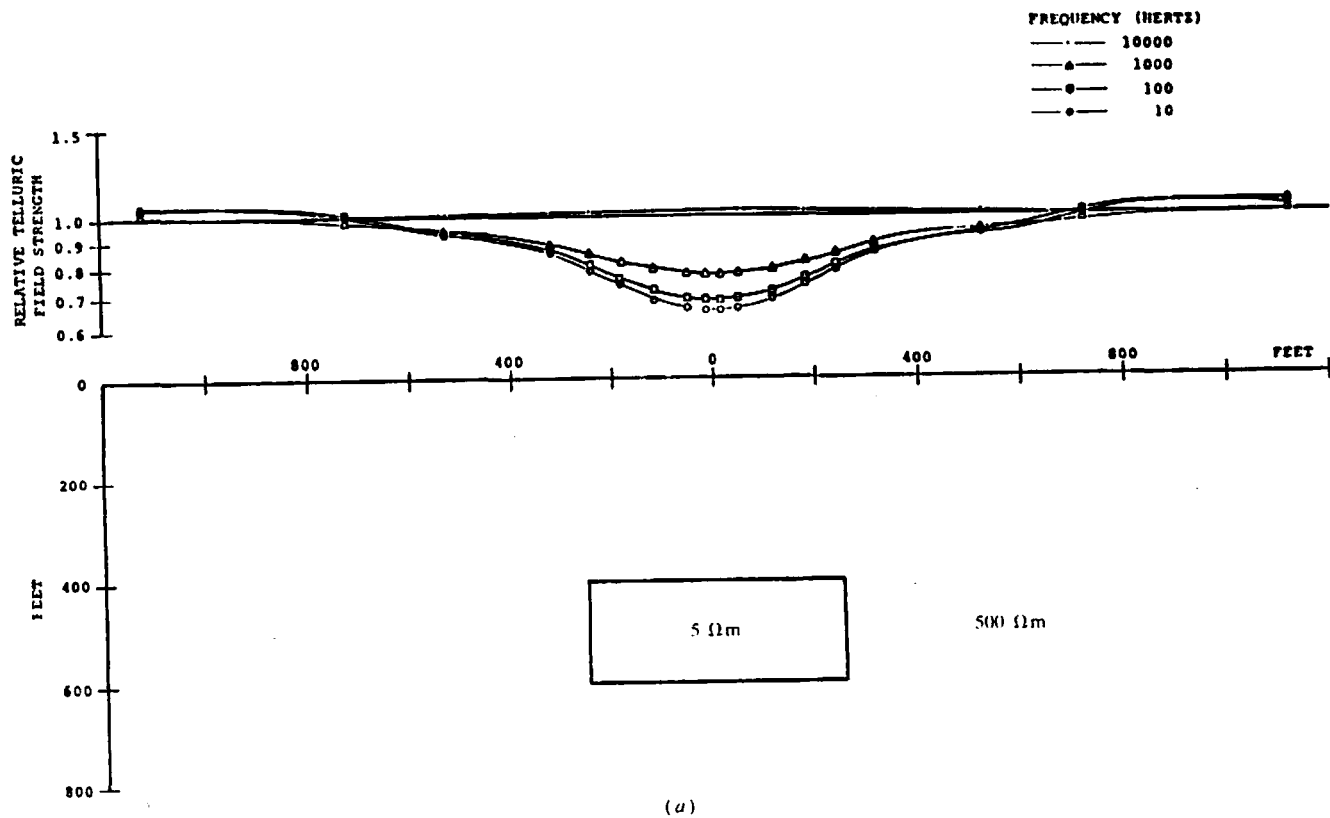
Figure 6.20. Theoretical amplitude and phase curves for a deeply buried slab. (a) Amplitude profiles.
