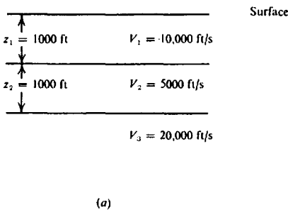
Figure 4.121. Two different geologic sections that give the same refraction time-distance curve.
