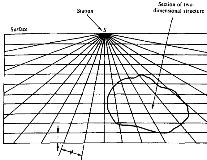
Figure 2.33. Template for calculating the gravity effect of two-dimensional bodies of irregular cross section. (From Hubbert, 1948).
