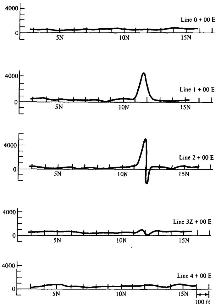
Figure 3.38. Vertical-component magnetic profiles, Rouyn-Noranda district, Quebec.
