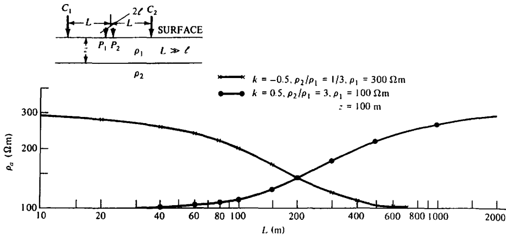
Figure 8.20. Plots of \rho_a versus L over two horizontal beds for a Schlumberger expanding spread. Curves were calculated from Equation (8.39b).
