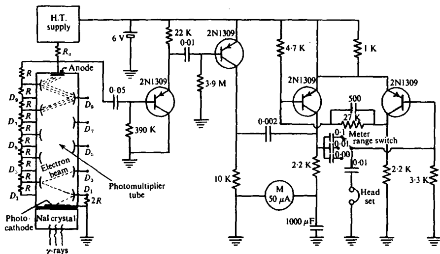
Figure 10.5. Scintillation-meter schematic.
