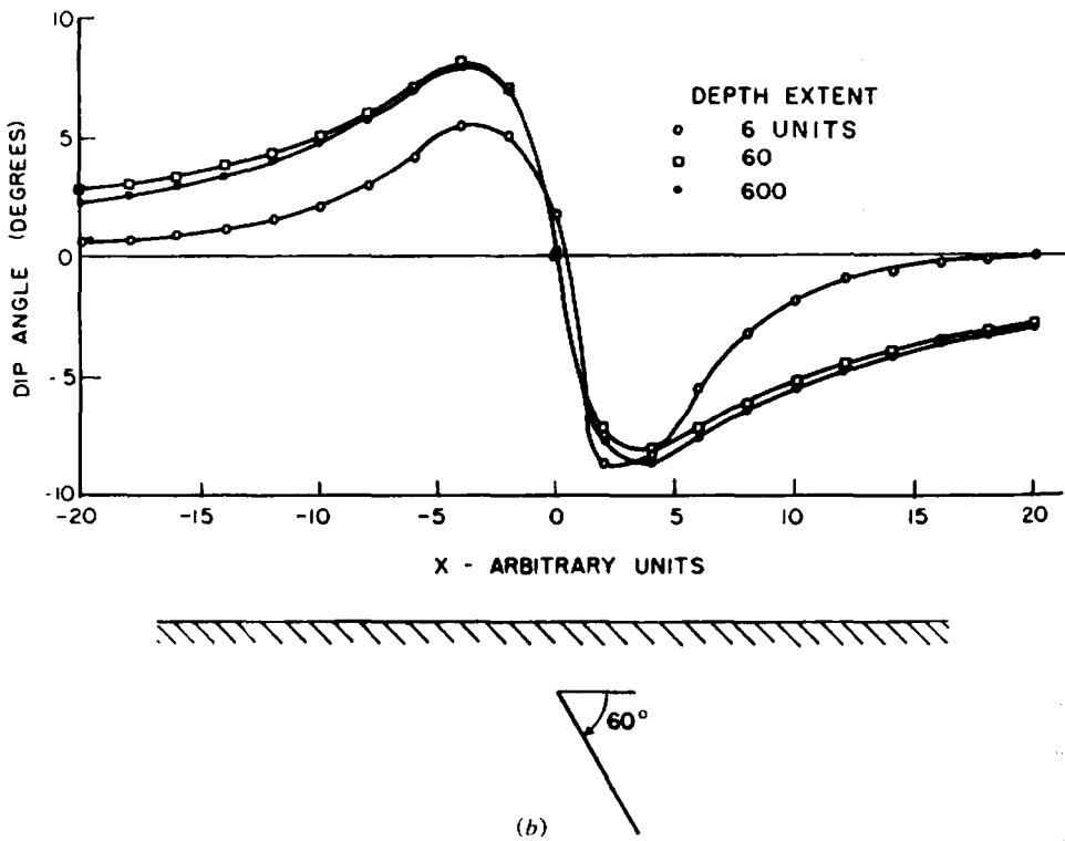
Figure 7.34. Variations of AFMAG profiles with different parameters. (After Ward, 1967.) (a) Effect of dip (b) Effect of depth extent
