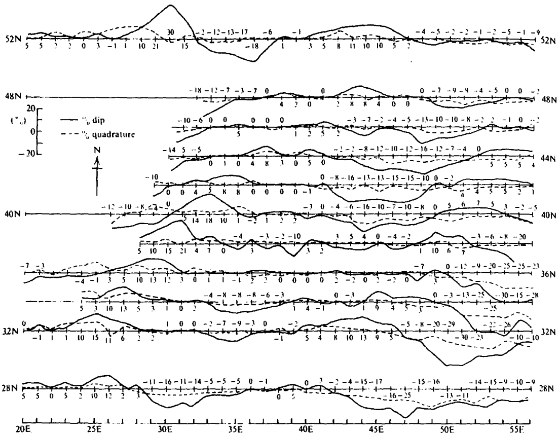
Figure 7.109. EM16 survey in eastern Nova Scotia.
