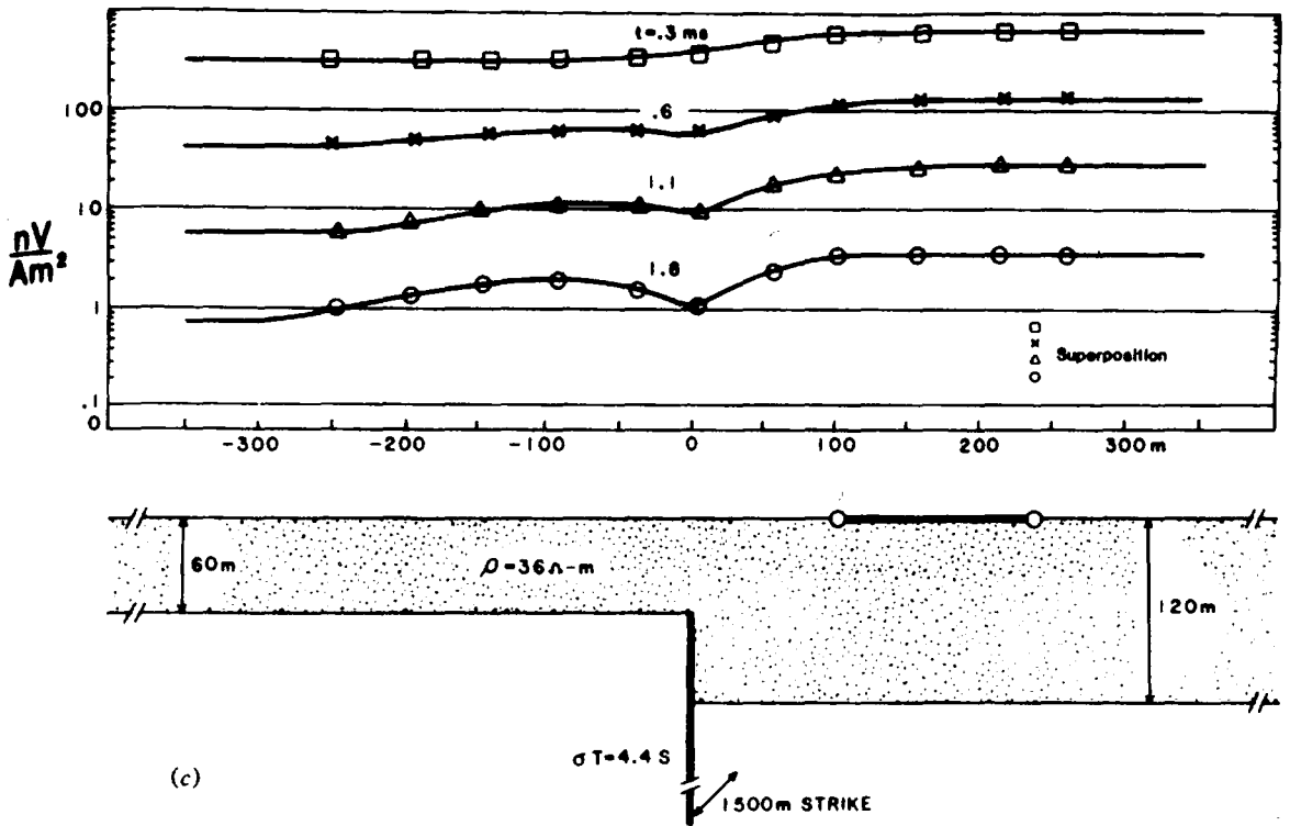
Figure 7.59. (Continued) (c) Coincident-loop traverse across the step.
