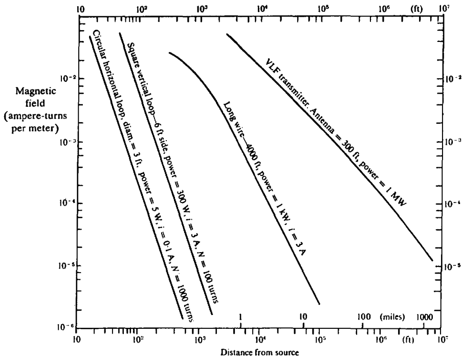
Figure 7.5. Comparison of magnetic fields produced by various sources.
