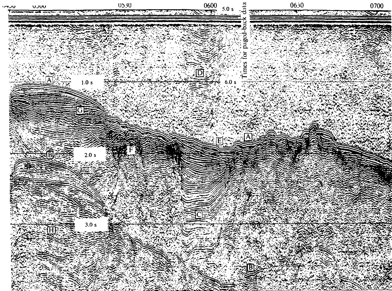
Figure 4.109. Profiler record offshore Japan. The water-bottom reflection (A) with traveltimes of 1.0 to 2.0 s indicates water depths of 750 to 1,500 m. The ship traveled 8,500 m between the 30 min marks shown at the top of the record. Most primary reflections are obscured below the water-bottom multiple (B) and subsequent multiples. Over 1,000 m of sediments are indicated in the vicinity of C; multiples of these appear paged-back at D. E indicates a fault scarp on the ocean floor. F are diffractions, probably from sea-floor relief slightly offset to the line. Note the onlap and thinning above G. H is a second multiple of the ocean floor. (Courtesy Teledyne.)
