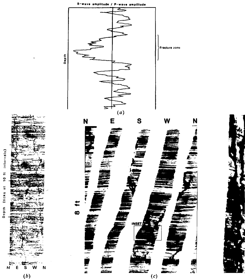
Figure 11.29. Fracture detection. (a) Fracture finder log showing low 5-wave/P-wave amplitudes in a fractured zone. (After Labo, 1987.) (b) Fracture seen by a borehole televiewer. (Courtesy Gearhart Industries.) (c) Formation microscanner showing fractures. The microscanner uses a number of electrodes on each of four pads pressed against the borehole walls to give four swaths of closely spaced electric log responses. The sonde was twisting somewhat during this log run. (Courtesy Schlumberger.)
