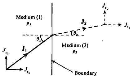
Figure 8.8. Distortion of current flow at a plane boundary when \rho_1 < \rho_2 .
