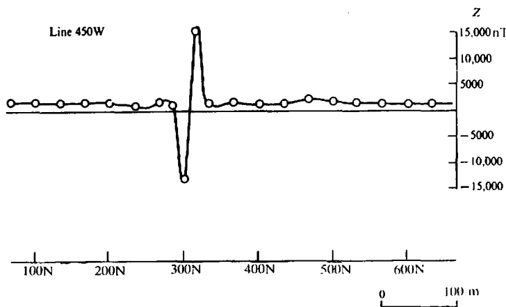
Figure 3.35. Vertical-component ground magnetic profile, East Africa.
