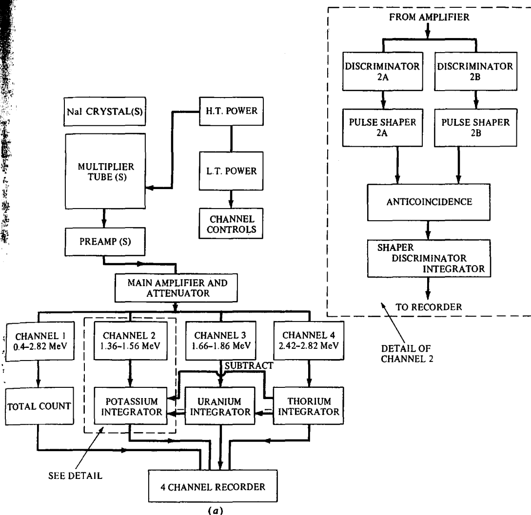
Figure 10.8. Four-channel \gamma -ray spectrometer. (a) Block diagram.
