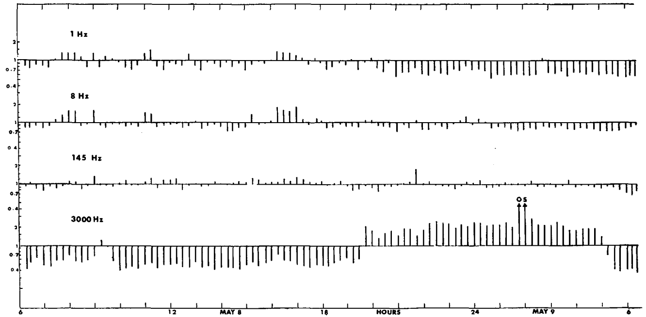
Figure 6.11. Telluric response, Vale Perkins, Quebec, May 8-9, 1975. Electrodes are north-south.
