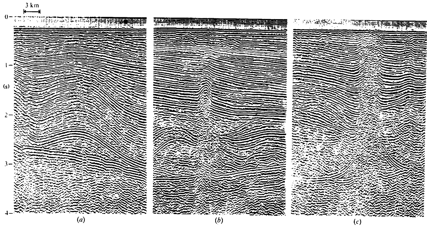
Figure 4.102. Portions of horizontally compressed sections in the North Sea. (Courtesy Grant-Norpac.) (a) Deep salt swell. (b) Salt dome that has pierced some of the sediments. (c) Salt dome that has pierced to the sea floor.
