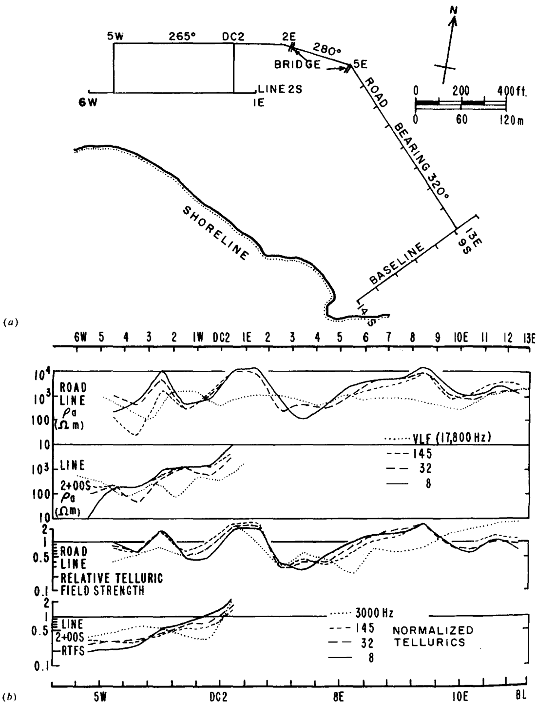
Figure 6.38. Telluric, MT, and VLF results. Canadian east coast. (a) Plan of survey area. (b) Top two sets of curves: \rho_a profiles from MT and VLF (EM16R) measurements; bottom two sets: relative telluric field strength (RTFS) profiles.
