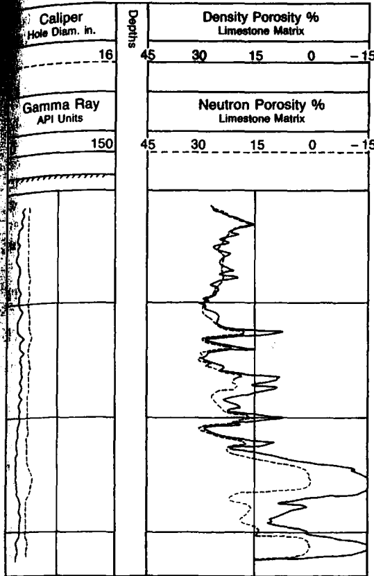
Figure 11.39. Portion of a dual-porosity neutron log. (From Schlumberger, 1987.)
