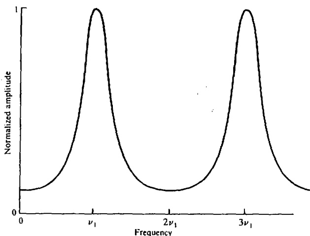
Figure 4.118. Spectrum of water-layer filter for water-bottom reflection coefficient of 0.5. If h = water depth and V = water velocity, \nu_1 = V/2h .
