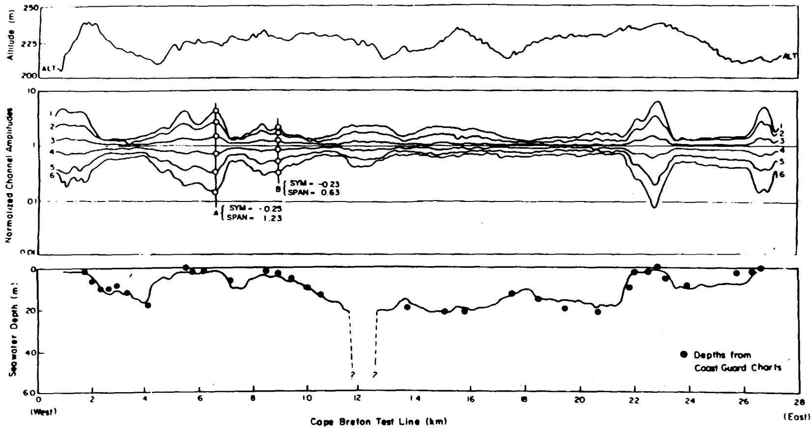
Figure 7.93. Bathymetry survey off the Canadian east coast using the Input system. (After Zollinger et al., 1987.) (a) Comparison of Input calculated depths and coastal charts, offshore Nova Scotia.
