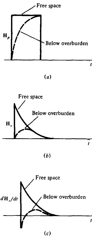
Figure 7.51. Effect of overburden (ob) on TDEM fields. (a) Primary field at target. (b) Secondary field at target. (c) Receiver response from target.
