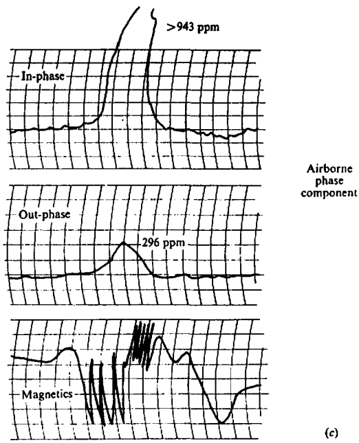
Figure 7.107. (Continued) (c) Phase-component EM and aeromagnetics. (From Ward, 1966.)
