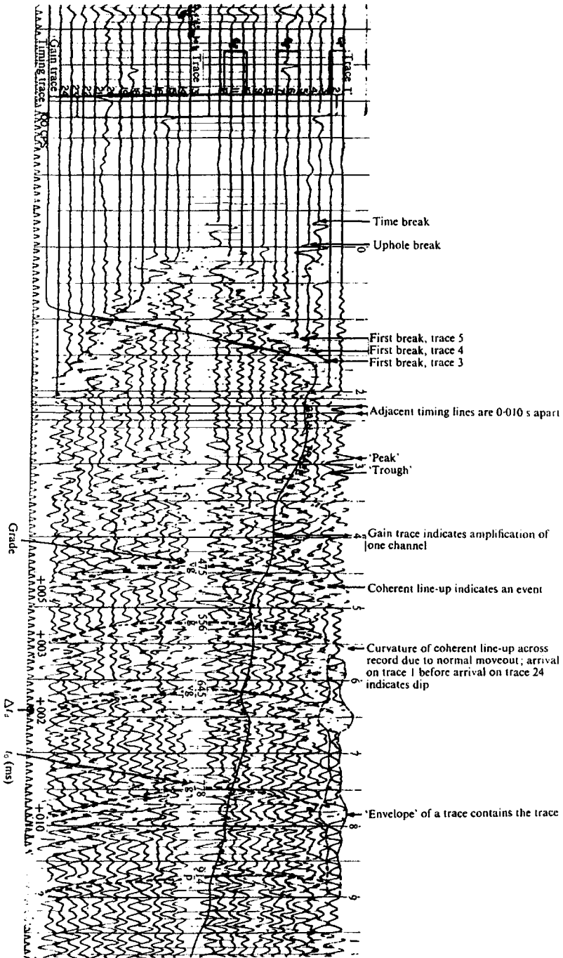
Figure 4.1. 24-trace seismic record for 12 geophone groups on either side of the sourcepoint. The trace spacing is 50 m, the heavy timing lines are 0.1 s apart, and the finer timing lines 0.01 s apart. Traces 12 and 13 are 50 m from the shotpoint. (Courtesy Chevron Oil Co.)
