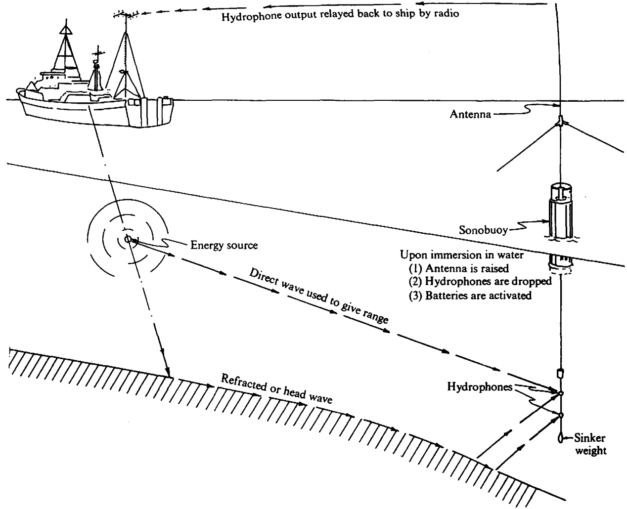
Figure 4.73. Sonobuoy operation.
