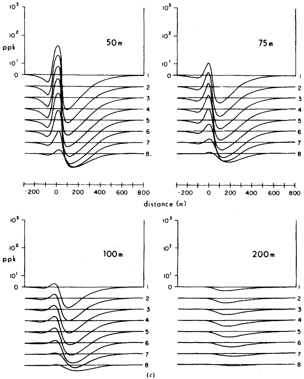
Figure 7.50. (Continued) (c) Same as (b) except dip = 30°.
