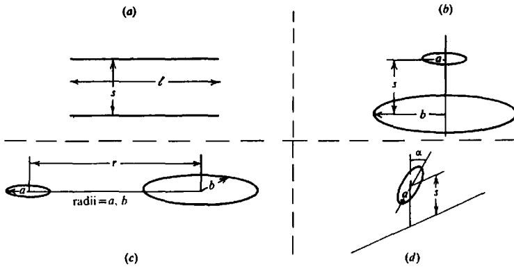
Figure 7.8. Calculating mutual inductance of various geometrical figures. (a) Two parallel straight lines. (b) Coaxial circles. (c) Coplanar circles. (d) Circle and long straight wire.
