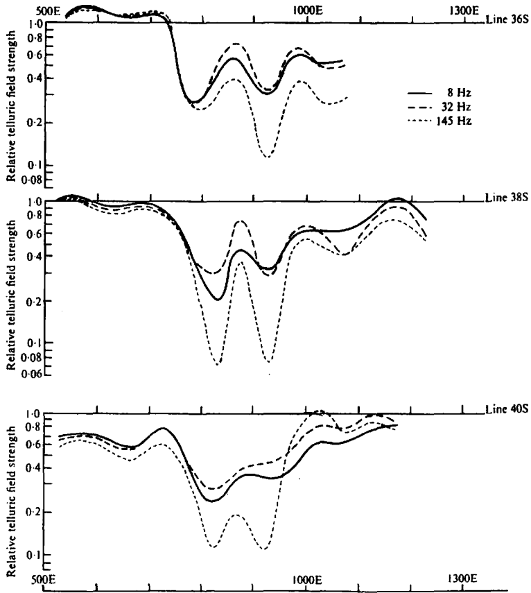
Figure 6.34. Multifrequency telluric profiles from Southeastern Quebec. Electrode spacing 50 ft.
