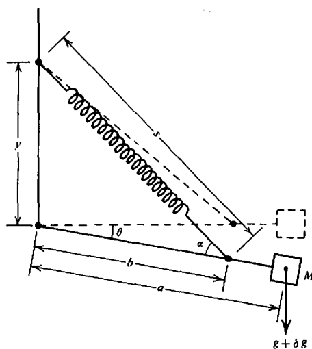
Figure 2.12. Lacoste–Romberg gravimeter.
