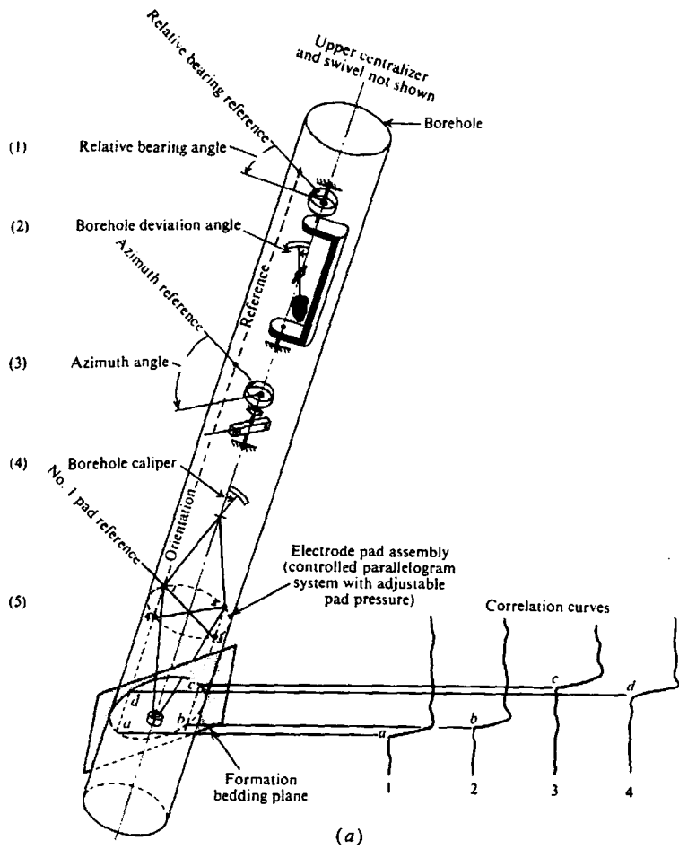
Figure 11.16. The dipmeter. (a) Schematic of diplog tool. (Courtesy Dresser Industries.) (b) Portion of a four-arm processed dipmeter log showing deviation of the hole, caliper log, smoothed resistivity, tadpole plot of dips, rosettes (each showing directions of all dips within a 10 ft. interval), and output of the four microresistivity pads with computer-drawn correlations. (Courtesy Schlumberger Ltd.)
