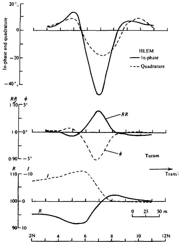
Figure 7.115. HLEM and Turam profiles, northern Quebec.
