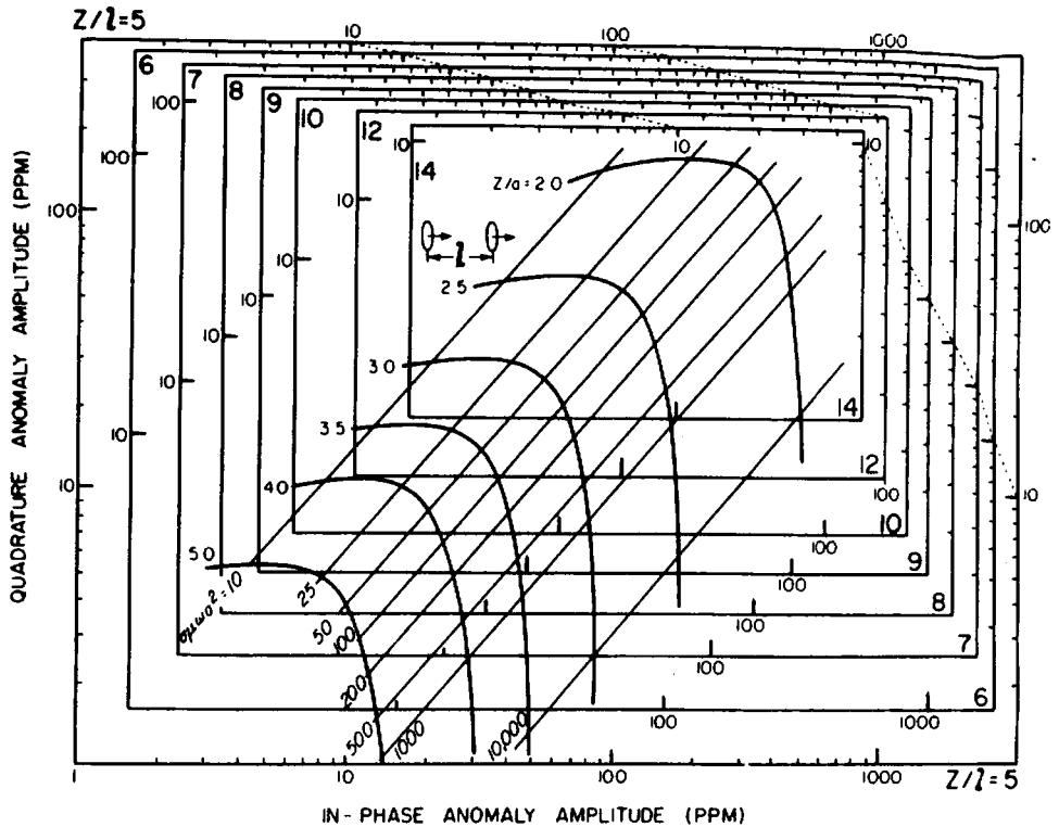
Figure 7.82. Interpretation diagram for a vertical coaxial-coil AEM system over a spherical conductor of radius a for z/l = 5, 6, 7, 8, 9, 10, 12, and 14; l = T-R . (After Lodha and West, 1976.)
