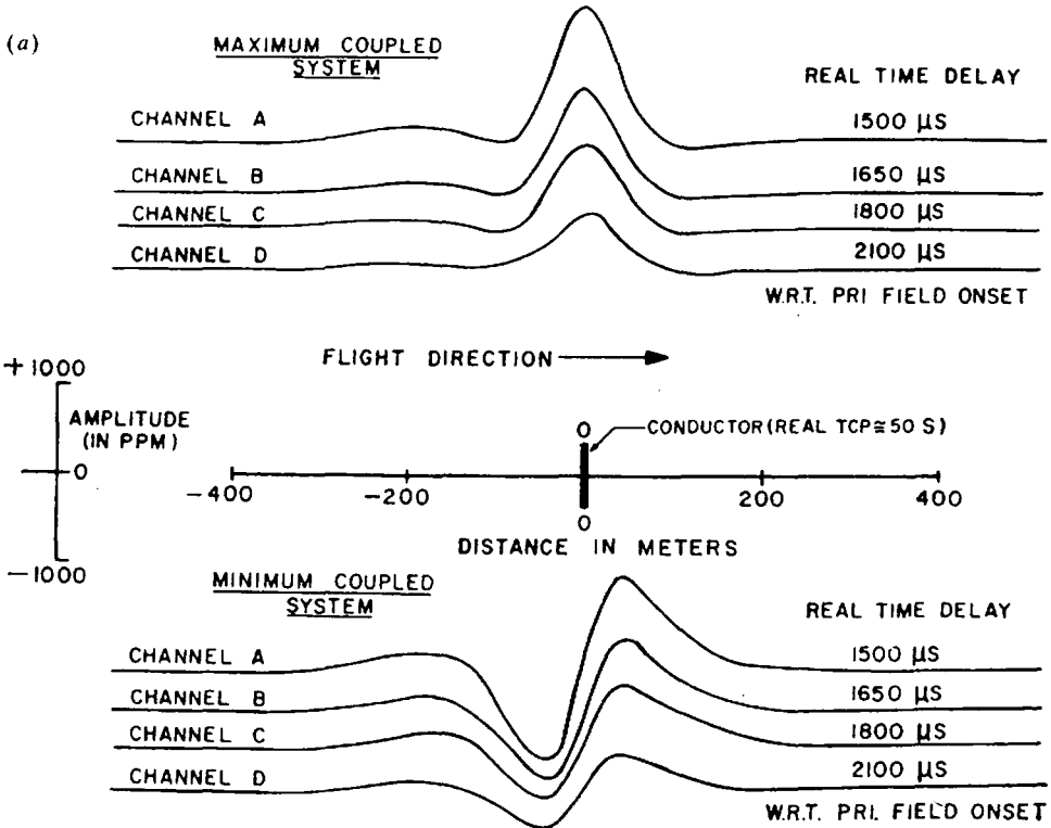
Figure 7.87. Model input response to a thin vertical sheet. (a) Four-channel response for maximum- and minimum-coupled systems for various values of the real-time delay. (After Becker, Gavreau, and Collet, 1972.)
