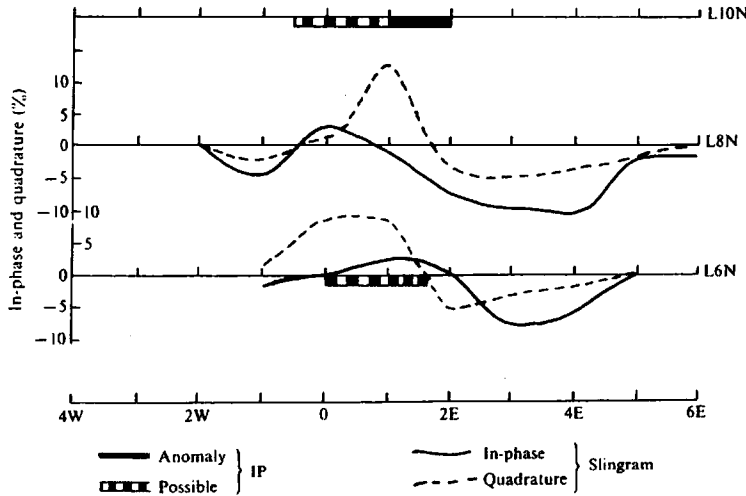
Figure 12.14. Slingram and IP results, northern New Brunswick. EM frequency 876 Hz, T-R separation 200 ft.
