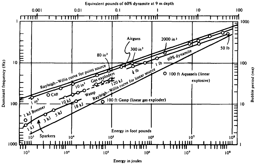
Figure 4.63. Energy-frequency relationships for marine sources at 10 m depth. (From Kramer, Peterson, and Walter, 1968.)
