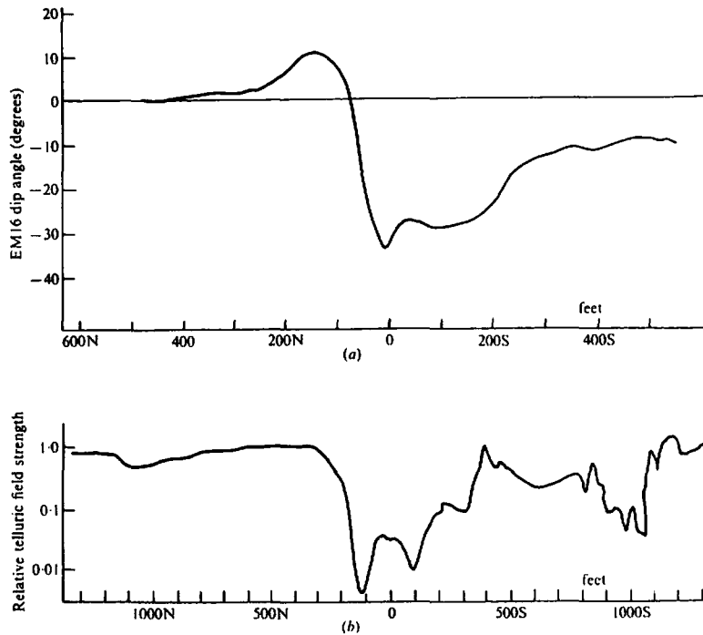
Figure 12.7. EM and telluric results, Bartouille, northwestern Quebec. (a) VLF-EM16 dip-angle profile. (b) Telluric profile, electrode spacing 25 ft.
