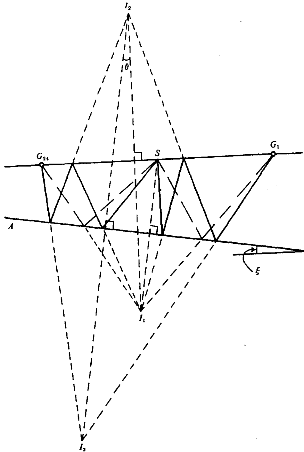
Figure 4.42. Raypath of a multiple from a dipping bed.
