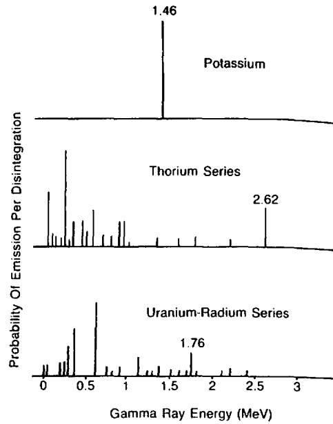
Figure 11.31. Gamma-ray spectra of potassium and the thorium and uranium series. (From Schlumberger, 1987.)
