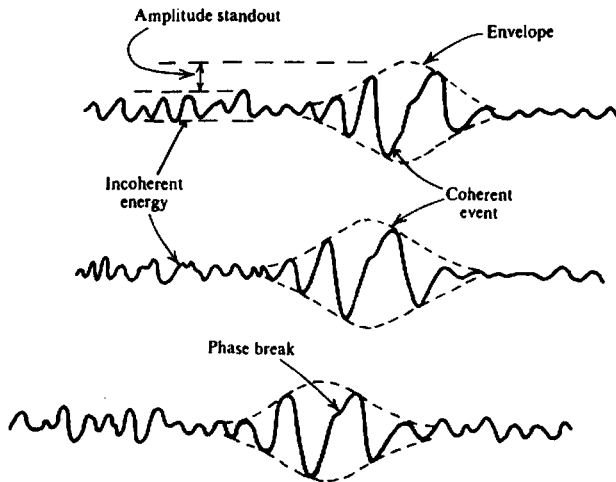
Figure 4.34. Characteristics of seismic events.
