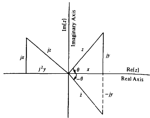
Figure A.5. Plotting complex quantities in the complex plane.
