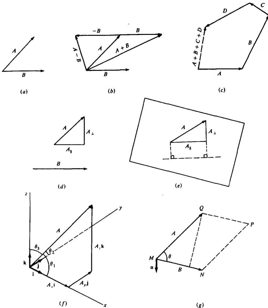
Figure A.1. Various operations on vectors. (a) Two vectors to be added or subtracted. (b) Addition and subtraction of vectors in (a). (c) Summing several vectors. (d) Resolving A into components parallel to and perpendicular to B . (e) Resolving A into components parallel to and perpendicular to a plane. (f) Resolving A into rectangular components. (g) Illustrating the products A \cdot B and A \times B .
