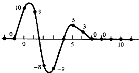
Figure 4.124. A minimum-phase wavelet.
