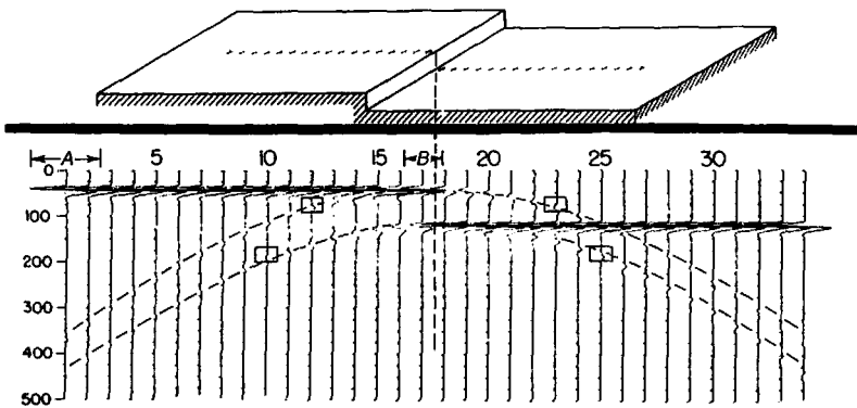
Figure 4.38. Reflection and diffraction response of a step for sources and receivers coincident. (After Hilterman, 1970.)
