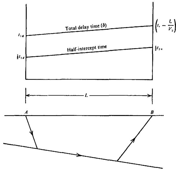
Figure 4.119. Demonstrating the parallelism of total-delay and half-intercept time curves.
