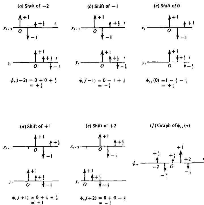
Figure 4.80. Calculating the cross-correlation of two functions.
