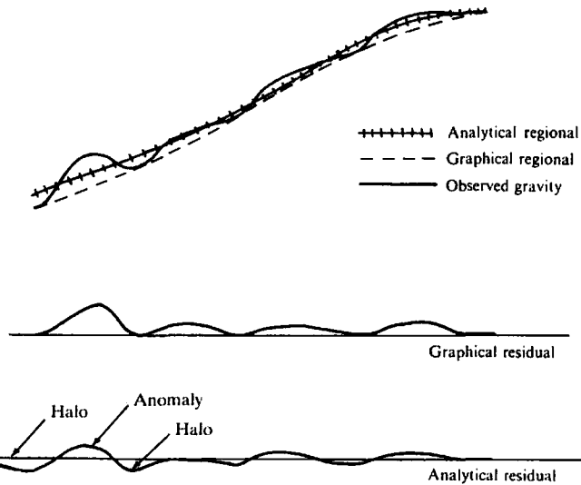
Figure 2.21. Comparison of graphical and analytical methods of removing regional gravity.
