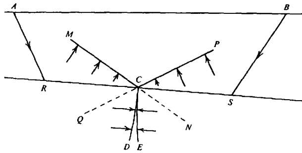
Figure 4.93. Determining refractor position from wavefront intersections.
