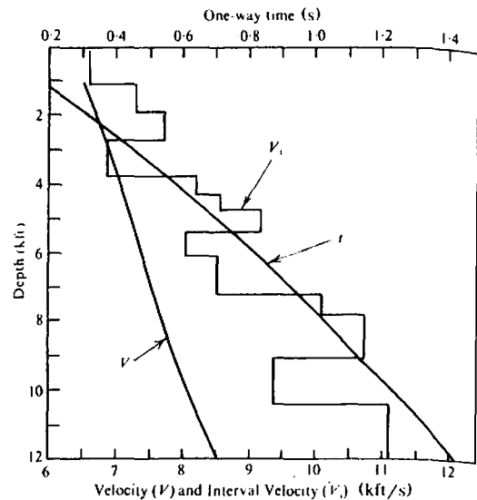
Figure 4.67. Plot of average velocity from datum to depth ( V ) and interval velocity ( V_i ) for a well-velocity survey.
