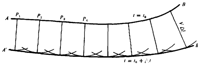
Figure 4.11. Using Huygens' principle to locate new wavefronts.
