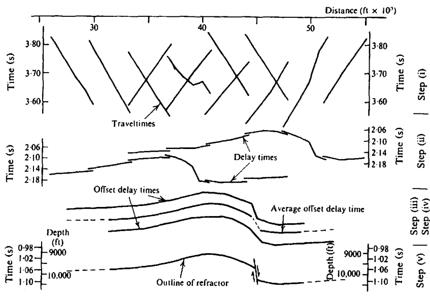
Figure 4.89. The delay-time method of interpreting reversed profiles. (After Barry, 1967.)
