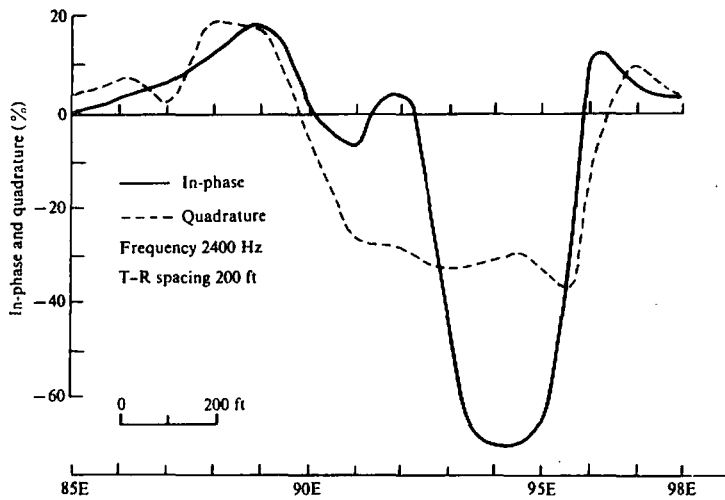
Figure 7.112. HLEM profiles, Eastern Townships, Quebec.
