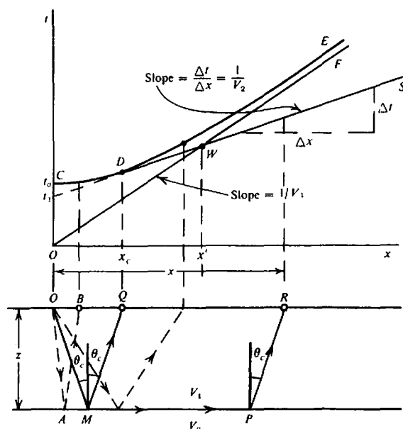
Figure 4.31. Relation between reflection and refraction raypaths and traveltimes curves.
