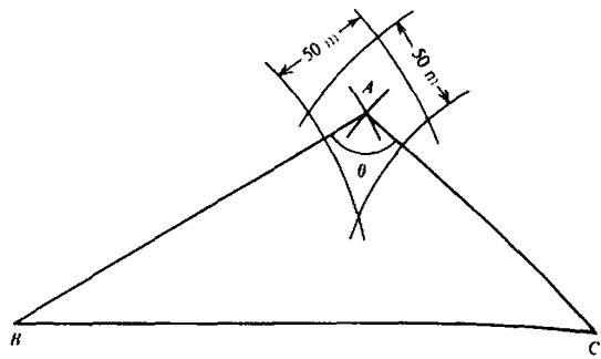
Figure B.1. Locating point A by striking arcs from fixed stations B and C (a rho-rho determination); effect of station angle on errors in position. \theta is the station angle, A is the mobile station, B and C are the shore stations. Point A can be anywhere inside the "parallelogram" formed by the four arcs. [Note: Range errors are not to scale.]
