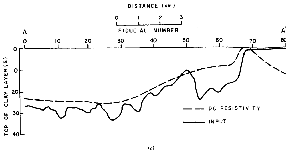
Figure 7.92. (Continued) (c) Comparison of TCP values for the overburden obtained using (b) and by dc resistivity surveys.
