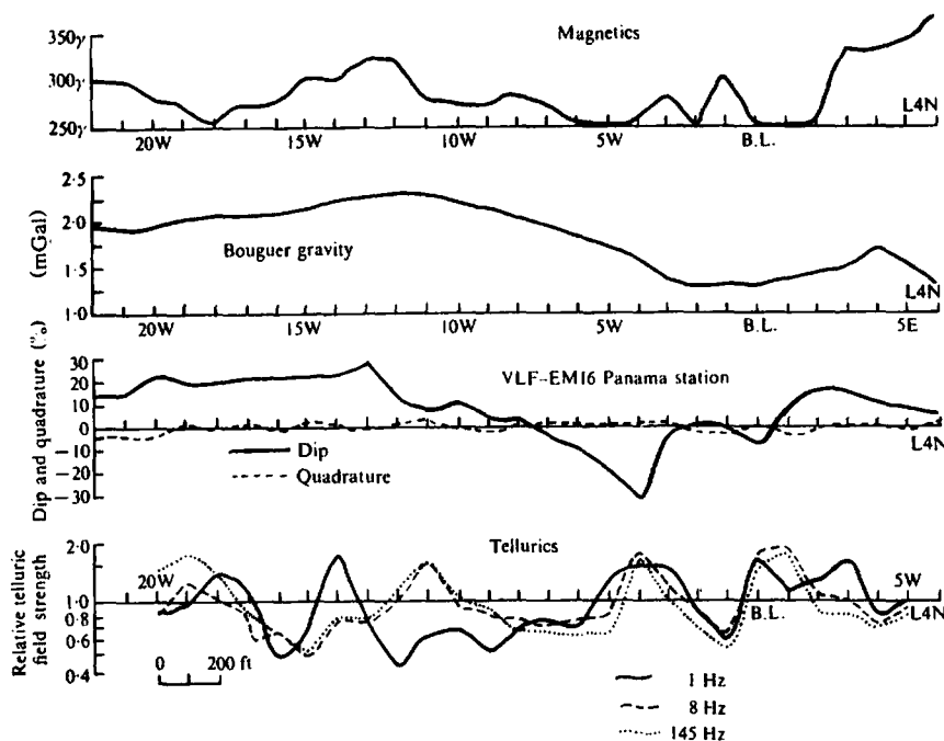
Figure 12.16. Magnetic, gravity, VLF, and telluric profiles, eastern Nova Scotia.
