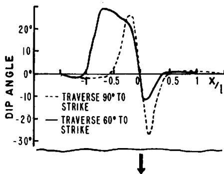
Figure 7.33. Effect of skew traverse direction on response of dip-angle broadside array.
