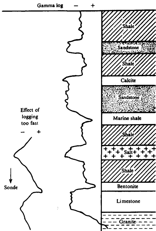
Figure 11.32. A \gamma -ray log.
