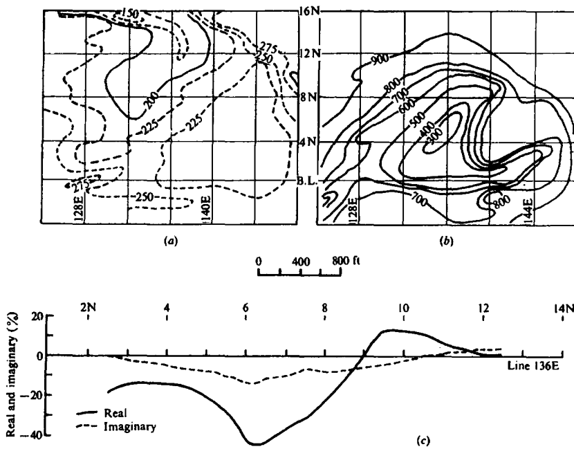
Figure 12.6. Magnetic and electrical data, Murray sulfide deposit, New Brunswick. (a) Magnetic contours; contour interval 25-g. (b) SP contours; contour interval 100 mV. (c) HLEM profile; frequency 440 Hz, T-R spacing 300 ft.
