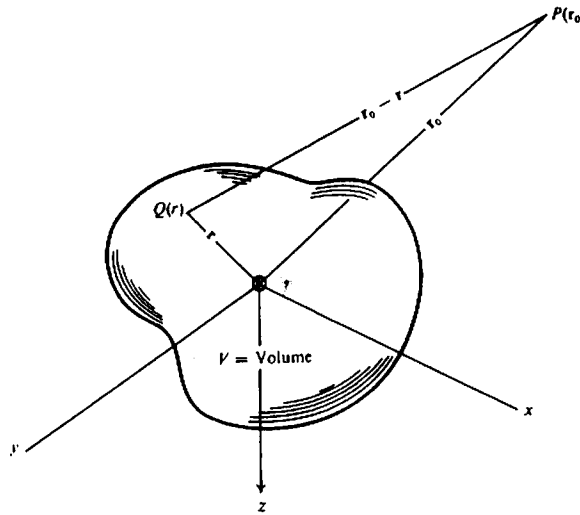
Figure 3.4. General magnetic anomaly.
