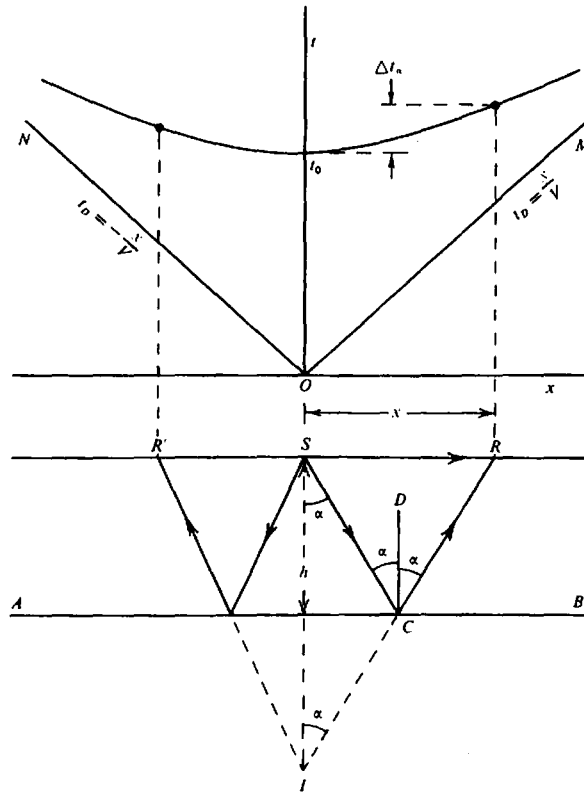
Figure 4.22. Geometry and travelt ime curve for horizontal reflector.
