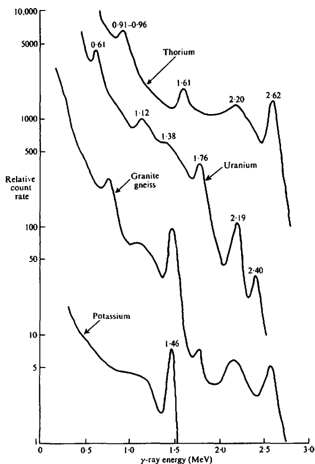
Figure 10.7. \gamma -ray spectra of K, U, and Th samples and granite-gneiss outcrop.
