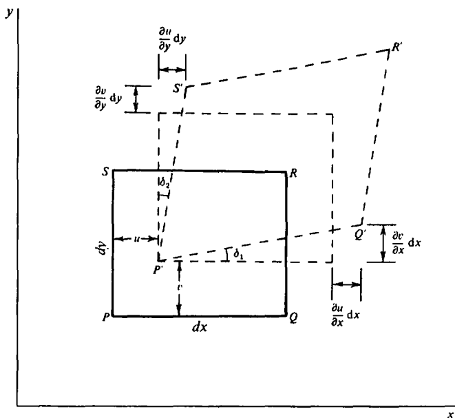
Figure 4.3. Analysis of two-dimensional strain.
