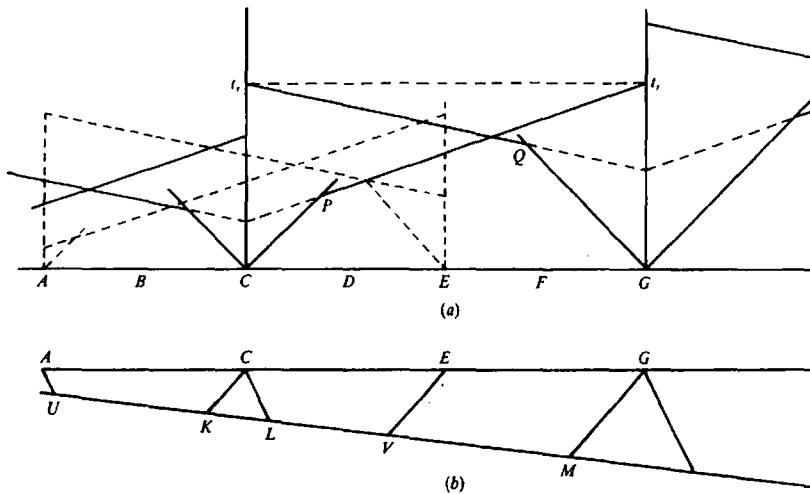
Figure 4.68. Reversed refraction profiles. (a) Time-distance plot for continuous reversed profiling. (b) Section showing raypaths for single refractor.
