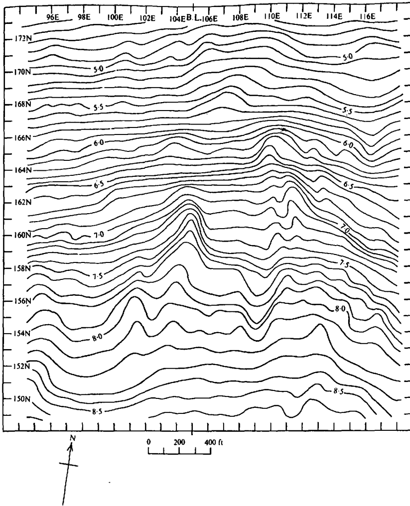
Figure 2.44. Bouguer gravity contours, southern New Brunswick; C.I. = 0.1 \text{ mGal} .
