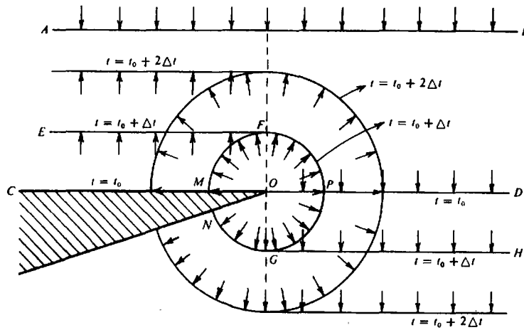
Figure 4.13. Diffracted wavefronts. Diffraction allows seismic energy to reach regions forbidden by ray theory, such as the shadow zone underneath the wedge.
