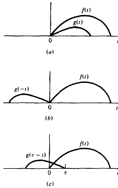
Figure A.6. Illustrating f(t) * g(t) . (a) Two functions, f(t) and g(t) . (b) g(t) reflected in the vertical axis. (c) g(t) reflected and displaced \tau units to the right.
