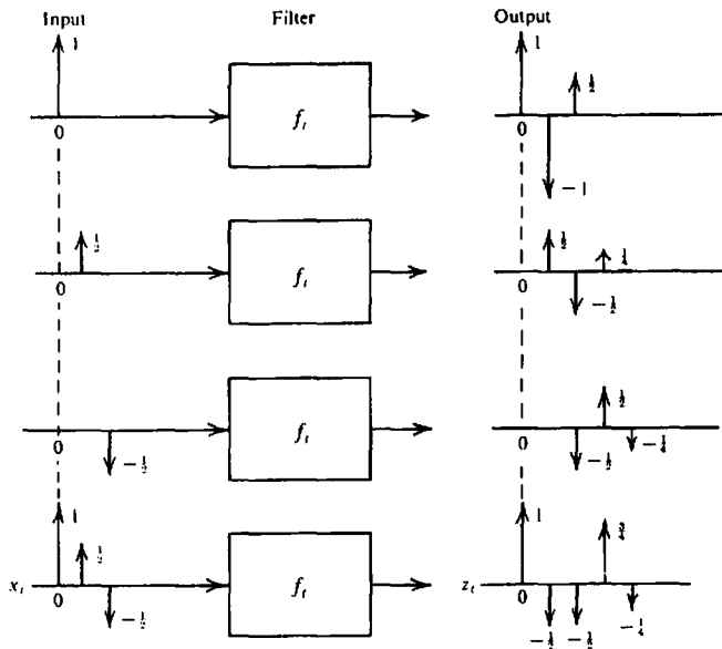
Figure 4.77. Filtering as an example of convolution.
