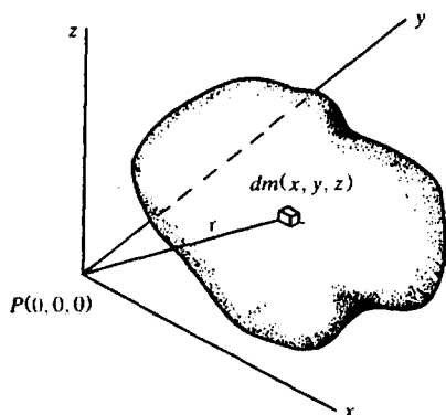
Figure 2.1. Potential of three-dimensional mass.
