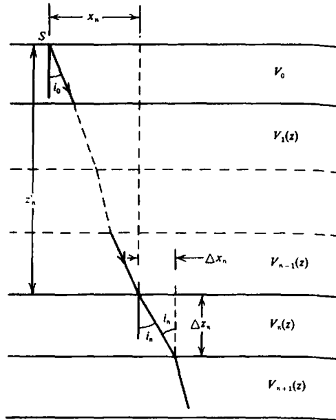
Figure 4.29. Raypath where velocity varies with depth.
