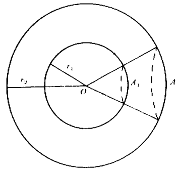
Figure 4.10. Dependence of intensity on distance.
