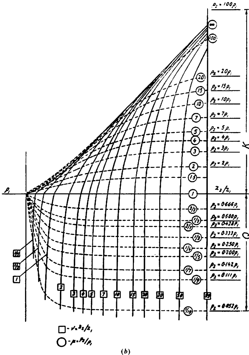
Figure 8.28. (Continued) Auxiliary-point charts (b) for K- and Q-type sounding curves.
