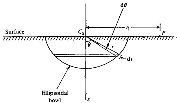
Figure 8.14. Point current source at the surface of anisotropic ground having resistivities \rho_h and \rho_v in the horizontal and vertical directions, respectively.
