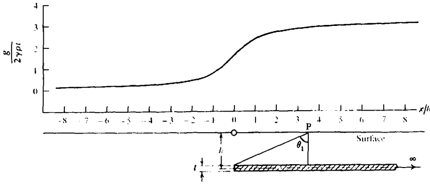
Figure 2.28. Gravity effect of a semiinfinite horizontal sheet.
