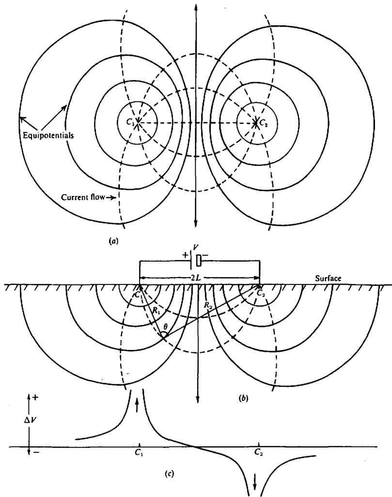
Figure 8.4. Equipotentials and current flow lines for two point sources of current on surface of homogeneous ground. (After Dobrin, 1960.) (a) Plan view. (b) Vertical section. (c) Potential variation at the surface along a straight line through the point sources.
