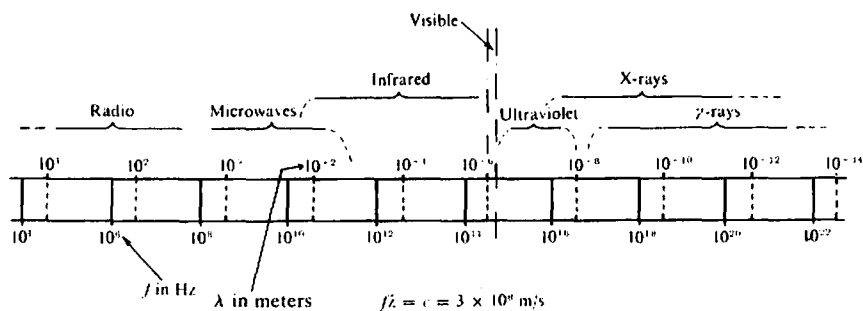
Figure 10.1. The electromagnetic spectrum showing relative frequency (wavelength) bands.
