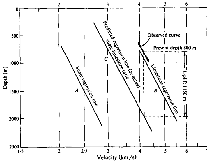
Figure 4.21. Finding maximum depth of burial from velocity. The shale and limestone regression lines represent rocks believed to have not been uplifted. (From Jankowsky, 1970.)
