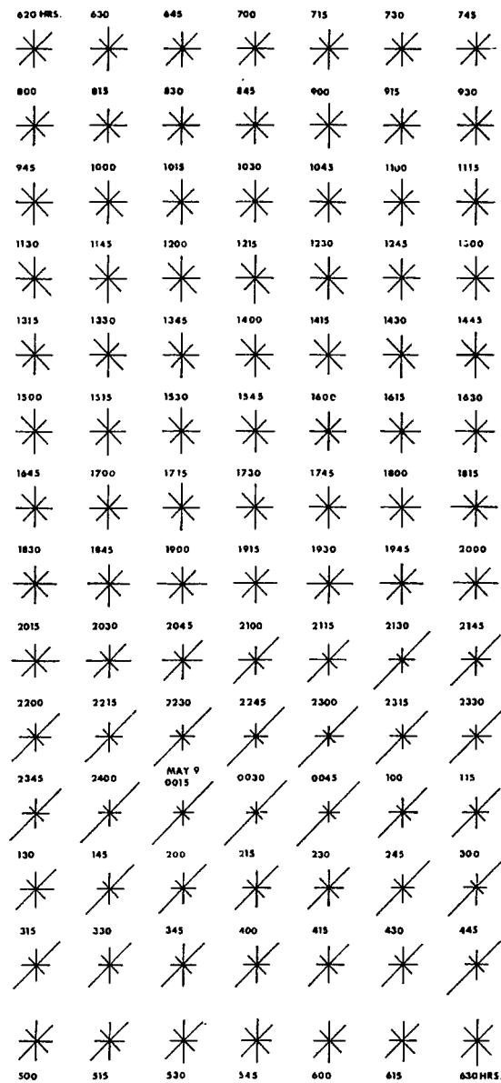
Figure 6.12. Anisotropic telluric response, Vale Perkins, Quebec, May 8-9, 1975. Frequency 145 Hz.
