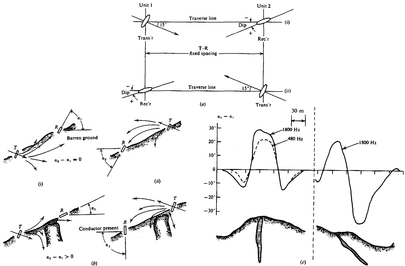
Figure 7.16. Crone shootback system. (After Grant and West, 1965). (a) Transmitter-receiver arrangements, (i) and (ii) representing interchanged positions of the transmitter and receiver for successive measurements at the same station. (b) Operation in rugged terrain. (c) Typical profiles with T-R spacing of 50 to 60 m.
