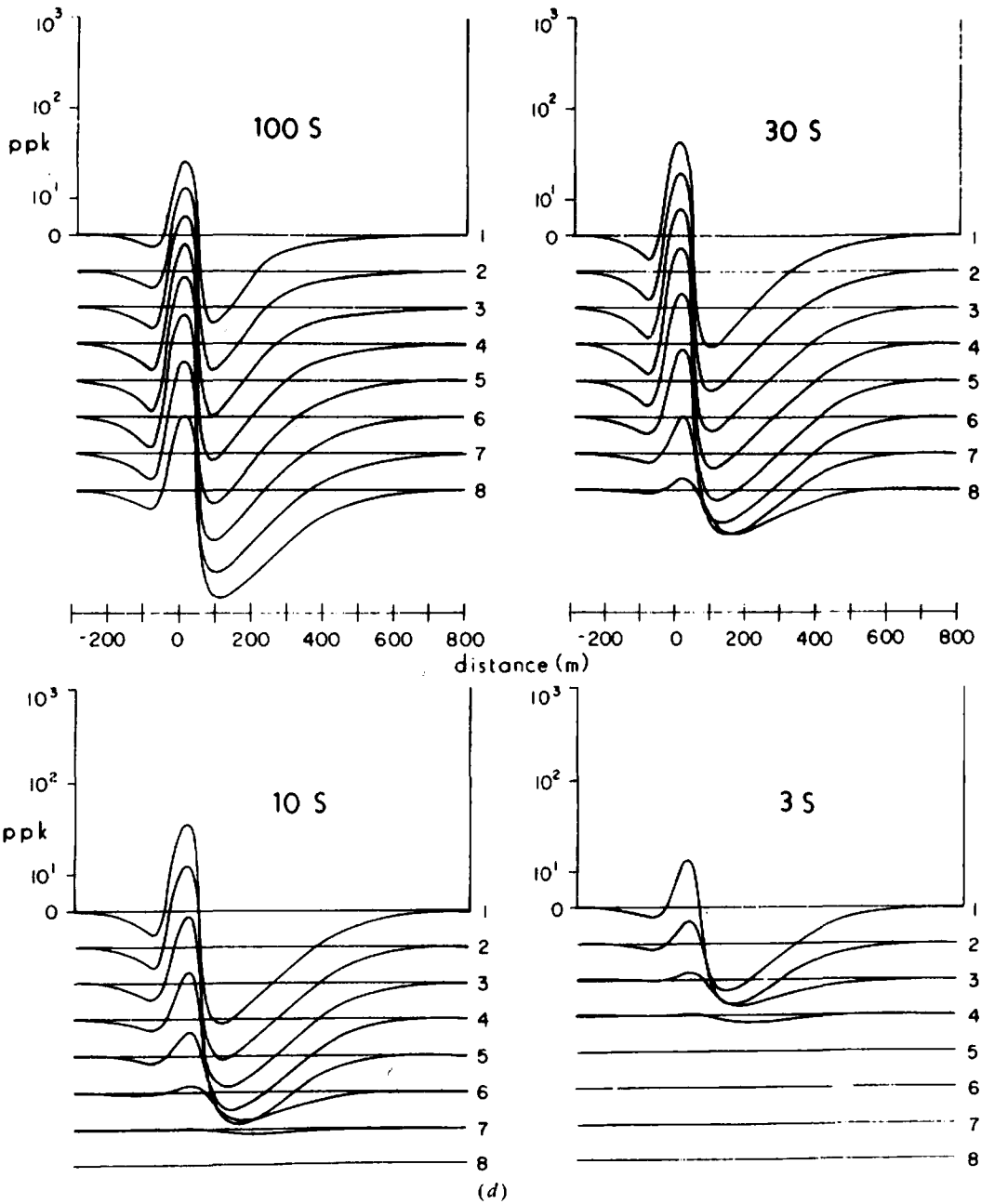
Figure 7.50. (Continued) (d) Variation with TCP; z = 50 m, dip = 30^\circ .
