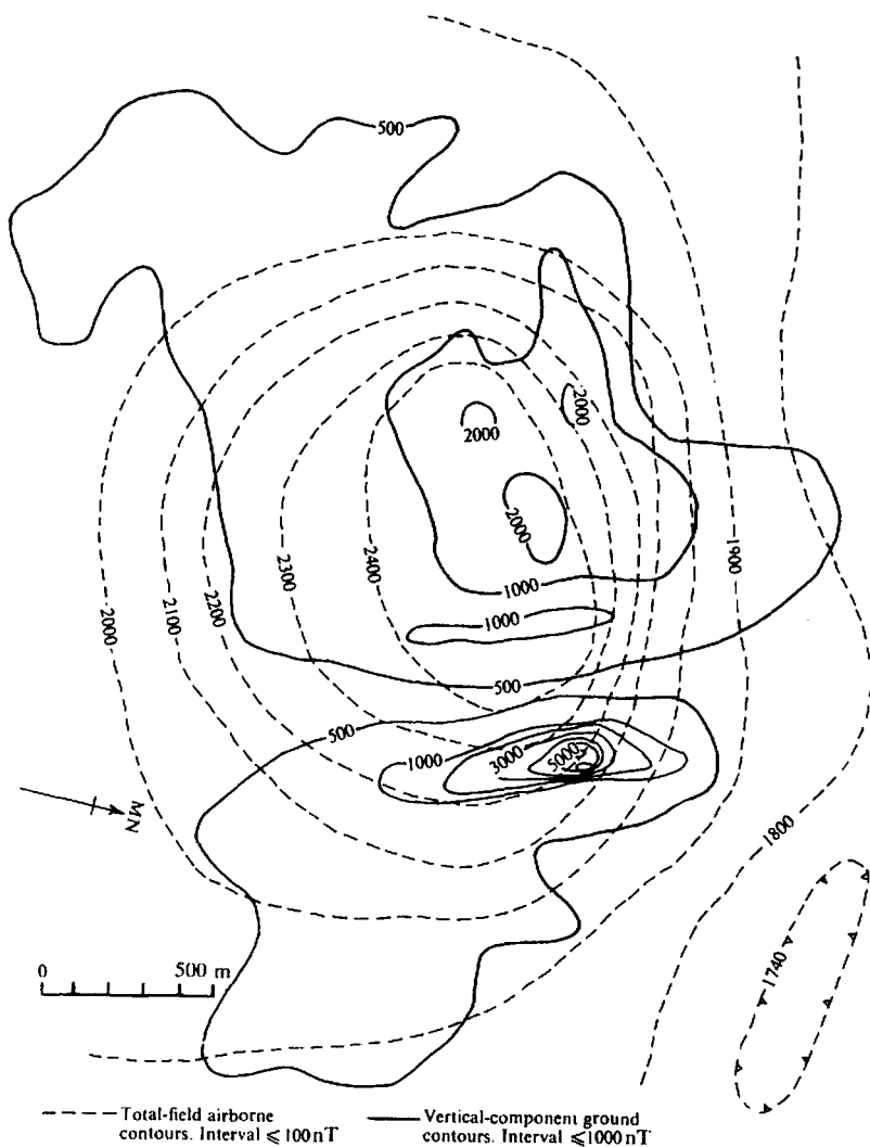
Figure 3.41. Comparison of ground vertical-component data with airborne total-field data.
