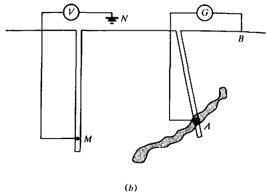
Figure 11.9. Resistivity log configurations for orebody definition. (After Roy, 1984.) (a) Directional resistivity method; the azimuthal direction of AB is changed 90° between measurements. (b) Mise-à-la-masse method with the A electrode embedded in conductive orebody and potential measured in nearby boreholes.
