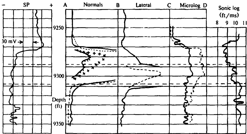
Figure 11.44. Log suite in Miocene sand section containing oil and gas. Full scale for the 16 in. normal (solid curve) is 10 \Omega m , for the amplified 16 in. normal (solid hachured) is 100 \Omega m , for the 64 in. normal (dashed) is 10 \Omega m , for the amplified 64 in. normal (crosses) is 1,000 \Omega m , for the 18 ft 8 in. lateral (solid) is 10 \Omega m , for the amplified 18 ft 8 in. lateral (dashed) is 100 \Omega m , and for the microlog inverse (solid) and for the micronormal (dashed) is 10 \Omega m .
