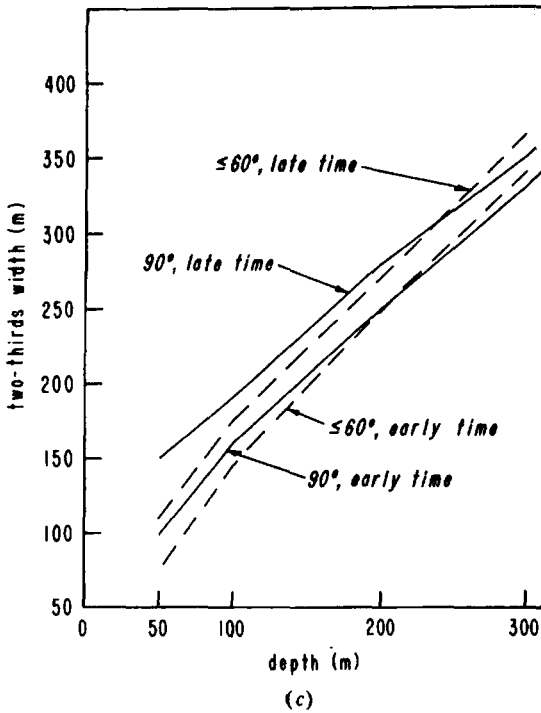
Figure 7.66. (Continued) (c) Two-thirds width versus depth for early and late times, dips 90 and \leq 60^\circ .
