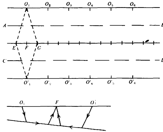
Figure 4.71. Broadside refraction profiling.
