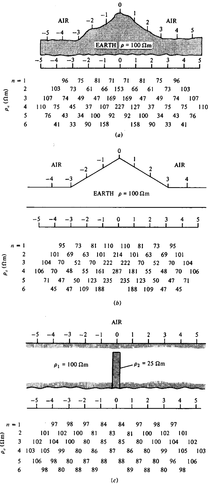
Figure 8.52. Effect of terrain on dipole-dipole resistivity survey. (a) Pseudodepth plot of \rho_a over 2-D ridge. (b) Model results for a 30° ridge. (c) Results over a buried vertical conductive dike.
