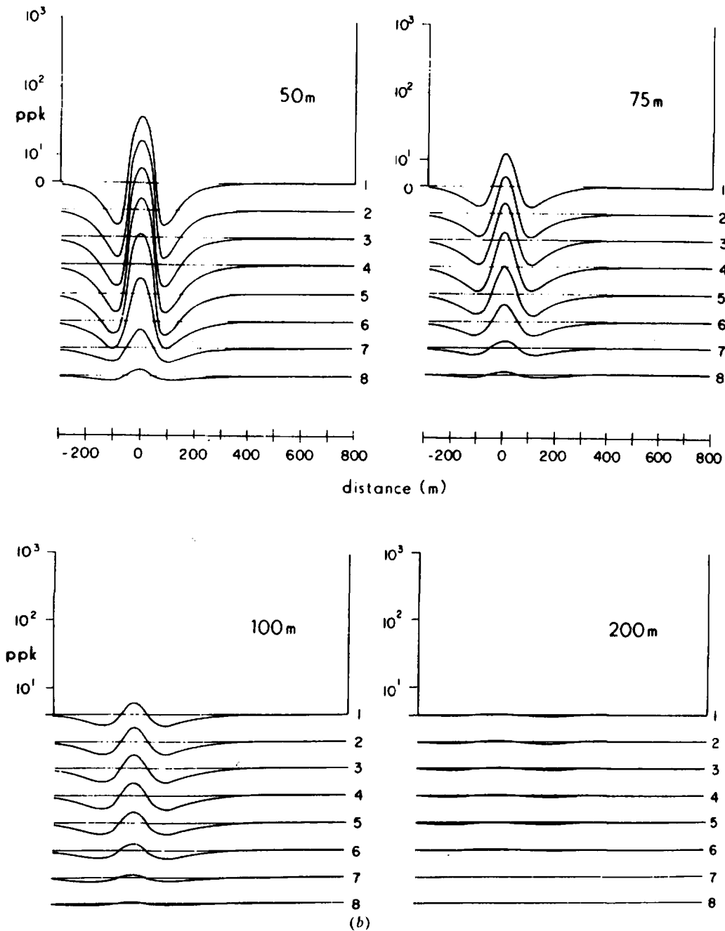
Figure 7.50. (Continued) (b) Effect of depth, dip = 90°.
