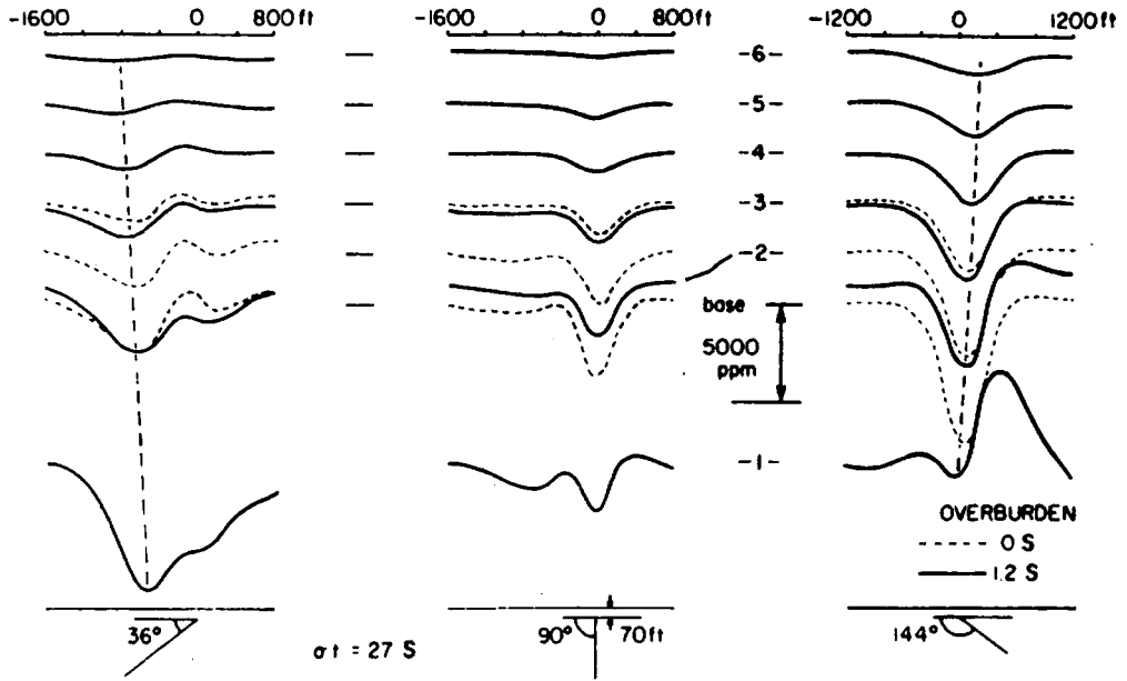
Figure 7.90. Model profiles over dipping half-plane ( \sigma t = 27 S , depth to top = 70 ft) under conductive overburden. Dashed line indicates shift of anomaly peak from early to late time. (After Palacky, 1975.)
