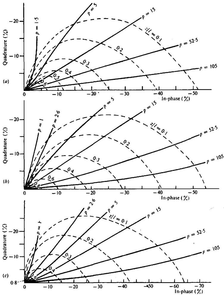
Figure 7.44. Characteristic curves for horizontal-loop system over a dipping sheet. \rho = \sigma\mu\omega t . (From Strangway, 1966.) (a) Dip = 90°. (b) Dip = 60°. (c) Dip = 30°.
