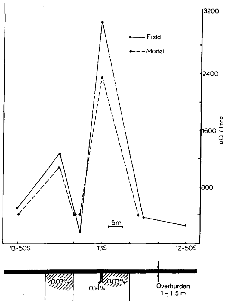
Figure 10.11. Radon profile and model results, Northern Saskatchewan. (From Soonawala, 1976.)
