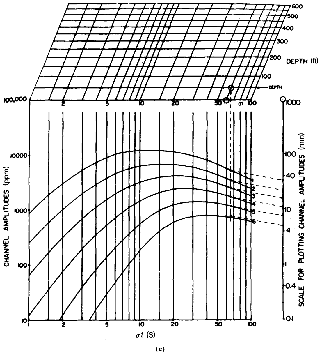
Figure 7.88. Nomograms for obtaining conductivity and depth. (a) Nomogram giving TCP and h for a vertical sheet. (After Palacky and West, 1973.)
