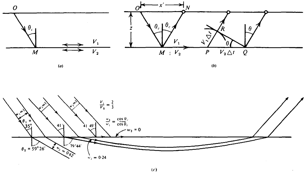
Figure 4.30. Headwaves. (a) Motion at the interface. (b) Wavefront emerging from refractor at critical angle. (c) Changes in beam width upon refraction and bending of refracted raypaths because of the velocity gradient in the high-velocity medium.
