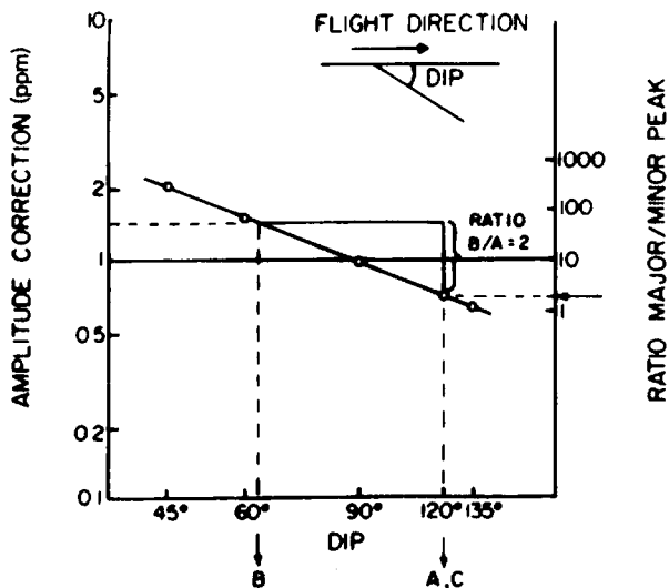
Figure 7.89. Estimating dip of a half-plane from the ratio of major-to-minor peak amplitudes. The amplitude correction (see left-hand vertical scale) corrects for the effect of dip on amplitude. (After Palacky and West, 1973.)
