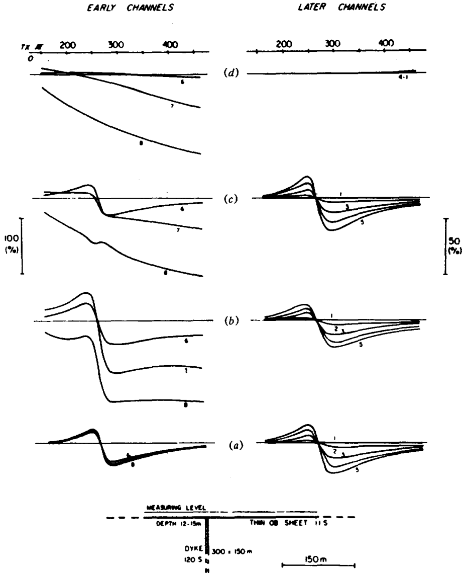
Figure 7.63. Model UTEM H_2^s profiles over a vertical conductive sheet under a thin conductive overburden. (After West, Macnae, and Lamontagne, 1984.) (a) Effect of sheet alone. (b) Sheet in contact with the overburden. (c) Sheet not in contact with overburden. (d) Overburden alone.
