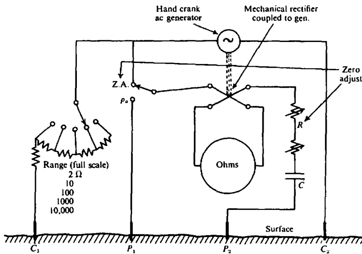
Figure 8.17. Portable equipment for measuring resistivity (schematic).
