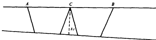
Figure 4.95. Refraction profile for determining depth to bedrock.
