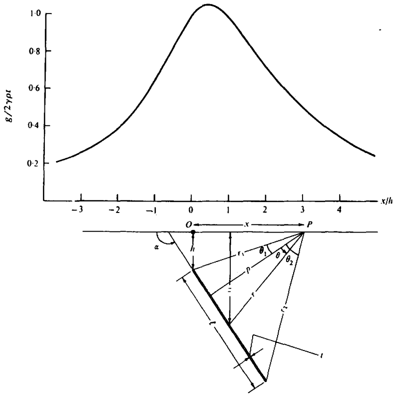
Figure 2.27. Gravity effect of a thin sheet of infinite strike length.
