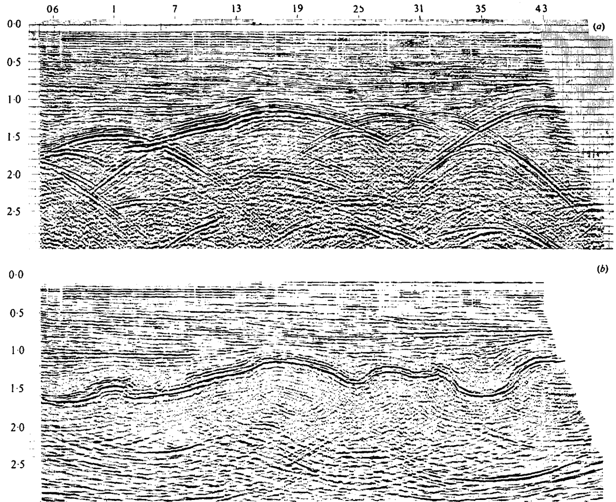
Figure 4.84. Unmigrated and migrated seismic sections. (Courtesy A.G.I.P. and Western Geophysical.) (a) Before migration. (b) After migration. Multiple-branch reflection events migrate into a relatively continuous reflector. Deeper data, which are principally multiples, are not migrated properly.
