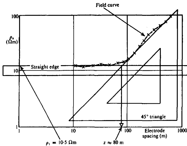
Figure 8.22. Estimate of \rho_1 and z from the 45^\circ asymptote. (After Keller and Frischknecht, 1966.)
