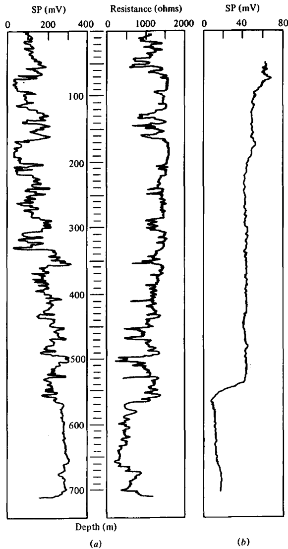
Figure 11.11. SP log comparison. (Data courtesy Atomic Energy Canada, Ltd., Chalk River, Ont.) (a) Result of a carefully designed survey. (b) Commercial log in the same borehole.
