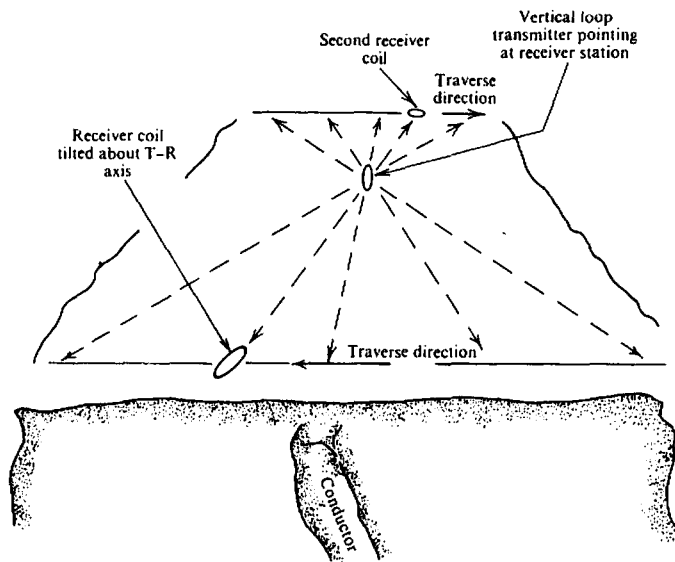
Figure 7.14. Dip-angle system, fixed transmitter.
