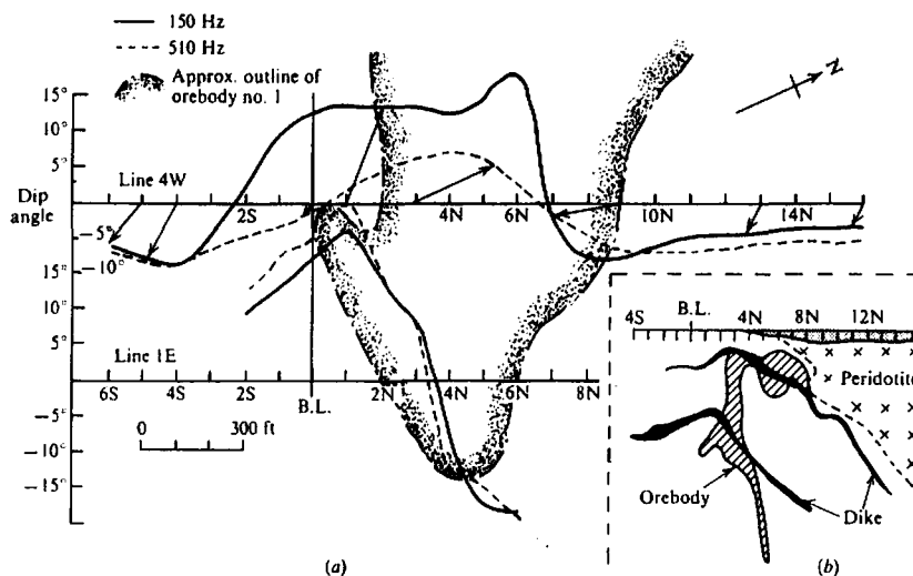
Figure 7.98. AFMAG survey, Mattagami Lake Mines, Quebec. (From Paterson, 1966.) (a) Profiles along lines 4W and 1E. (b) Cross section, line 4W.
