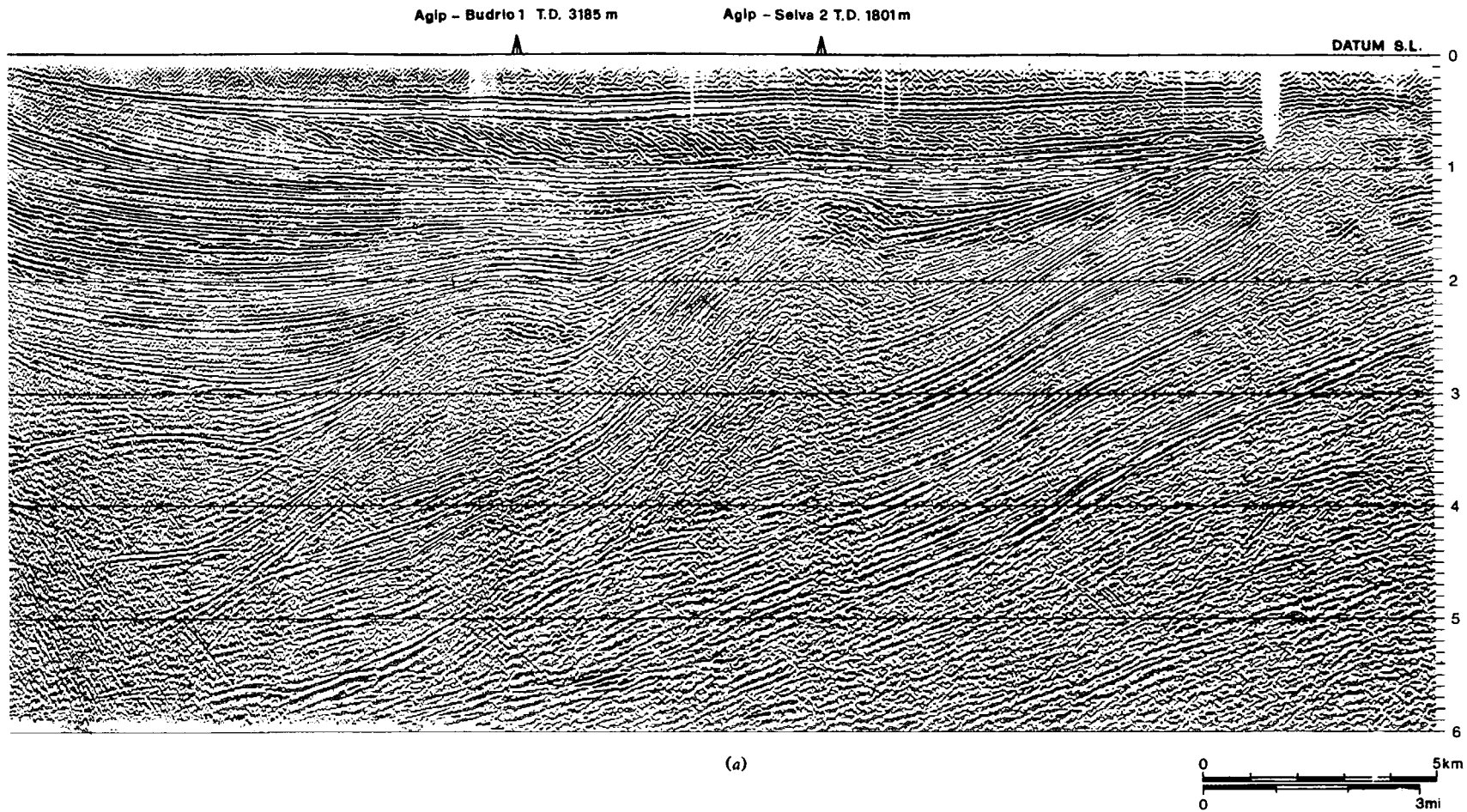
Figure 4.100. Seismic profile in the Po Valley. Thrust faulting from the north produced a series of folds. The Budrio thrust appears to have been relatively quiet in the Middle Pliocene, the Selva thrust quiet since the Late Pliocene, and the thrust only partially seen at the right active into the Quaternary. (From Pieri, 1983.) (a) Migrated seismic section.
