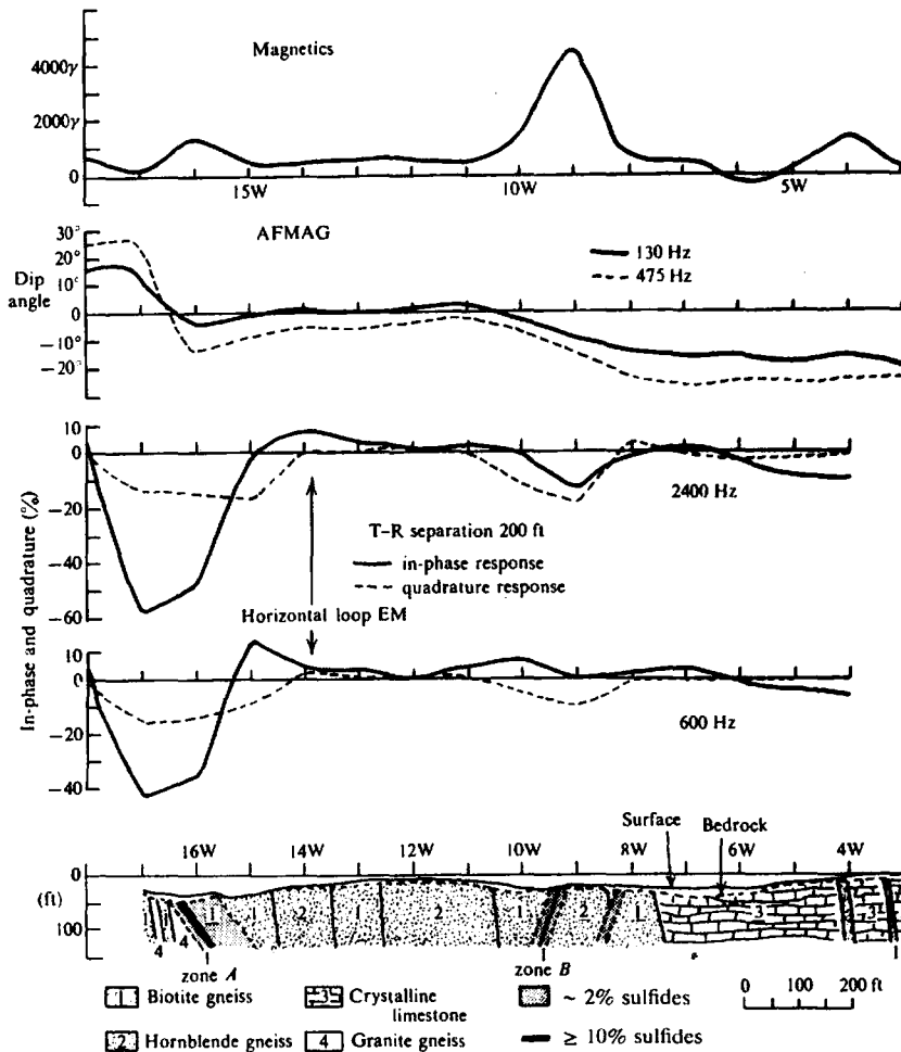
Figure 12.9. Geophysical results and geologic section, line C, Cavendish Township, Ontario.
