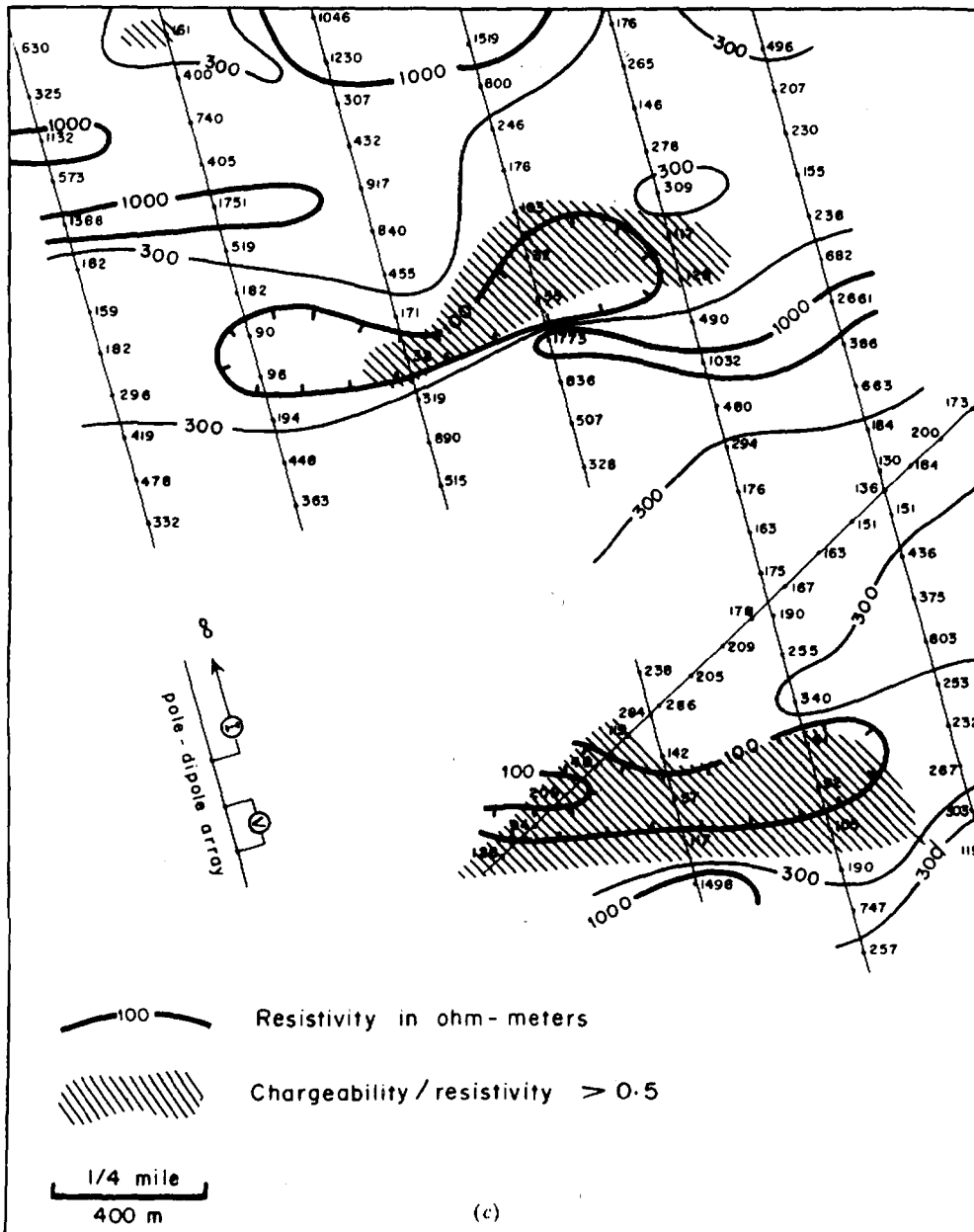
Figure 7.85. (Continued) (c) Ground IP resistivity map of the same area showing two anomalies.
