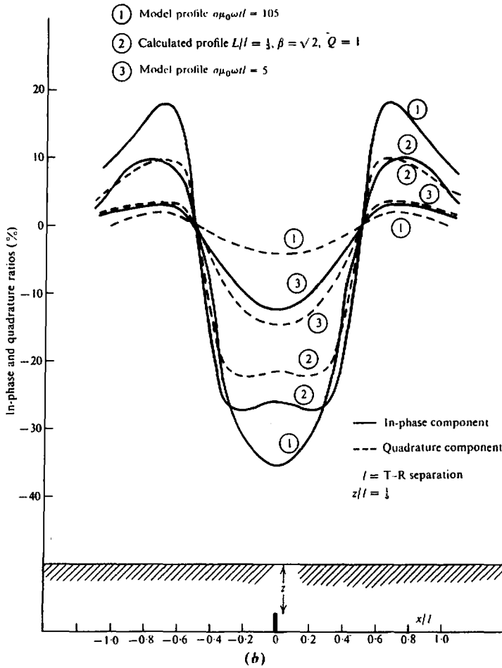
Figure 7.36. (Continued) (b) Effect of conductivity of a semiinfinite vertical sheet.
