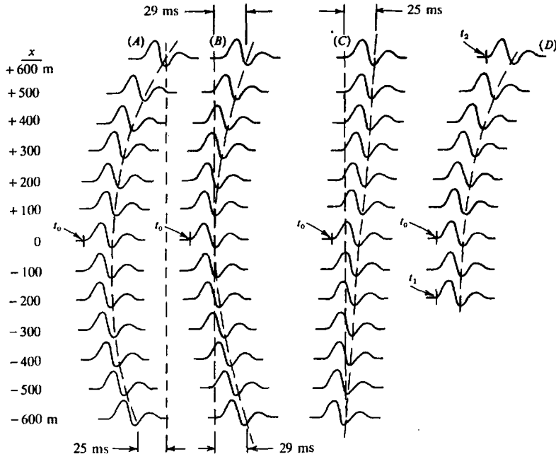
Figure 4.24. Relation between normal moveout and dip moveout; t_0 = 1,000 s, V = 2,500 m/s.
