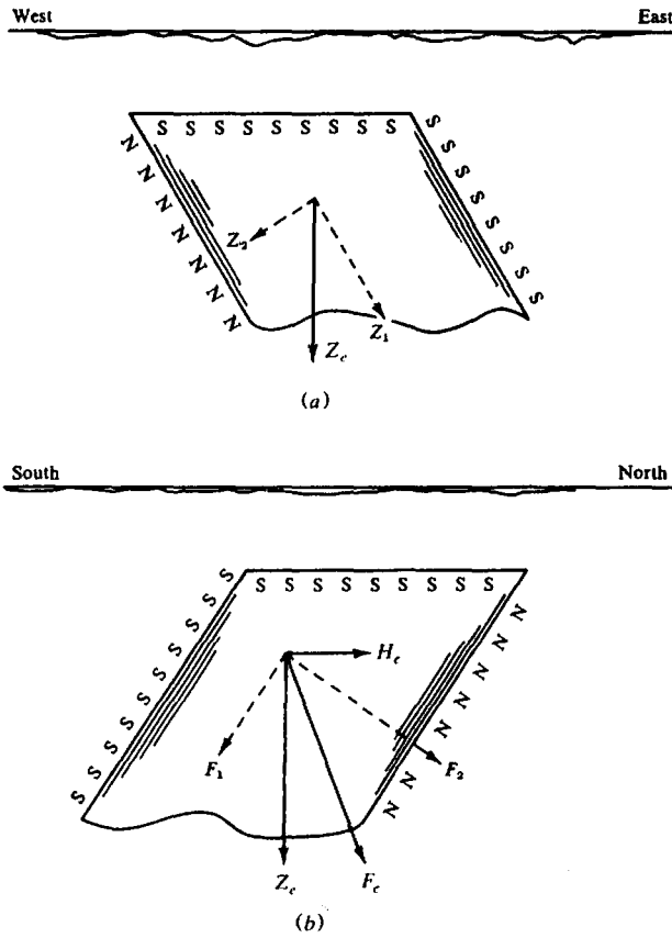
Figure 3.19. Pole distribution in a dike.
