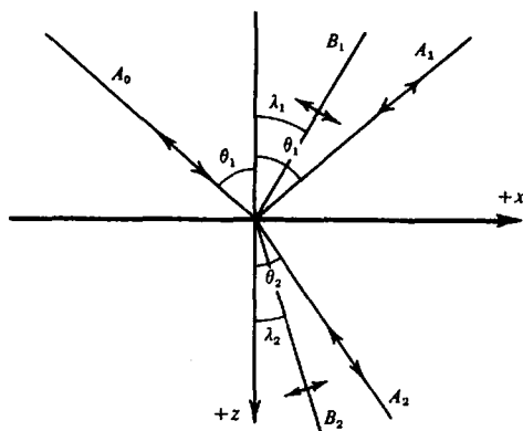
Figure 4.16. Waves generated at an interface by an incident P wave.
