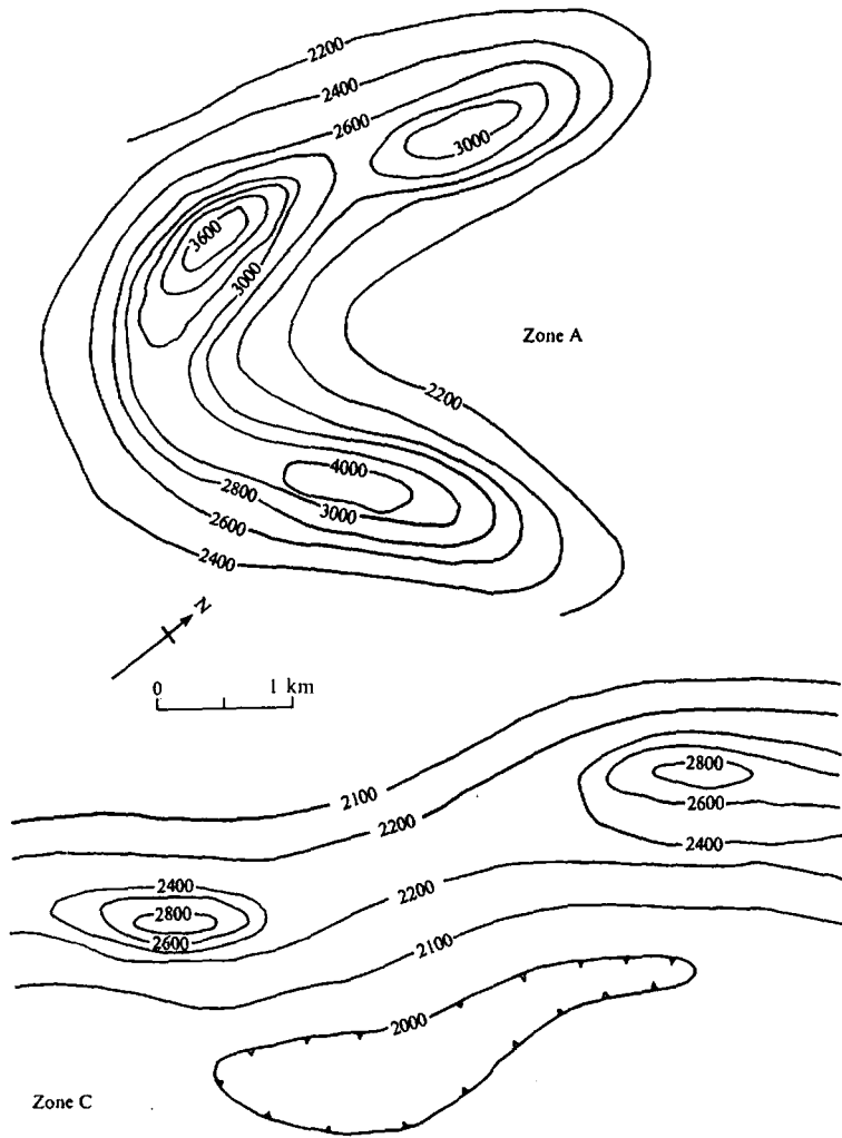
Figure 3.37. Ground magnetic contours, northern Manitoba. C.I. = 100 nT.
