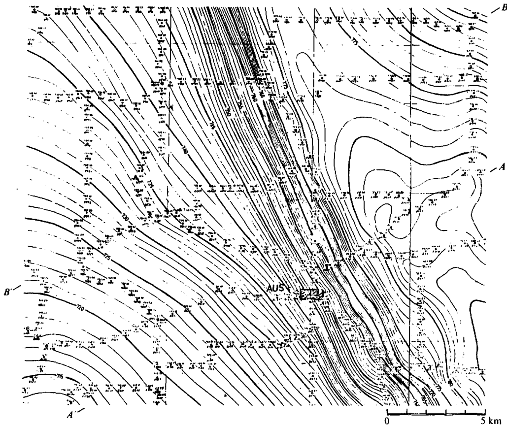
Figure 2.46. Bouguer gravity map, Western Australia; C.I. = 1.0 \text{ mGal} . (Courtesy West Australian Petroleum.)
