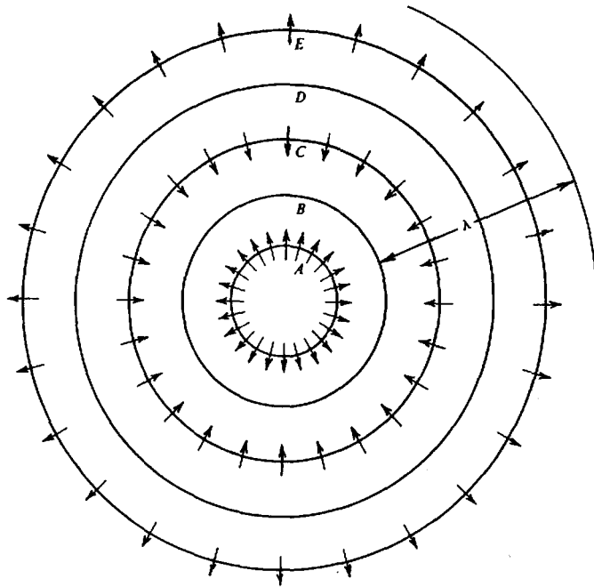
Figure 4.7. Displacements for a spherical P wave.
