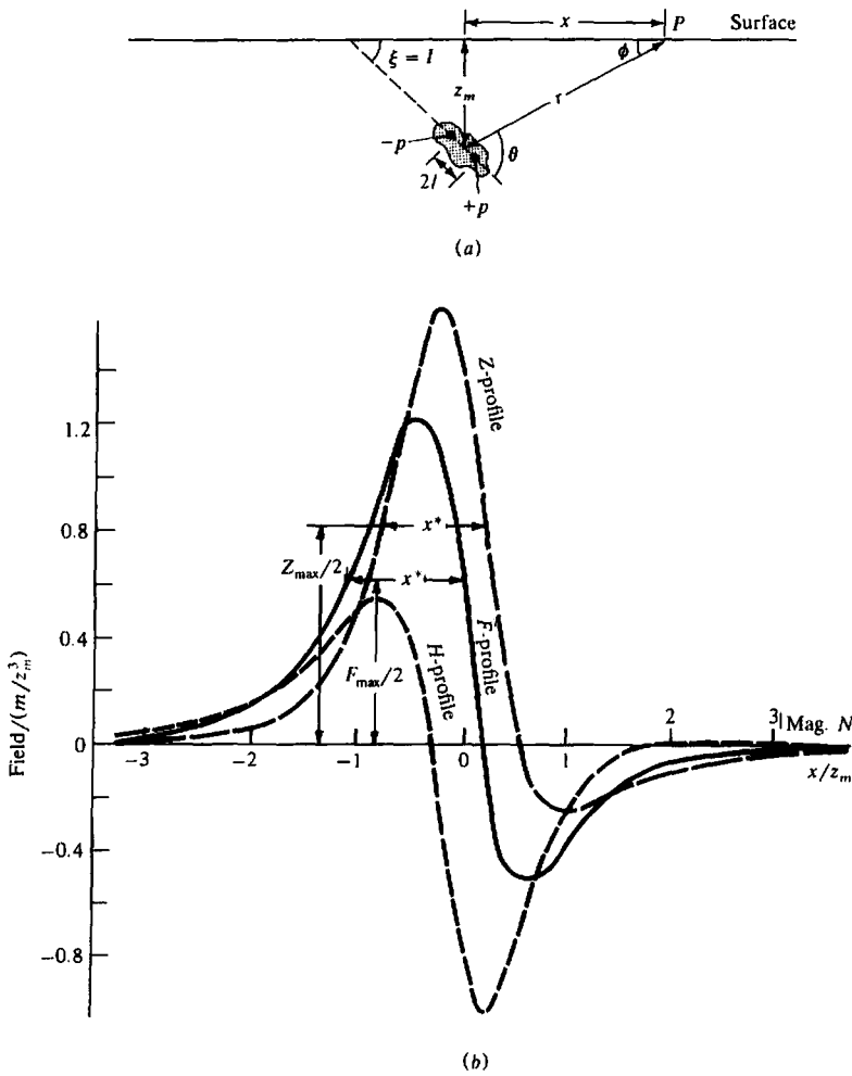
Figure 3.15. Magnetic effects of an isolated dipole. (a) Geometry. (b) Profiles for l = 45^\circ .
