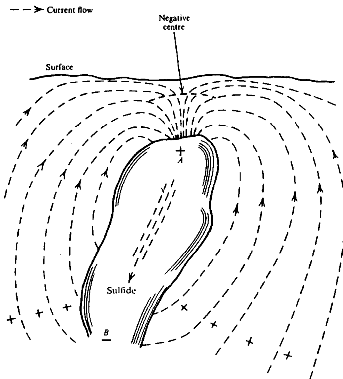
Figure 6.1. Oxidizing sulfide zone as a galvanic cell.
