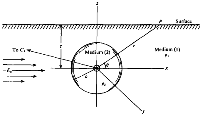
Figure 8.12. Buried conducting sphere in uniform field.
