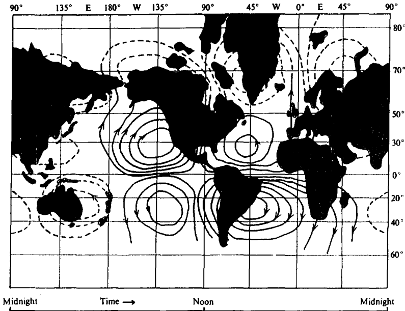
Figure 6.9. Worldwide telluric-current system on Mercator's projection. (After Dobrin, 1960.)
