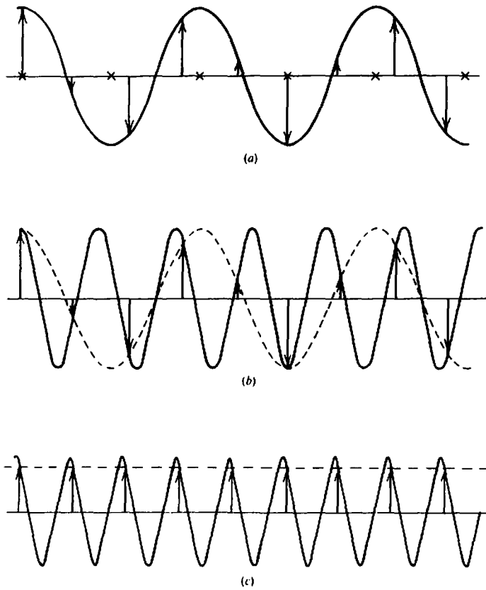
Figure 4.79. Sampling and aliasing. Different frequencies sampled at 4 ms intervals (250 times per second). (a) 75 Hz signal. (b) The 175 Hz signal yields the same sample values as 75 Hz. (c) The 250 Hz signal yields samples of constant value (dc).
