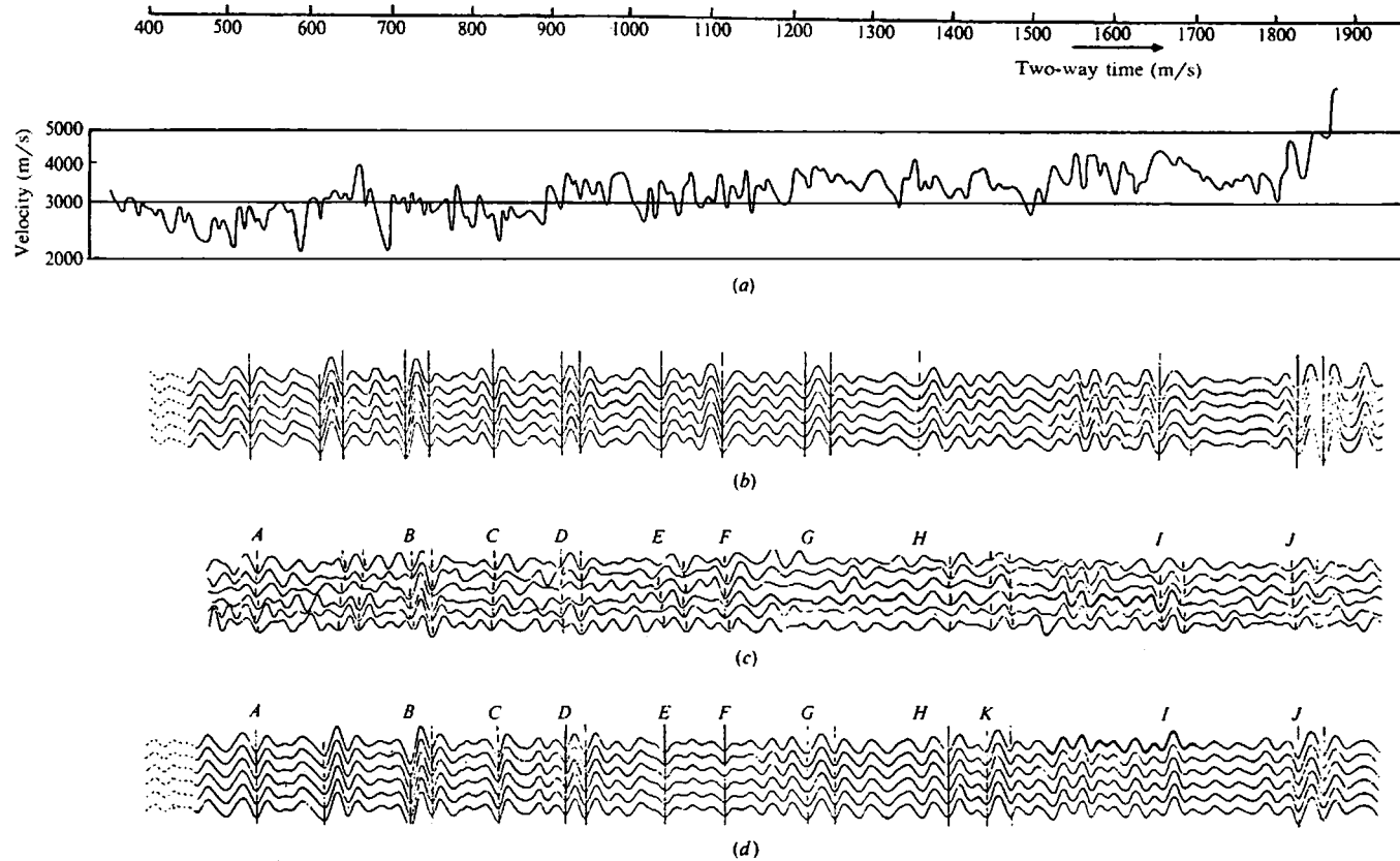
Figure 4.96. Synthetic seismograms. (Courtesy Compagnie Générale de Géophysique.) (a) Sonic log plotted in time. (b) Synthetic seismogram of primary reflections only. (c) Field record after normal-moveout correction. (d) Synthetic seismogram with simple multiples added.
