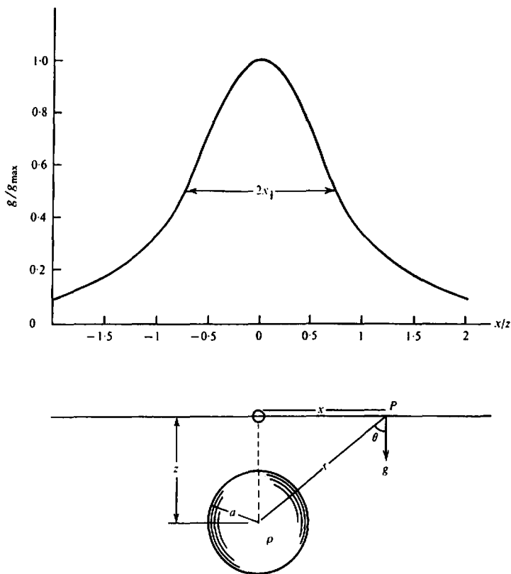
Figure 2.23. Gravity effect of a sphere.
