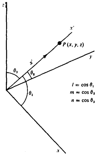
Figure 4.5. Wave direction not along an axis.
