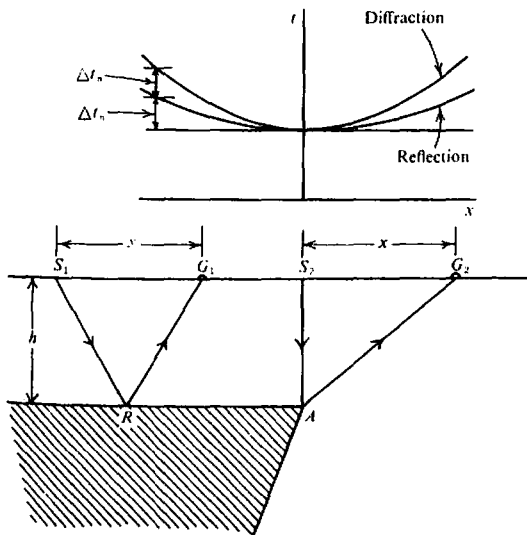
Figure 4.37. Diffraction travelttime curve.
