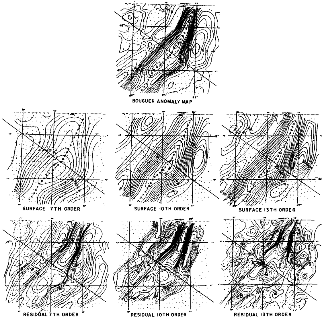
Figure 2.19. Fits of surfaces of different order and the respective residuals. (After Coons, Woolard, and Hershey, 1967.)
