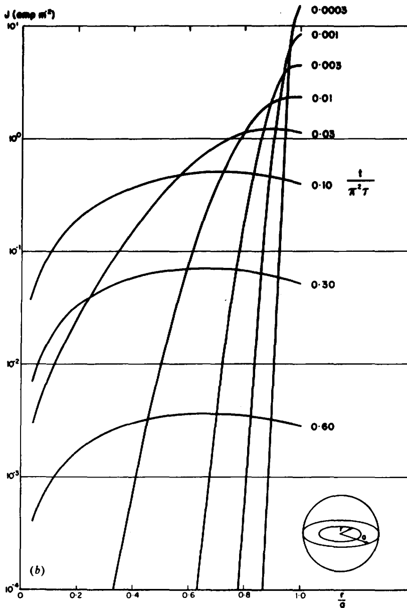
Figure 7.69. (Continued) (b) Radial distribution of current in a sphere for several values of (t/\pi^2\tau) . (After McNeill, 1980.)
