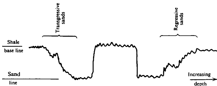
Figure 11.14. Characteristic SP curves for transgressive and regressive sands.
