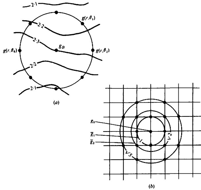
Figure 2.20. Analytical separation of the residual and the regional. (a) Griffin method. (b) Second-derivative method.
