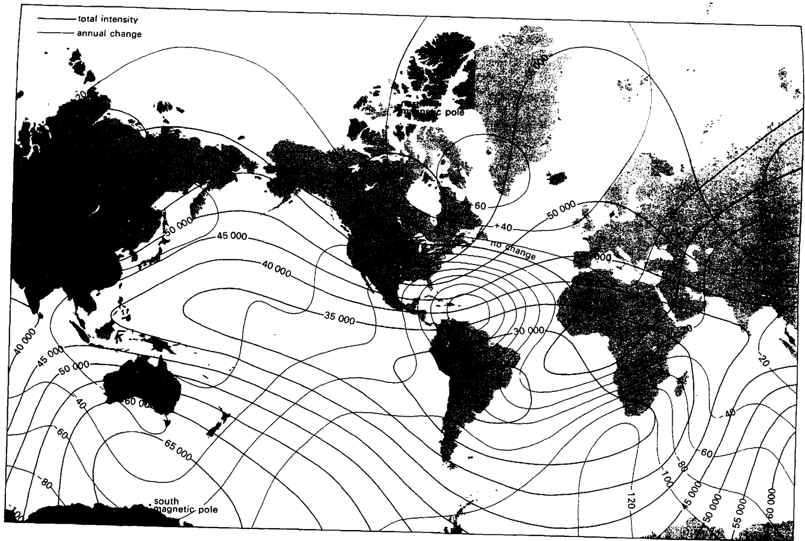
Figure 3.6. (Continued) (c) total field strength in nanotesla (heavy lines) and rate of change in nanotesla/year (light lines).
