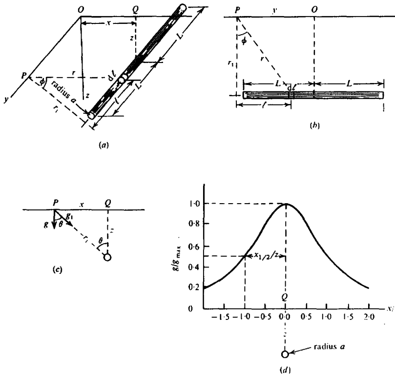
Figure 2.24. Gravity effect of a horizontal rod. (a) Three-dimensional view. (b) Projection on the plane containing the rod and the y axis. (c) Projection on the xz plane. (d) Gravity profile along the x axis ( L = \infty ).
