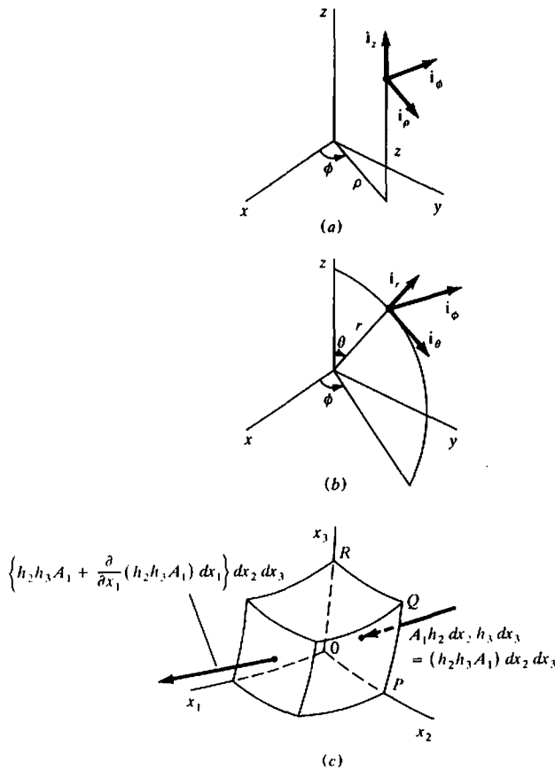
Figure A.4. Curvilinear coordinates. (a) Cylindrical coordinates. (b) Spherical coordinates. (c) \text{div} A in curvilinear coordinates.
