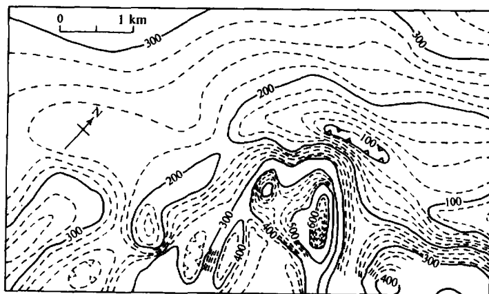
Figure 3.42. Total-field aeromagnetic contours, northwest Newfoundland. C.I. = 20 nT and flight altitude 300 m.
