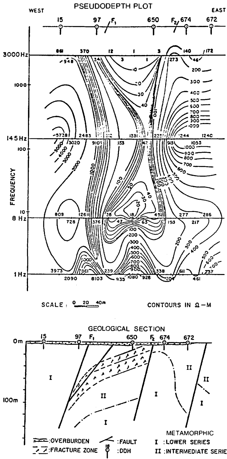
Figure 6.29. Magnetotelluric pseudodepth plot for conductive fracture zone, Northern Saskatchewan.
