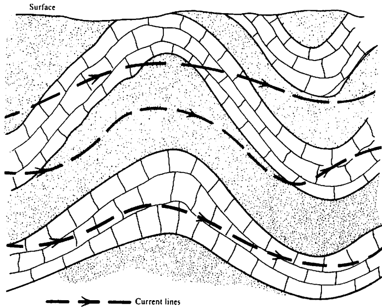
Figure 6.18. Distortion of telluric current flow by anticline. (After Boissonnas and Leonardon, 1948.)
