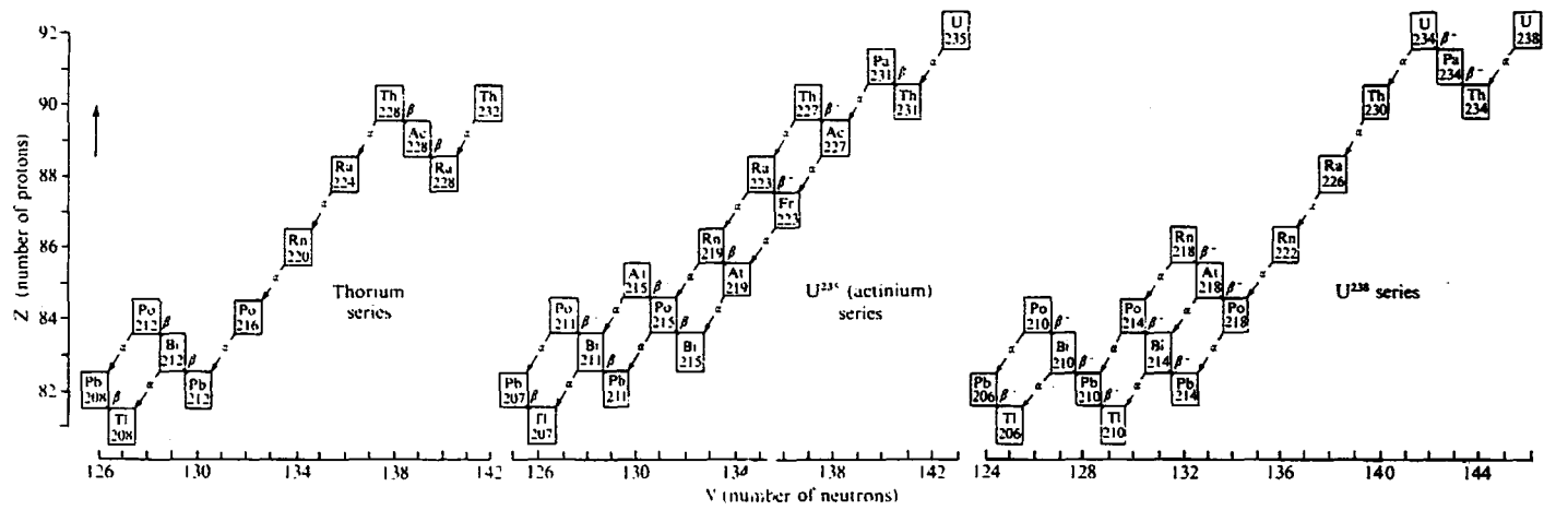
Figure 10.3. Uranium and thorium radioactive series. Schematic showing decay processes.
