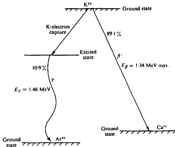
Figure 10.2. Energy-level diagram for radioactive potassium.
