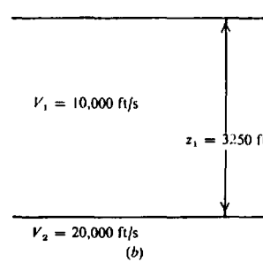
Figure 4.121. Two different geologic sections that give the same refraction time-distance curve.
