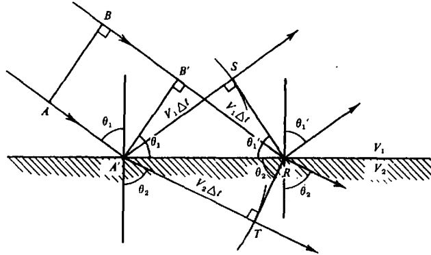
Figure 4.12. Reflection and refraction of a plane wave.
