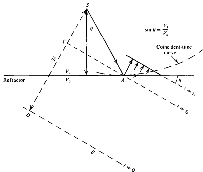
Figure 4.120. Deriving the properties of the coincident-time curve.
