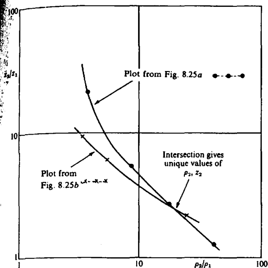
Figure 8.26. Determining second-layer parameters using data from Figure 8.25. (After Keller and Frischknecht, 1966.)
