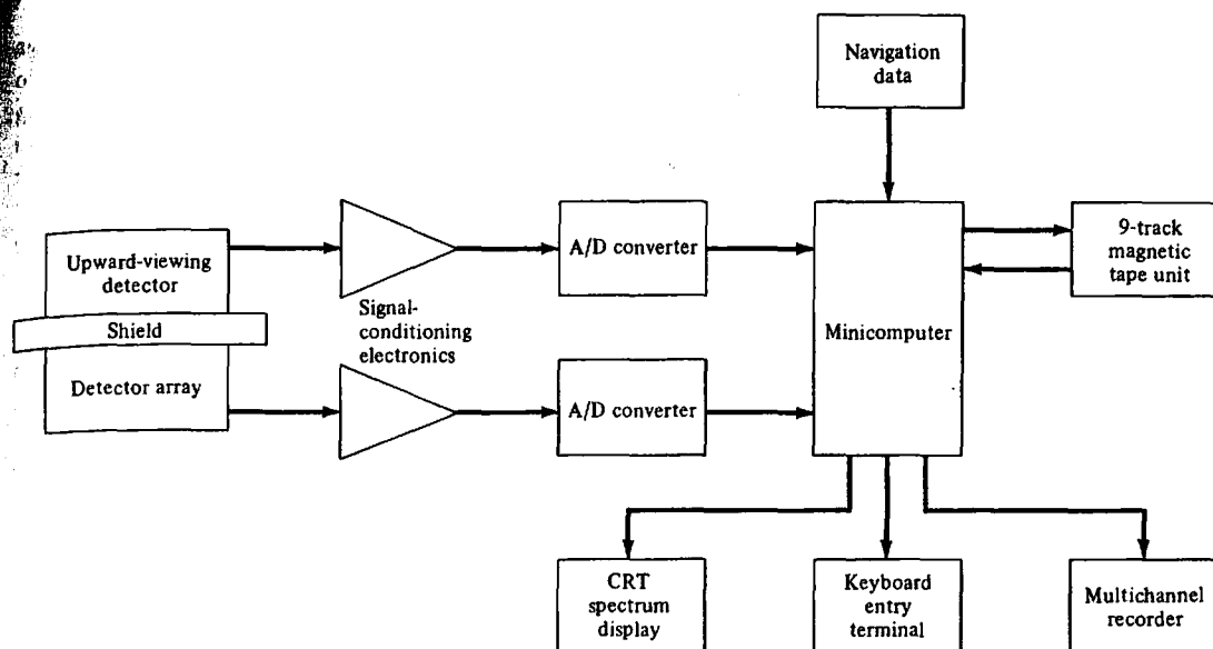
Figure 10.9. Modern \gamma -ray spectrometer. (After Bristow, 1979.)
