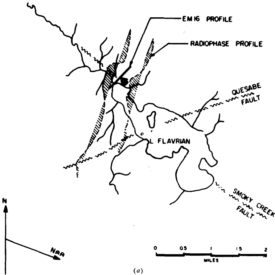
Figure 7.80. Airborne VLF (radiophase) and detailed EM16 ground survey, Smoky Creek fault area, near Lake Abitibi-Noranda, Quebec. (From Telford, King, and Becker, 1977.) (a) Map showing survey lines, fault traces, and profile locations.
