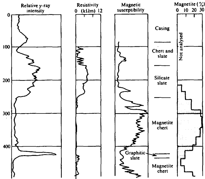
Figure 11.48. Gamma-ray, susceptibility, and resistivity logs in chert and slate beds.
