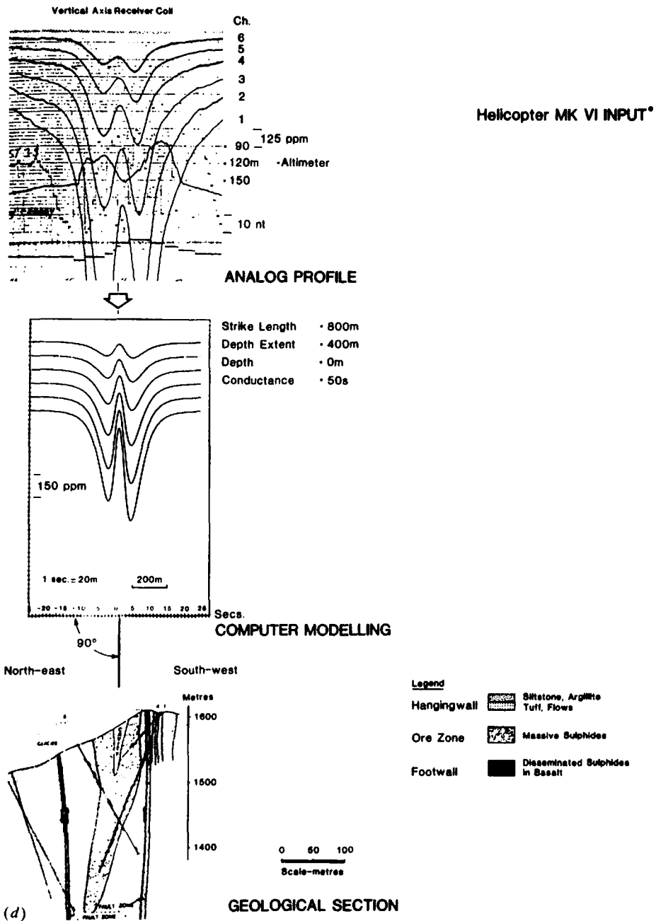
Figure 7.108. (Continued) (d) Windy Craggy sulfide body (Cu).
