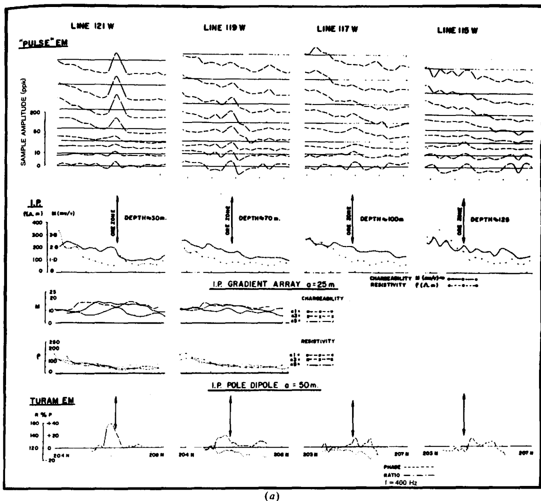
Figure 7.118. Multimethod surveys over a sulfide ore body, southwest Africa. (a) PEM ("Pulse" EM), IP (gradient and pole-dipole arrays), Turam.
