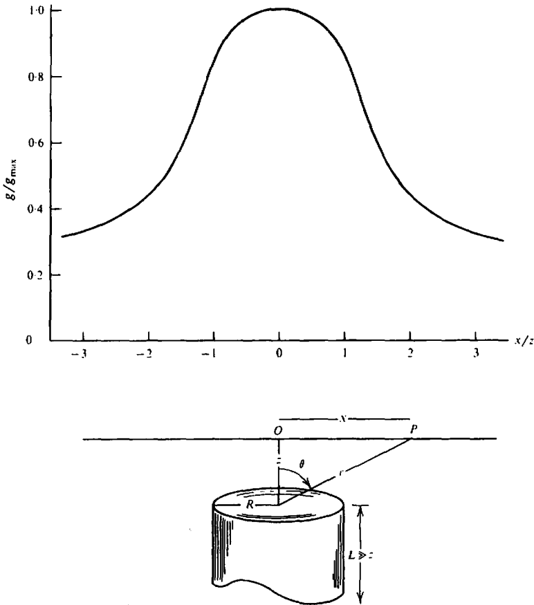
Figure 2.26. Gravity effect off the axis of a vertical cylinder.
