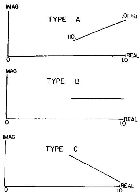
Figure 9.15. Idealized spectral IP response for three types of host rock. (After Zonge and Wynn, 1975.)
