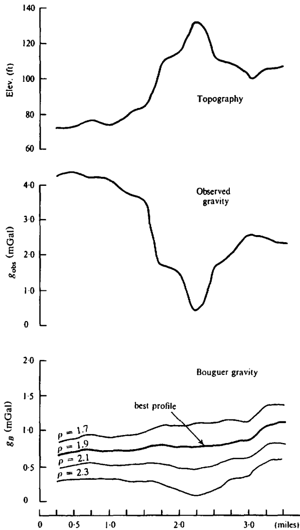
Figure 2.8. Method for estimating surface density.
