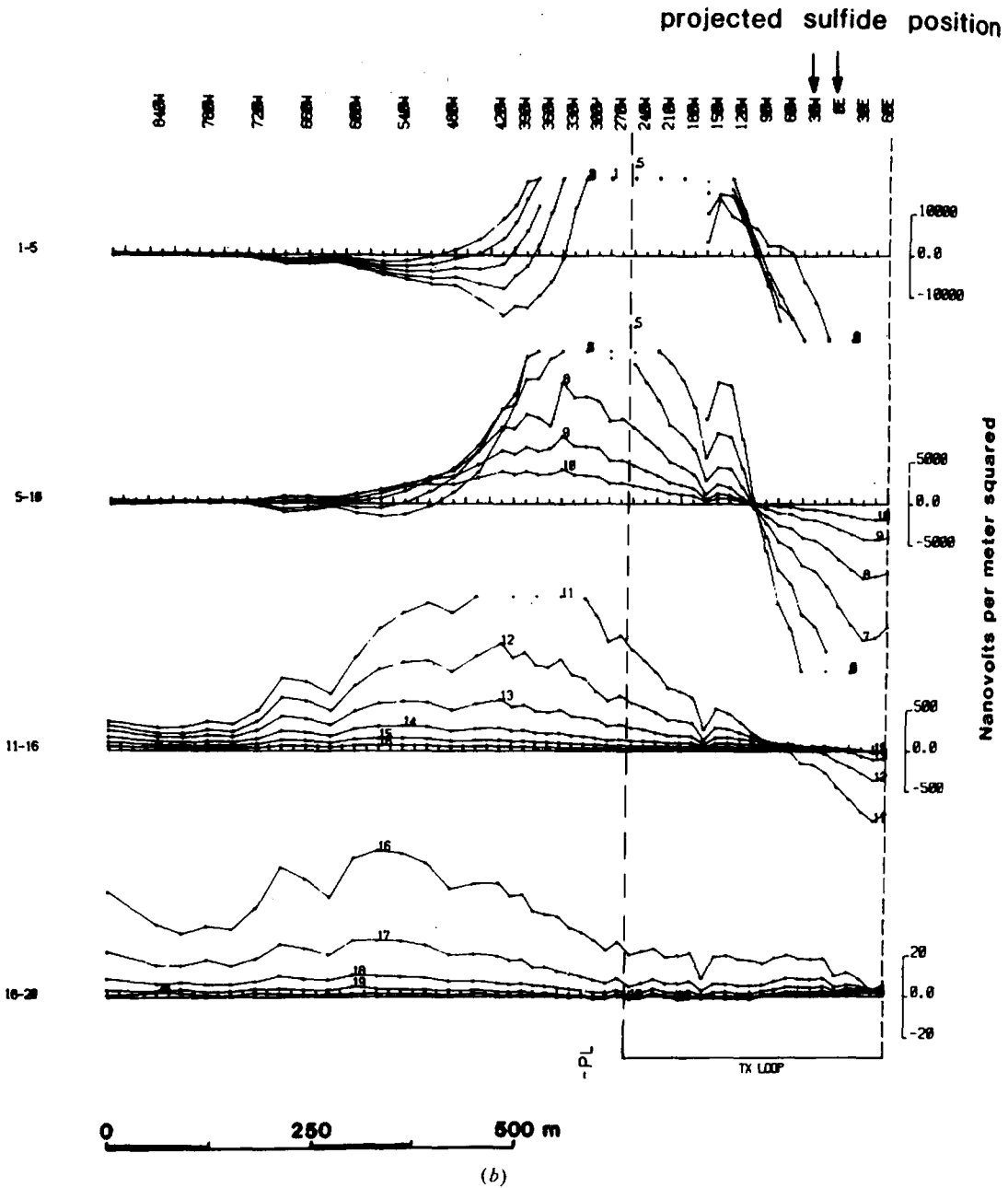
Figure 7.103. (Continued) (b) Horizontal component.
