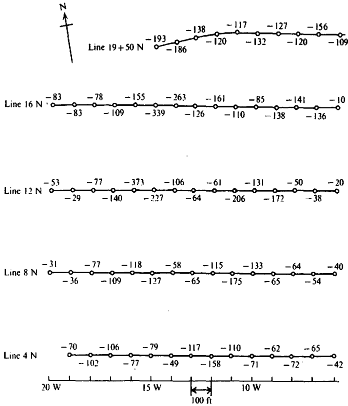
Figure 6.33. SP survey in Southeastern Ontario. Readings in millivolts.
