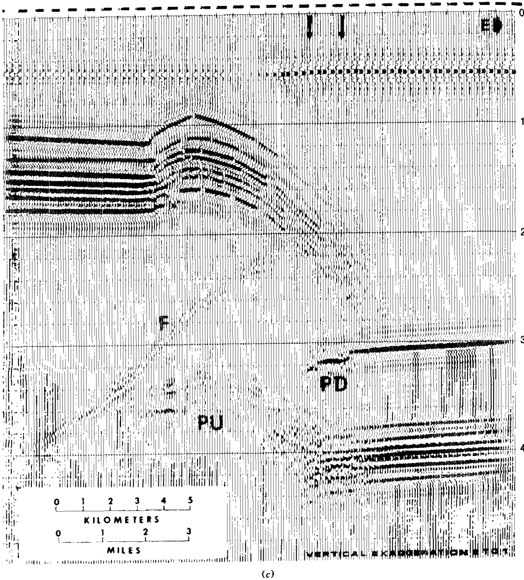
Figure 4.98. (Continued) (c) Seismic section predicted from the model.
