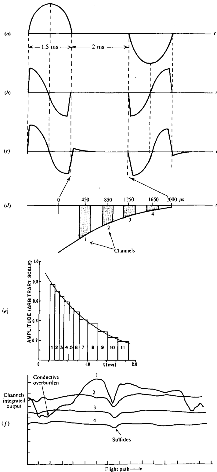
Figure 7.28. Input airborne EM system. (a) Primary magnetic field, H_p . (b) Receiver-coil voltage due to H_p when H_s = 0 . (c) Receiver-coil voltage due to H_p + H_s . (d) Decay signals in the four sampling channels. (e) 11-channel sampling with zero off-time between. (f) Four-channel record over Texas Gulf Sulphur, Timmins, Ontario.
