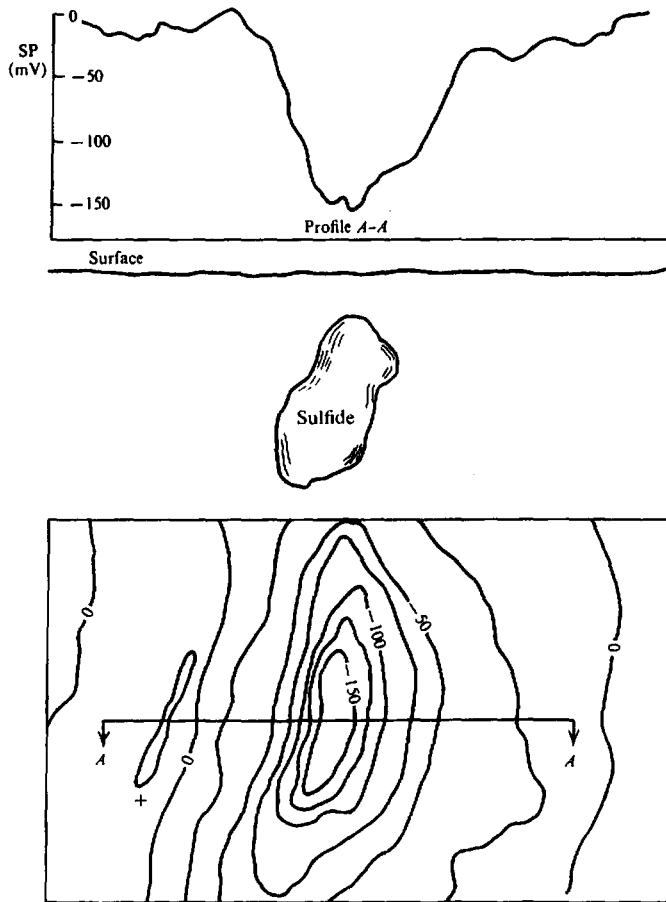
Figure 6.4. Typical SP profile and contours over sulfide body.
