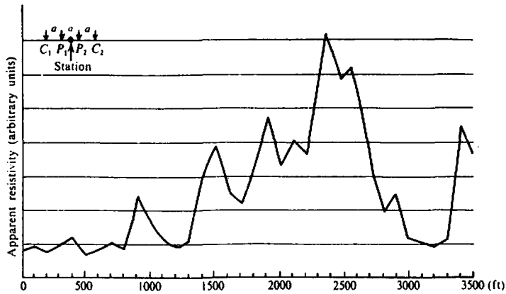
Figure 8.46. Resistivity mapping with Wenner spread over karst topography, Hardin County, Illinois. Station interval = 100 ft, a = 100 ft. (After Van Nostrand and Cook, 1966.)
