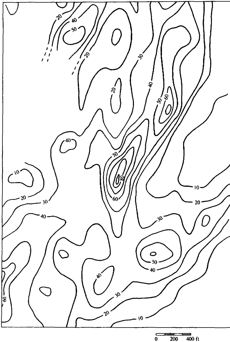
Figure 9.23. Metal-factor contours, double-dipole array: x = 100 ft, n = 1 .
