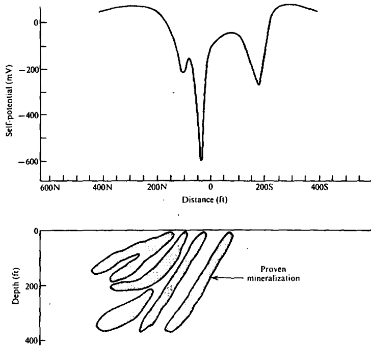
Figure 6.25. SP profile across massive sulfides, Senneterre Area, Quebec.
