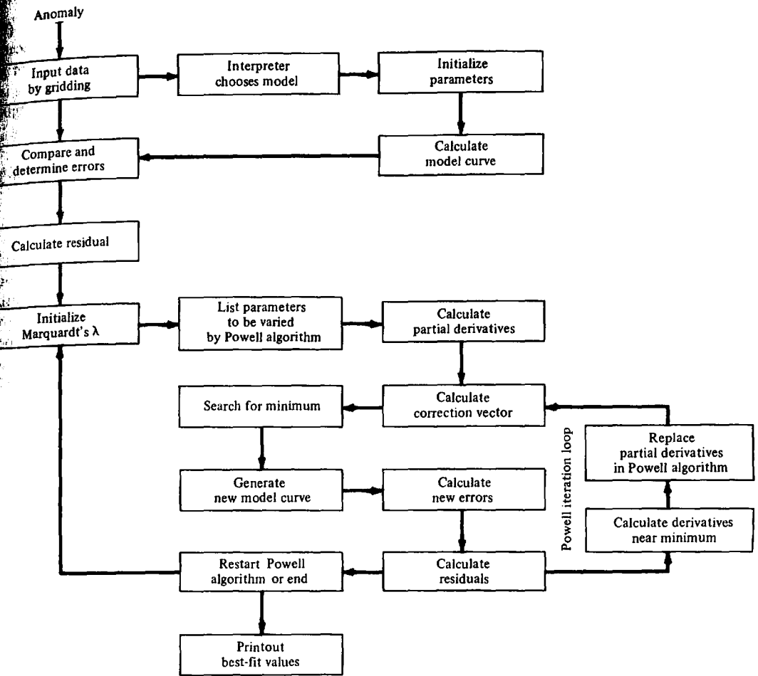
Figure 3.32. Generalized flow chart of computerized interpretation. (From McGrath and Hood, 1973.)
