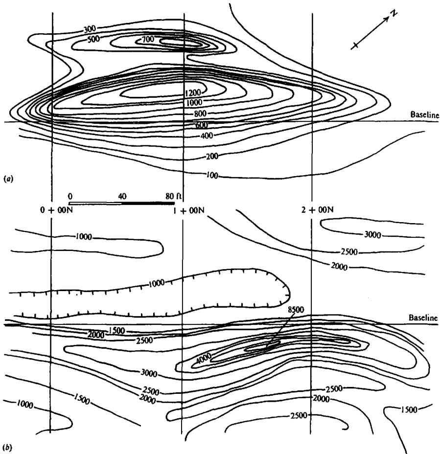
Figure 10.16. Radioactivity and magnetic contours, Northern Canada. (a) Wide-window \gamma -ray flux (counts/s), background 60 counts/s. (b) Vertical-component of the magnetic field (gammas).
