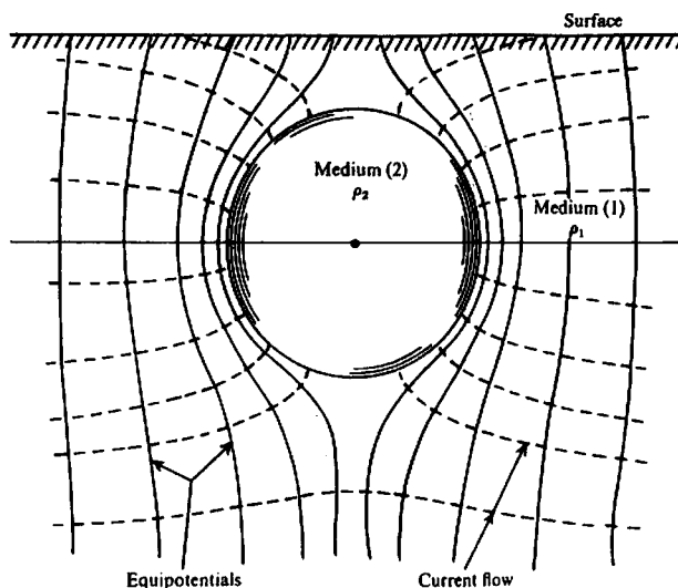
Figure 8.13. Equipotentials and current flow lines for buried conductive sphere.
