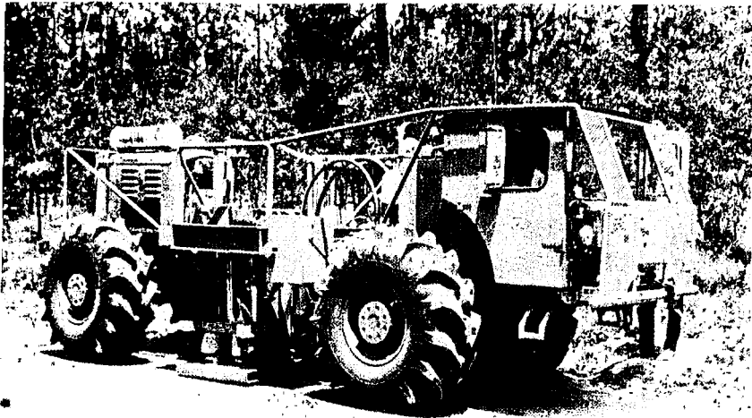
Figure 4.52. Vibrators mounted for off-road survey. (Courtesy Conoco.)
