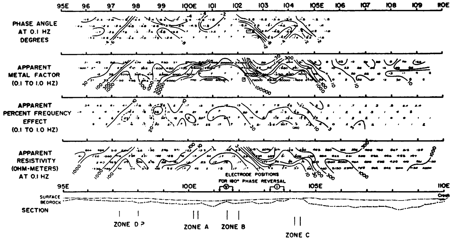
Figure 9.26. Results of an F-D survey in southern New Brunswick, using a double-dipole array: x = 50 ft, n = 1, 2, 3, 4 . (After Scott, 1971.)
