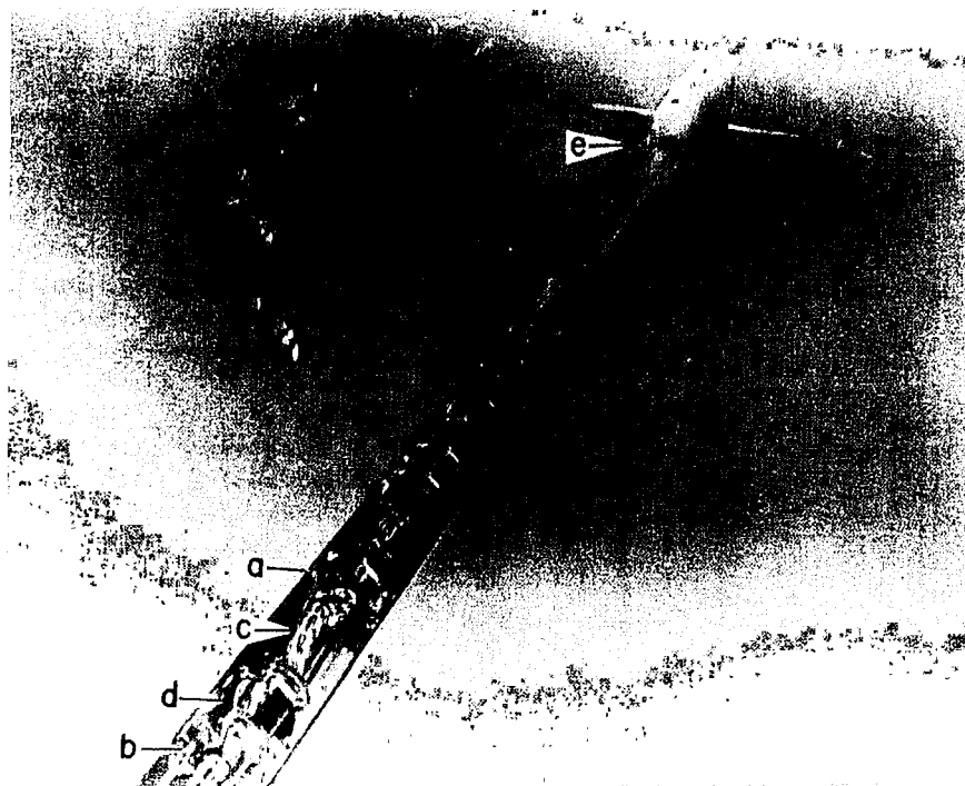
Figure 4.65. Photo of seismic streamer. Plastic spacers (a) are connected by three tensile cables (b). A bundle of electrical conductors (c) passes through holes in the centers of the spacers. A hydrophone is at (d). A depth controller (e) is clamped over the streamer (Courtesy Seismic Engineering.)
