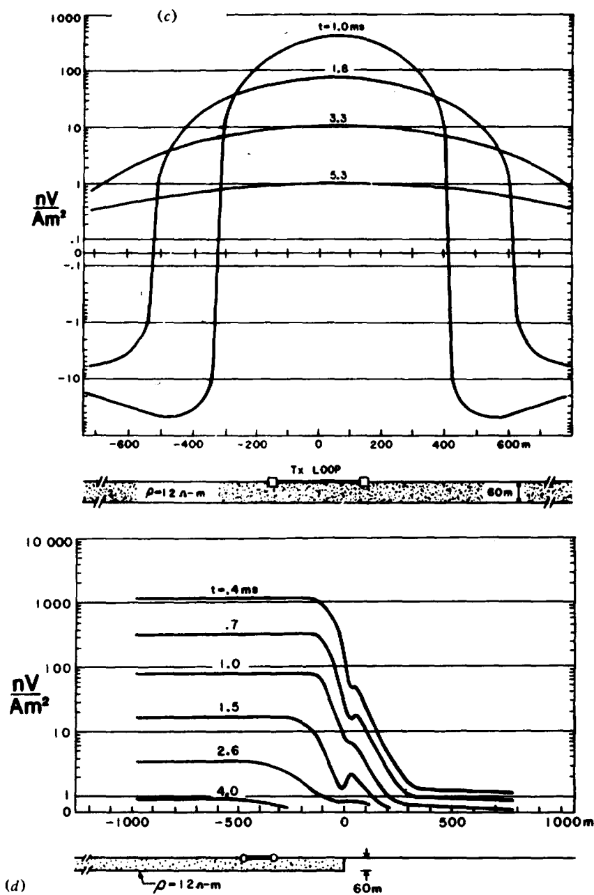
Figure 7.54. (Continued) (c) Tx on 1-D overburden. (d) SIROTEM(1) with 150 m diameter loop over overburden \sim 350 m from edge.
