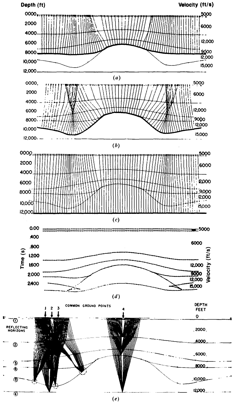
Figure 4.97. Ray-trace modeling of a CMP section. Rays perpendicular to reflectors are bent according to Snell's law as they pass through intervening interfaces. (From Taner, Cook, and Neidell, 1970.) (a), (b), (c) Tracing three reflectors for a North Sea model; (b)/(c) are the top/base of a salt layer. (d) The predicted CMP section. (e) Ray tracing to determine stacking velocity values.
