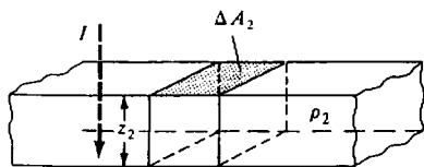
Figure 8.30. Effect of topography on expanding Wenner spread.
