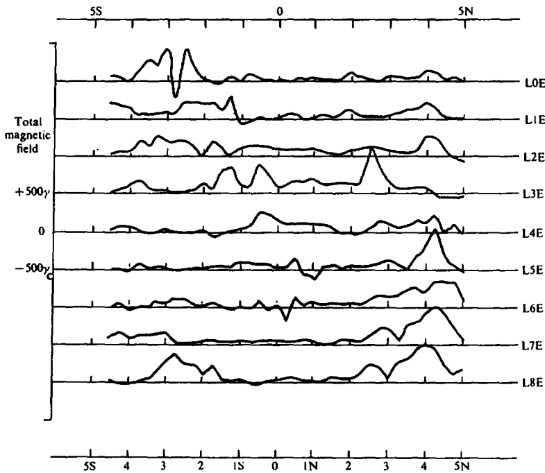
Figure 12.2. Total-field ground-magnetic profiles, Uchi Lake, northwestern Ontario.
