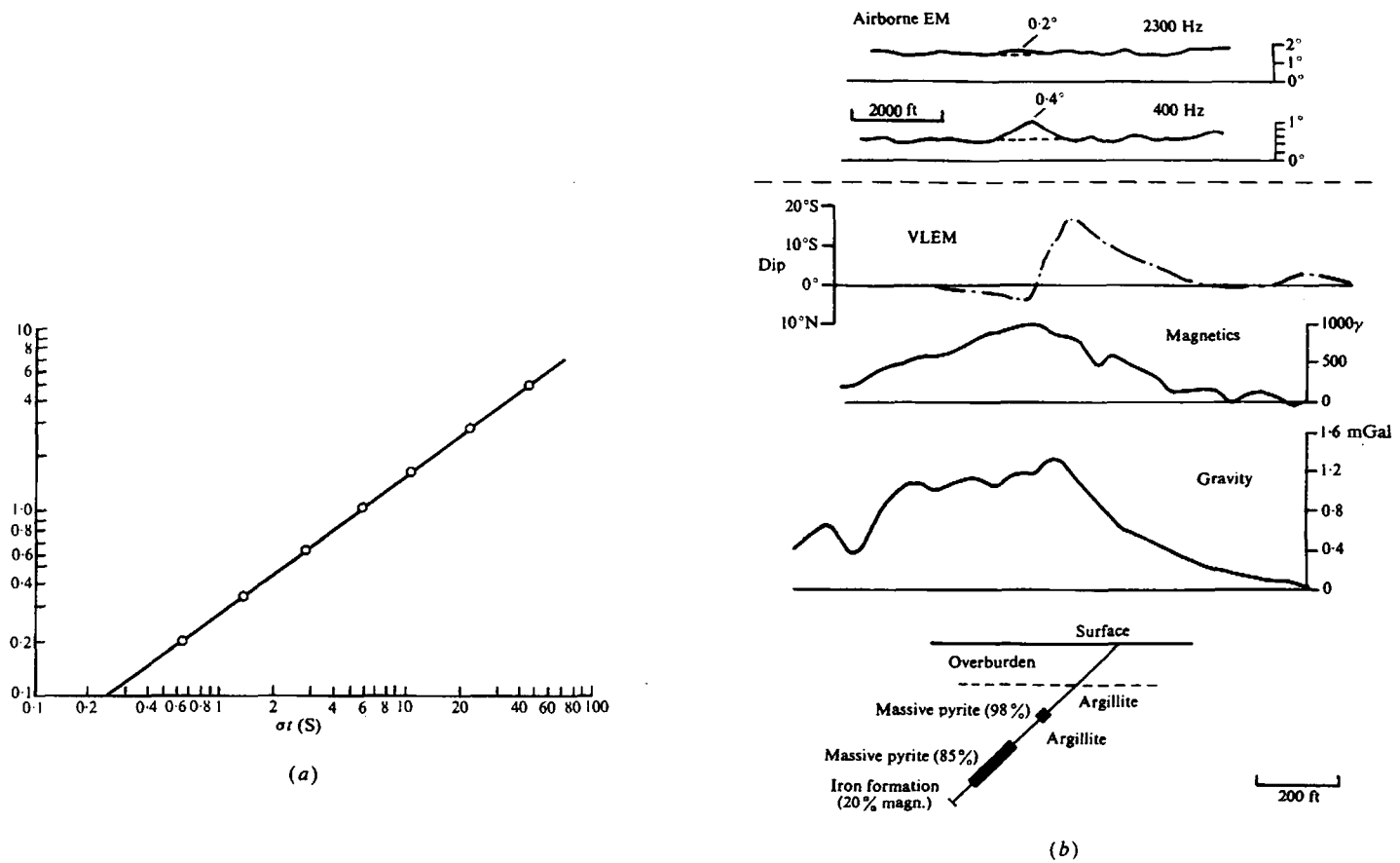
Figure 7.106. Comparison of airborne quadrature EM and several ground methods over various conductors. (After Paterson, 1967.) (a) Curve of TCP versus P , the airborne peak-response ratio over vertical-sheet model; P = (400 \text{ Hz peak}) / (2,300 \text{ Hz peak}) . (b) Comparison with several methods over deep sulfides.
