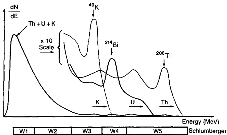
Figure 11.33. Gamma-ray spectra using a NaI crystal detector and energy windows for examining portions of the spectra. (From Schlumberger, 1987.)
