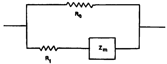
Figure 9.3. Equivalent electrical circuit to simulate the IP effect.
