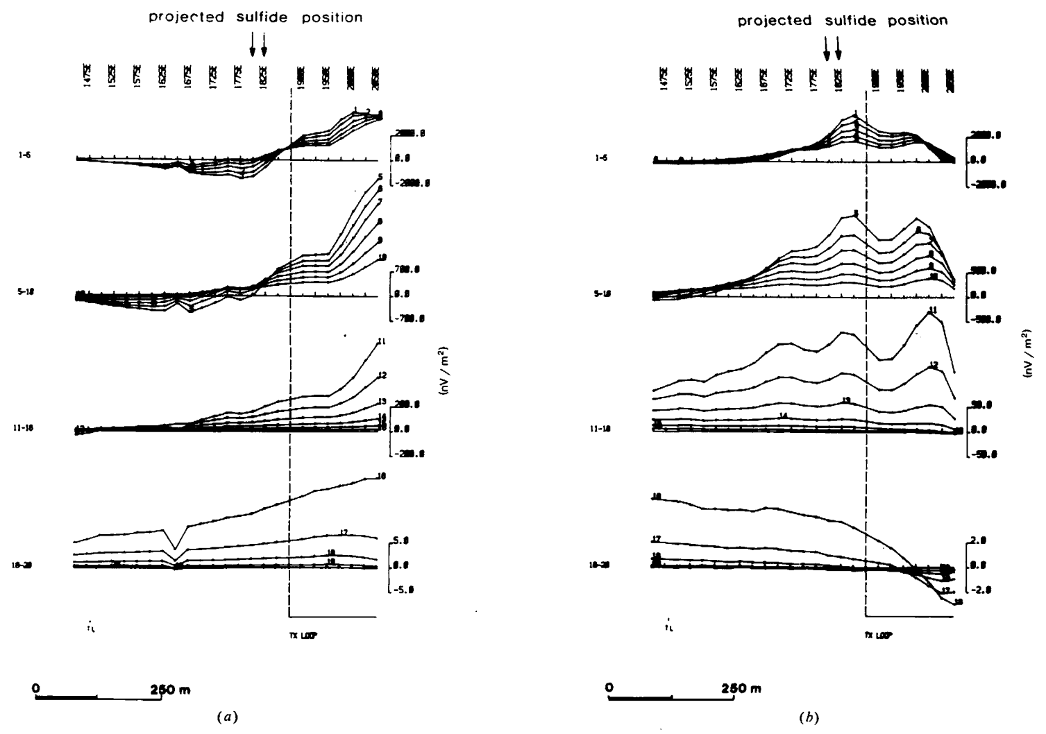
Figure 7.104. EM37 profiles, section 272.2, White Leads prospect, Broken Hill, New South Wales. (After Smith, 1985.) (a) Vertical component. (b) Horizontal component.
