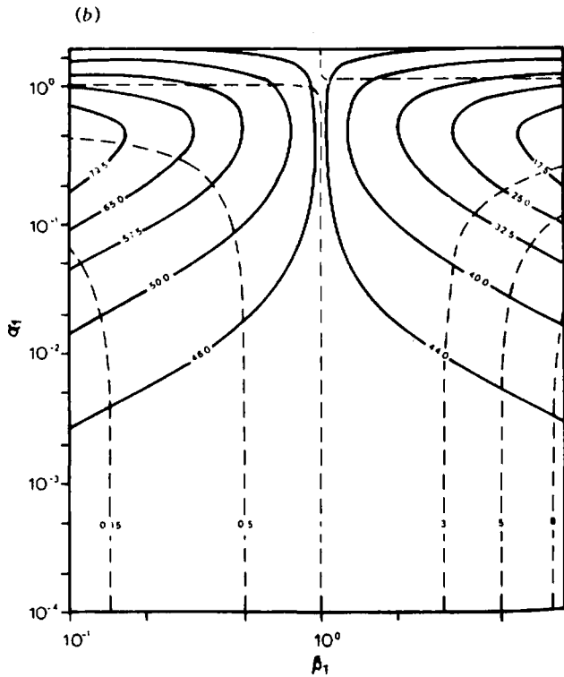
Figure 7.71. Master curves for two-layer VLF resistivity interpretation. (After Mathieson and Crossley, 1982.) (a) Contours of \phi (solid) and |Q_1| (dashed) as functions of \alpha_1 and \beta_1 [Eq. (7.40)]. (b) Enlargement of the central portion of (a).
