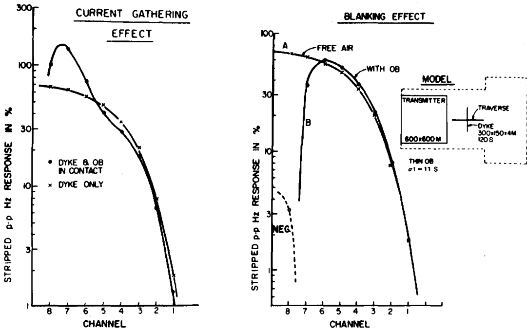
Figure 7.64. Decay plots for the H_z^S anomalies of Figure 7.63. (After West, Macnae, and Lamontagne, 1984.)
