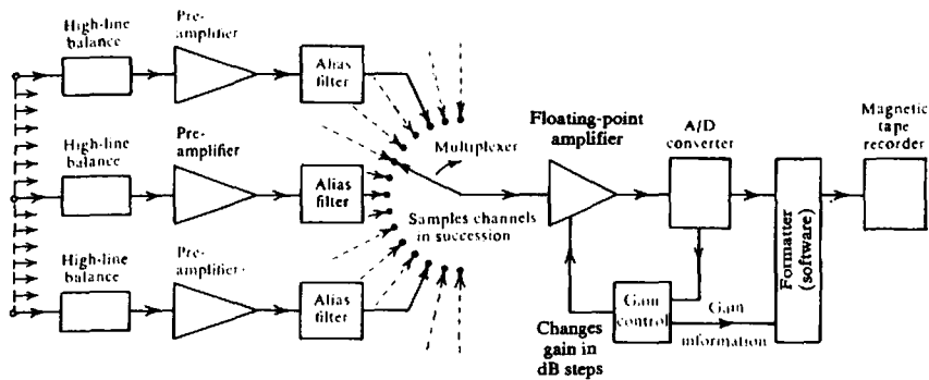
Figure 4.58. Block diagram of digital seismic amplifier.
