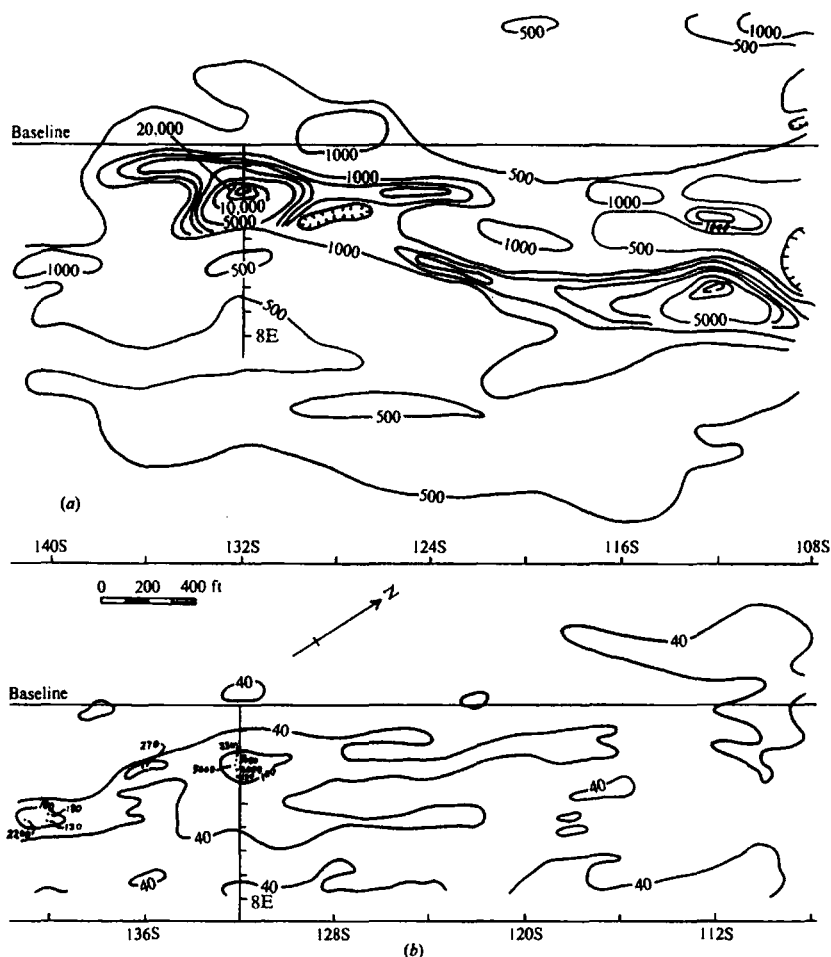
Figure 10.13. Uranium exploration using ground magnetics and radiometrics. (a) Magnetic contours (nT). (b) Radioactivity contours (total \gamma -ray flux in counts/s).
