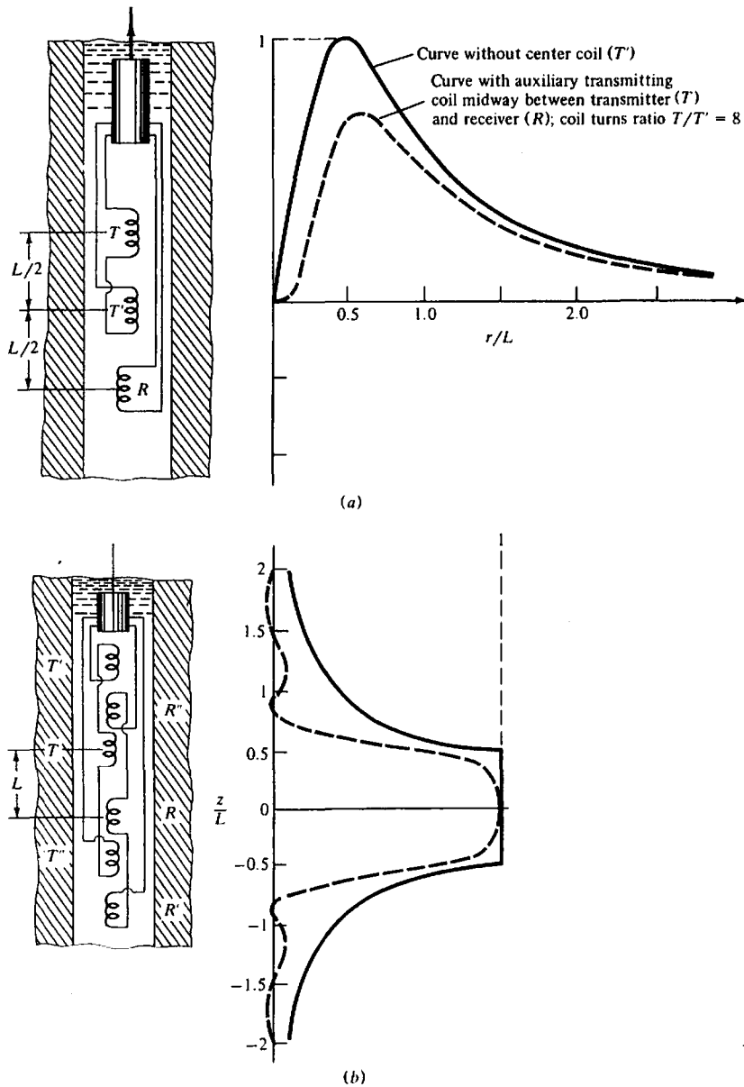
Figure 11.8. Geometric factors for induction sondes without (solid curves) and with (dashed curves) auxiliary coils ( T' , T'' , R' , R'' ). (After Doll, 1949.) (a) Radial factor g(r) . (b) Depth factor g(z) .
