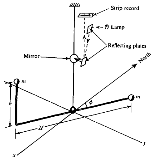
Figure 2.9. Torsion balance (schematic).
