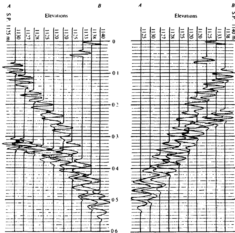
Figure 4.116. First breaks and a reflection on reversed end-on spreads.
