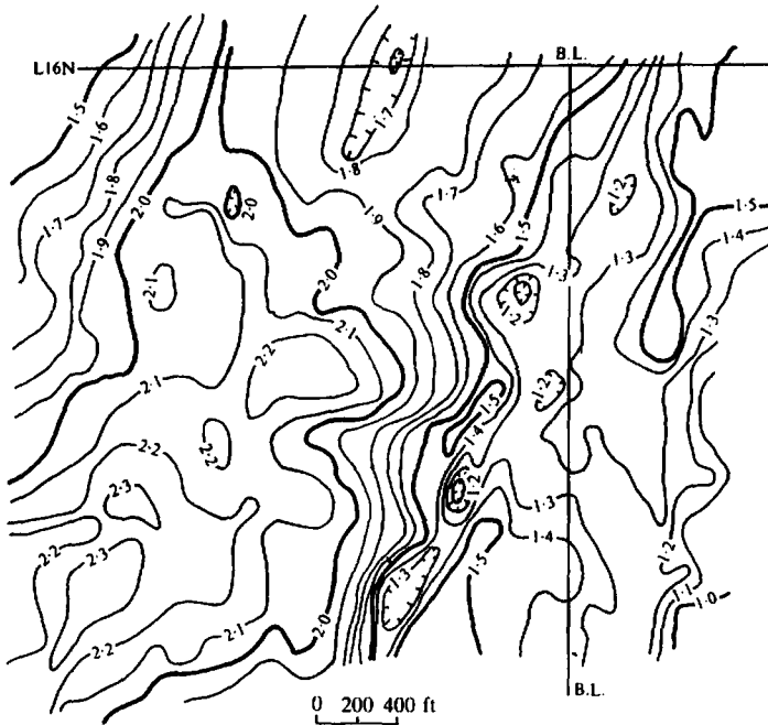
Figure 2.43. Bouguer gravity contours, eastern Nova Scotia; C.I. = 0.1 \text{ mGal} .
