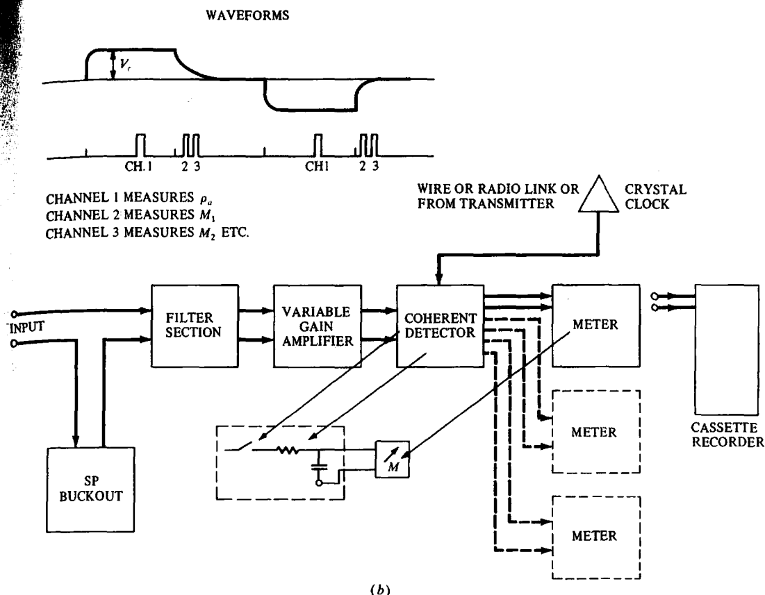
Figure 9.6. (Continued) (b) F-D receiver. (After Sumner, 1976.)
