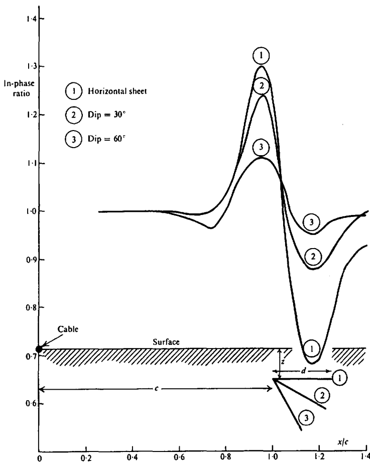
Figure 7.38. Effect of dip on Turam profiles over sheet of finite depth extent. z/d = \frac{1}{2} ; z/c = \frac{1}{8} .
