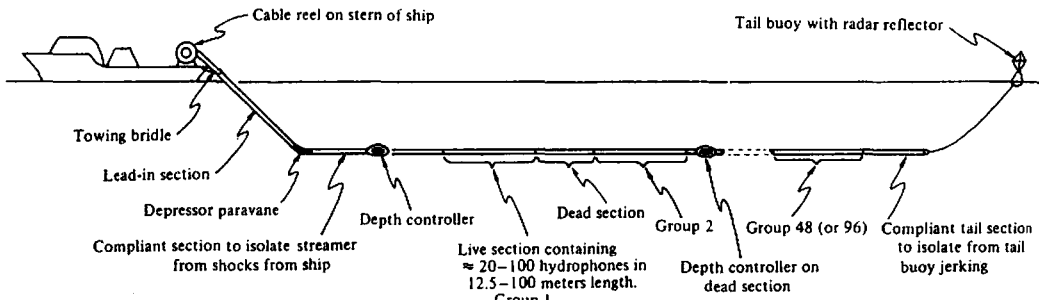
Figure 4.64. Streamer. (After Sheriff, 1984.)
