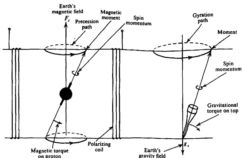
Figure 3.9. Proton precession and spinning-top analogy.
