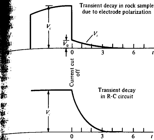
Figure 9.1. Comparison of IP and R-C decay curves.
