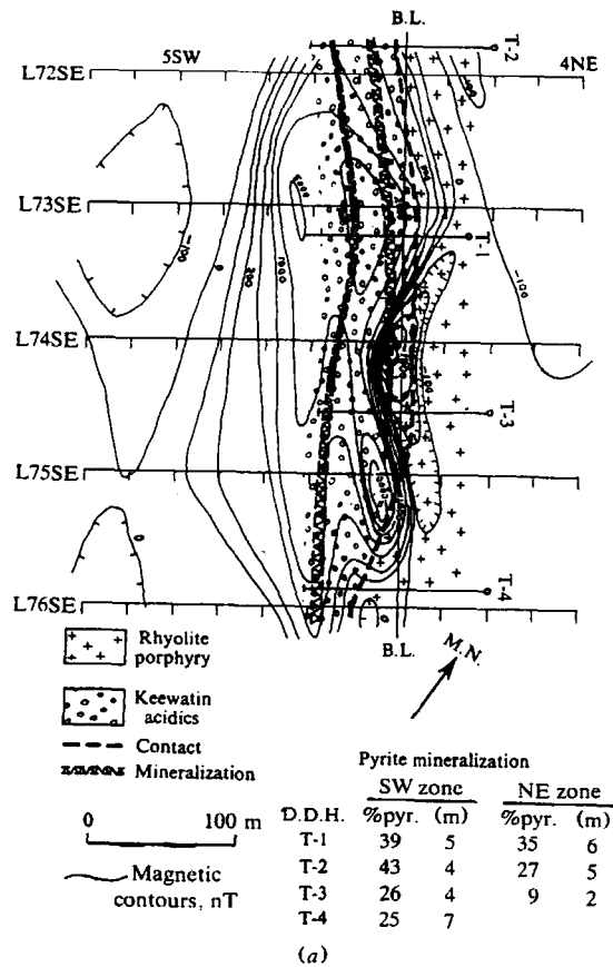
Figure 3.28. Ground magnetic survey over pyrite mineralization, Barraute, northwest Quebec. (a) Magnetic map. (b) Attempt to match profiles on lines 75SE and 73SE.
