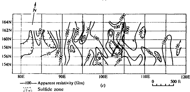
Figure 12.3. Results of different electrical surveys, Atlantic Nickel Property, southern New Brunswick. (a) SP profiles. (b) HLEM profiles; frequency 876 Hz, coil separation 200 ft. (c) Telluric contour map; frequency 8 Hz, electrode spacing 100 ft.
