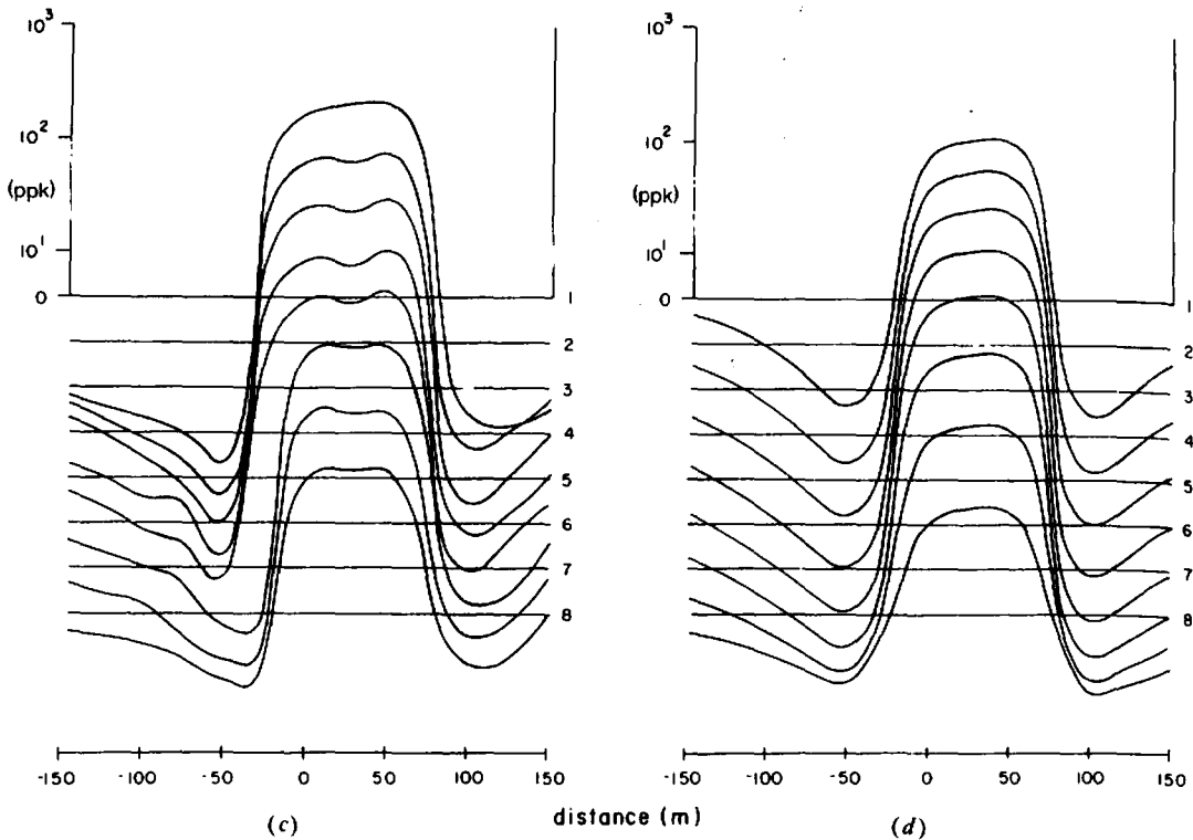
Figure 7.101. (Continued) (c) Field data over Maydan deposit; coil spacing 100 m. (d) Best-fit plate response to profile in (c); \ell = d = 600 m, z = 20 m, dip = 80^\circ , TCP = 60 S.
