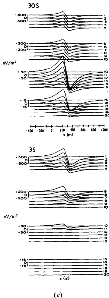
Figure 7.53. (Continued) (c) Variation in \partial H_z/\partial t with conductance; z = 50 m, dip = 90^\circ .
