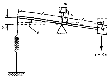
Figure 2.11. Basic principle of the unstable (Thyssen) gravimeter. (After Dobrin, 1960.)
