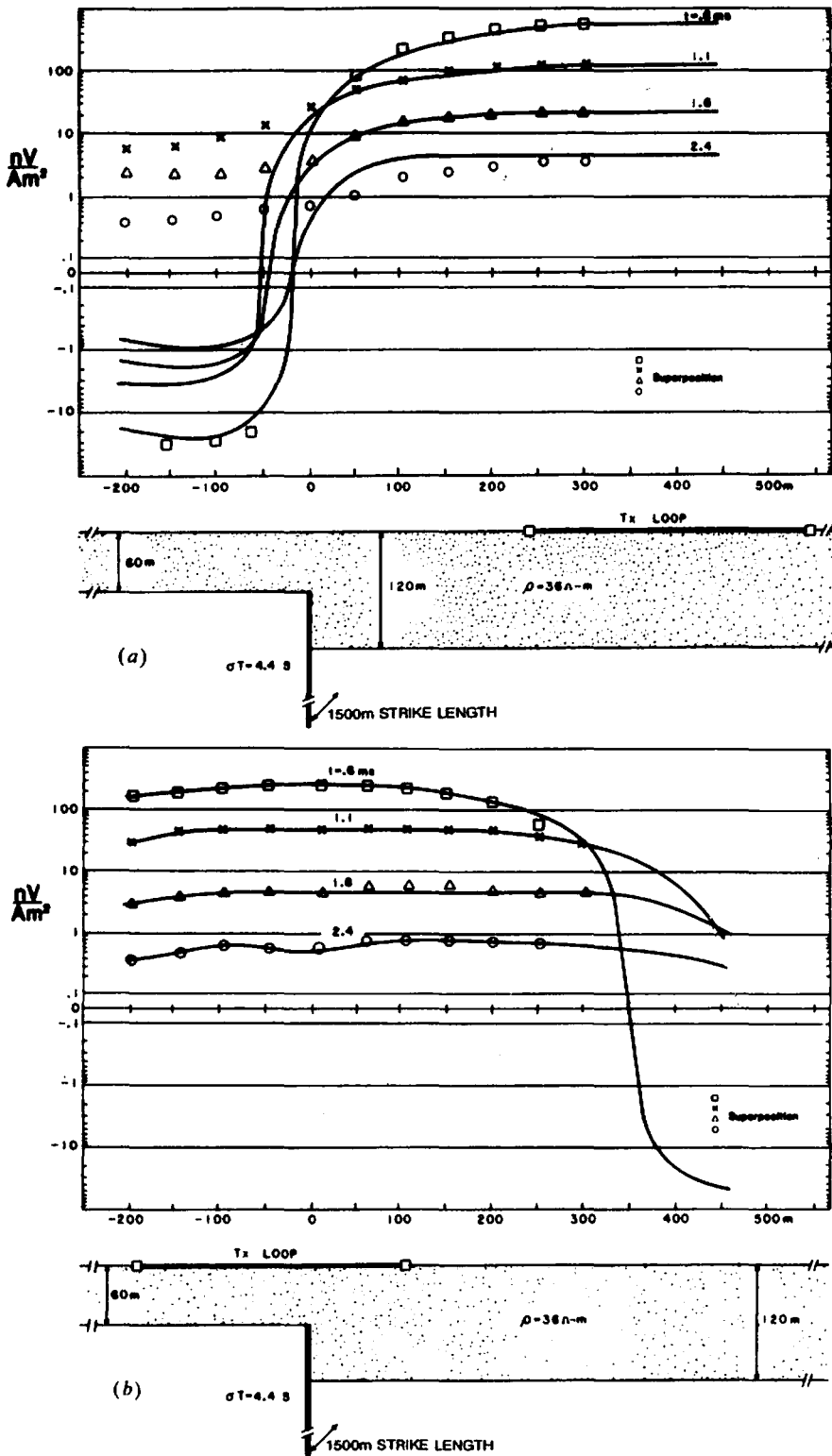
Figure 7.59. Comparison of fixed-loop and coincident loop results over a model consisting of a semi-infinite vertical-sheet conductor in contact with conducting overburden at a step in the latter. (After Spies and Parker, 1984.) (a) Fixed-loop system with Tx loop located several hundred meters from the step. (b) As in (a) except that the Tx loop straddles the step.
