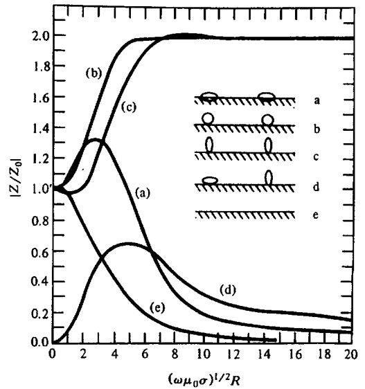
Figure 7.72. Mutual impedance ratios for systems (a) to (e) in Equation (7.41) as a function of (\omega\mu_0\sigma)^{1/2}R . (After Wait, 1955.)
