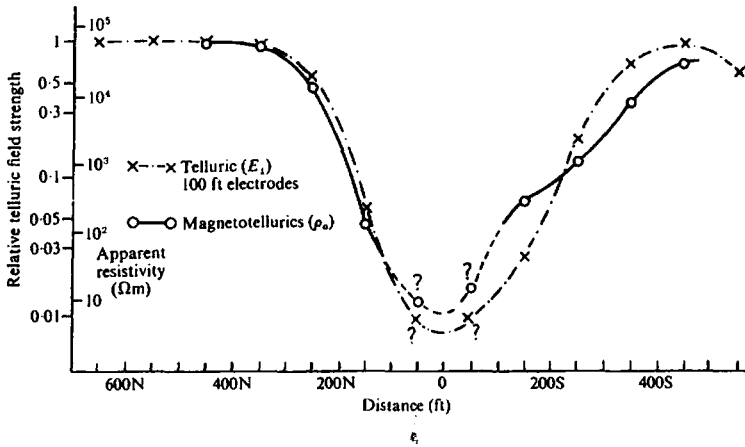
Figure 6.37. 8 Hz magnetotelluric profile, Northern Quebec.
