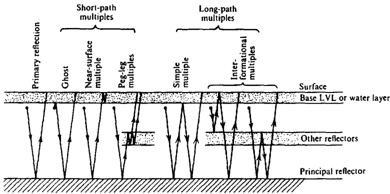
Figure 4.40. Types of multiples.
