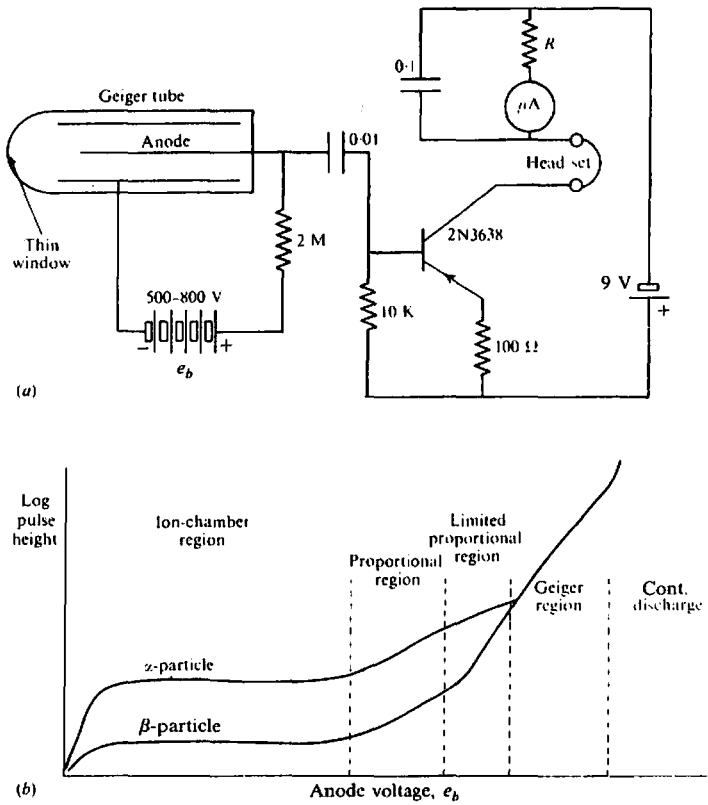
Figure 10.4. Geiger-Müller counter. (a) Simplified counter circuit. (b) Geiger-tube characteristics as a function of anode voltage.
