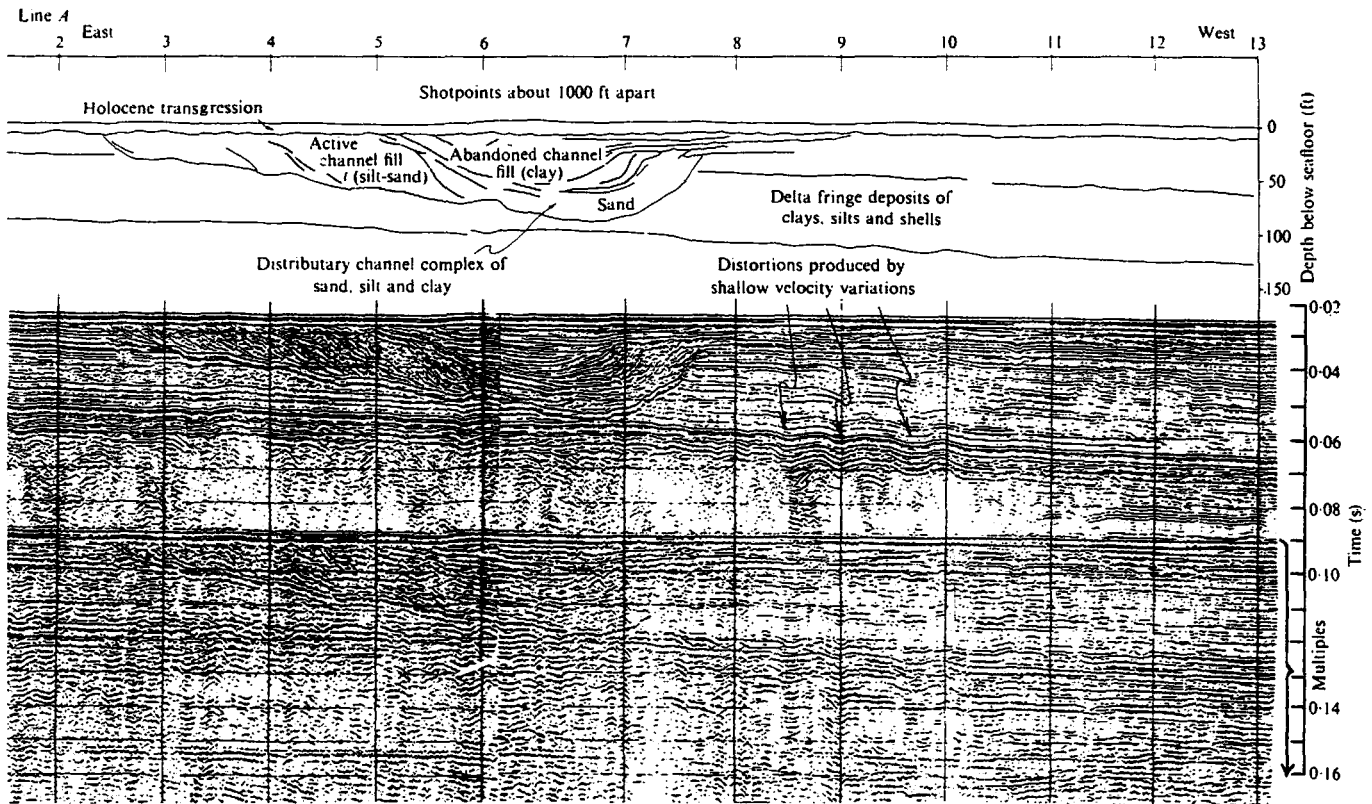
Figure 4.108. Profiler record showing subbottom deposits. (From King, 1973.)
