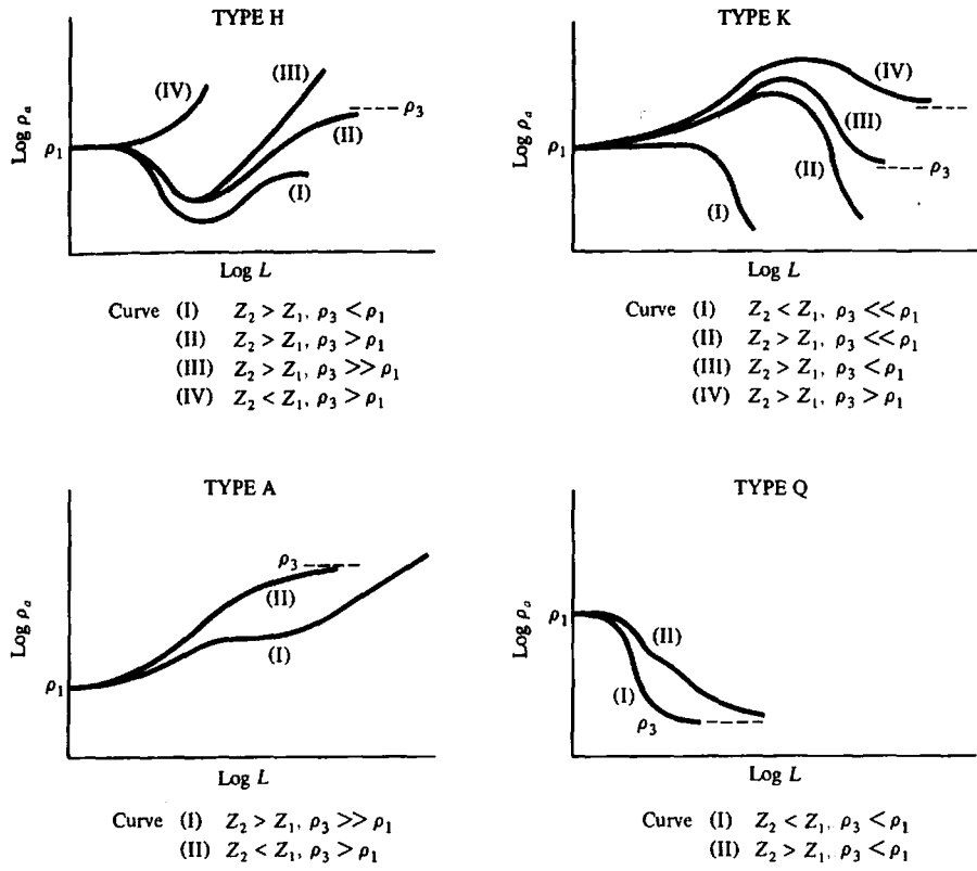
Figure 8.24. Various types of sounding curves over multilayer structures of three or more beds.
