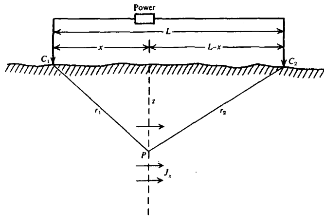
Figure 8.5. Determining the current density in uniform ground below two surface electrodes.
