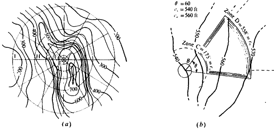
Figure 2.4. Use of terrain chart with topographic map. (a) Terrain chart overlying map. (b) Enlarged view of a single zone.
