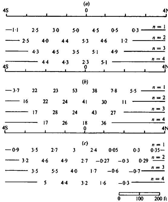
Figure 9.21. Time- and frequency-domain IP pseudodepth plots. Double-dipole array, x = 100 ft. (a) Percent frequency effect. (b) Metal factor (mhos per foot). (c) Chargeability (milliseconds).
