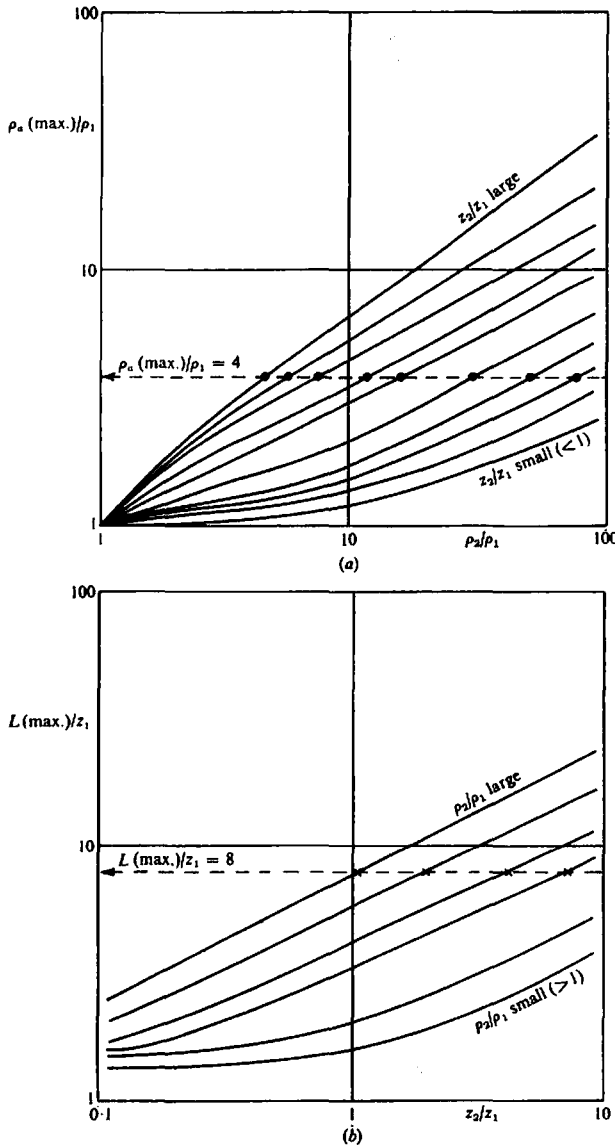
Figure 8.25. Schlumberger array - characteristic curves for three layers with type-K curves (see Fig. 8.24). (After Keller and Frischknecht, 1966.) (a) Plots of \rho_e(\text{max.})/\rho_1 versus \rho_2/\rho_1 for various z_2/z_1 ratios. (b) Plots of L(\text{max.})/z_1 versus z_2/z_1 for various \rho_2/\rho_1 ratios.
