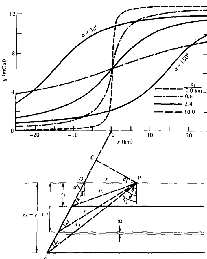
Figure 2.30. Gravity effect of a semiinfinite slab. t = 300 \text{ m} , \alpha = 90^\circ except where otherwise noted on the curves. \rho = 1 \text{ gm/cm}^3 .
