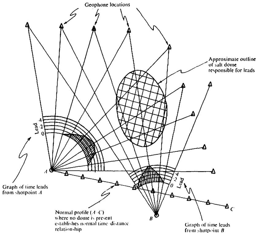
Figure 4.72. Fan shooting. (After Nettleton, 1940.)
