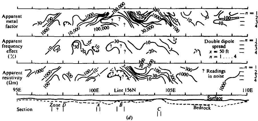
Figure 12.3. (Continued) (d) IP and resistivity pseudodepth plots, double-dipole spread, x = 50 ft, n = 1, 2, 3, 4 .
