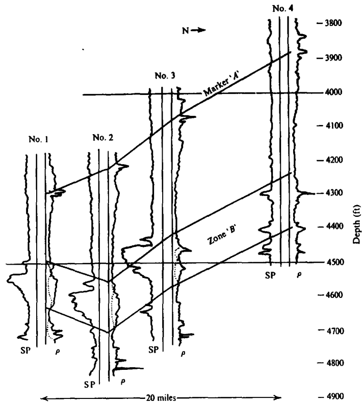
Figure 11.15. Well-log correlation. The convention for plotting well logs is to show an SP or \gamma -ray log to the left of the borehole and a resistivity log to the right. (After Pirson, 1970.)
