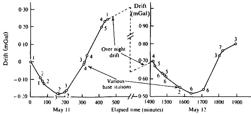
Figure 2.15. Gravimeter drift during a field survey.
