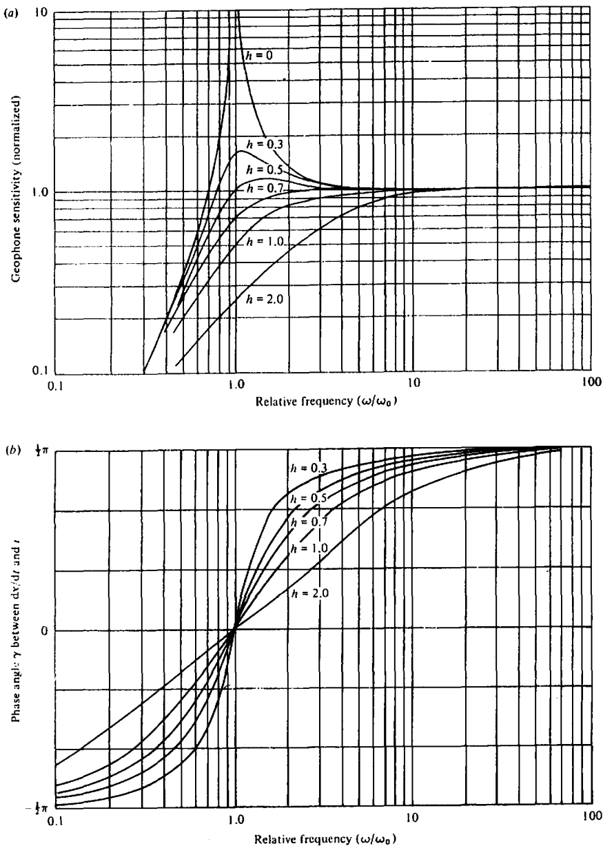
Figure 4.54. Geophone response curves. (After Dennison, 1953) (a) Amplitude of output relative to input. (b) Phase of output relative to input.
