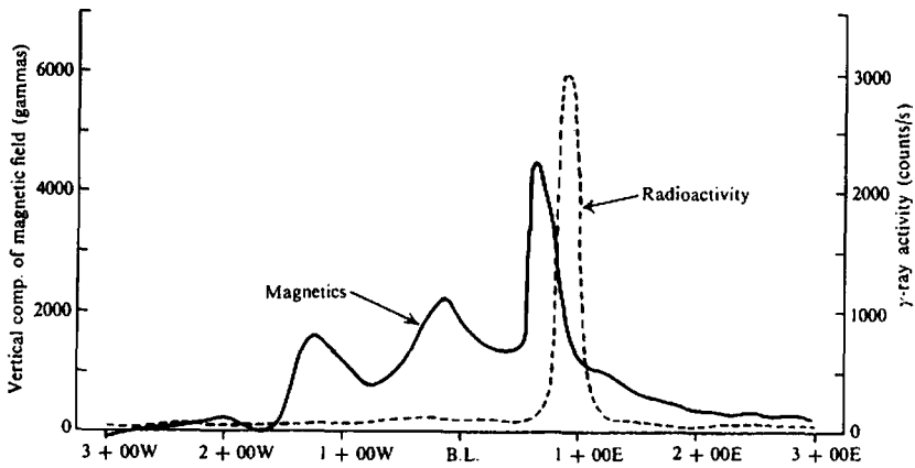
Figure 10.18. Radiometric and magnetic profiles from a survey for base-metals plus uranium.
