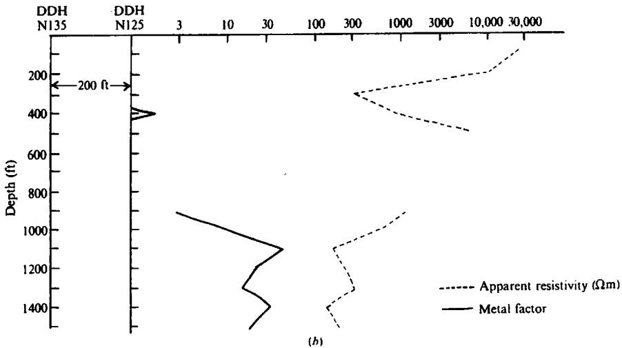
Figure 11.49. Combined IP-electrical survey to locate orebody at depth, Lac Dufault, Quebec. (From Salt, 1966.) (a) Plan of orebody and diamond-drill holes. (b) IP logs in DDH N125 and N135.
