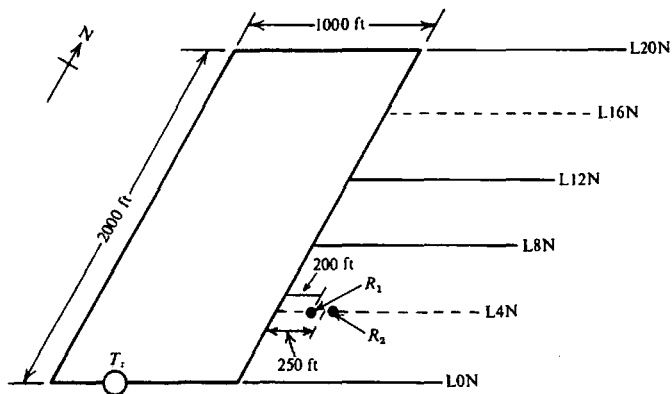
Figure 7.114. Model Turam configuration.
