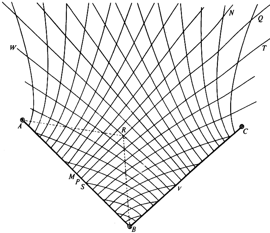
Figure B.2. Hyperbolic coordinates for radionavigation system.
