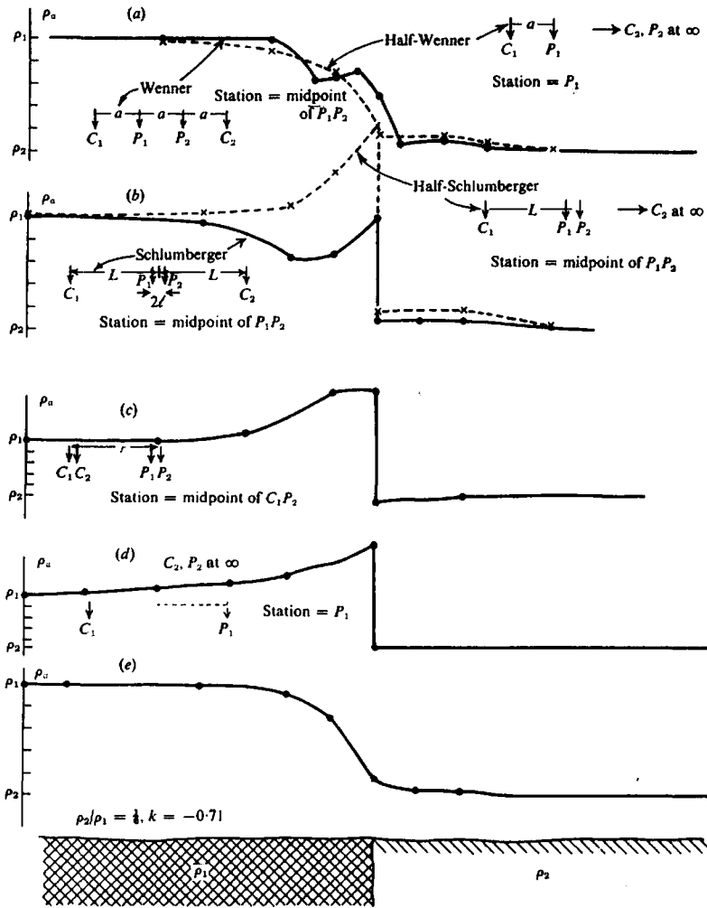
Figure 8.34. Profiles over a vertical contact using different electrode spreads. (a) Wenner spread. (b) Schlumberger spread. (c) Double-dipole spread. (d) Spread with fixed C_1 , movable P_1 . (e) Schlumberger broadside spread.
