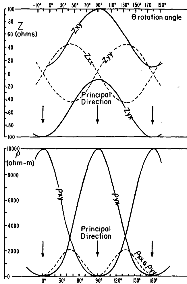
Figure 6.24. Rotation of axes for two-dimensional model with Z'_{xy} = 100 \Omega and Z'_{yx} = 10 \Omega .
