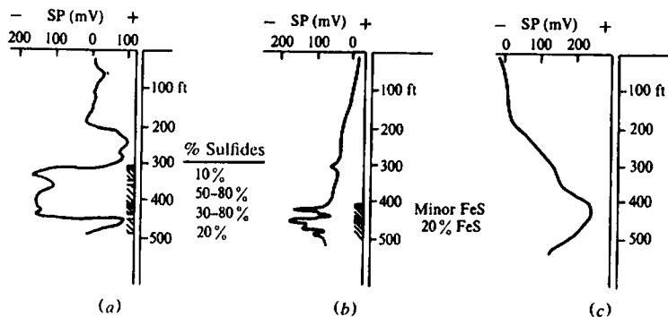
Figure 11.13. Characteristic SP curves in mineral zones. (a), (b) Logs through sulfide zones. (c) Log near a massive pyrite zone not intercepted in the borehole.
