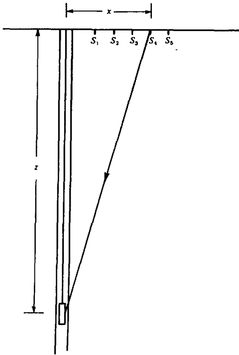
Figure 4.66. Shooting a well for velocity.
