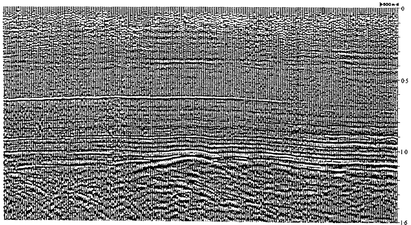
Figure 4.107. Seismic section with relative amplitudes preserved. The local increased amplitude of the reflection just below 0.6 s results from a gas accumulation. Such a "bright spot" is one of several hydrocarbon indicators. (Courtesy Chevron Oil Co.)
