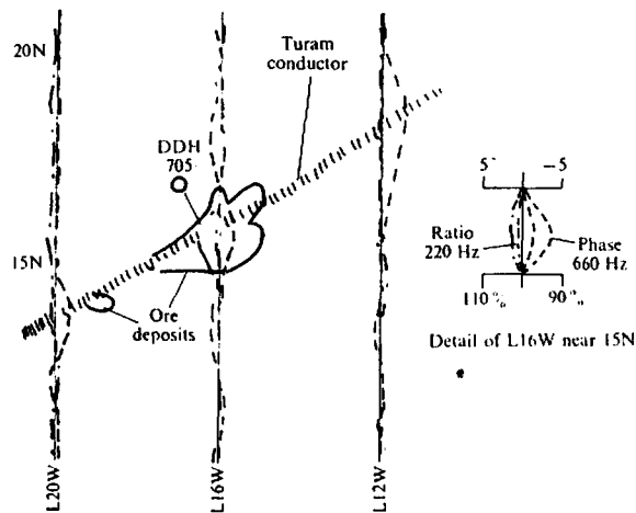
Figure 12.1. Magnetics, IP, and Turam results, Louvicourt area, Quebec. (a) Magnetic and IP profiles, L16W, and vertical section. (b) Turam results; loop located at 0 + 00N .
