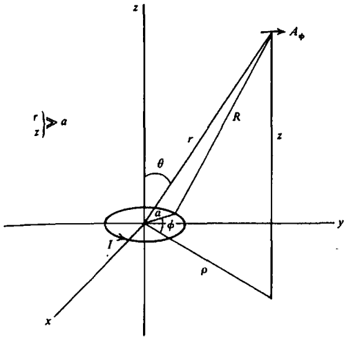
Figure 7.3. Field of a small circular coil at a point outside the plane of the loop.
