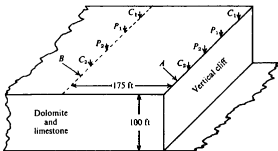
Figure 8.30. Effect of topography on expanding Wenner spread.
