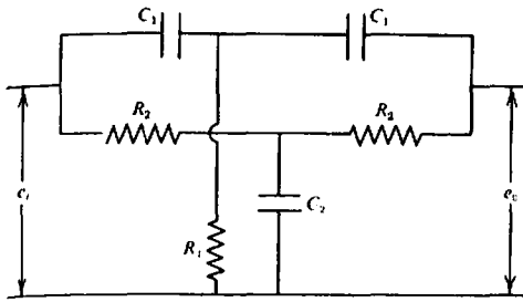
Figure 7.13. Twin-T network for EM receivers. \omega^2 = 1/(2C_1^2R_1R_2) = 2/(C_1C_2R_2^2) . Generally R_2 \approx 2R_1 , C_2 \approx 2C_1 for convenience in design.
