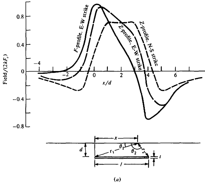
Figure 3.21. Thin horizontal plate of finite width, t/l = 0.125 . (a) Profiles for l = 60^\circ , \beta = 0^\circ and 90^\circ , d/l = 0.25 .
