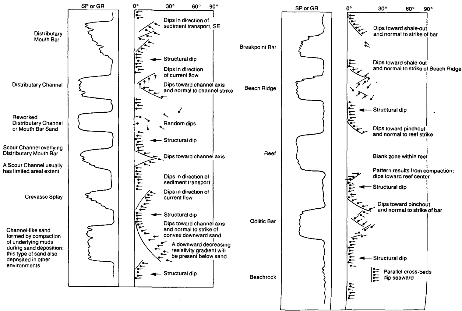
Figure 11.18. Stratigraphic patterns in SP (or \gamma -ray) and dipmeter data. (From Gilreath, 1987.)
