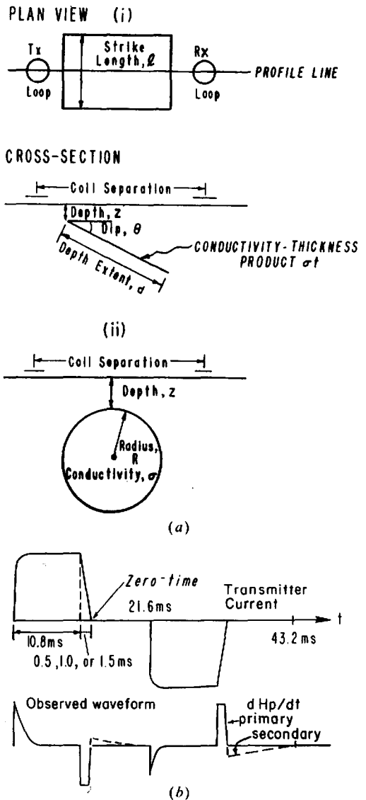
Figure 7.49. PEM(1) moving-source TDEM. (After Bartel and Hohmann, 1985.) (a) Geometry of thin-plate and sphere models. (b) Waveform for 10.8 ms pulse.
