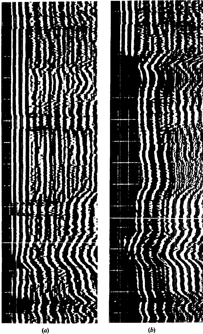
Figure 11.26. Microseismogram log used to indicate cement bonding. (Courtesy Welex.) (a) The first arrival is a strong signal transmitted through the casing before cementing. (b) After bonding the casing to the formation with cement, the first arrival is energy which travels through the formation.
