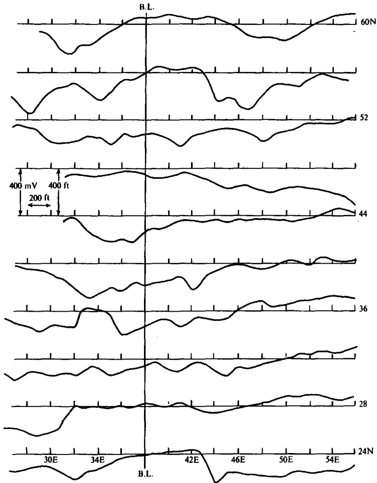
Figure 6.32. SP survey in Eastern Nova Scotia.
