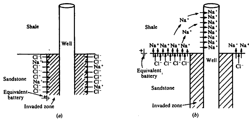
Figure 11.10. The self-potential effect in a sand-shale section. (Courtesy Schlumberger, Ltd.) (a) Liquid-junction (diffusion) potential. (b) Shale (Nerst) potential.
