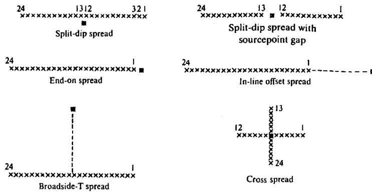
Figure 4.47. Types of reflection spreads. The symbols x and O represent geophone groups and sourcepoints, respectively.
