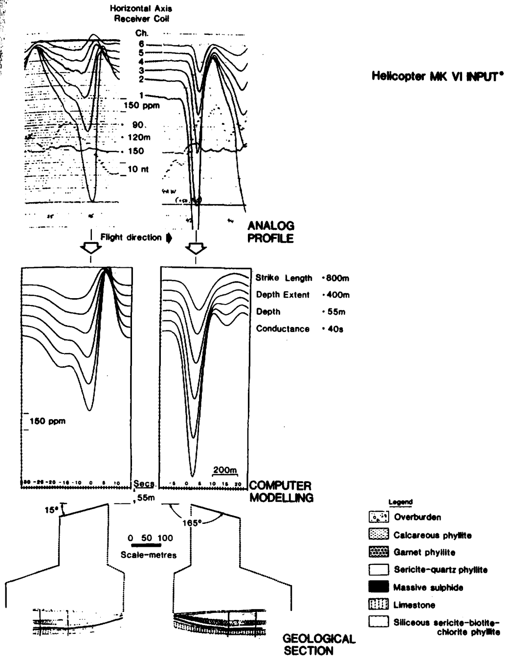
Figure 7.108. (Continued) (b) Goldstream sulfide body (Cu, Zn, Ag). In lower half of top set of profiles, solid line is elevation, dotted line is aeromagnetics.
