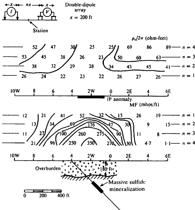
Figure 9.18. Frequency-domain IP results for massive sulfides overlain by thick conductive overburden.
