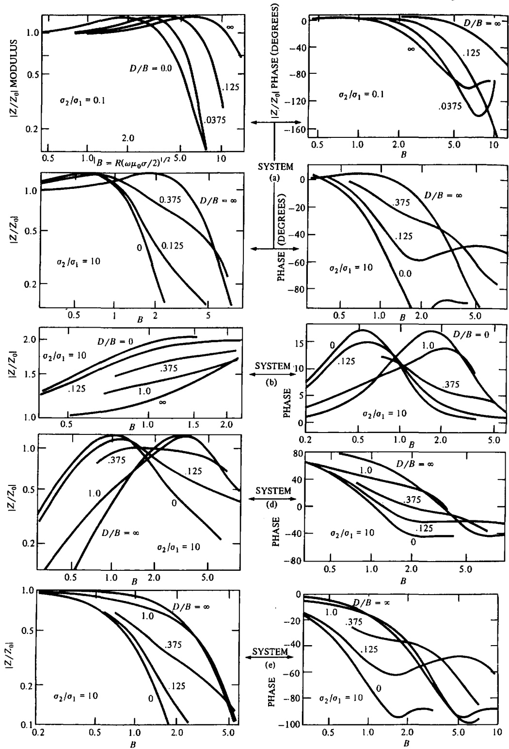
Figure 7.73. Modulus and phase of mutual coupling ratio ( Z/Z_0 ) for systems (a), (b), (d), and (e) in Equations (7.41) over a two-layer earth. (After Frischknecht, 1967.)
