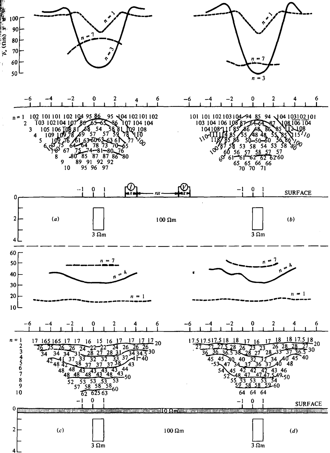
Figure 8.38. Resistivity finite-difference modeling; profiles and pseudodepth plots for the dipole-dipole array of Figure 9.8a. (After Dey and Morrison, 1979.) (a) 3-D block, strike length = 6 units. (b) 2-D block, infinite strike length. (c) and (d) same as (a) and (b) with conductive overburden 0.5 units thick, \rho = 10 \Omega m .
