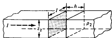
Figure 8.31. The equivalence principle (schematic). (a) \rho_1 < \rho_2 > \rho_3 , \rho_2 z_2 = \text{constant} . (b) \rho_1 > \rho_2 < \rho_3 , \rho_2 / z_2 = \text{constant} .
