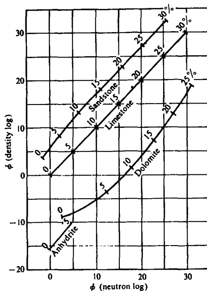
Figure 11.42. Porosity cross-plot. (Courtesy Schlumberger Ltd.)
