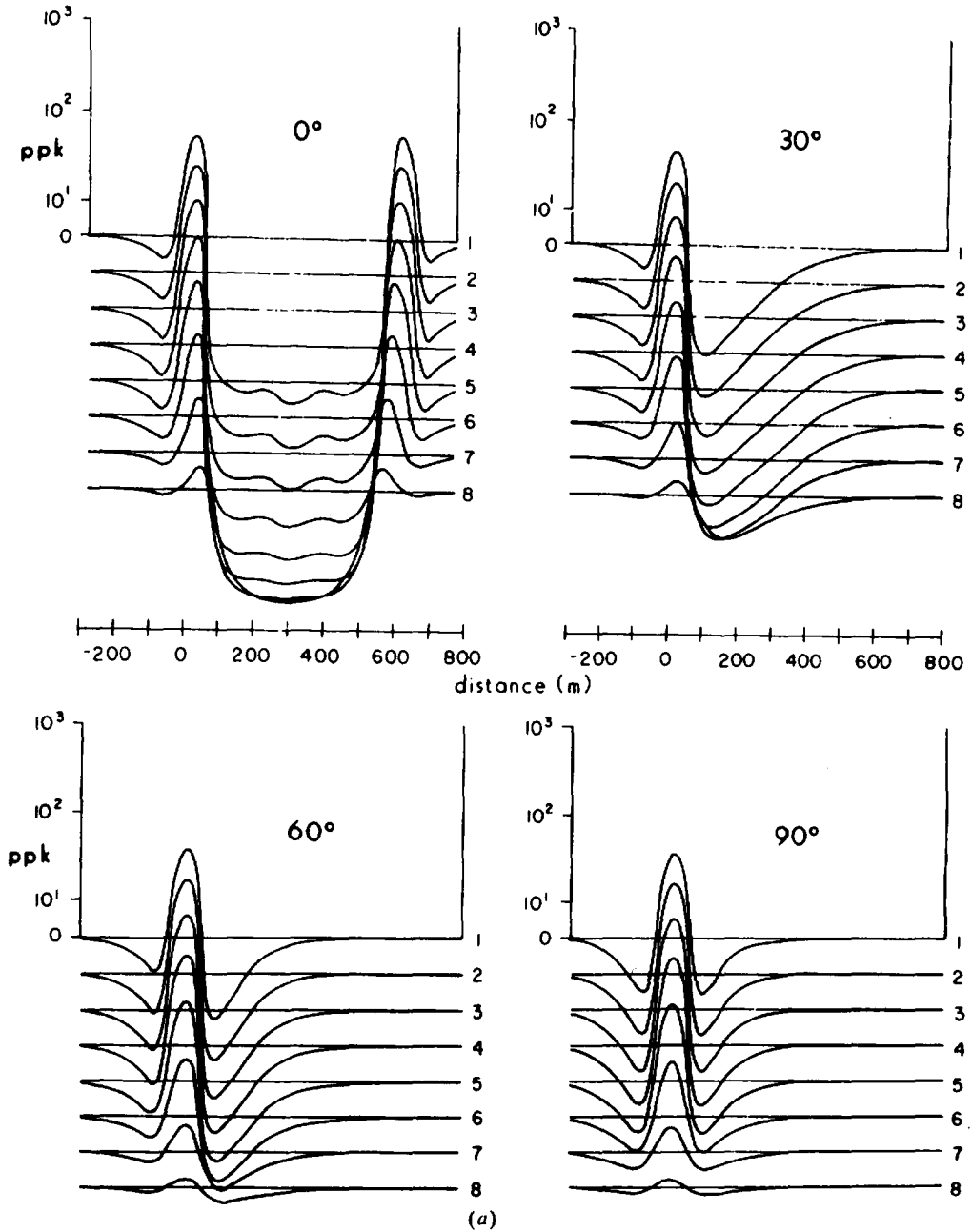
Figure 7.50. PEM(1) response to a dipping sheet as a function of dip, depth, and TCP. \ell = d = 600 m, T-R = 100 m, TCP = at = 30 S [except in (d)]. (After Bartel and Hohmann, 1985.) (a) Effect of dip; z = 50 m.
