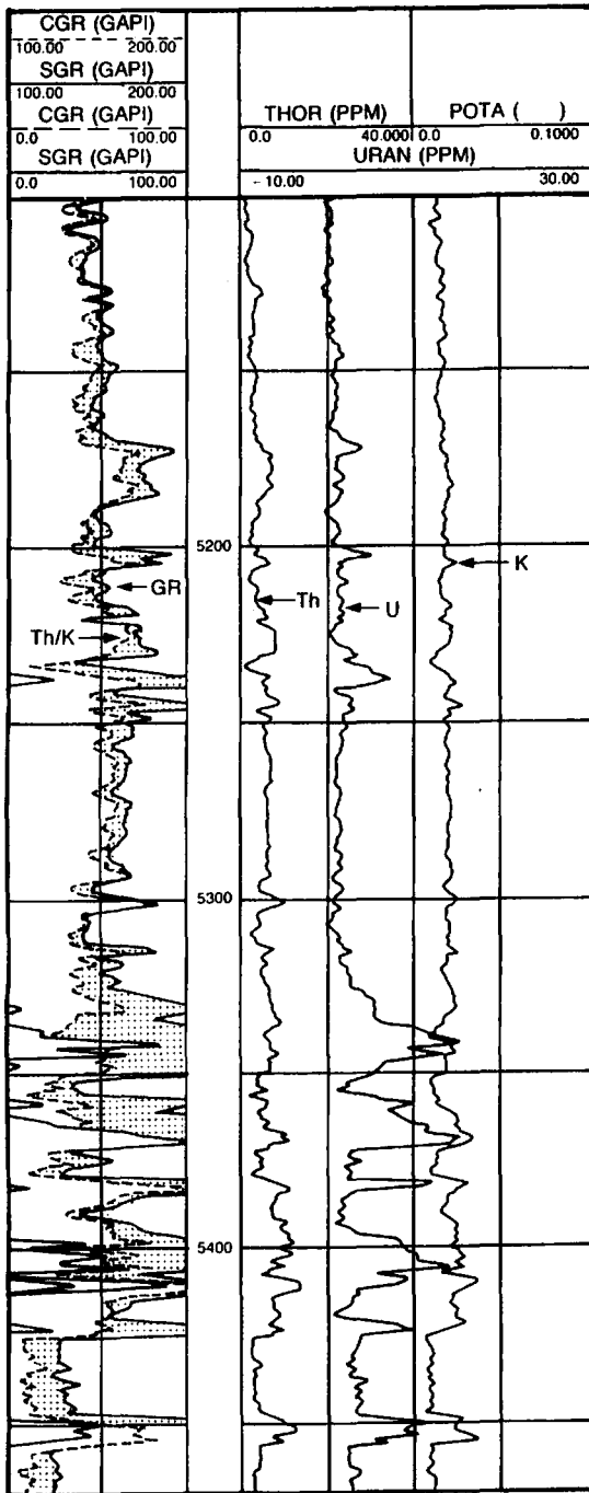
Figure 11.34. A natural \gamma -ray spectrometry log. (From Schlumberger, 1987.)
