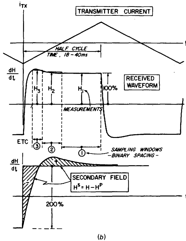
Figure 7.23. UTEM time-domain system. (After West, Macnae, and Lamontagne, 1984.) (a) Block diagram. (b) Transmitter and receiver waveforms.
