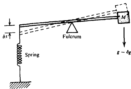
Figure 2.10. Basic principle of the stable gravimeter.
