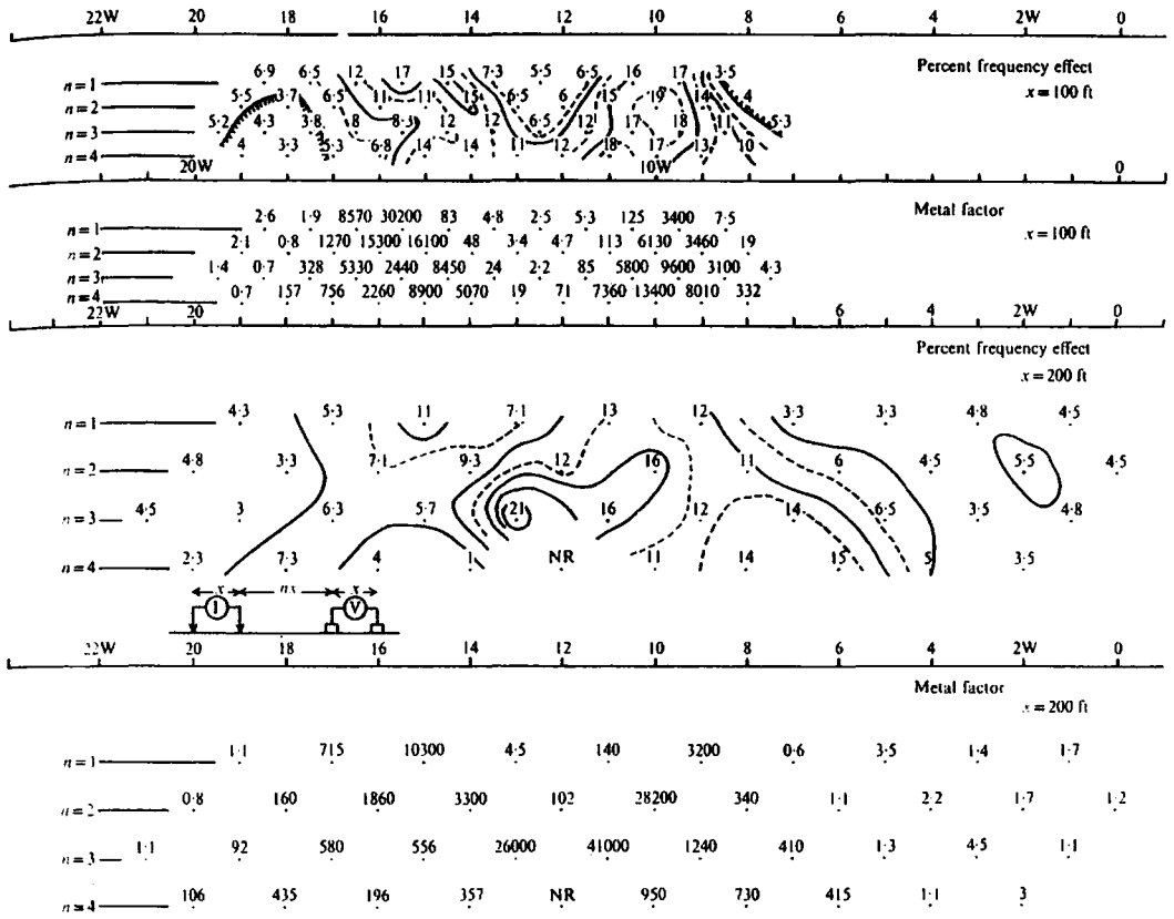
Figure 9.24. Pseudodepth plots for frequency-domain IP, western Ontario.
