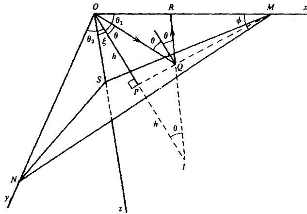
Figure 4.26. Three-dimensional view of a reflection path for a dipping bed.
