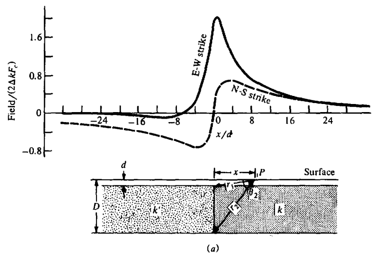
Figure 3.24. F profiles for a semiinfinite horizontal slab striking N-S, I = 45^\circ , dip of slab terminus 45 and 135^\circ , D = 3d .
