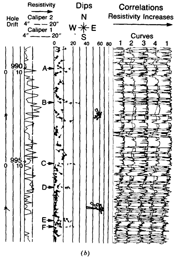
Figure 11.16. The dipmeter. (a) Schematic of diplog tool. (Courtesy Dresser Industries.) (b) Portion of a four-arm processed dipmeter log showing deviation of the hole, caliper log, smoothed resistivity, tadpole plot of dips, rosettes (each showing directions of all dips within a 10 ft. interval), and output of the four microresistivity pads with computer-drawn correlations. (Courtesy Schlumberger Ltd.)
