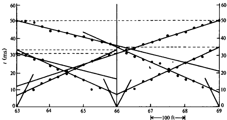
Figure 4.122. Engineering refraction profile.
