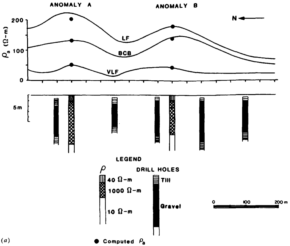
Figure 7.78. Results of an E-phase survey for gravel near Wadena, Saskatchewan. (From Palacky and Jagodits, 1975.) (a) Profile along line 47 [see map in (b)] for three frequencies plus interpretation of anomalies A and B based on \rho_a values and results of DDH logs. BCB = Broadcast band.
