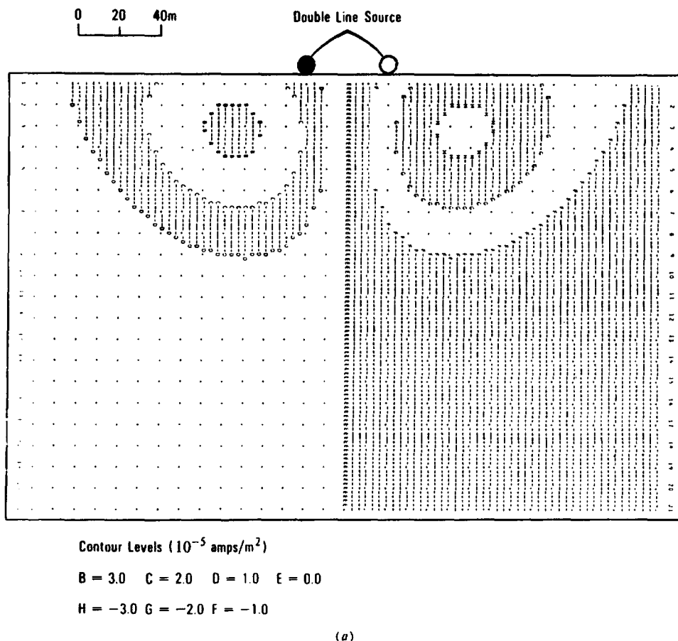
Figure 7.11. Plots of subsurface current density. Current flow 1 A, into page at ●, out at ○. Current shut-off time t = 0 . Contour intervals 10^{-5} A/m 2 in (a) and (b), 10^{-6} A/m 2 in (c). (After Oristaglio, 1982). (a) Plot for t/\sigma\mu = 10^3 m 2 .
