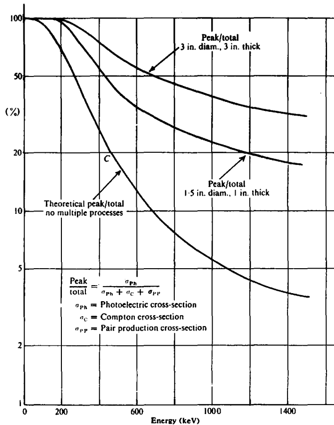
Figure 10.6. \gamma -ray absorption efficiency in NaI crystals.
