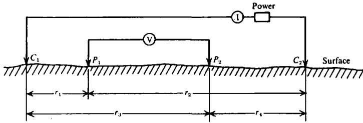
Figure 8.3. Two current and two potential electrodes on the surface of homogeneous isotropic ground of resistivity ρ.
