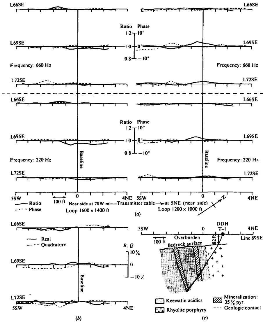
Figure 12.5. Geophysical results and geologic section, Barraute, northwestern Quebec. (a) Turam profiles; frequencies 660 Hz (upper three profiles) and 220 Hz (lower three profiles). (b) HLEM profiles; frequency 1,000 Hz, T-R spacing 300 ft. (c) Assumed geologic section.
