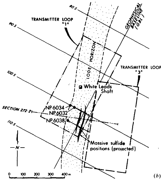
Figure 7.102. (Continued) (b) Plan showing lode horizon, geophysical grid, and drill hole locations.
