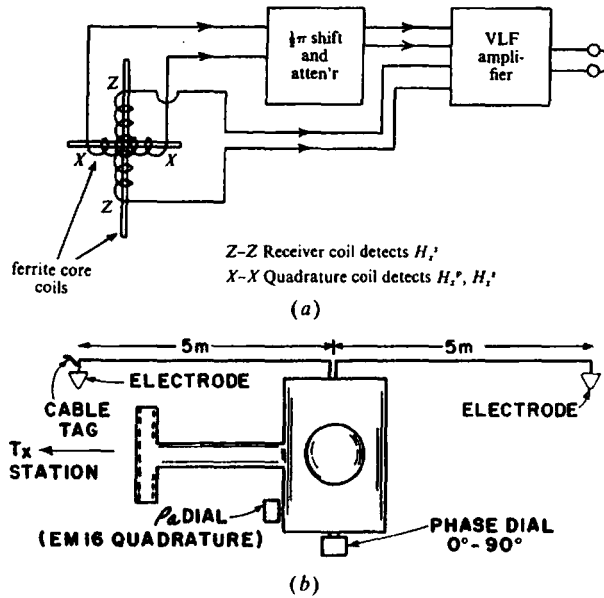
Figure 7.18. VLF receivers. (a) Schematic. (b) Schematic of the EM16R unit.
