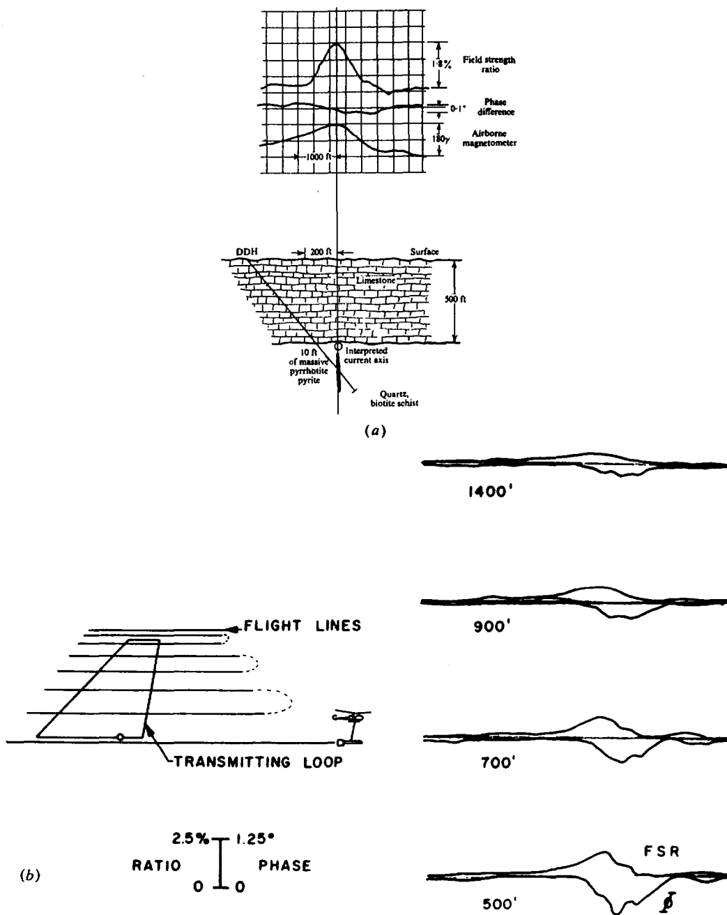
Figure 7.77. Examples of Turair responses. (a) Response over massive sulfide. (b) Effect of altitude over unknown conductor. FSR = Field strength ratio, \Phi = Phase.
