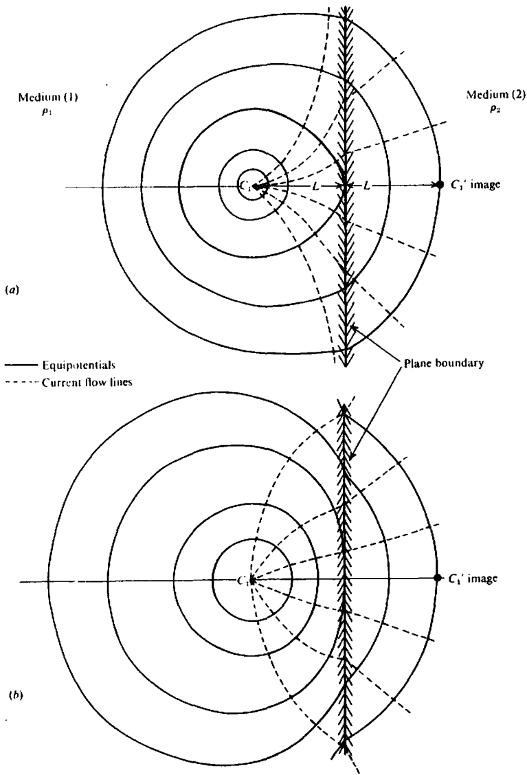
Figure 8.10. Distortion of equipotentials and current flow lines at a boundary between two media of different resistivities. (a) \rho_2/\rho_1 = 3 , k = 0.5 . (b) \rho_2/\rho_1 = 1/3 , k = -0.5 .
