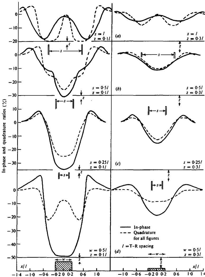
Figure 7.41. Horizontal-loop EM profiles over various conductors of great depth extent. (a) Two thin sheets with spacing equal to the T-R spacing. (b) Two thin sheets with spacing equal to one-half the T-R spacing. (c) Two thin sheets with spacing equal to one-quarter the T-R spacing. (d) Conducting dike with width equal to half the T-R spacing.
