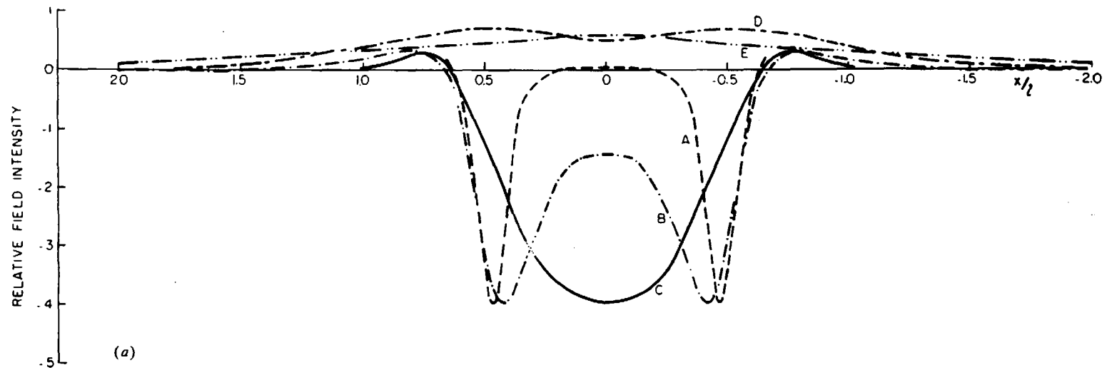
Figure 7.68. Response to a buried sphere. (a) HLEM profiles: l = T-R , depth to center of sphere is l/8 , l/4 , l/2 , l , and 2l for curves A to E, respectively. (After Bhattacharya and Sinha, 1965.)
