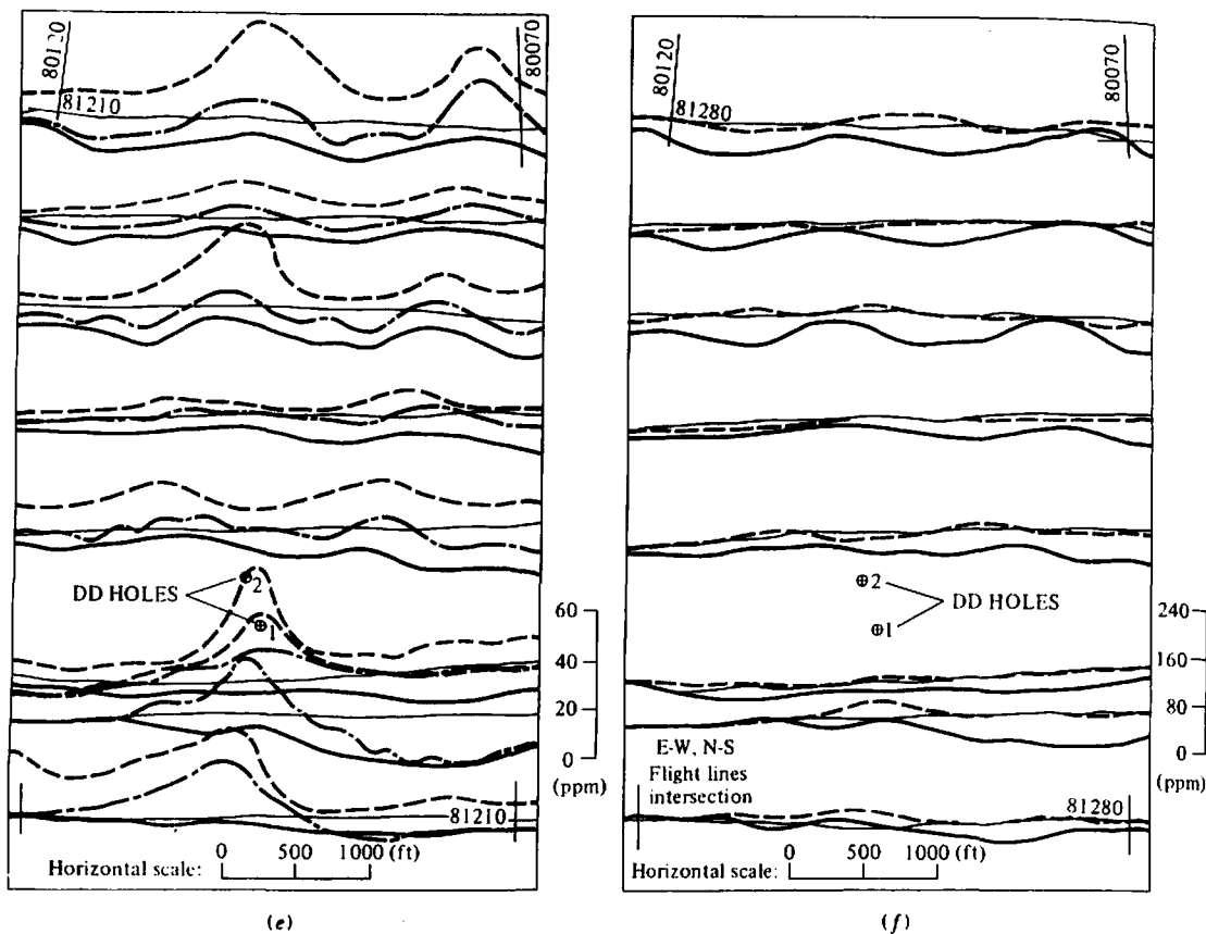
Figure 12.11. (Continued) (e) 935 Hz coaxial pair in-phase (—); 34 kHz coplanar pair in-phase (---) and quadrature (-·-) on line 81210. (f) 4,600 Hz coaxial pair (—); 4,175 Hz coplanar pair (---) (both in-phase) on line 81280.
