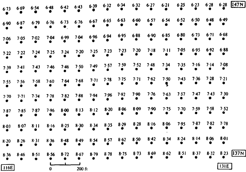
Figure 2.41. Bouguer gravity values on 30 m grid; values in milligals.
