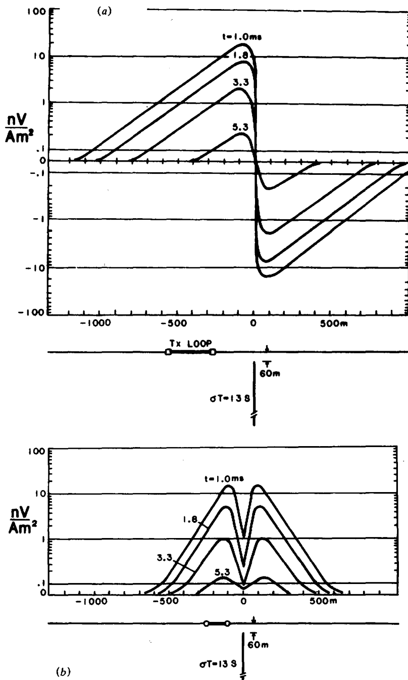
Figure 7.55. Large-loop Tx and coincident-loop responses over a vertical sheet. (After Spies and Parker, 1984.) (a) Large-loop Tx \sim 300 m from target. (b) Coincident-loop crossing sheet.
