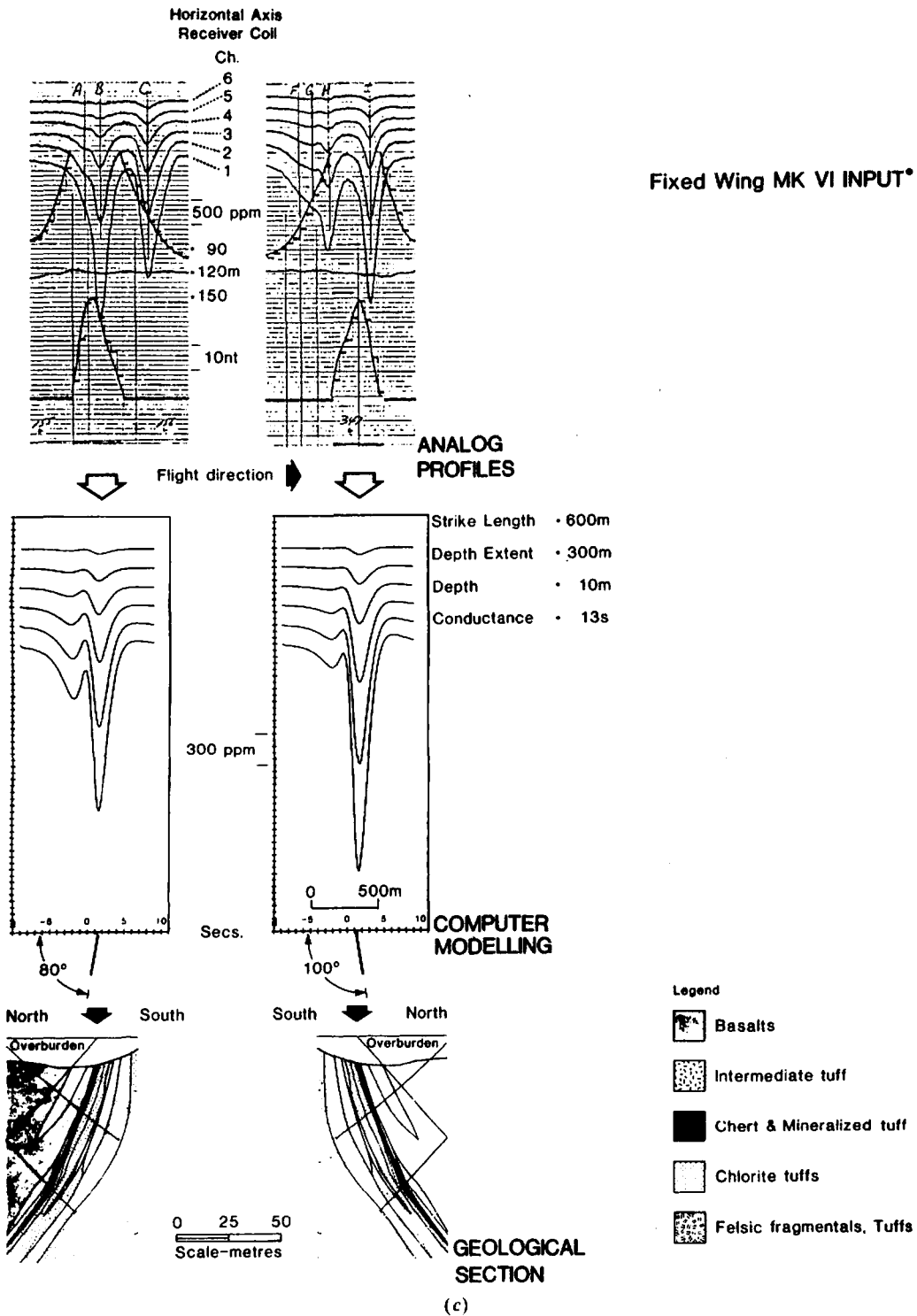
Figure 7.108. (Continued) (c) Detour Lake gold deposit.
