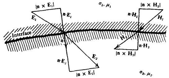
Figure 6.14. Boundary conditions on EM fields at an interface.
