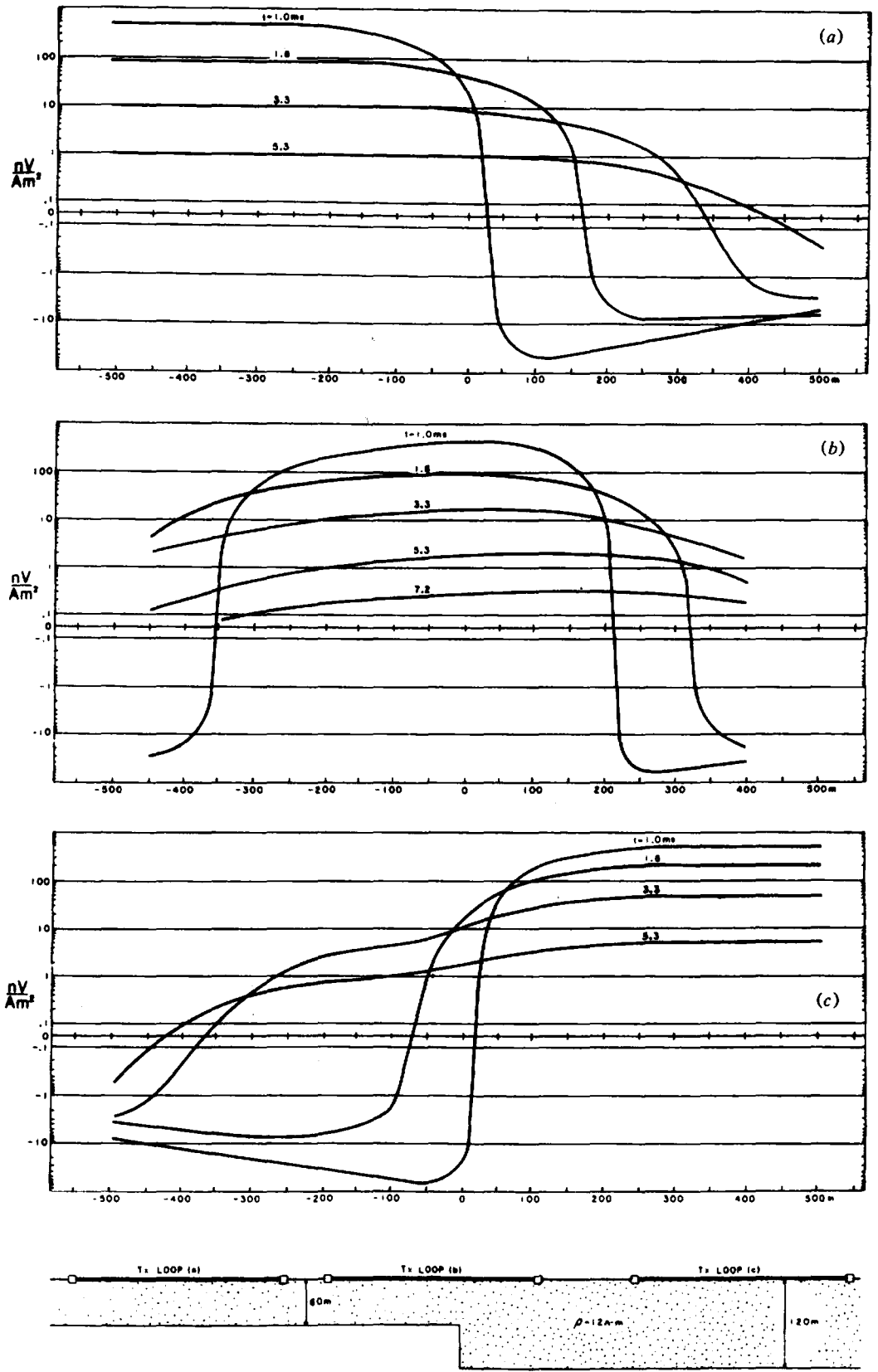
Figure 7.57. Turam and coincident-loop responses to a step in conductive overburden. (After Spies and Parker, 1984.) (a) Turam Tx over 60 m section. (b) Tx centered over step. (c) Tx over 120 m section.
