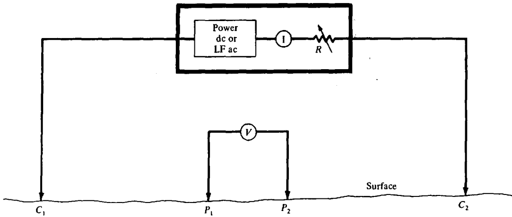
Figure 8.16. Schematic of equipment for measuring resistivity.
