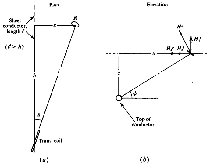
Figure 7.29. Dip-angle fixed transmitter over steeply dipping sheet. (a) Plan view. (b) Elevation showing receiver signals.
