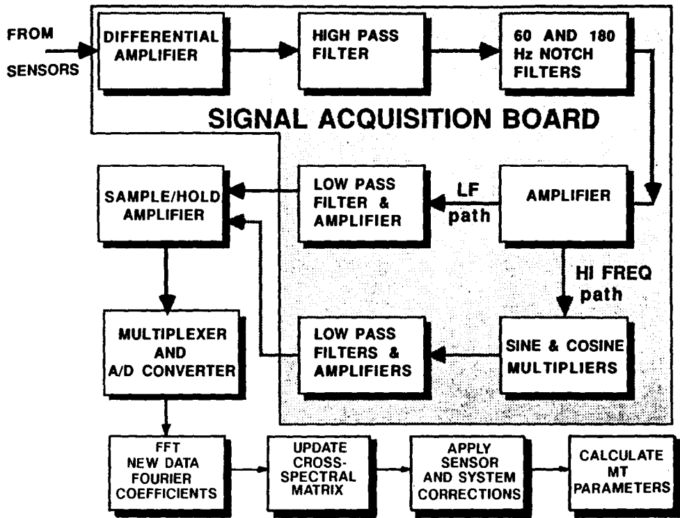
Figure 6.21. Block diagram of a wide-band MT system with computerized data processing. (After Nichols, 1987.)
