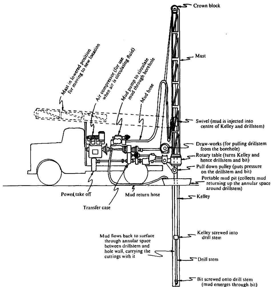
Figure 4.51. Rotary drill. (From Sheriff, 1984.)
