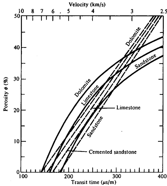
Figure 11.24. Porosity versus interval transit time. The curved lines are empirical, the straight lines give values from the time-average equation. (After Schlumberger, 1986.)
