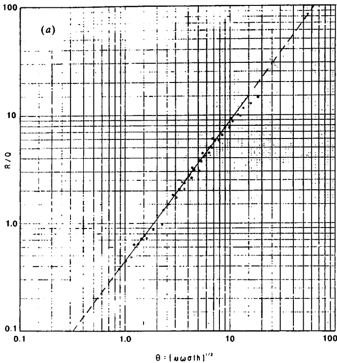
Figure 7.81. Response of a maximum-coupled coil to a thin vertical dike. (After Fraser, 1972.) (a) Ratio of in-phase ( R ) to quadrature ( Q ) components as a function of the induction number \theta = (\mu_0 \omega \sigma h)^{1/2} .
