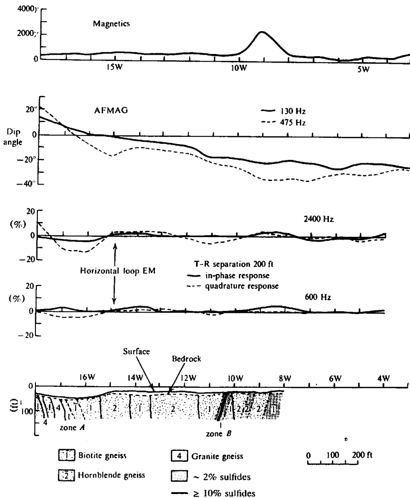
Figure 12.10. Geophysical results and geologic section, line D, Cavendish Township, Ontario.
