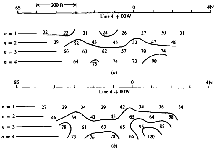
Figure 8.48. Apparent resistivities ( \rho_a/2\pi \Omega ft ) from two IP surveys using a double-dipole array with separation 100 ft. (a) Data from frequency-domain IP. (b) Data from time-domain IP.
