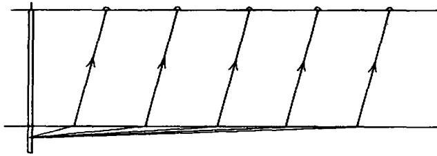
Figure 4.76. Refraction weathering profile.
