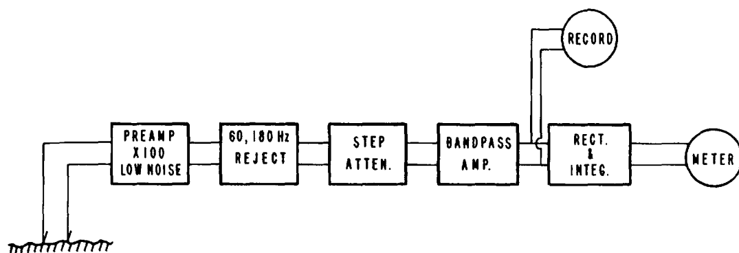
Figure 6.15. Schematic of telluric unit for audio and subaudio frequencies.
