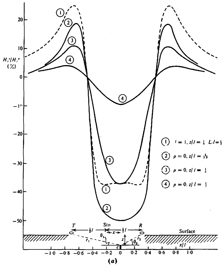
Figure 7.36. Effect of various parameters on horizontal-loop profiles over dipping sheets. (a) Effect of depth of a semiinfinite vertical sheet.
