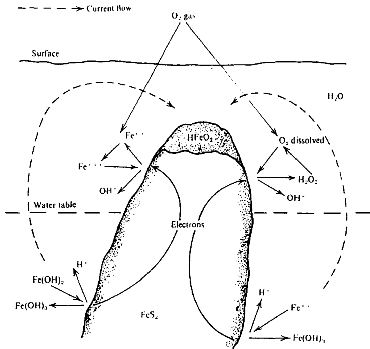
Figure 6.2. Self-potential mechanism in pyrite. (From Sato and Mooney, 1960.)
