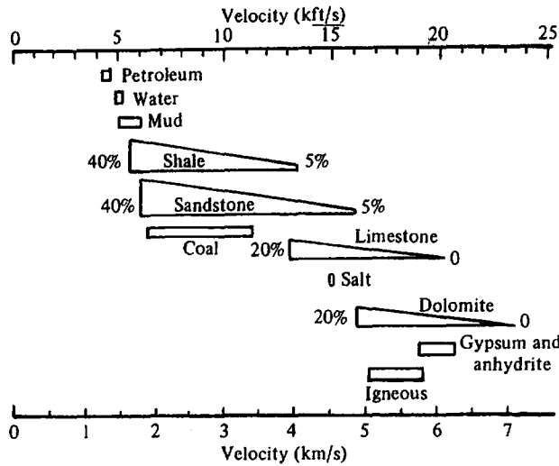
Figure 4.18. Measurement of velocity in different rock types reported by Birch (1966). (From Sheriff and Geldart, 1983.)
