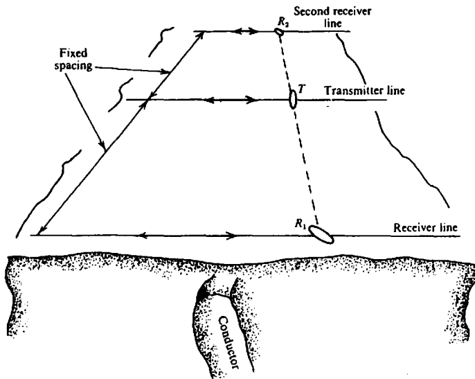
Figure 7.15. Dip-angle system, broadside orientation.
