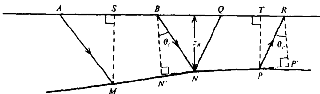
Figure 4.88. Determining sourcepoint and geophone delay times.
