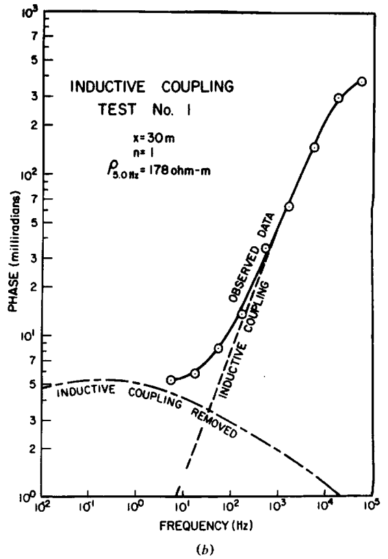
Figure 9.10. Phase-angle spectra and their use in removing EM coupling effects. Double-dipole array: n = 1 , x = 30 m. (After Pelton et al., 1978.) (a) Typical porphyry spectrum and EM coupling spectrum over homogeneous earth. (b) Observed data and curve (solid line) obtained using two Cole-Cole dispersion terms; dashed line is EM coupling spectrum calculated using the Cole-Cole parameters; the dash-dot line is the difference between the two previous curves.
