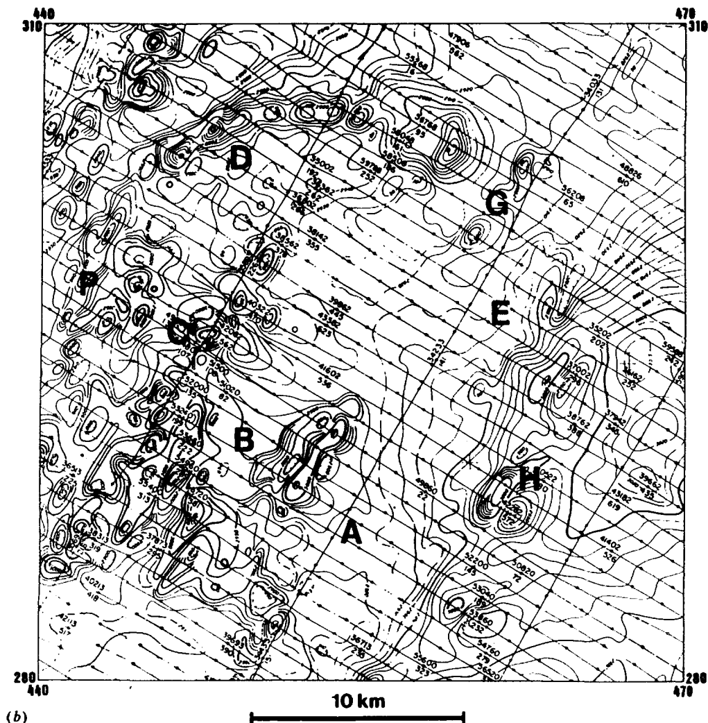
Figure 10.20. (Continued) (b) Total-field magnetic map; contour interval five gammas.
