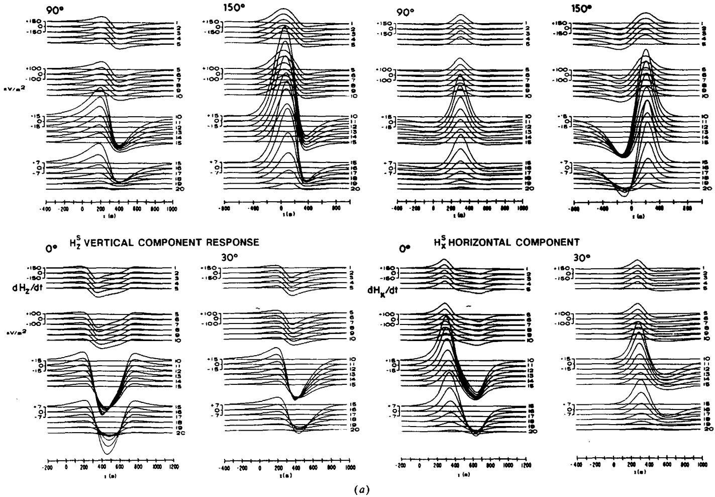
Figure 7.53. EM37 response over a plate model; curves show \partial H_z/\partial t and \partial H_x/\partial t . \ell \times d = 800 \times 400 m [except in (d) and (e)], TCP = 30 S [except in (c)]. (After Gallagher, Ward, and Hohmann, 1985.) (a) Effect of dip; z = 100 m; left-hand half shows curves for H_z , right-hand half for H_x .
