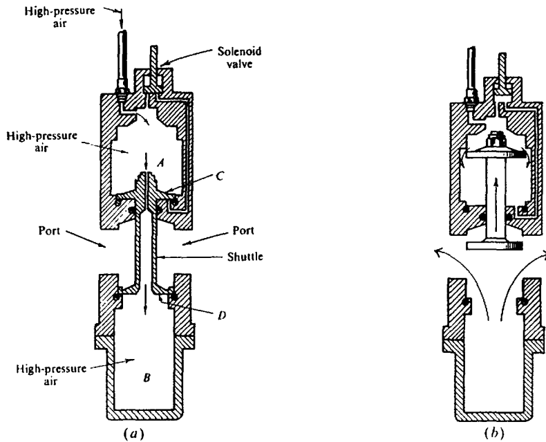
Figure 4.61. Air gun. (Courtesy Bolt Associates.) (a) Ready for firing. (b) Firing.
