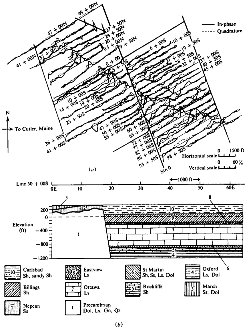
Figure 7.97. VLF survey across the Gloucester Fault, eastern Ontario. (a) Plot of the field data. (b) Geological section, line 50 + 00S.
