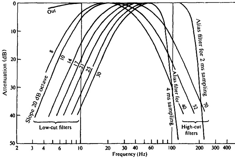
Figure 4.56. Response of seismic filters.
