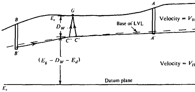
Figure 4.75. Datum correction for geophone between shotpoints.
