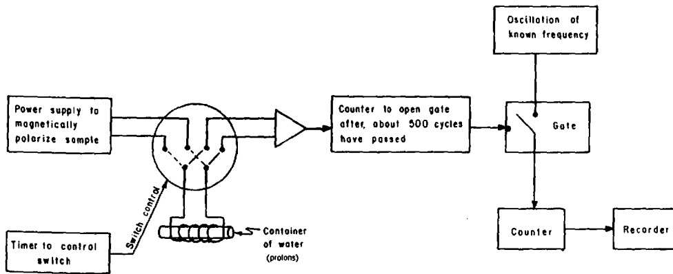
Figure 3.10. Proton-precession magnetometer. (From Sheriff, 1984.)
