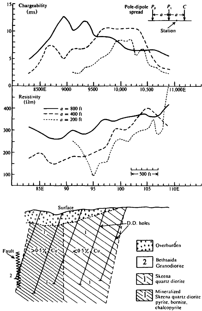
Figure 9.19. Time-domain IP results over porphyry-copper deposit. (After Seigel, 1967.)
