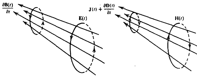
Figure 6.13. Electric and magnetic fields of Equations (6.3) and (6.4). (After Grant and West, 1965.)
