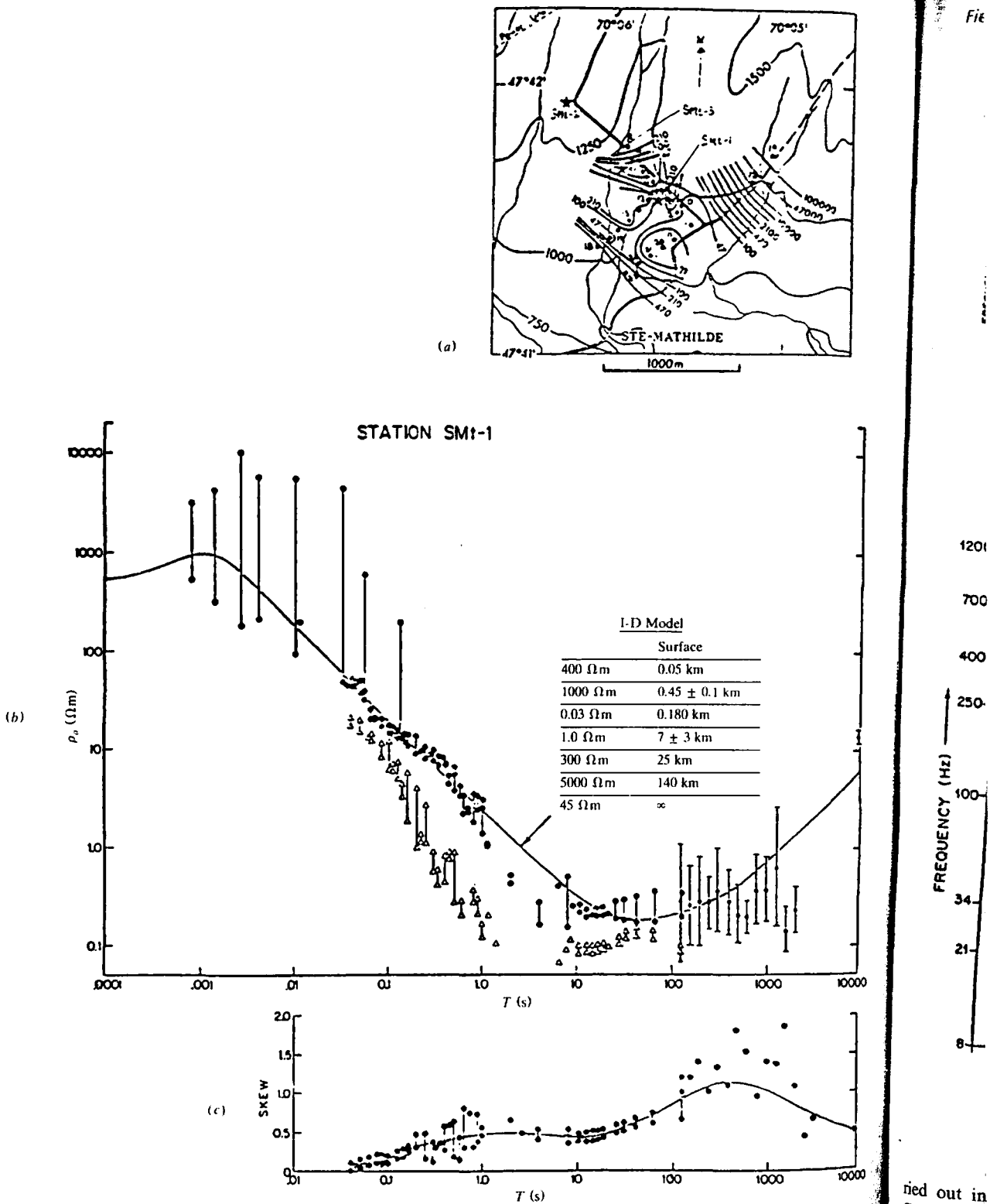
Figure 6.30. \rho_p results near Ste. Mathilde, Quebec. (a) Map showing elevations, locations of profiles 1-3 plus \rho_p contours. (b) Results for station SMt-1: \rho_p curve, tensor data in the principal axis of anisotropy from 0.03 to 10,000 s, and scalar data from 0.0008 to 0.13 s; dots and triangles are \rho_p values for the major and minor axes of anisotropy, respectively; error bars show maximum scatter from 0.0008 to 100 s, two standard deviations from 100 to 10,000 s; solid curve is for the 1-D model. (c) Skew ratios.
