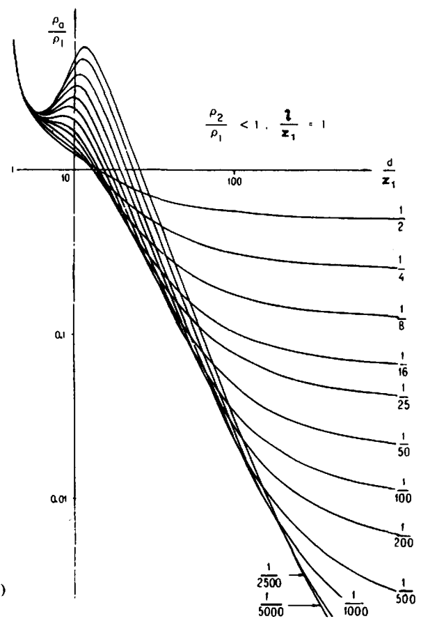
Figure 7.76. Master curves of late-time (\rho_0/\rho_1) versus (d/z_1) . [Parts (a) and (b): After McNeill, 1980; parts (c) to (f): After Kaufmann and Keller, 1983.] (a) Two-layer curves for resistive basement. (b) Same as (a) except for conductive basement.
