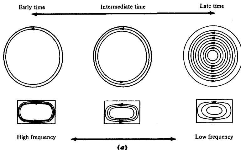
Figure 7.69. Time-domain eddy-current distribution in a spherical conductor. (a) Schematic comparing eddy-current diffusion in a sphere and a plate (After McNeill, 1980.)
