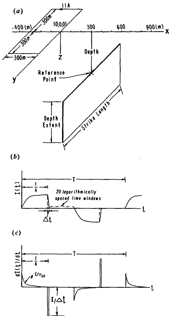
Figure 7.22. EM37 TDEM system. (After Gallagher, Ward, and Hohmann, 1985.) (a) Field layout. (b) Transmitter-current waveform. (c) Time derivative of current waveform.
