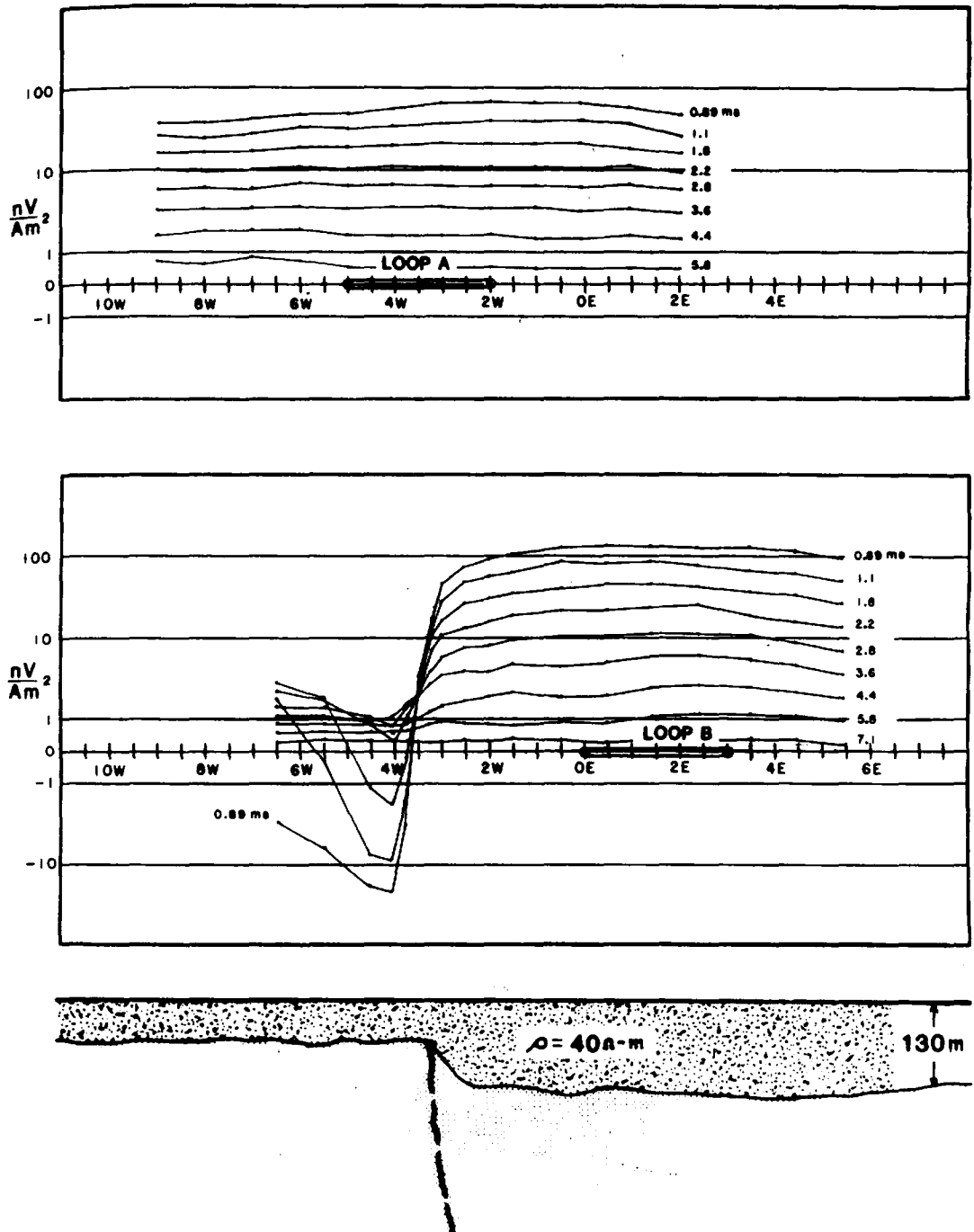
Figure 7.58. Field traverses obtained with a fixed-loop system for two different transmitter-loop positions. The strong anomaly recorded with loop B disappeared when loop A was used. (After Spies and Parker, 1984.)
