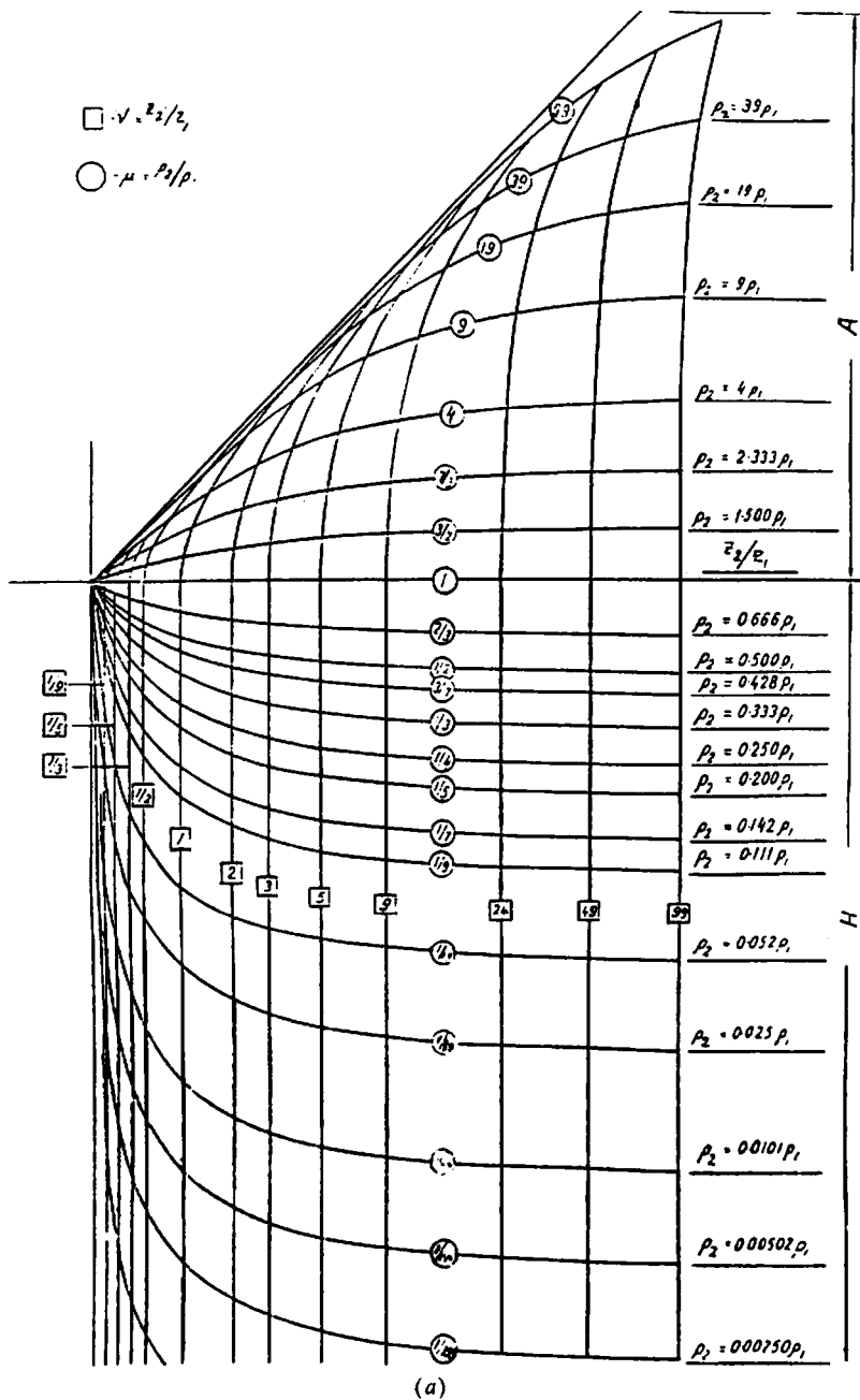
Figure 8.28. Auxiliary-point charts (a) for H- and A-type sounding curves.
