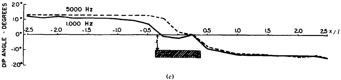
Figure 7.31. Effect of transmitter location and frequency on dip-angle fixed-transmitter results. l = T-R . (After Ward, 1967.) (a) Sheet of depth extent d dipping 45^\circ . (b) Horizontal sheets of width d , various Tx locations; z/l = 0.1 , d/l = 1.2 . (c) Responses at 1,000 and 5,000 Hz to a conducting slab of finite width (graphite in the model).
