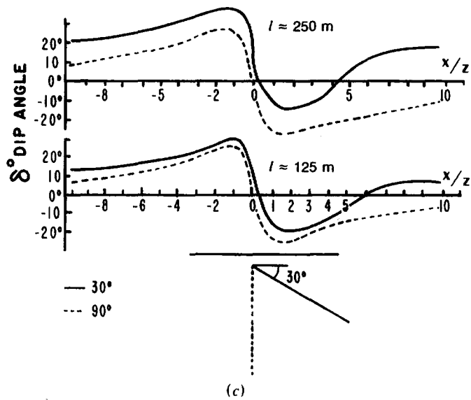
Figure 7.30. Response of dip-angle fixed-transmitter system to dipping sheets. l = T-R . (After Ward, 1967.) (a) Sheets of depth extent d dipping 30^\circ and 60^\circ . (b) Effect of variable depth of vertical sheet. (c) Effect of T-R separation.
