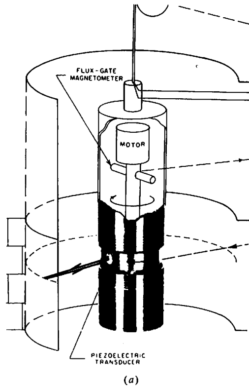
Figure 11.30. The borehole televiewer. (From Zemanek et al., 1970.) (a) Schematic view of the sonde; the magnetometer gives the sonde orientation.
