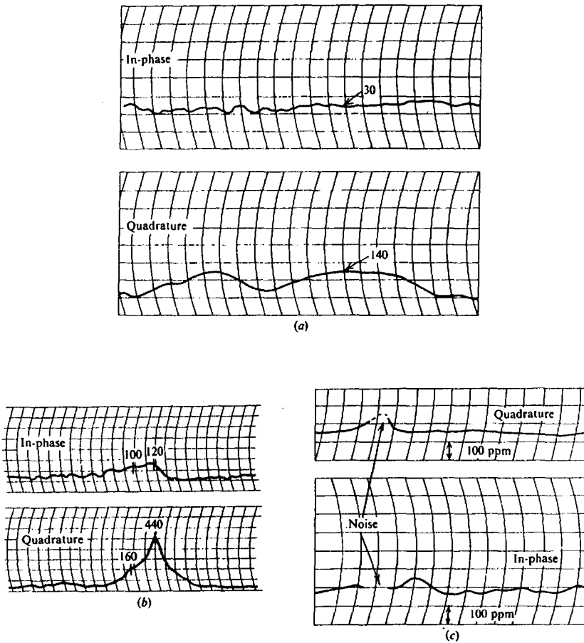
Figure 7.121. Airborne phase-component EM profiles. (a) Helicopter survey, transmitter frequency 400 Hz. (b) As in (a) for 320 Hz. (c) Fixed-wing aircraft, transmitter frequency 390 Hz.
