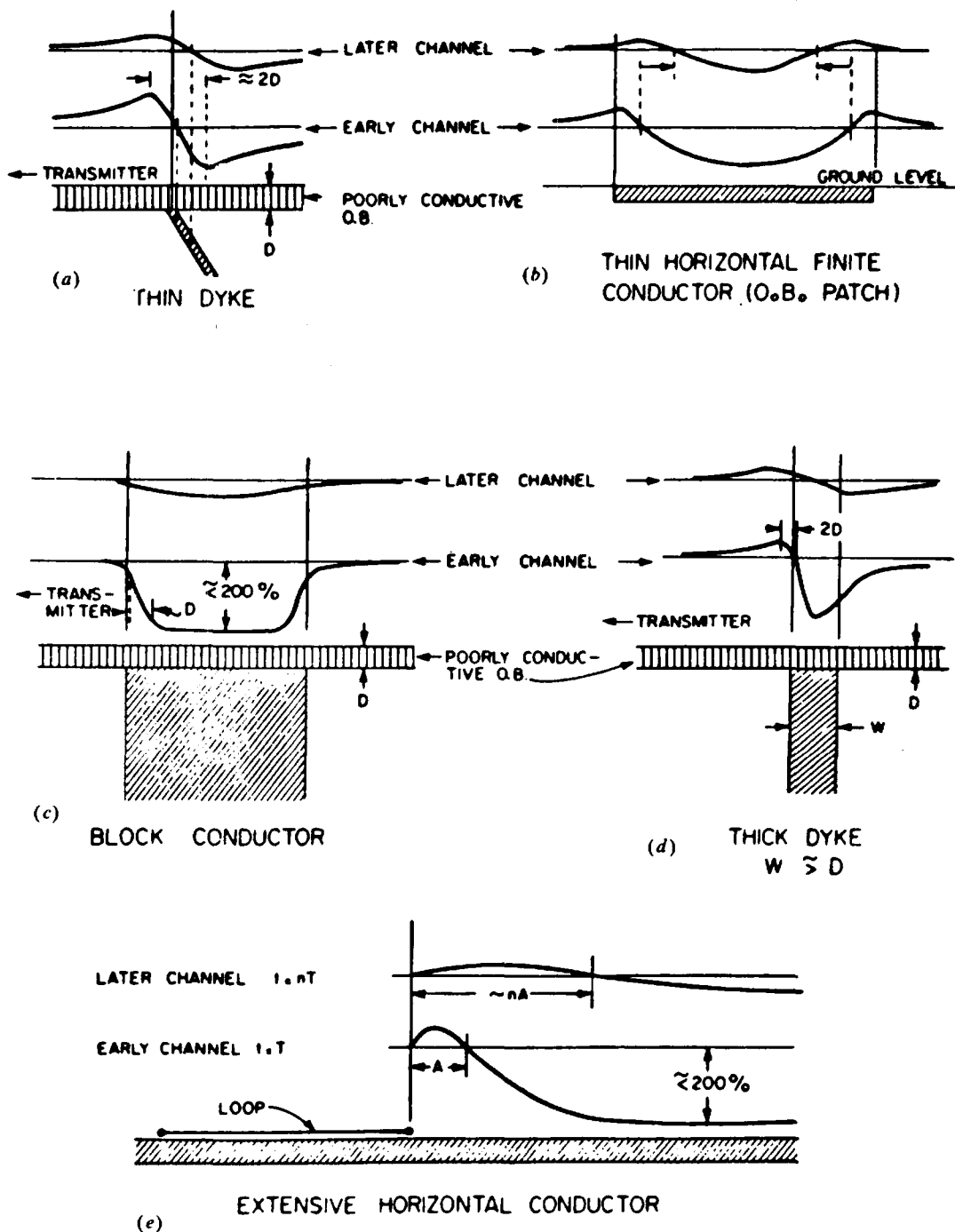
Figure 7.62. The form of continuously normalized UTEM H_z^2 profiles over some simple shapes. All conductors are in free space. (After West, Macnae, and Lamontagne, 1984.)
