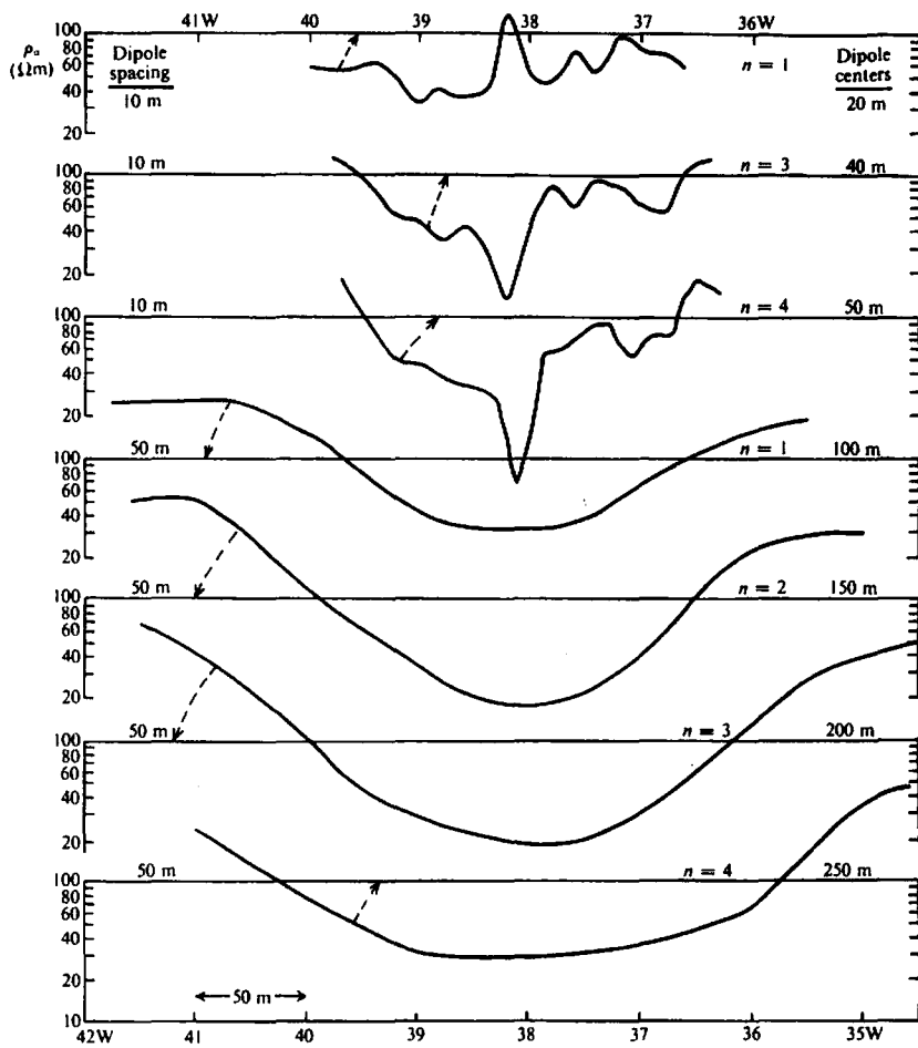
Figure 8.47. Apparent resistivities from IP survey, northeast Brazil.
