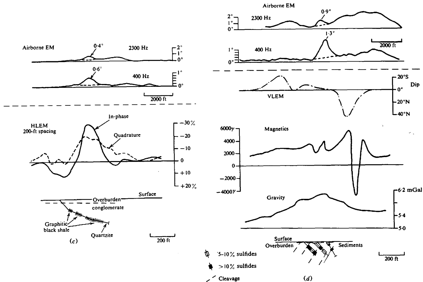
Figure 7.106. (Continued) (c) Comparison with HLEM over shallow graphite deposit. (d) Comparison with several methods over shallow sulfides.
