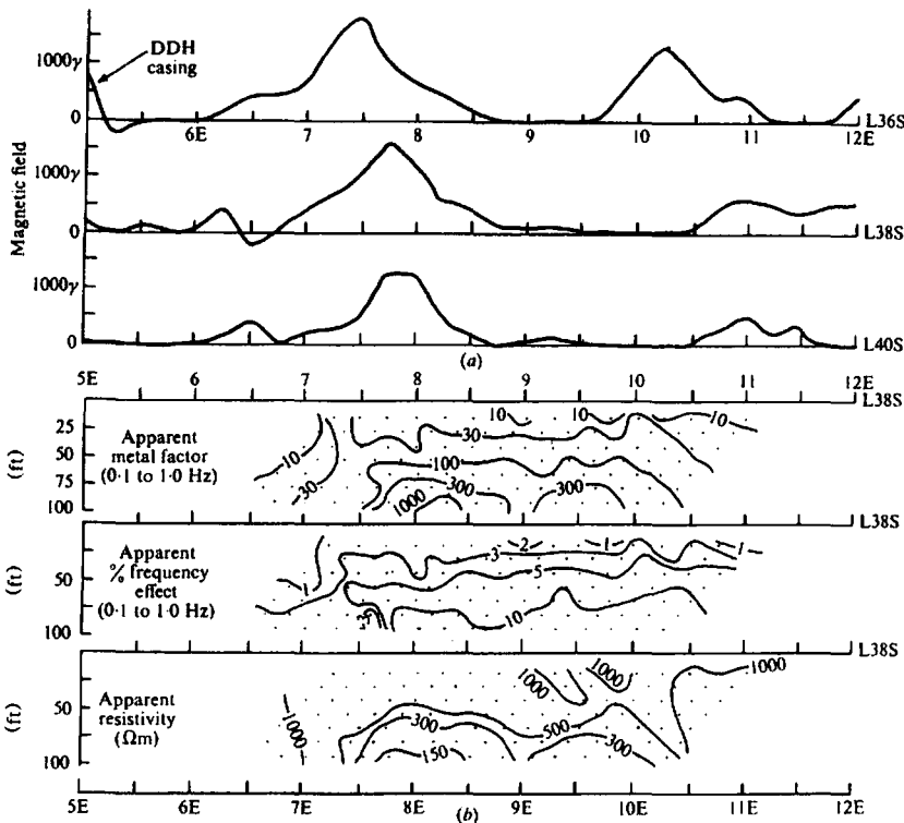
Figure 12.8. Magnetic and electrical results, Woburn, Quebec. (a) Vertical component (magnetic field) profiles. (b) IP and apparent-resistivity pseudodepth plots.
