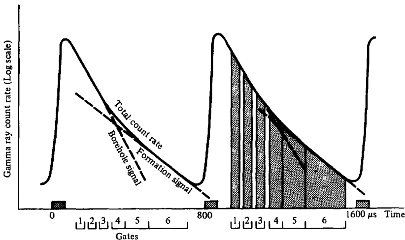
Figure 11.40. Pulsing and gating parameters for pulsed neutron log. A burst of neutrons occurs every 800 \mu s. (From Snyder and Fleming, 1985.)
