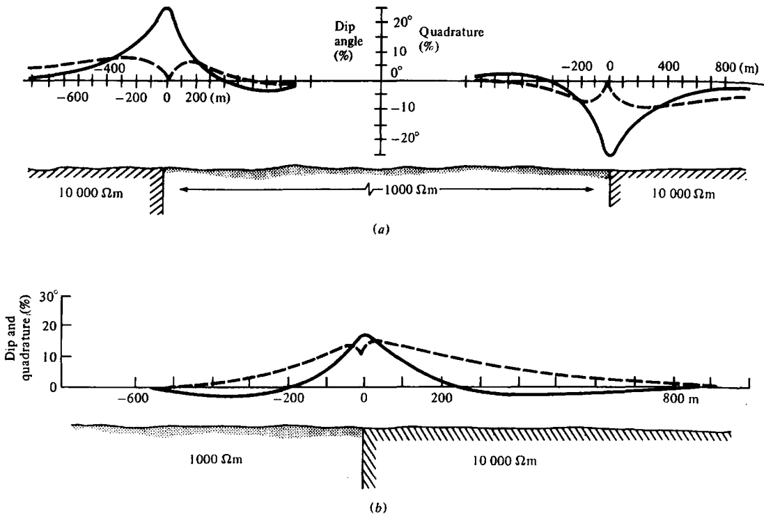
Figure 7.48. VLF profiles over vertical contacts between beds of different conductivities. (a) 1,000 Ωm bed between two half-spaces of 10,000 Ωm; no overburden. (b) Same as (a) except overlain by 6 m of conductive overburden, \rho = 100 \Omega m .
