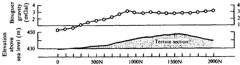
Figure 2.42. Bouguer gravity and topographic profiles, East Africa.
