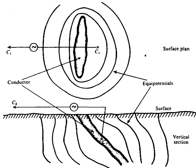
Figure 8.19. Distortion of the equipotentials around the near current electrode by a dipping conductor when using the mise-à-la-masse method.
