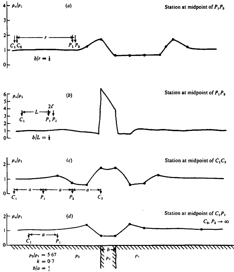
Figure 8.36. Profiles over a thin dike using different electrode spreads. (a) Double-dipole spread. (b) Half-Schlumberger spread. (c) Full-Wenner spread. (d) Half-Wenner spread.
