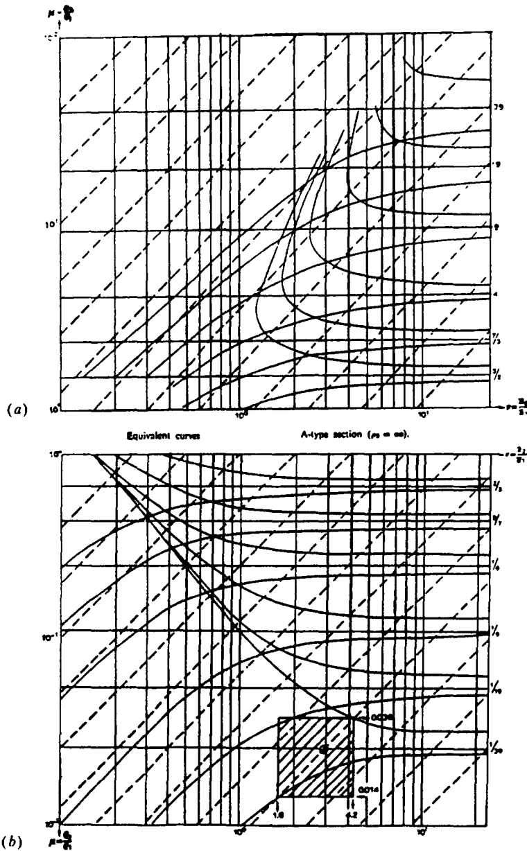
Figure 8.32. Equivalent curves. Solid-line curves are limiting values of \mu = \rho_2/\rho_1 and \nu = z_2/z_1 for equivalence; dashed lines are lines of equal S_2/S_1 in (a) and (b), equal T_2/T_1 in (c) and (d). (a) A-type section, \rho_3 = \infty . (b) H-type section, \rho_3 = \rho_1 .
