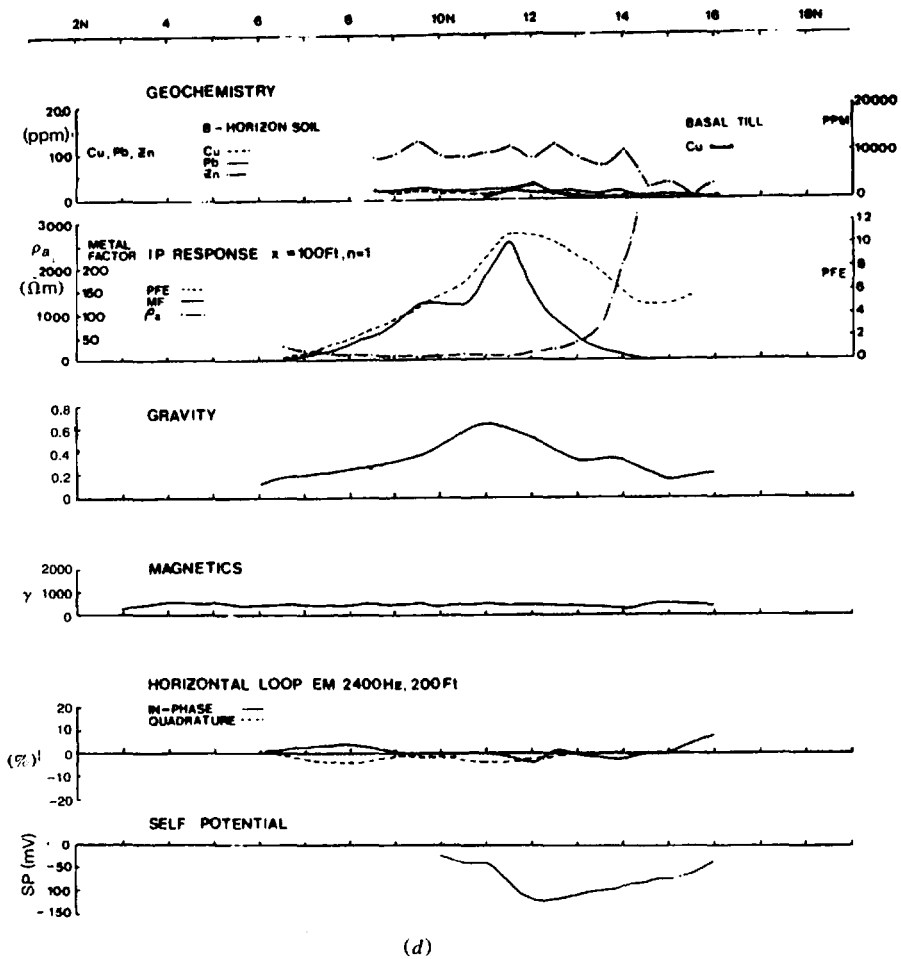
Figure 12.13. (Continued) (d) same as (b) for line 4 + 00E
