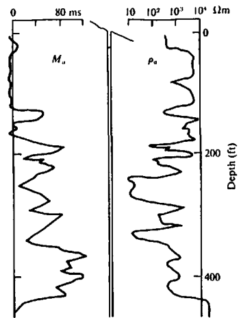
Figure 11.51. IP log in northwest Quebec.
