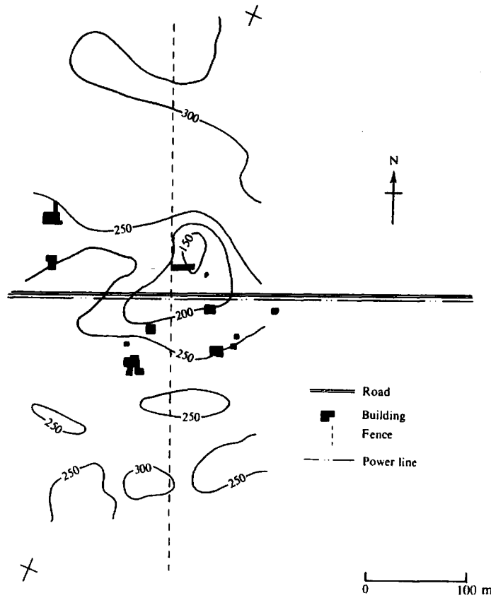
Figure 3.34. Vertical magnetic ground survey, Noranda area; C.I. = 50 nT. (After Seigel, 1957.)
