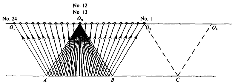
Figure 4.45. Symmetrical spread with continuous subsurface coverage.
