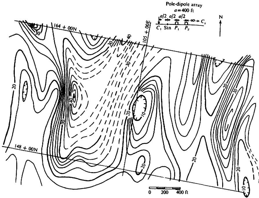
Figure 9.22. Time-domain IP survey, southern New Brunswick. Contour interval: 2 ms.
