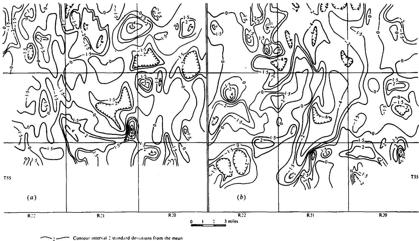
Figure 10.17. Aeroradiometric survey, Redwater Oilfield, Alberta. (a) Area flown east-west, winter of 1957; contours are total-count for energies above 1.5 MeV. (b) Area flown east-west, autumn of 1951; contours are for total count only.
