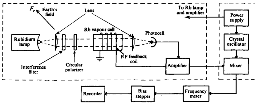
Figure 3.12. Rubidium-vapor magnetometer (schematic).
