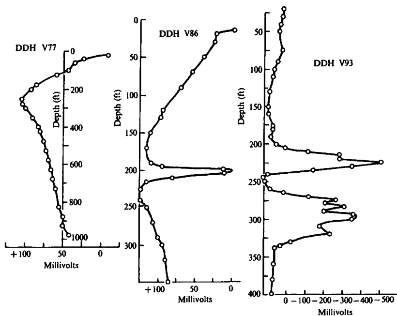
Figure 11.53. SP-logs in base-metal zones.
