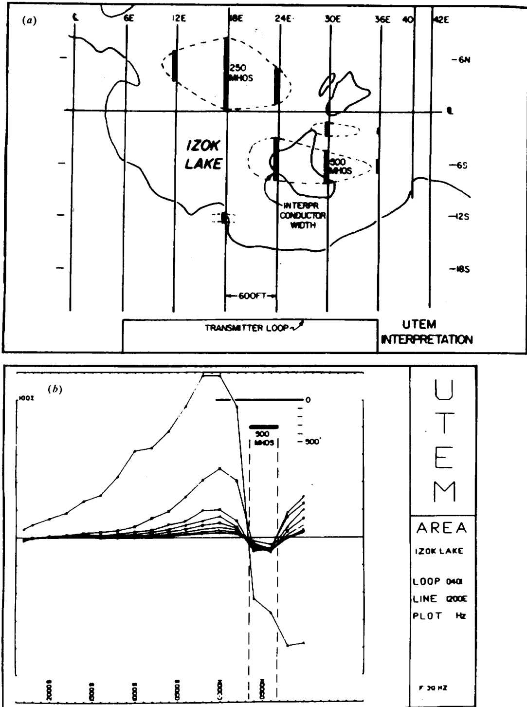
Figure 7.105. UTEM test over Izok Lake deposit, North West Territories, Canada. (After Podolsky and Slankis, 1979.) (a) Map of interpreted mineralization. (b) Profile along line 12E.
