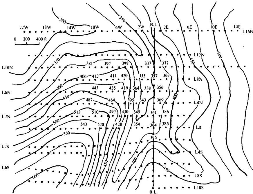
Figure 2.39. Topographic map for terrain correction.
