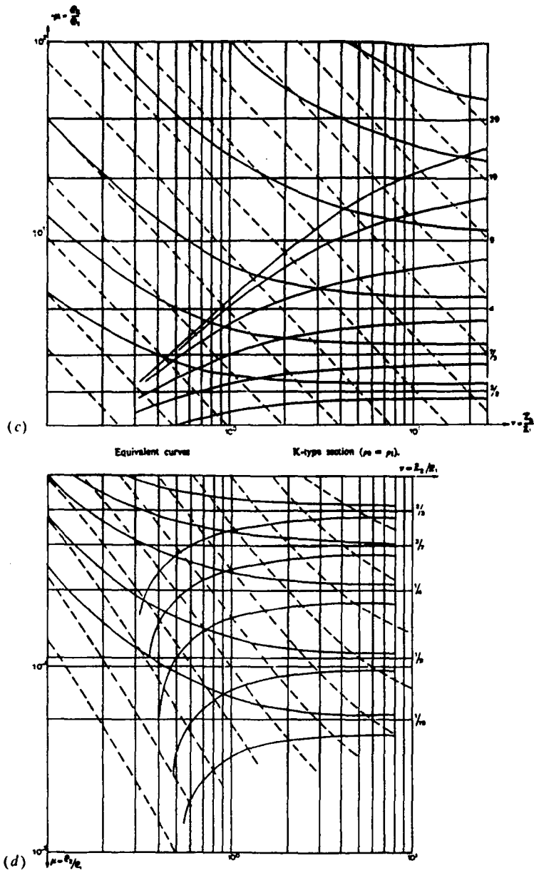
Figure 8.32. (Continued) (c) K-type section, \rho_2 = \rho_1 . (d) Q-type section \rho_2 = 0 .
