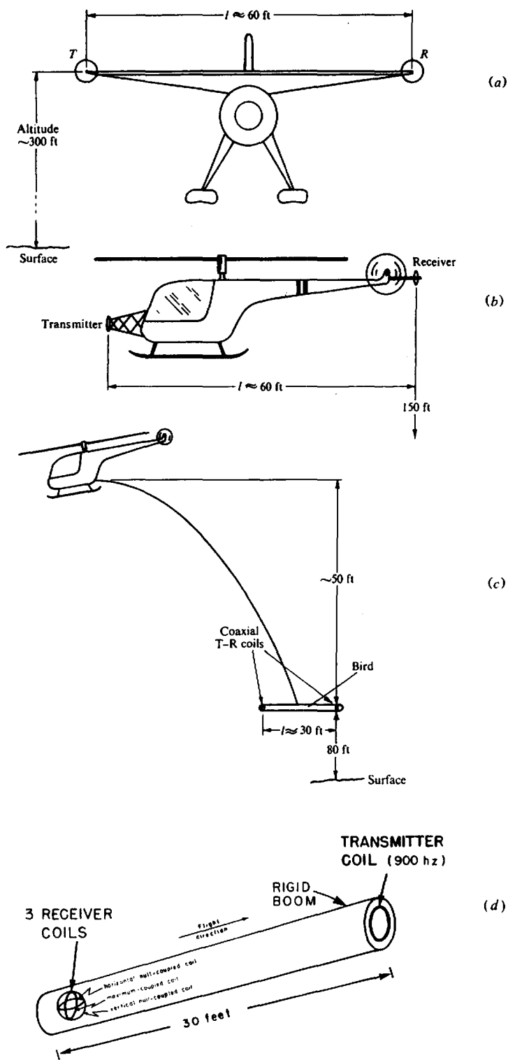
Figure 7.26. Airborne double-dipole EM systems. (a) Fixed-wing, coplanar. (b) Helicopter on-board coaxial mounting. (c) Helicopter boom mounting. (d) Dighem multi-coil bird.
