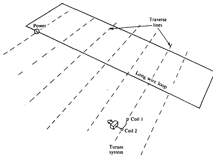
Figure 7.19. Turam field layout.
