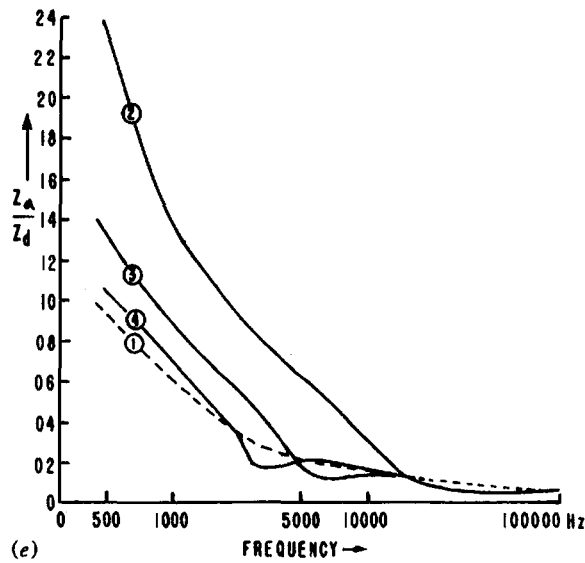
Figure 7.74. (Continued) (e) Ratio of moduli for systems (a) and (d) over one-, two-, three-, and four-layer earths.
