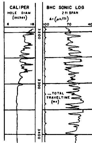
Figure 11.25. Portion of a sonic log. (From Schlumberger, 1987.)
