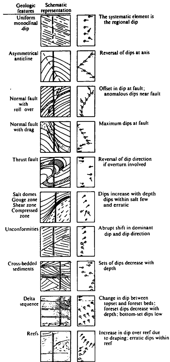
Figure 11.17. Idealized dipmeter patterns indicating structural and stratigraphic features. (After Pirson, 1970.)
