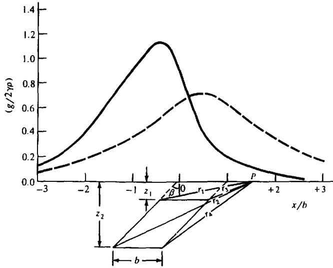
Figure 2.31. Gravity effect of a dike. Profiles are perpendicular to the dike. L = \infty , b = 1 , z_1 = 1/3 , z_2 = 4/3 , \beta = 45^\circ (solid line), 0^\circ (dashed line).
