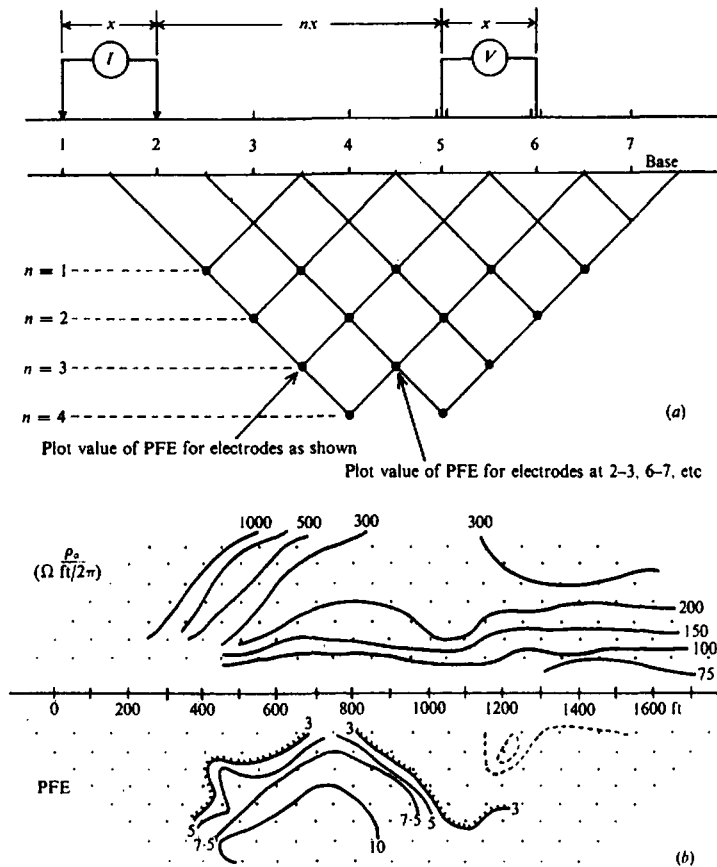
Figure 9.13. Variable-frequency IP pseudodepth plots. (After Marshall and Madden, 1959.) (a) Graphical construction for locating data points. (b) Pseudodepth plot of the data of Figure 9.11b.
