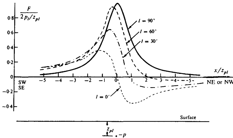
Figure 3.16. Total-field profiles normal to a line of poles striking NW-SE.
