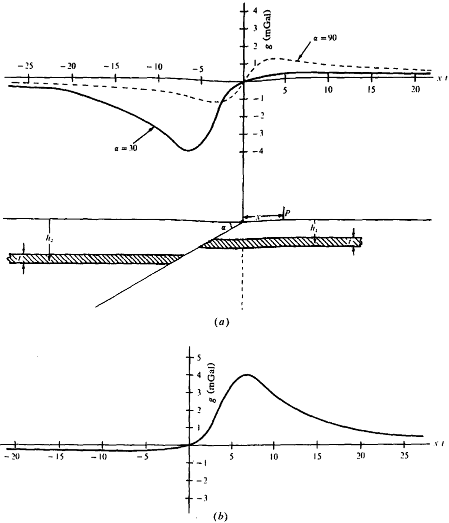
Figure 2.29. Gravity effect of a faulted horizontal sheet; t = 300 m, h_1 = 750 m, h_2 = 1350 m, and \rho = 1 g/cm 3 . (a) Normal fault dipping \alpha = 30 and 90^\circ . (b) Reverse fault, \alpha = -30^\circ .
