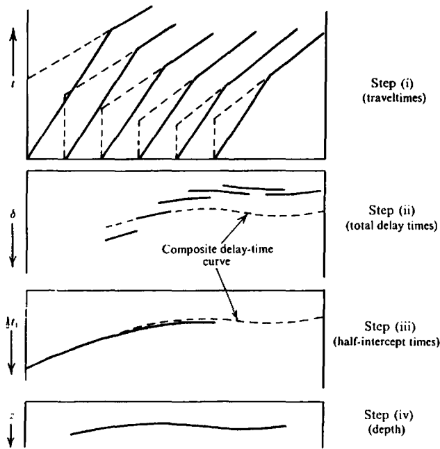
Figure 4.90. Wyrobek's method using unreversed profiles. (After Wyrobek, 1956).
