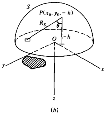
Figure 2.22. The continuation theorem. (After Grant and West, 1965.) (a) Hemisphere S on positive side of xy plane. (b) Hemisphere on negative side of xy plane.
