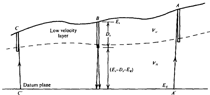
Figure 4.74. Calculation of weathering corrections.
