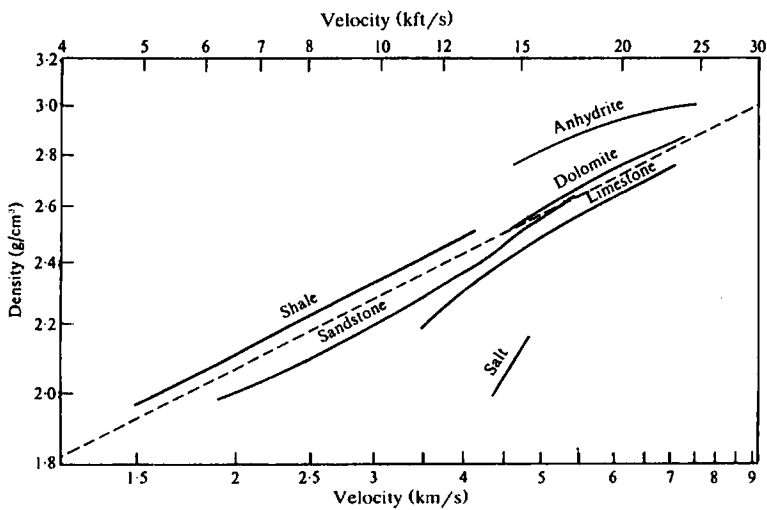
Figure 4.20. P-wave velocity-density relationships for different lithologies (log-log scale). The dotted line represents Gardner's rule: \rho = aV^{1/4} . (From Gardner, Gardner, and Gregory, 1974.)
