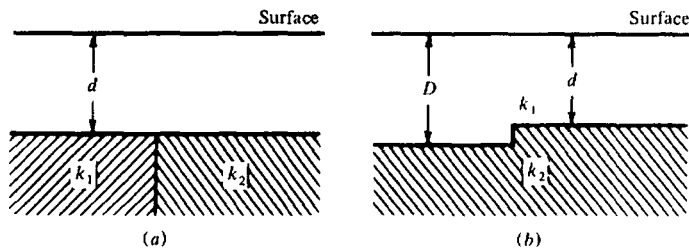
Figure 3.45. Basement structures. (a) Contact between slabs of different susceptibility. (b) Uniform bed with a step.
