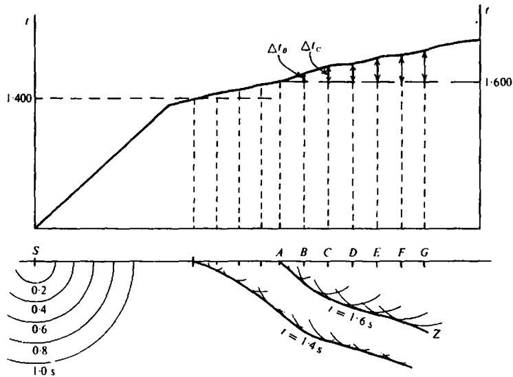
Figure 4.91. Reconstruction of wavefronts.
