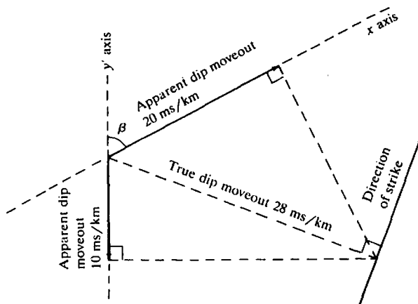
Figure 4.27. Resolution of cross-spread information.
