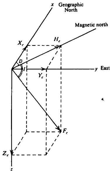
Figure 3.5. Elements of the Earth's magnetic field.
