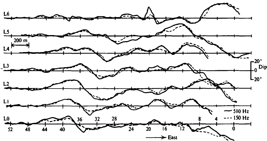
Figure 7.111. AFMAG profiles, northeastern Brazil.
