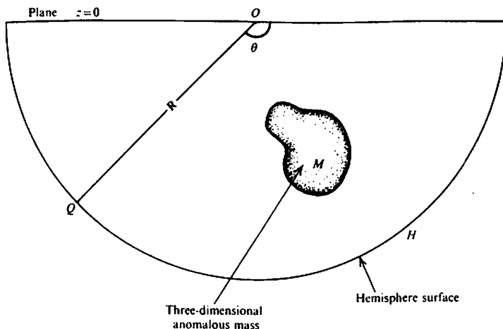
Figure 2.35. Calculation of excess mass.
