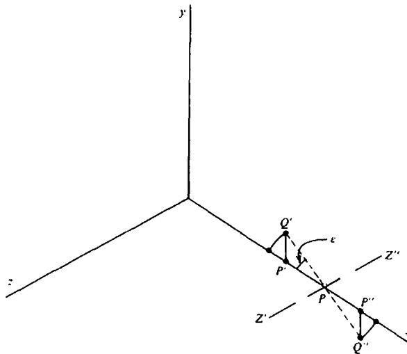
Figure 4.8. Motion during passage of an S wave.
