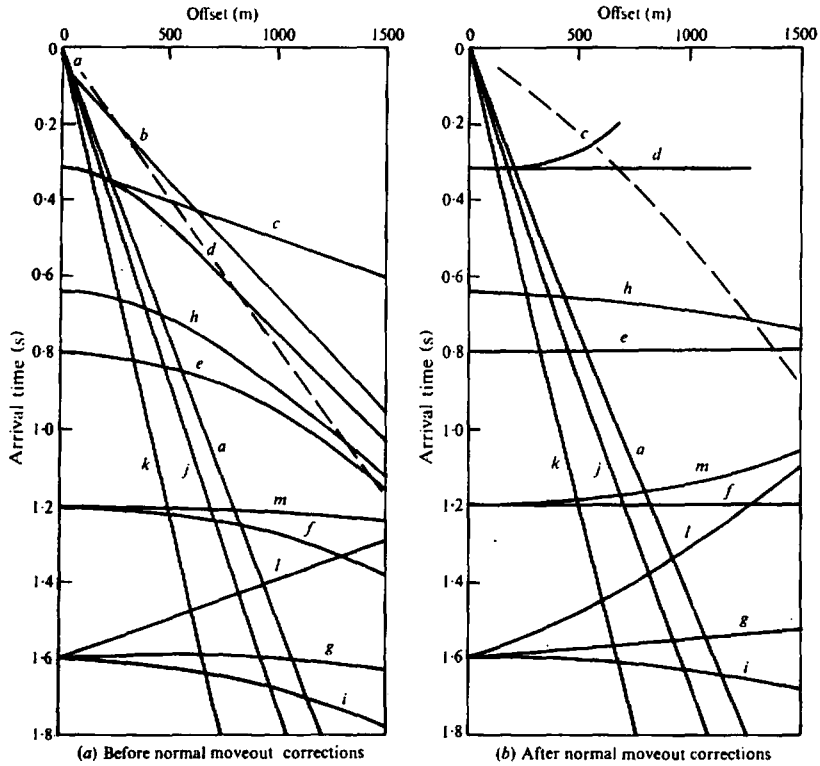
Figure 4.36. Types of events on a seismic record. Identities of events are: a = direct wave, V = 650 m/s; b = refraction at base of weathering, V_H = 1,640 m/s; c = refraction from flat reflector, V_R = 4,920 m/s; d = reflection from reflector c, V_{av} = 1,640 m/s; e = reflection from flat reflector, V_{av} = 1,970 m/s; f = reflection from flat reflector, V_{av} = 2,300 m/s; g = reflection from dipping reflector, V_{av} = 2,630 m/s; h = multiple of d; i = multiple of c; j = ground roll, V = 575 m/s; k = air wave, V = 330 m/s; l = reflected refraction from in-line disruption of the reflector c; m = reflected refraction from broadside disruption of reflector c. After normal-moveout correction, primary reflections are straight. In processing, data are usually muted, that is, data earlier than that indicated by the dashed lines are set to zero so that the data in the upper right corner do not appear.
