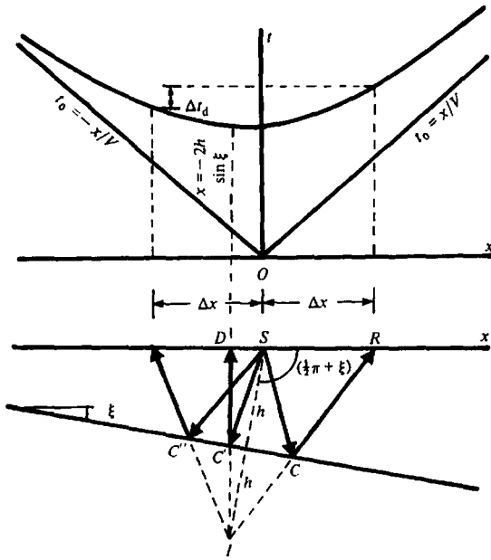
Figure 4.23. Geometry and traveltime curve for dipping reflector.
