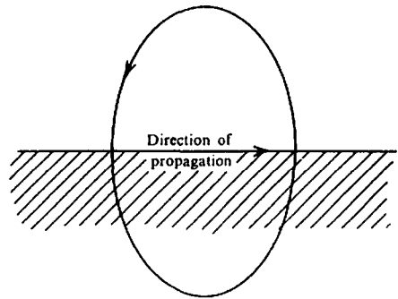
Figure 4.9. Motion during passage of a Rayleigh wave.
