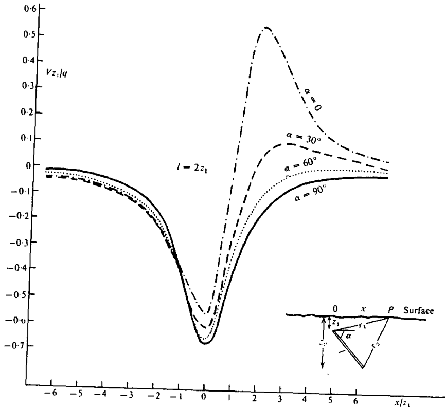
Figure 6.5. SP profiles over buried polarized rod.
