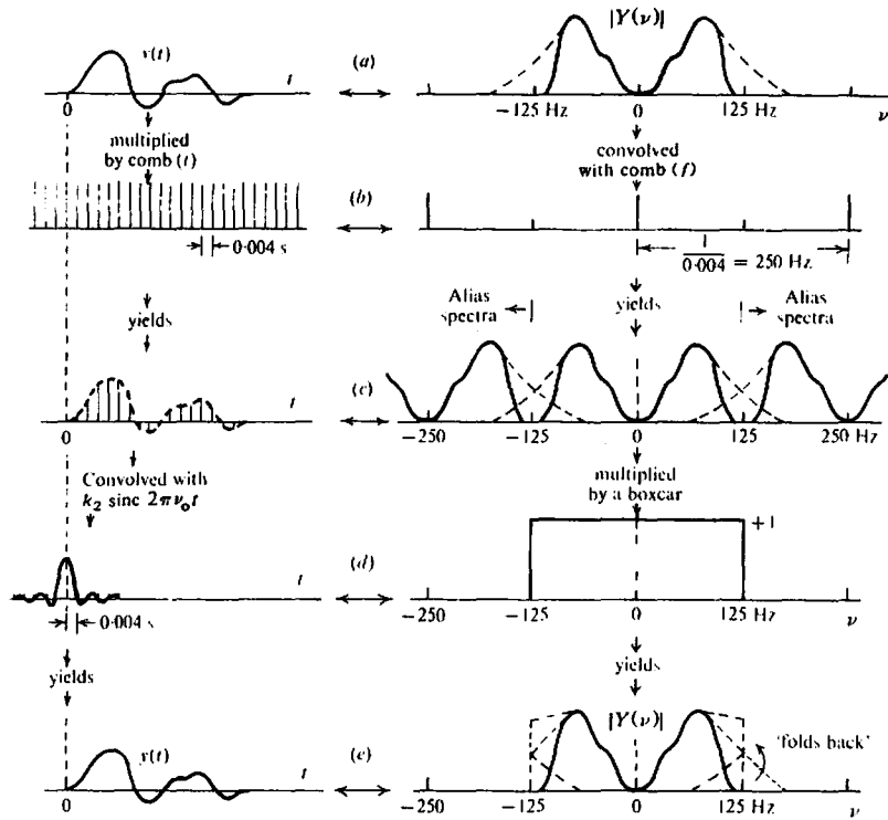
Figure 4.7B. Sampling and reconstituting.
