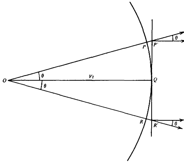
Figure 4.6. Relation between spherical and plane waves.
