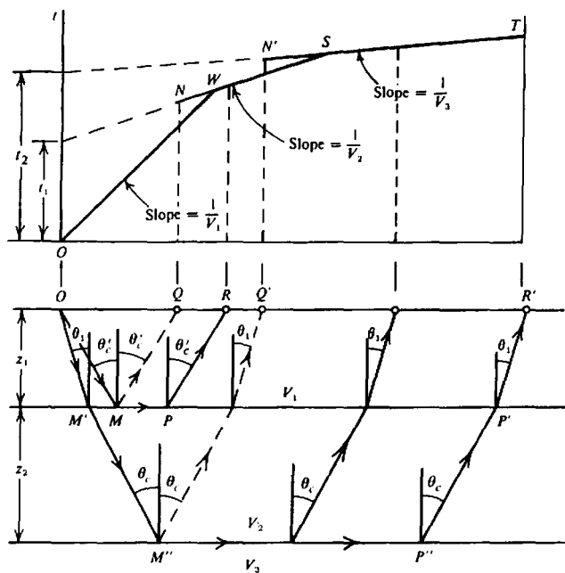
Figure 4.32. Raypaths and traveltime curves for the two-refractor case.
