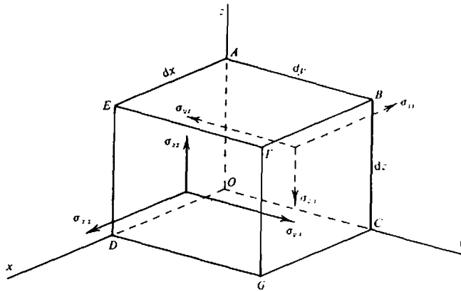
Figure 4.2. Components of stress.
