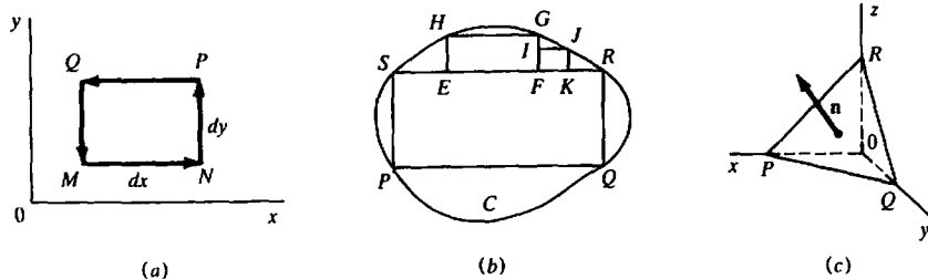
Figure A.3. Derivation of Stokes's theorem. (a) Evaluating a line integral around a rectangle. (b) Evaluating a line integral around an arbitrary closed planar curve C . (c) Resolving a surface integral over a plane triangle into components.
