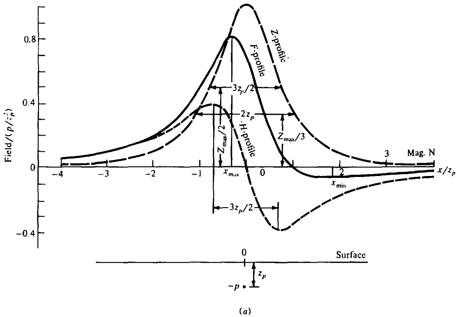
Figure 3.14. Magnetic effects of an isolated pole. (a) F , Z , and H profiles for I = 45^\circ
