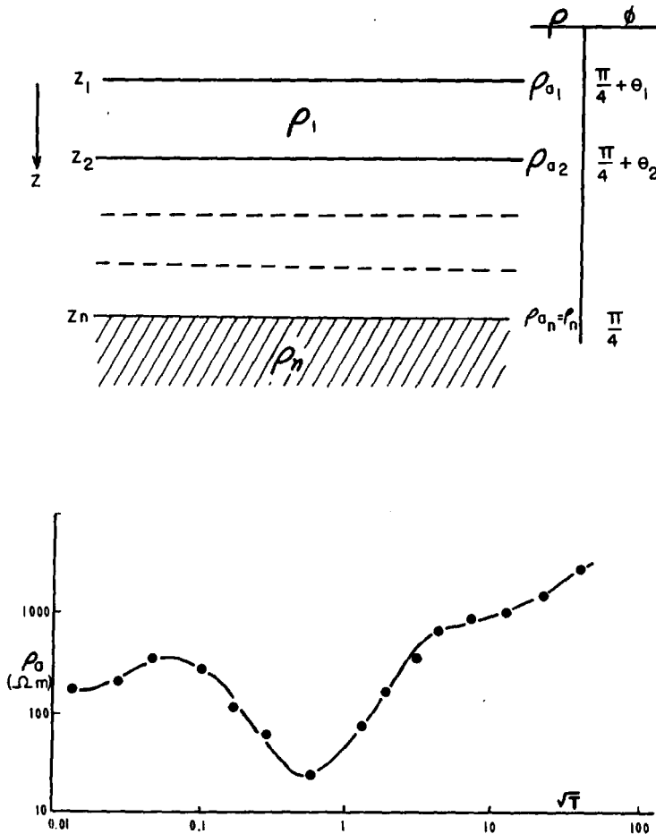
Figure 6.23. Magnetotelluric sounding over multiple beds.
