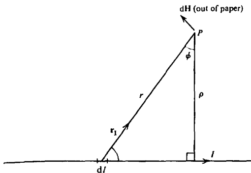
Figure 7.1. Illustrating the Biot-Savart law.
