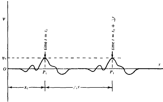
Figure 4.4. Illustrating the velocity of a wave.
