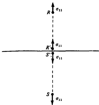
Figure 4.15. Continuity of normal stress.
