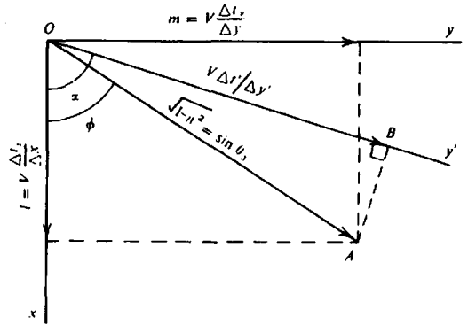
Figure 4.115. Combining dip components.
