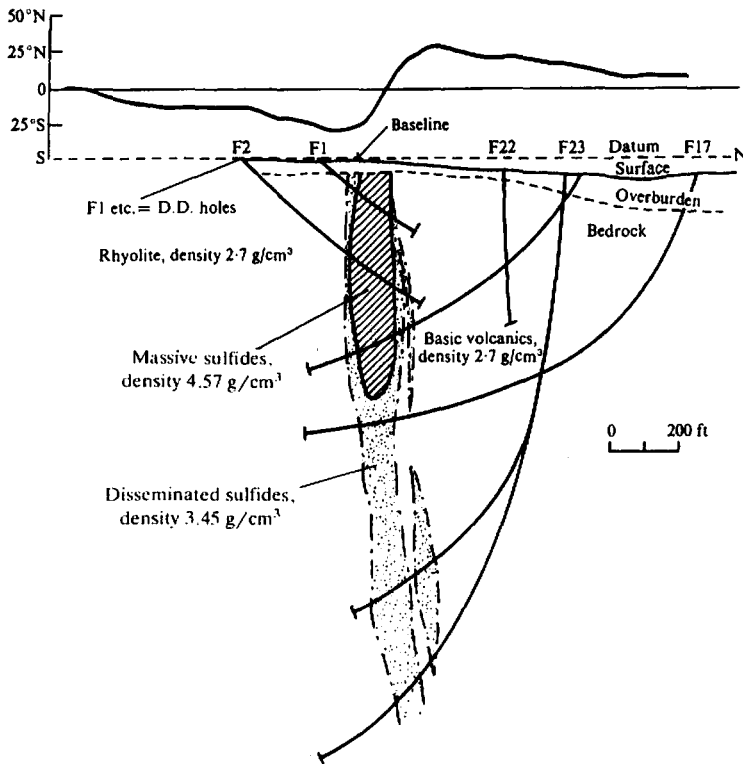
Figure 7.94. Vertical-loop fixed-transmitter profiles over Moberly orebody. (After Seigel, 1957.)
