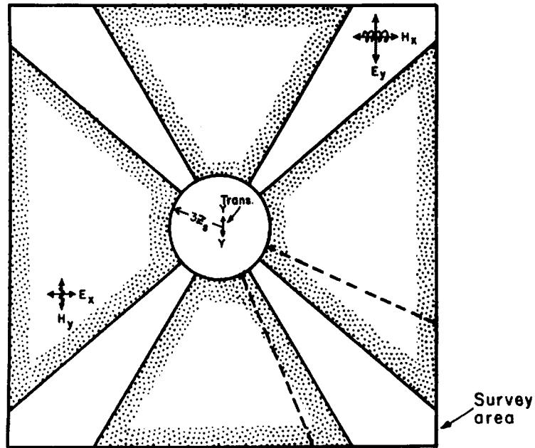
Figure 6.17. AMT survey with dipole source. Shaded areas represent areas with minimum coupling between Y-oriented transmitter (center) and E_x - H_y receiver orientation; dotted lines show approximate limits of strong coupling for E_y - H_x receiver directions. (After Goldstein and Strangway, 1975.)
