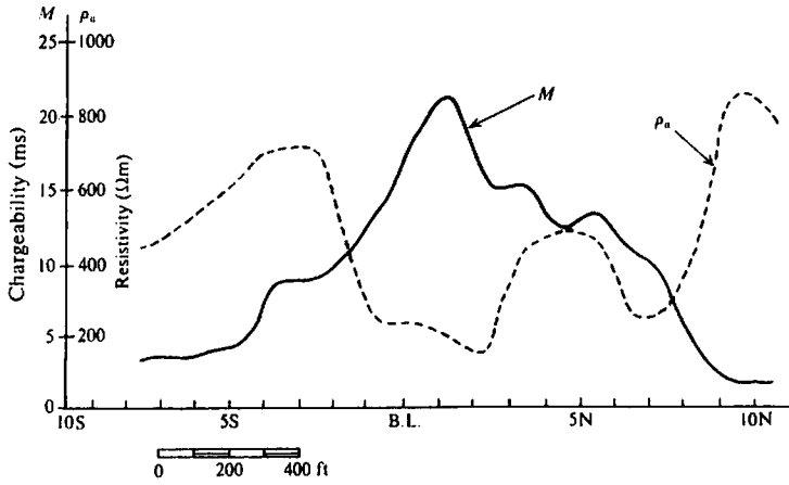
Figure 9.20. IP chargeability and apparent resistivity, Northwest Territories, Canada. (After Seigel, 1967.)
