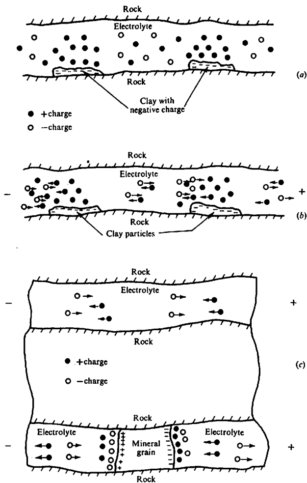
Figure 9.2. Membrane and electrode polarization effects. (a) Normal distribution of ions in a porous sandstone; (b) Membrane polarization in a porous sandstone due to an applied dc voltage; (c) Electrolytic flow in upper pore, electrode polarization in lower pore.
