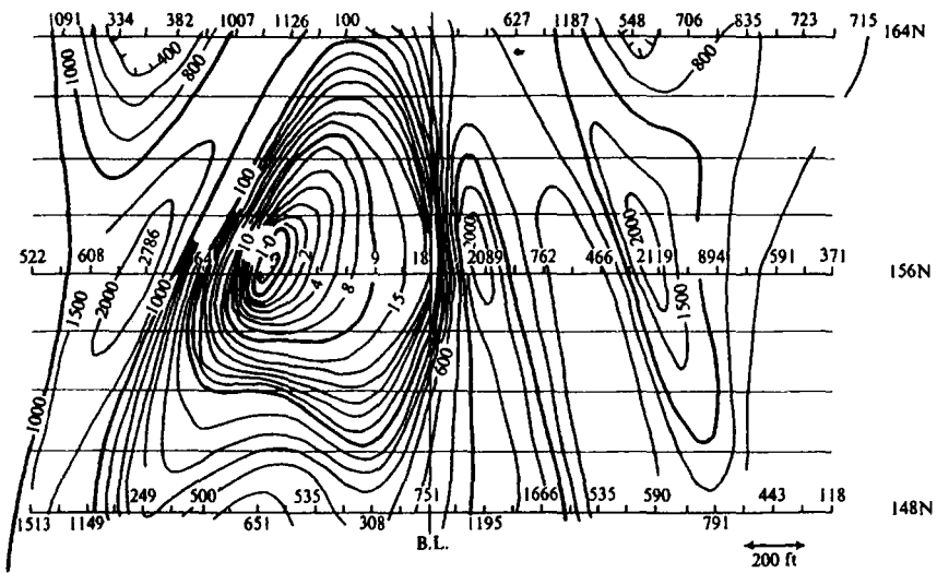
Figure 8.50. Apparent-resistivity contours ( \Omega m ), southern New Brunswick.
