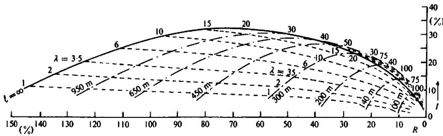
Figure 7.45. Characteristic curves for Turam system over dipping-sheet conductor of infinite depth extent and variable strike length \ell . Depth z = 20 m, dip \phi = 60^\circ , Tx loop 600 \times 1,200 m, \lambda = 10^5/\sigma t f , \mu \approx \mu_0 (mks units).
