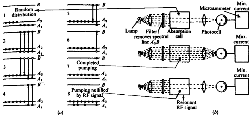
Figure 3.11. Optical pumping. (a) Energy level transitions. (b) Effect of pumping on light transmission.
