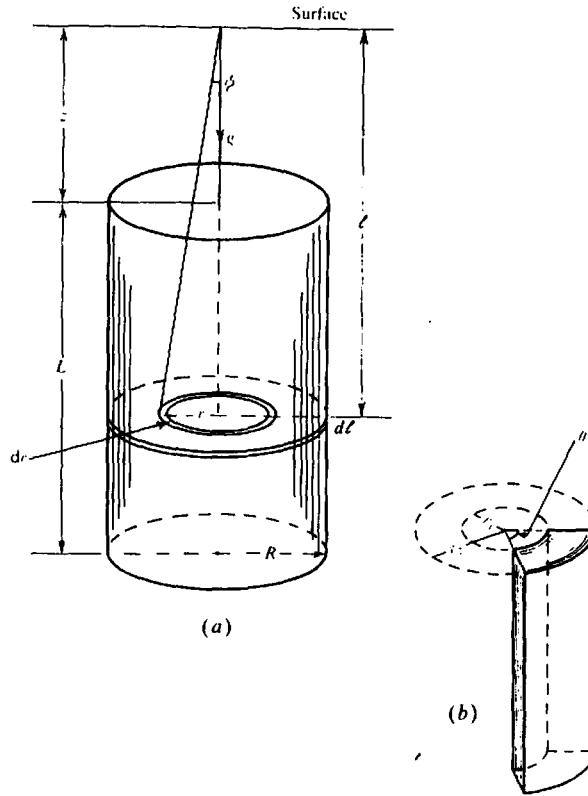
Figure 2.25. Gravity effect of a vertical cylinder. (a) Calculation of gravity over the axis. (b) Geometry of a cylindrical slice.
