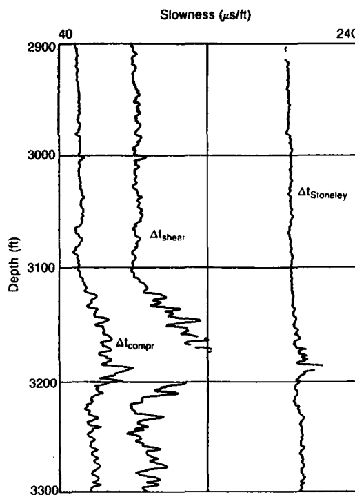
Figure 11.28. Log of P -, S -, and Stoneley-wave transit times. (From Schlumberger, 1987.)
