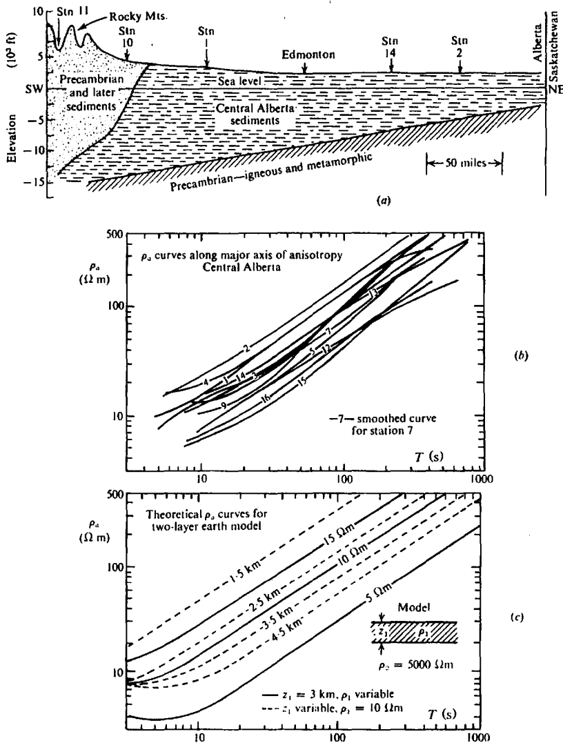
Figure 6.27. Magnetotelluric deep soundings in Central Alberta. (After Reddy and Rankin, 1971.) (a) Geological section. (b) \rho_a curves along major axis of anisotropy. (c) Theoretical \rho_a curves for two-layer earth.
