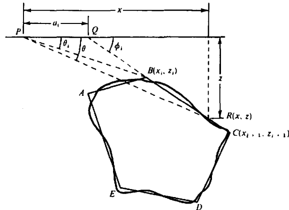
Figure 2.34. Polygon approximation of an irregular vertical section of a two-dimensional body.
