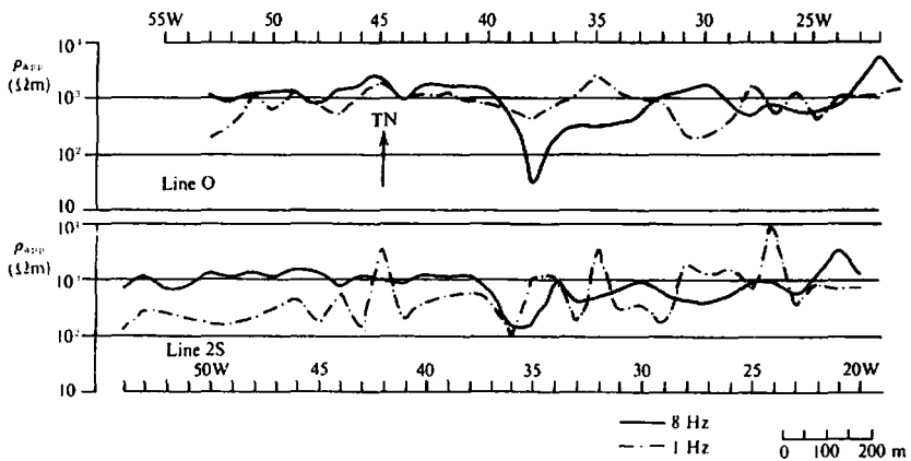
Figure 6.35. Telluric profiles at 1 and 8 Hz, Northeastern Brazil.
