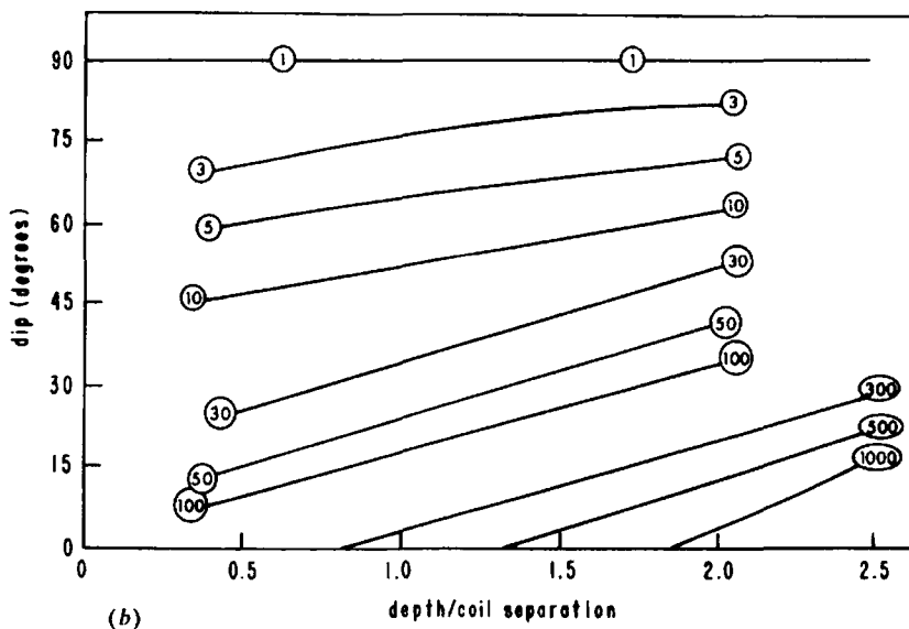
Figure 7.66. Characteristic curves for a dipping-model plate. (Parts a, c: After Gallagher, Ward, and Hohmann, 1985; part b: After Bartel and Hohmann, 1985.) (a) Early- and late-time peak ratio as a function of depth and dip, EM37; (b) Ratio of on-conductor side-lobe area to off-conductor side-lobe area as a function of dip and depth, PEM(1).
