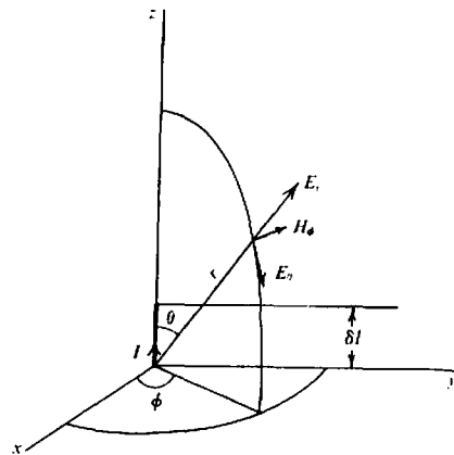
Figure 7.4. Field of a short vertical wire at a distant point.
