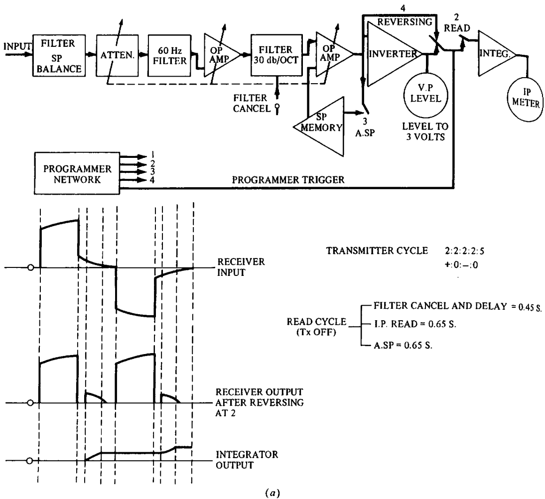
Figure 9.6. Block diagrams of typical IP receivers. (a) Newmont T-D receiver. (After Dolan and McLaughlin, 1967.)
