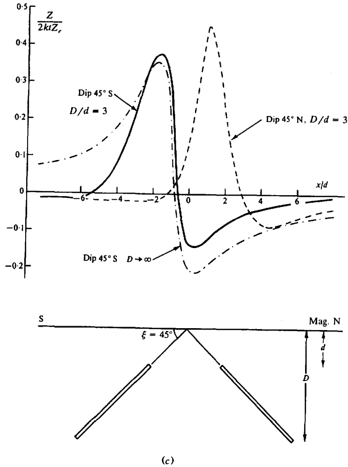
Figure 3.20. (Continued) (c) Z profiles for E-W strike, \xi = 45^\circ\text{N} and 45^\circ\text{S} , \beta = 90^\circ .
