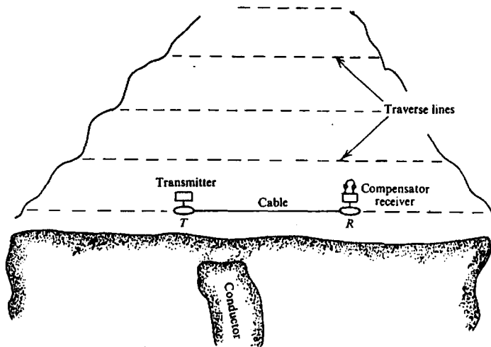
Figure 7.20. Horizontal-loop system.
