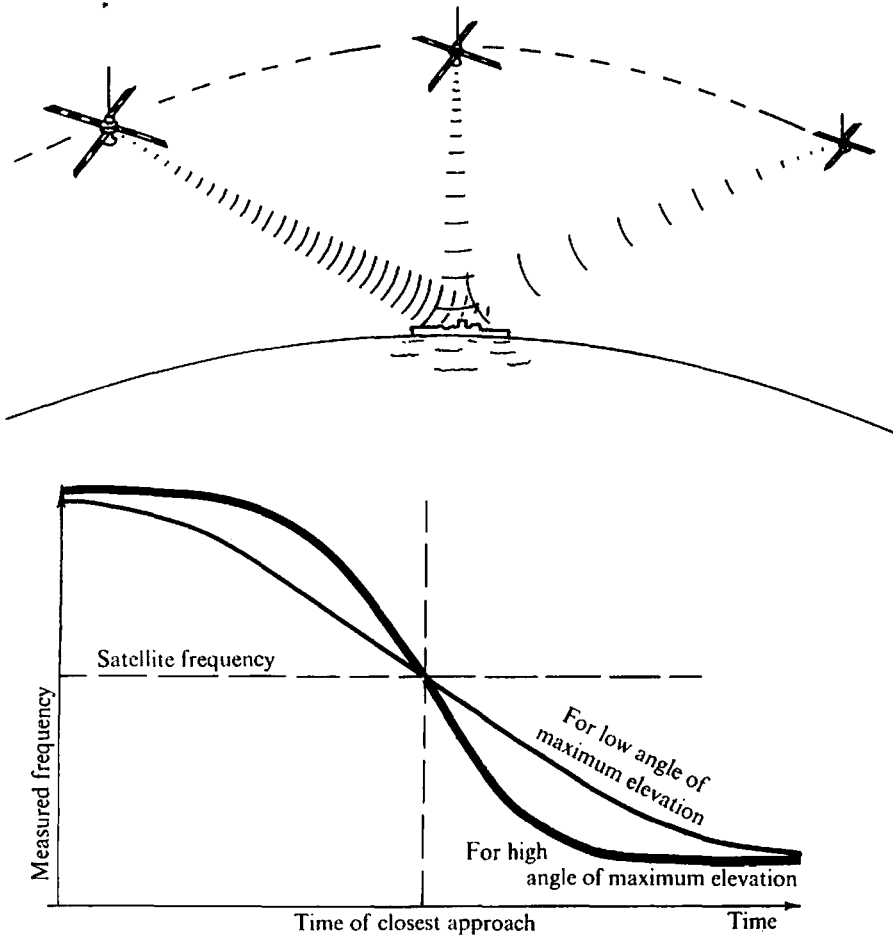
Figure B.4. Position-fix from navigation satellite. (From Sheriff, 1973.)
