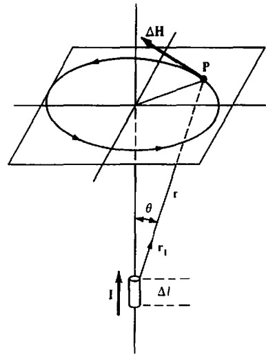
Figure 3.1. Ampère's law. A current I through a length of conductor \Delta l creates a magnetizing field \Delta H at a point P :
