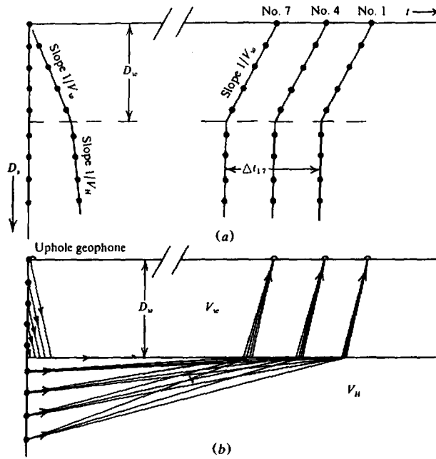
Figure 4.50. Uphole survey. (a) Traveltime versus shot depth. (b) Vertical section showing raypaths.
