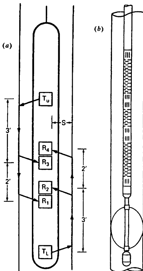
Figure 11.23. Sonic logging sonde. (a) Borehole-compensated sonde. (b) The sonde in a borehole. Vertical slits are openings to transmitters and receivers; horizontal slits prevent signal travel in the sonde itself.
