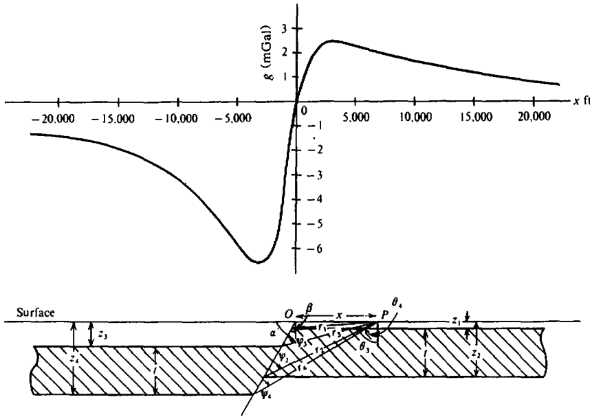
Figure 2.32. Gravity effect of a faulted horizontal bed; t = 1,200 m, z_1 = 150 m, z_2 = 1,350 m, z_3 = 600 m, z_4 = 1,800 m, \alpha = 60^\circ , and \rho = 1 g/cm 3 . (From Geldart, Gill, and Sharma, 1966.)
