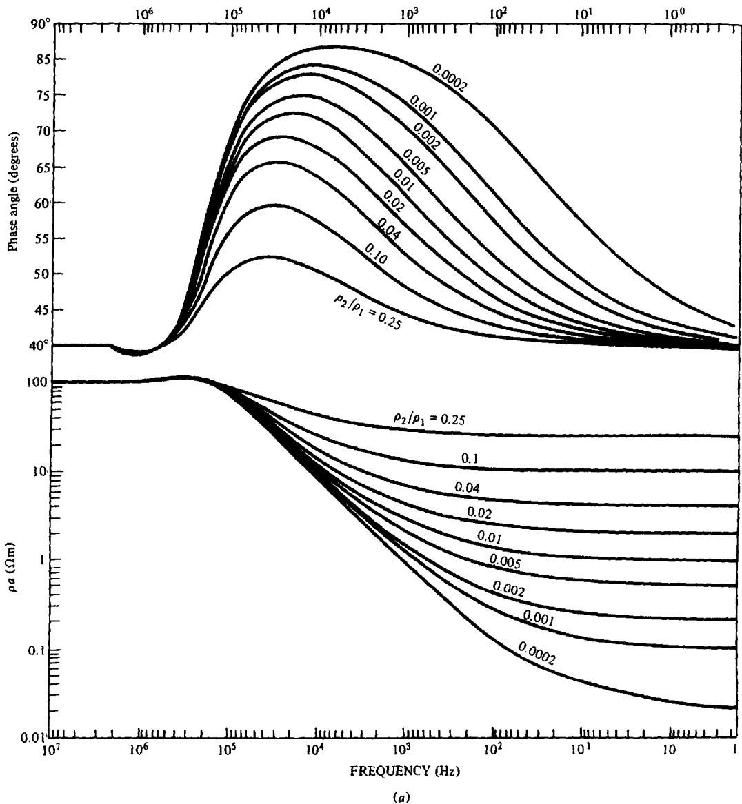
Figure 6.22. Master curves for MT sounding over two-layer earth. \rho_1 = 100 \Omega\text{m} and z_1 = 10 \text{ m} . (a) \rho_2 < \rho_1 .
