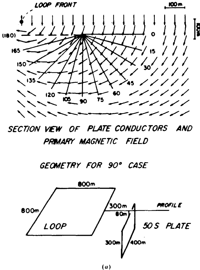
Figure 7.61. UTEM profiles over a dipping-plate model. (After West, Macnae, and Lamontagne, 1984.) (a) Geometry and dimensions of the model, and configuration of the primary field in the vicinity of the conductive plate.
