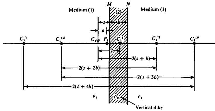
Figure 8.35. Locations of current images near a vertical dike.
