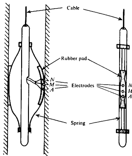
Figure 11.5. Microlog wall-resistivity arrangement.
