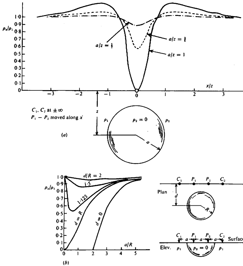
Figure 8.37. Resistivity profiles over three-dimensional conductors. (a) Schlumberger array over buried sphere. (b) Expanding Wenner array over outcropping hemispherical conductor.
