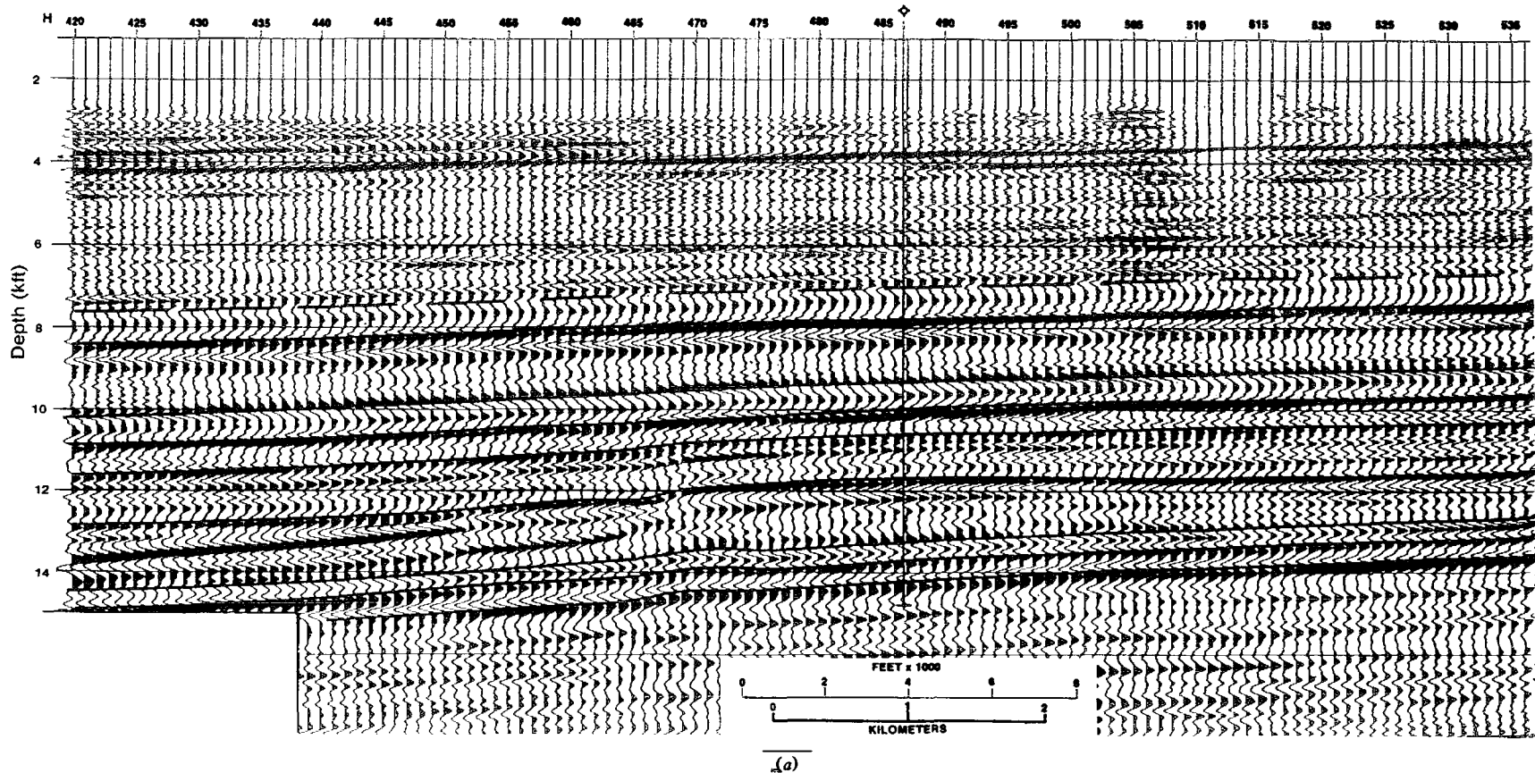
Figure 4.104. Section across a Louisiana reef. (From Phelps and Roripaugh, 1983.) (a) Seismic section where the vertical scale is linear with depth.
