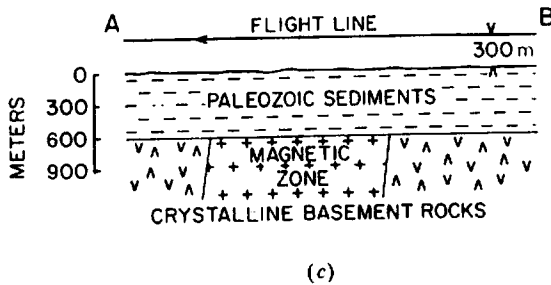
Figure 3.33. Belec Lake anomaly, Ontario. (From McGrath and Hood, 1973.) (a) Aeromagnetic map of the anomaly. (b) Profile AB and the anomaly computed from the model. (c) Inferred geological cross section.
