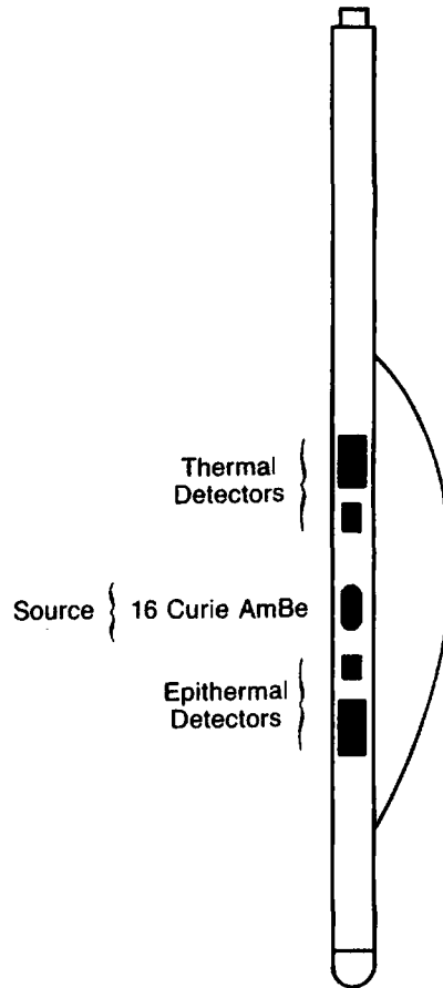
Figure 11.38. Schematic of dual-porosity neutron logging sonde. (From Schlumberger, 1987.)
