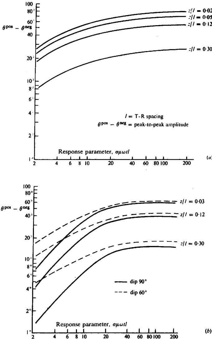
Figure 7.43. Characteristic curves for semiinfinite sheet. (From Ward, 1967). (a) Fixed-transmitter dip-angle system, vertical sheet. (b) Broadside array, dipping sheet.
