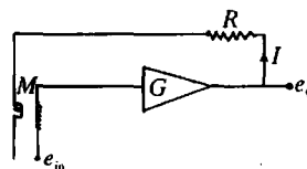
Figure 7.24. Feedback circuit to convert \partial H/\partial t signal to H .
