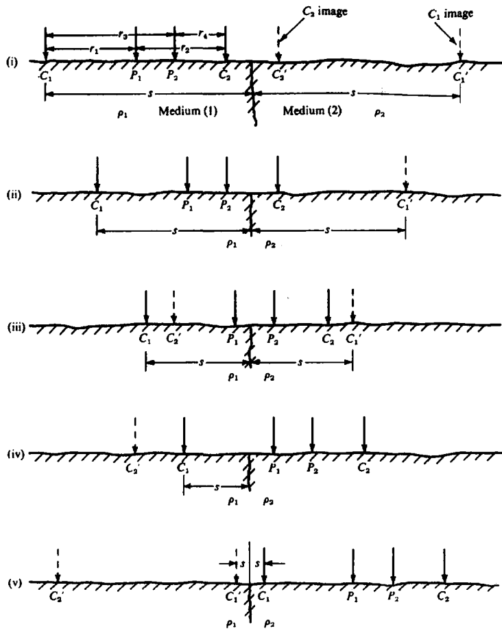
Figure 8.33. General resistivity spread over a vertical contact.
