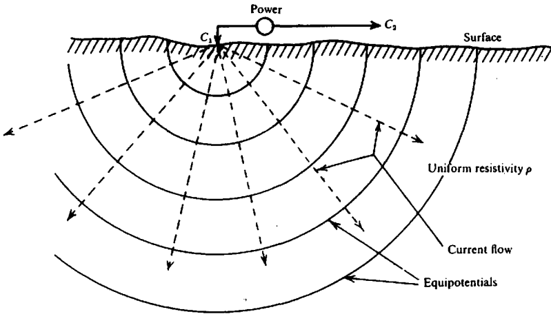
Figure 8.2. Point source of current at the surface of a homogeneous medium.
