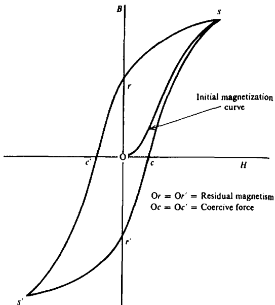
Figure 3.2. Hysteresis loop. s, s' = saturation, r and r' = remanent magnetism, c and c' = coercive force.
