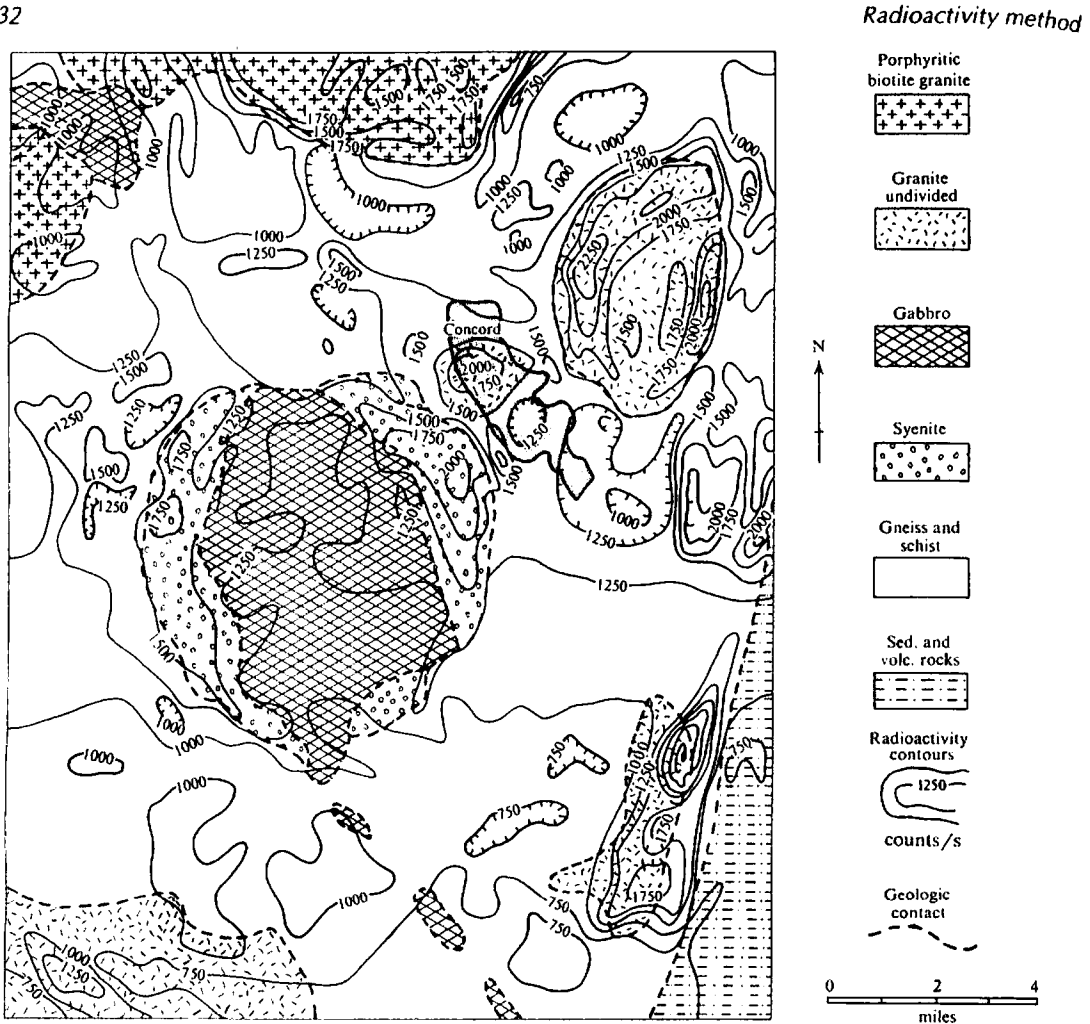
Figure 10.12. Airborne radiometrics as an aid to geological mapping, Concord Quadrangle, North Carolina. (After Bates, 1966.)
