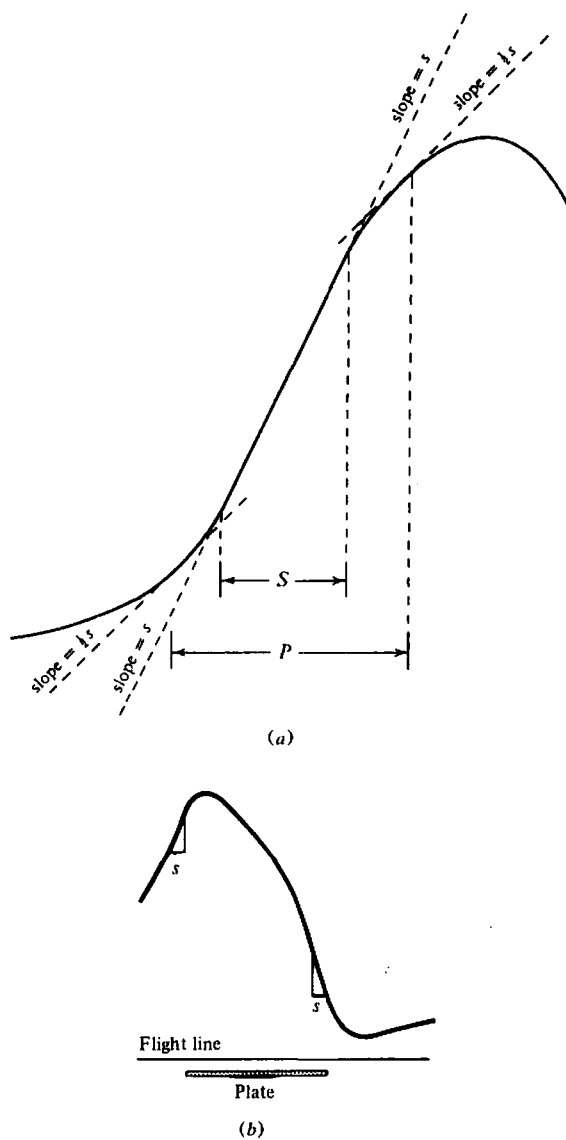
Figure 3.27. Determining anomaly depth from the slope of a magnetic profile. (a) Maximum-slope ( S ) and half-slope ( P ) measurements. (b) Maximum-slope measurements on a thin plate anomaly.
