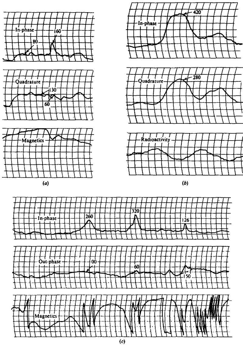
Figure 7.120. Typical response curves of the airborne phase-component EM system (Aero-Newmont) plus airborne magnetics and radiometric curves. (After Wieduwilt, 1962.) (a) Phase-component and magnetic curves. (b) Phase-component and radioactivity curves. (c) Same as in (a).
