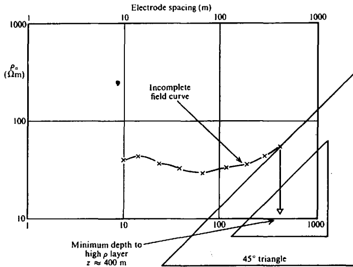
Figure 8.23. Asymptote method of estimating minimum depth.
