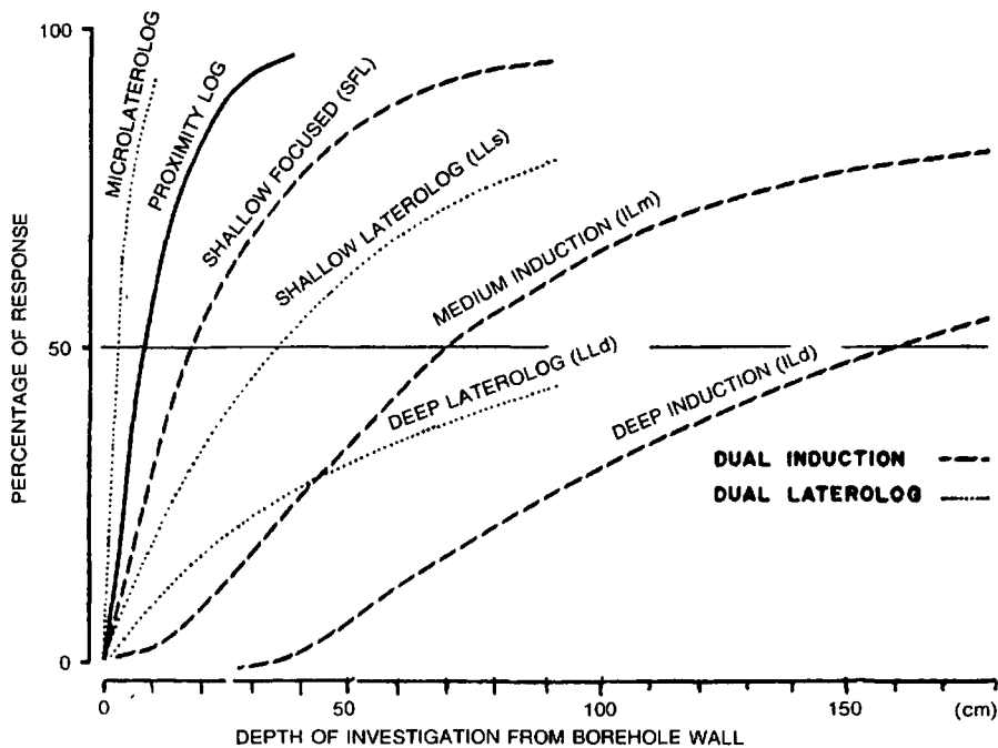
Figure 11.2. Percent of response attributable to rocks within different distances from the borehole for infinite homogeneous medium. (After Schlumberger, 1972).
