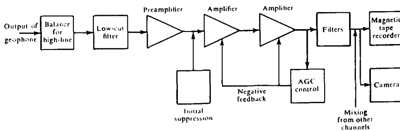
Figure 4.55. Block diagram of analog seismic amplifier.
