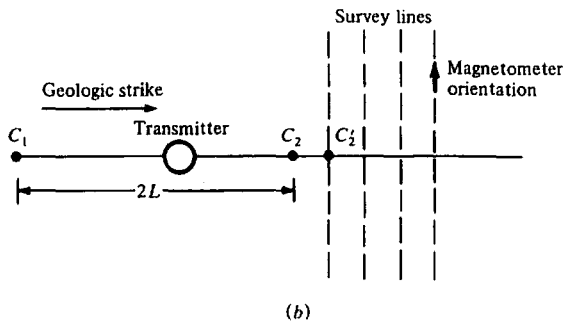
Figure 9.9. Magnetic IP arrays. (After Seigel, 1983.) (a) Horseshoe array for reconnaissance. (b) Linear array for detail surveying.
