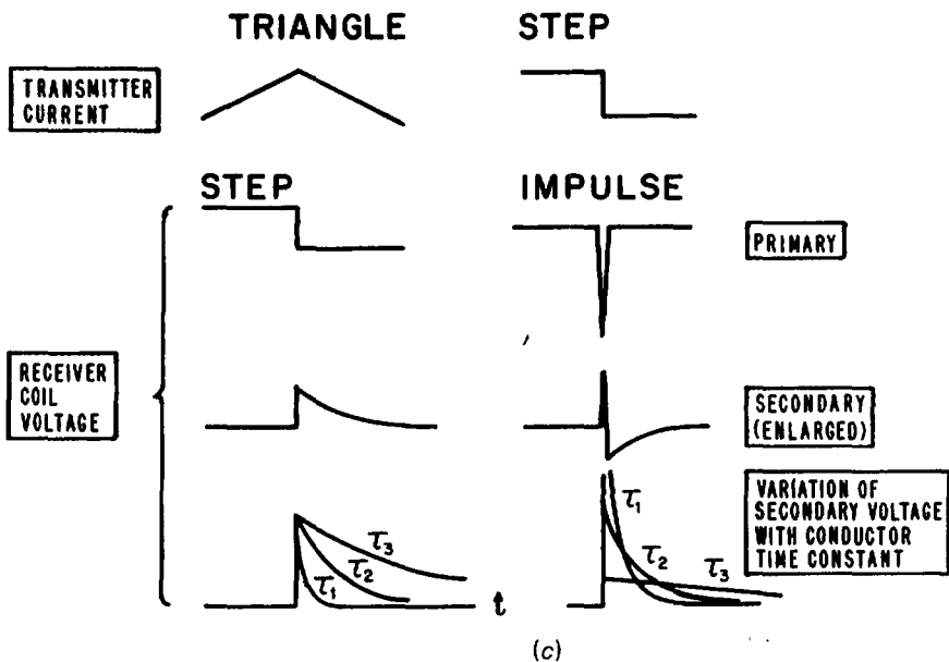
Figure 7.23. (Continued) (c) Comparison of signals for triangular and step-function inputs.
