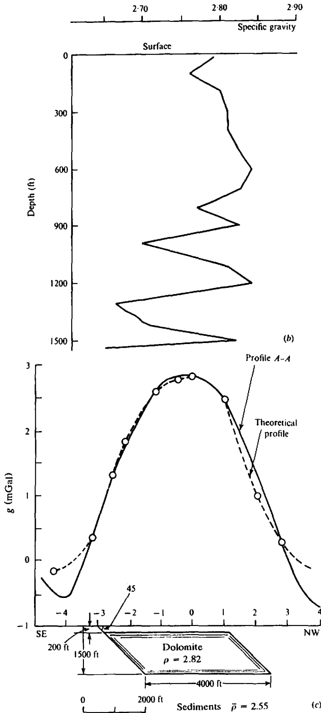
Figure 2.36. (Continued) (b) Density log in borehole DDH PCI-70. (c) Comparison with calculated profile for a 2-D dipping prism.
