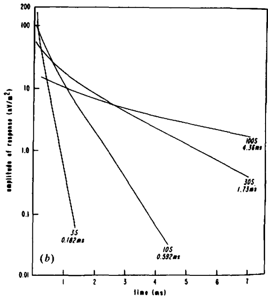
Figure 7.67. Nomograms for estimating at product. (a) PEM(1) system, channel ratios versus TCP (numbers at ends of curves denote channels); model plate 600 \times 600 m, z = 50 m, dip = 30^\circ , T-R = 100 m. (After Bartel and Hohmann, 1985.) (b) EM37 system, curves of response amplitude versus time for various values of TCP (or time constant); model plate 800 \times 400 m, z = 50 m, dip = 90^\circ . (After Gallagher, Ward, and Huhmann, 1985.)
