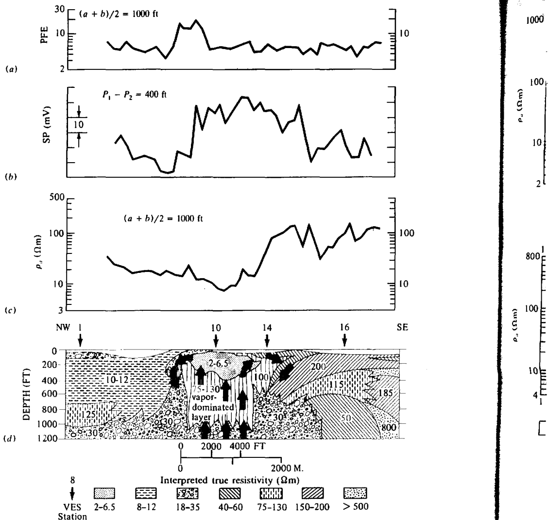
Figure 8.43. IP, SP, and resistivity profiles with geoelectric section, Mud Volcano, Yellowstone National Park geothermal zone. (After Zohdy, Anderson, and Muffler, 1973.)
