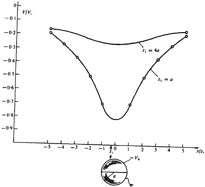
Figure 6.6. SP profiles over buried polarized sphere.
