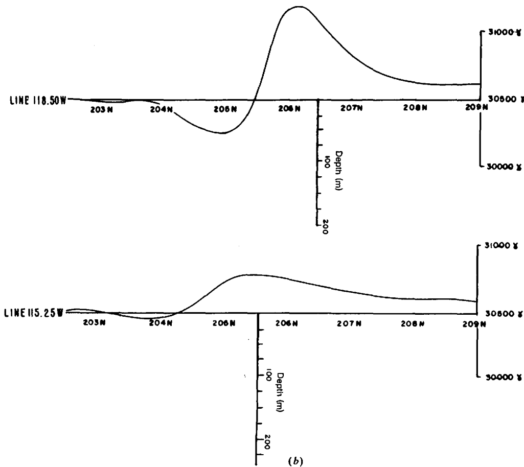
Figure 7.118. (Continued) (b) Total-field magnetics on lines 118.50W and 115.25W.
