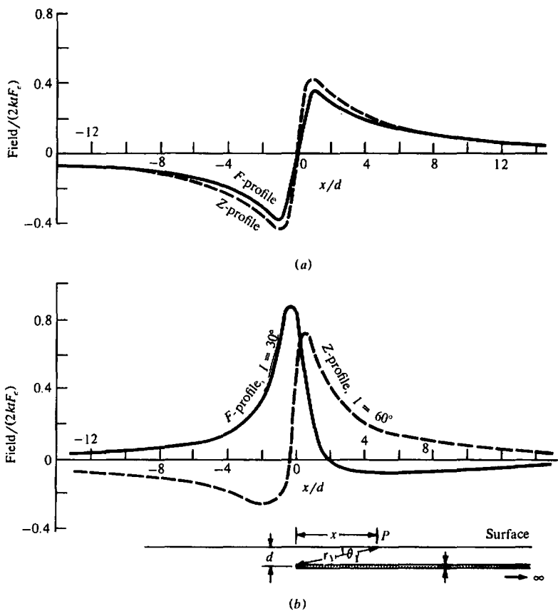
Figure 3.22. Semiinfinite horizontal sheet. F , Z profiles for (a) N-S strike, I = 60^\circ ; (b) E-W strike, I = 60 and 30^\circ .
