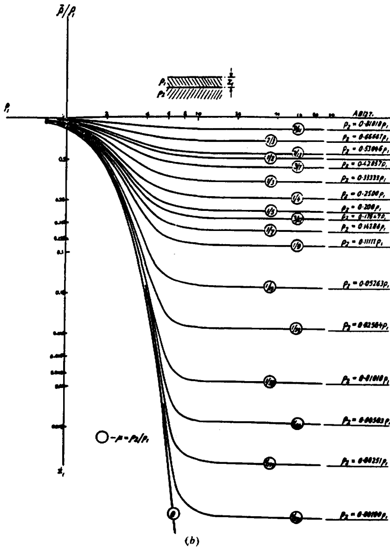
Figure 8.27. (Continued) (b) Descending type ( \rho_2 < \rho_1 ).
