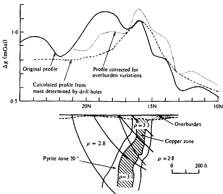
Figure 2.37. Gravity profiles over a copper deposit, Louvicourt, Quebec.
